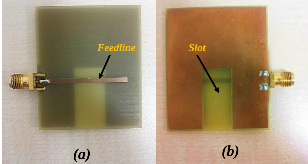
Figure 3.7. Fabricated microstrip single-slot antenna: a) Backside with the feed-line and b) front side with the slot.
