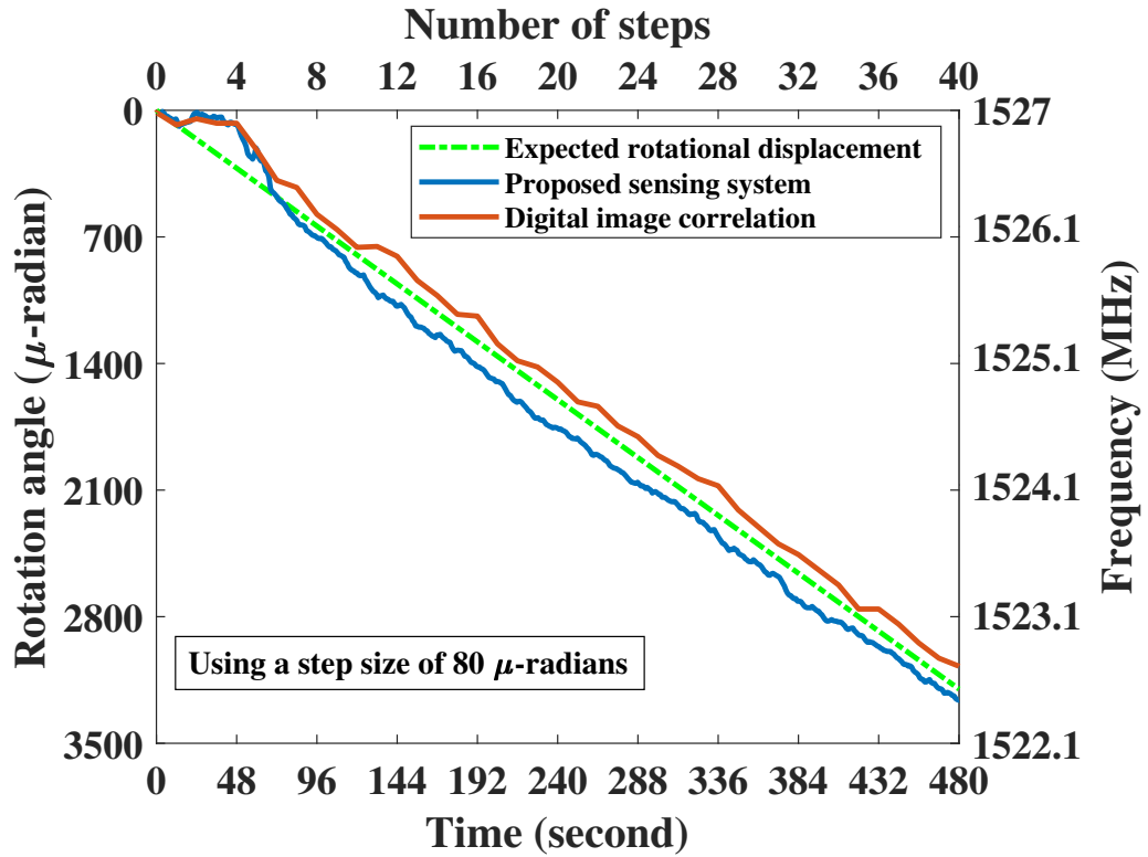
Figure 4.12. Comparing the experimental results of the proposed sensing method with the DIC method for a 80- \mu -radian resolution level, shown along with the expected rotational displacement generated by moving the translation stage.
