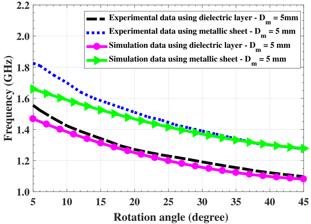
Figure 4.5. Shift in the operating frequency versus the rotation angle.
