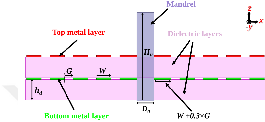
Figure 3.3. Cross-sectional view of the overlapped configuration at the rotation angle of \theta=20^\circ , which corresponds to the MDMD arrangement of layers.
