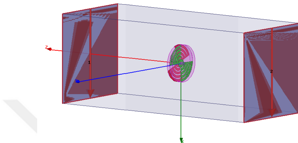
Figure 3.8. Simulating the proposed sensor inside a waveguide.
