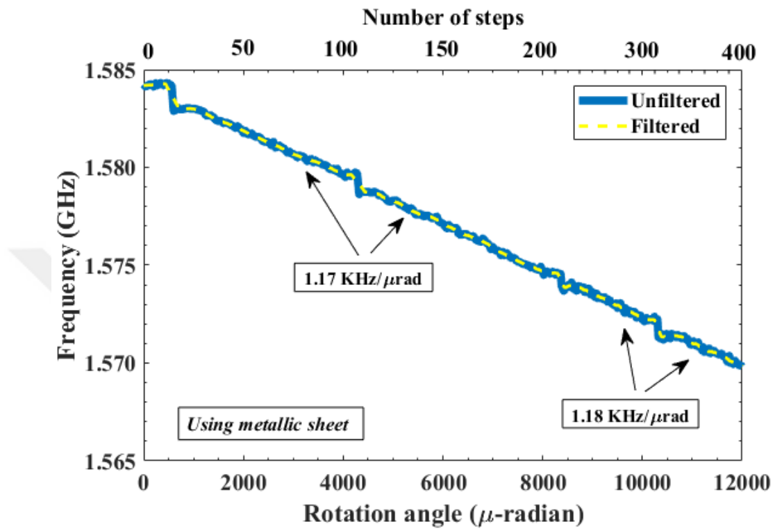
Figure 4.9. Resolution test using metallic sheet (with 5 min pausing after every 100 steps).
