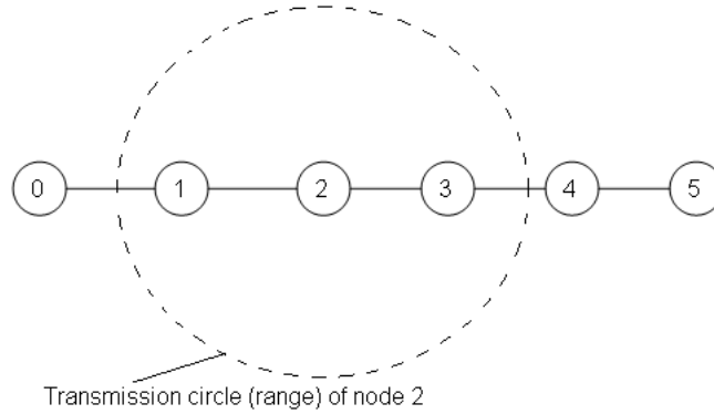
Figure 3.1: The hidden and exposed terminal problems.
