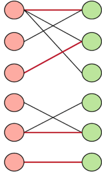
Figure 4.5: Bipartite matching
