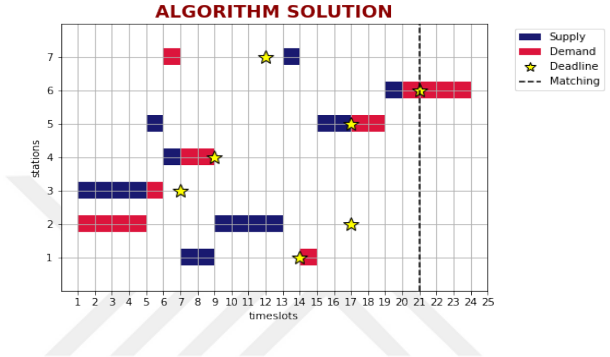
Figure 5.1: Deadline algorithm solution schedule of an instance with 7 stations
