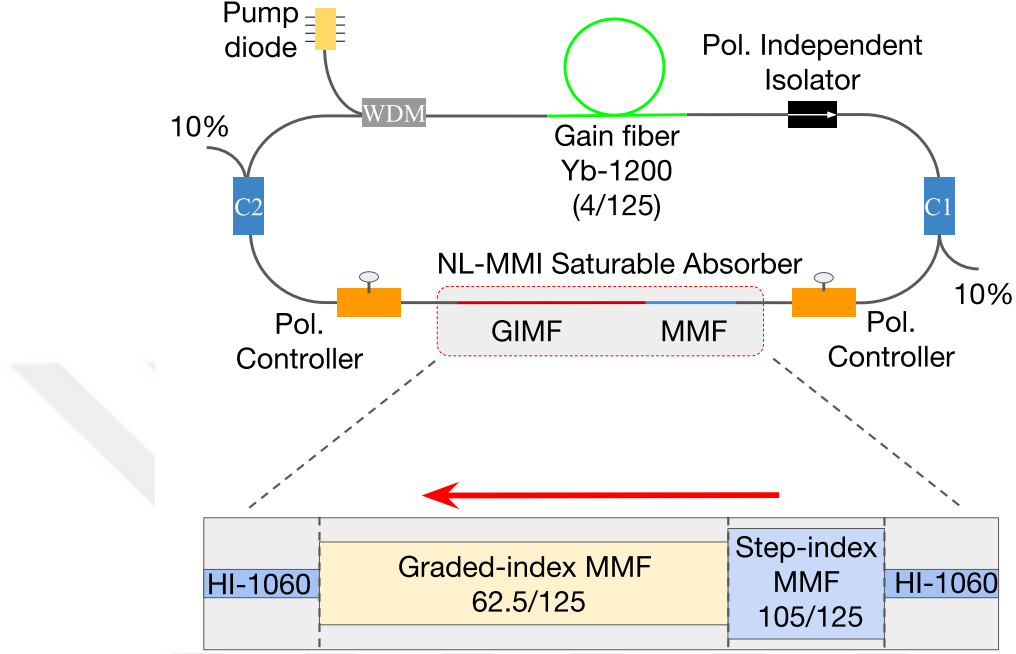
Figure 5.1: Schematic of the all-fiber Yb-doped laser with NL-MMI based saturable absorber: WDM, wavelength division multiplexer; GIMF, graded-index multimode fiber; MMF, multimode fiber.
