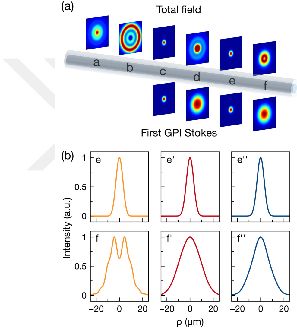
Figure 3.2: Numerical results for spatial evolution inside the graded-index MMF with 50\mu\text{m} core diameter. (a) Spatial intensity distributions at 2 cm, 5 cm, 17.03 cm, 17.12 cm, 17.21 cm, 17.28 cm (a-f). (b) Beam profiles of total field (e, f), first Stokes sideband (e', f') and first anti-Stokes sideband (e'', f'') for 17.21 and 17.28 cm of the fiber, respectively.
