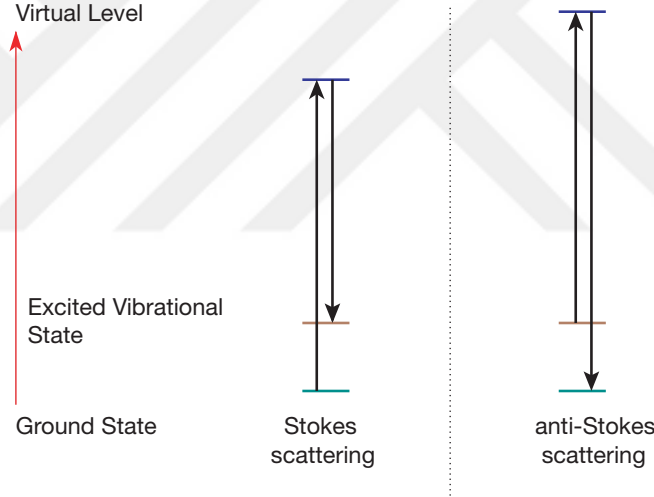
Figure 2.4: Quantum mechanical illustration of Raman Stokes and anti-Stokes scattering.
