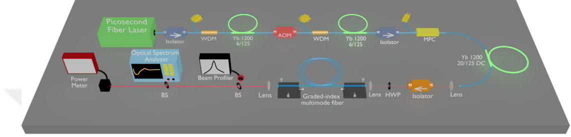
Figure 4.1: Schematic of the experimental setup comprising of Yb-doped fiber, wavelength division multiplier (WDM), beam splitter (BS), acousto-optic modulator (AOM), multi-pump combiner (MPC), three-dimensional stage (3DS), half-wave plate (HWP).
