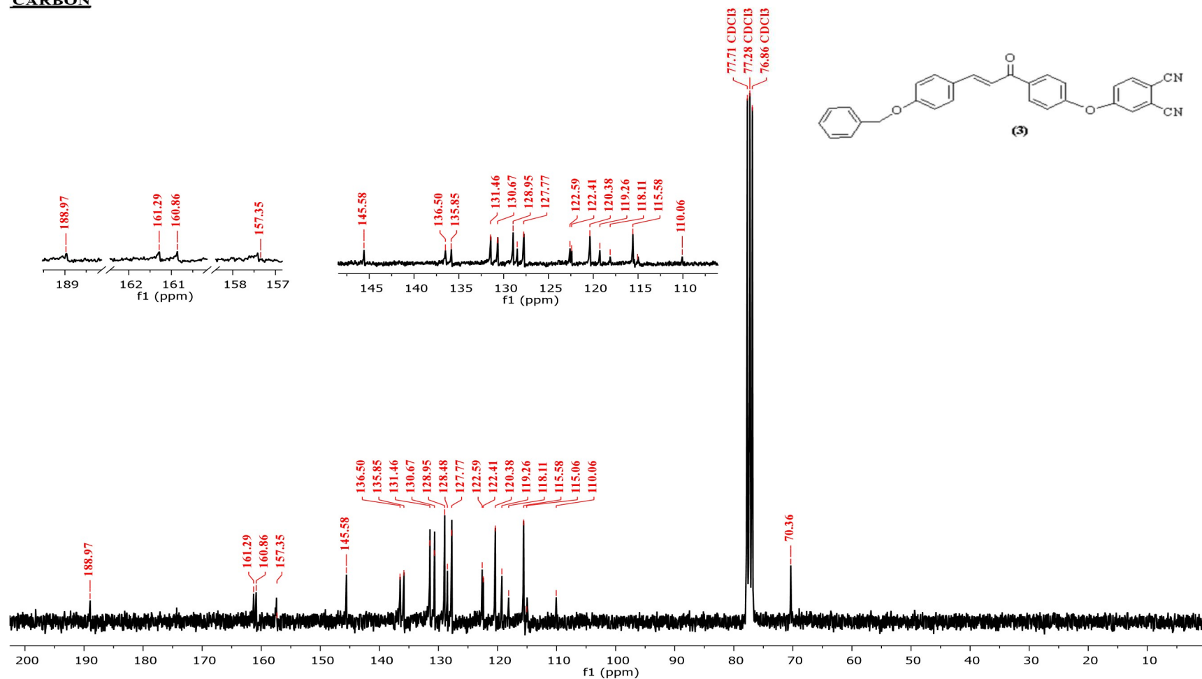
EK 8: (E)-4-(4-(3-(4-(benziloksi) fenil) akriloi) fenoksi) ftalonitril ( 3 ) ^{13}\text{C} NMR spektrumu (75 MHz, \text{CDCl}_3 )
