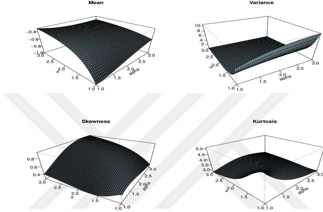
Figure 4: The plots for location, spread and shape measures of the ASGN distribution.
