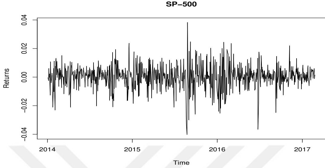
Figure 16: Daily log-returns of S&P-500 index
