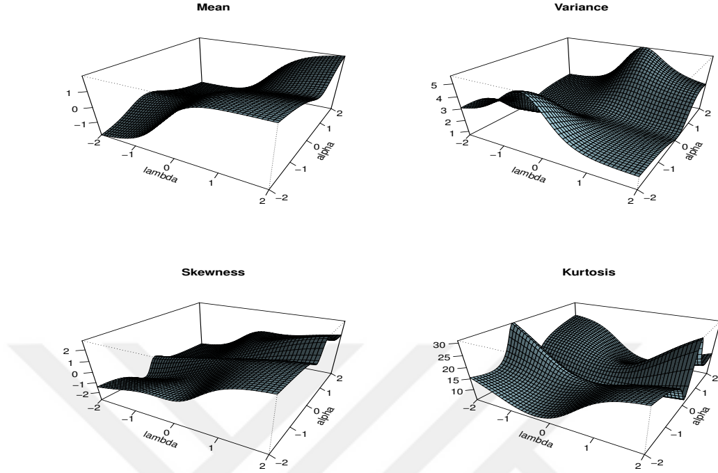
Figure 8: The plots for location, spread and shape measures of GAST distribution for \nu = 7
