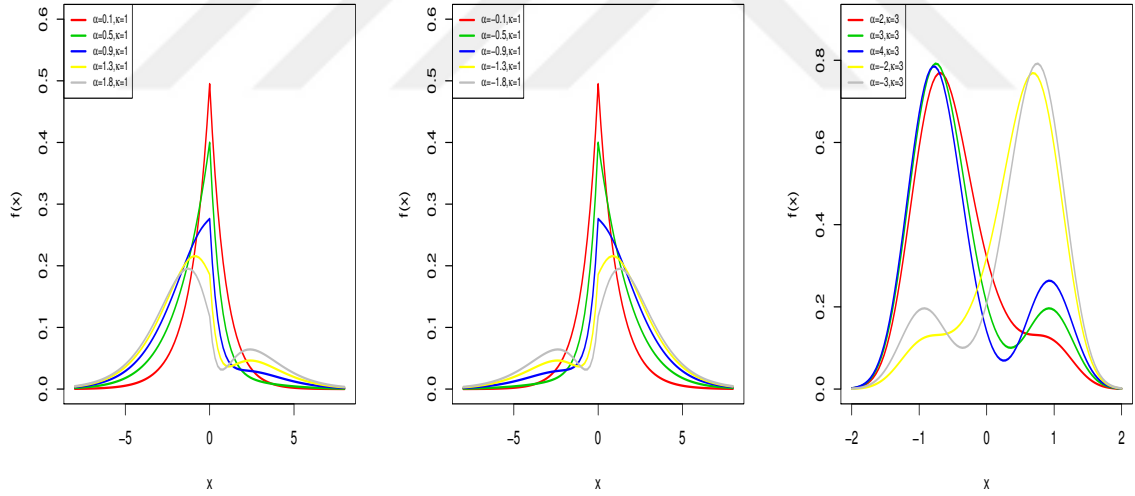
Figure 3: Plots of density functions for the ASGN distribution for several parameter values.
