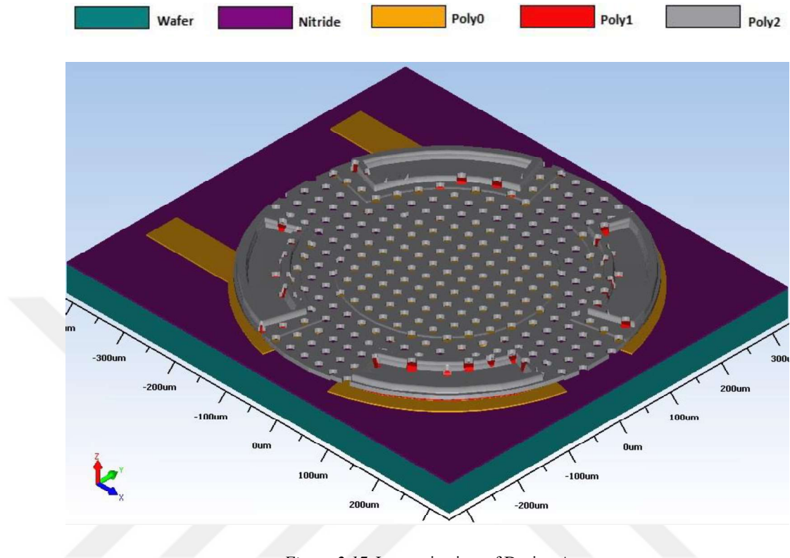
Figure 2.17. Isometric view of Design A
