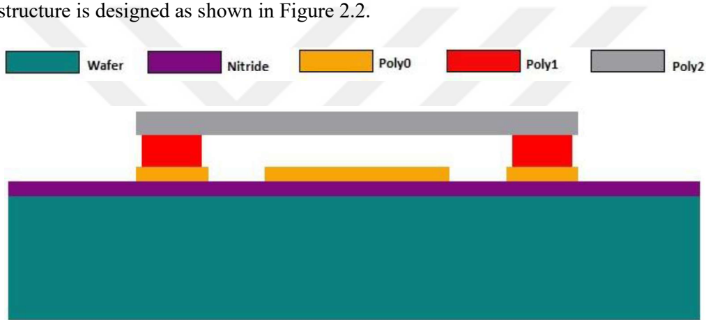
Figure 2.2. General structure of the proposed design
