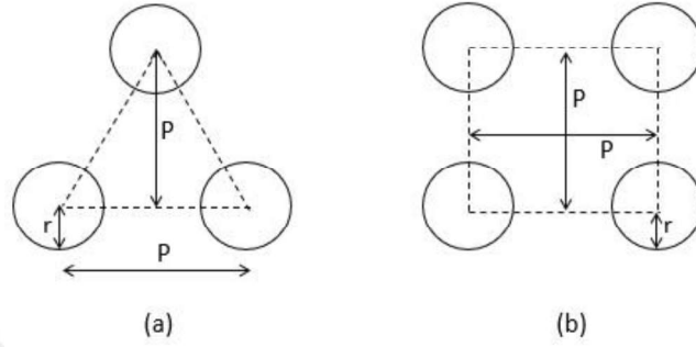
Figure 2.9. Dimensional representation of the perforation types
