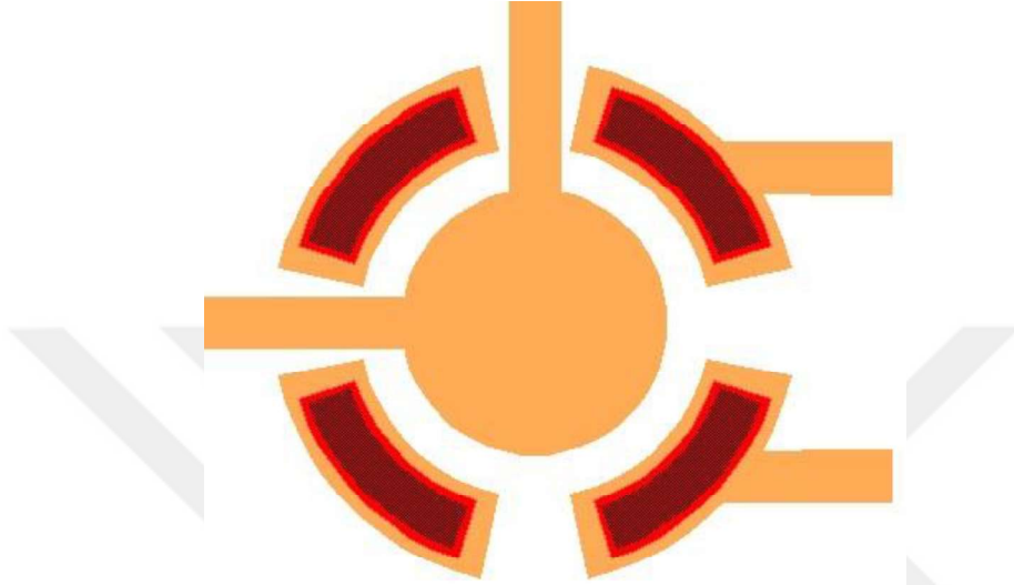
Figure 2.12. POLY0 (orange), ANCHOR1 (gray) and POLY1 (red) masks
