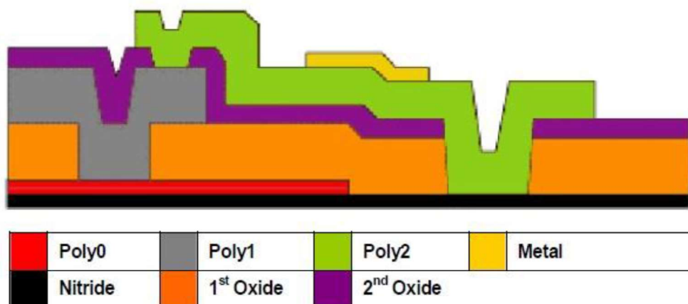
Figure 2.1. Cross sectional view of PolyMUMPs layers [25]
