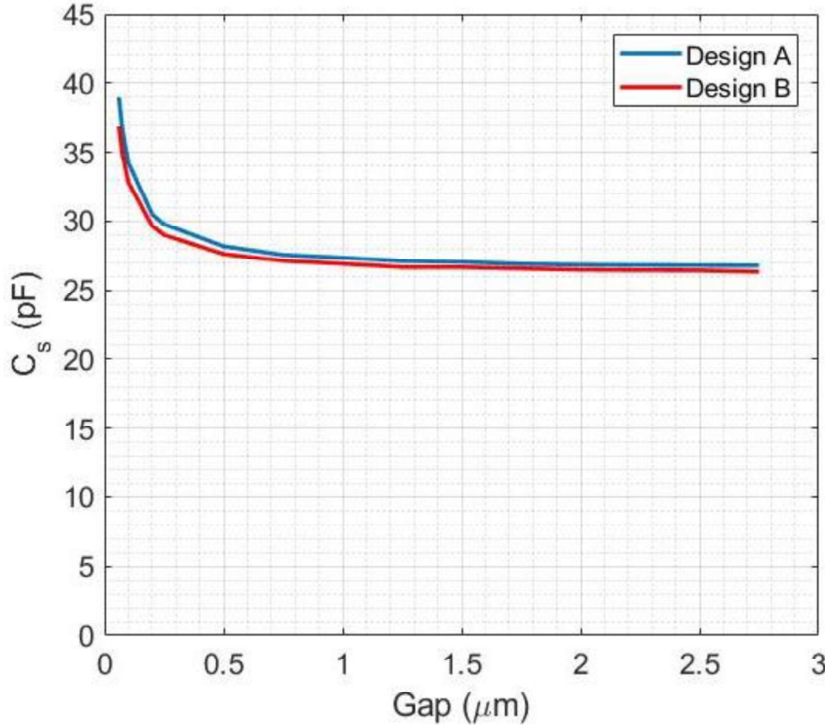
Figure 3.9. Series capacitance extraction of the proposed designs as a function of gap
