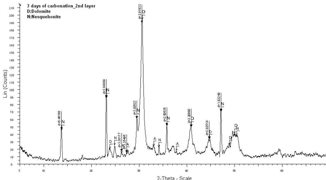
Figure 79. XRD traces of carbonation products in petri dish, bottom layer, 3 days of carbonation
