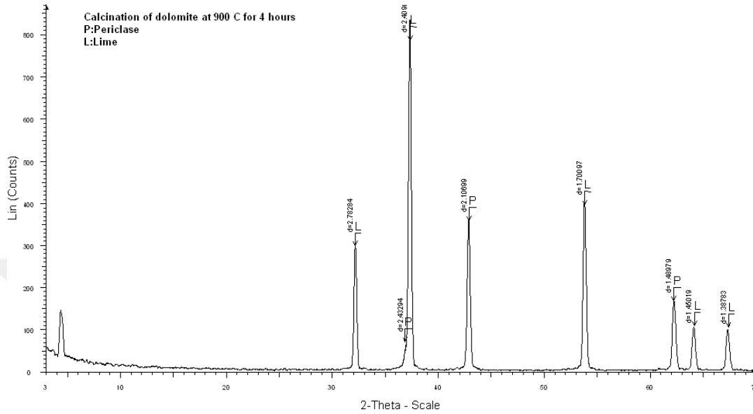
Figure 30. XRD traces of products formed after calcination of dolostone
