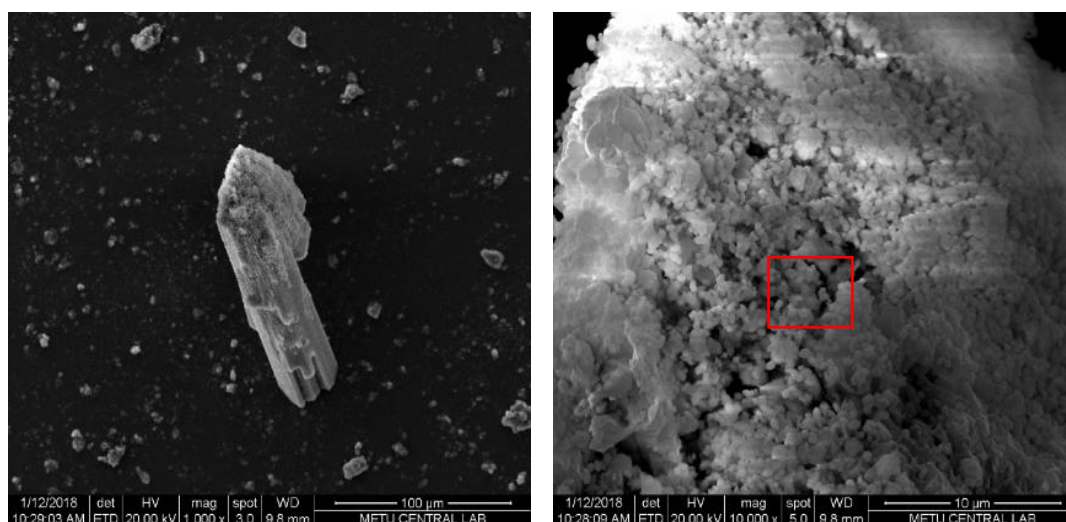
Figure 62. SEM images of carbonation products on the 17th day: nesquehonite, and calcite aggregates 1000x(left), and closer view showing aggregates of calcite or dolomite nanoparticles 10000 (right).
