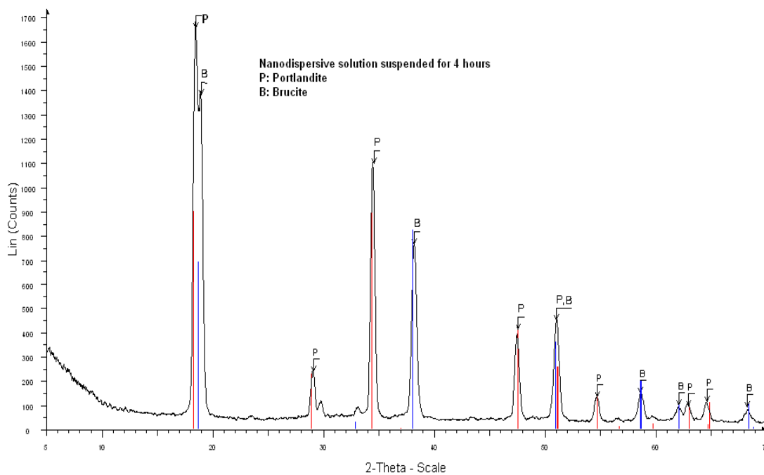
Figure 38. XRD traces of \text{Ca}(\text{OH})_2 and \text{Mg}(\text{OH})_2 nanoparticles dispersed in ethanol, after 4 hours of settlement: P:Portlandite \text{Ca}(\text{OH})_2 and B:Brucite \text{Mg}(\text{OH})_2
