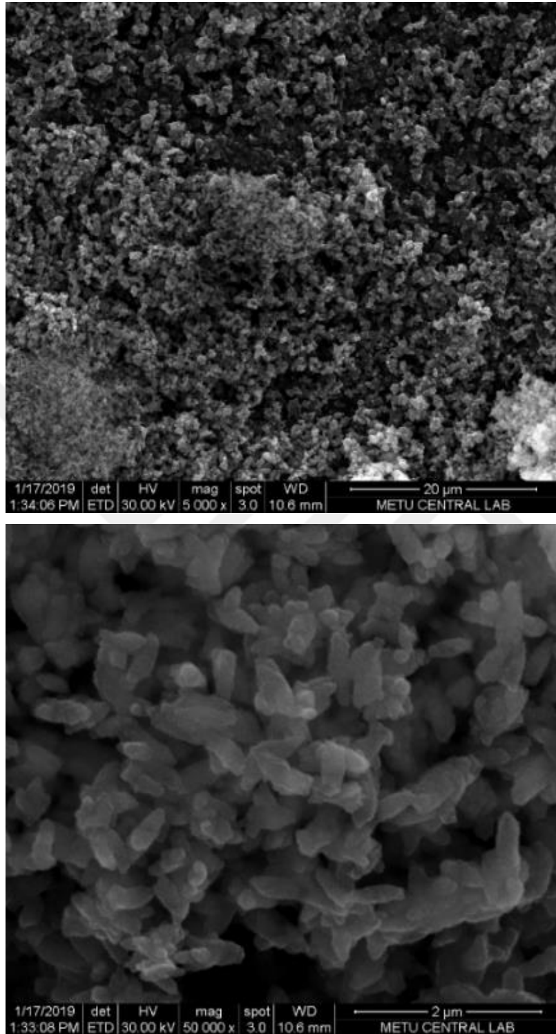
Figure 95. Another view of the upper layer at the tenth day: SEM images of carbonation products showing dolomite aggregates (up:5000x, down: 50000x magnification).
