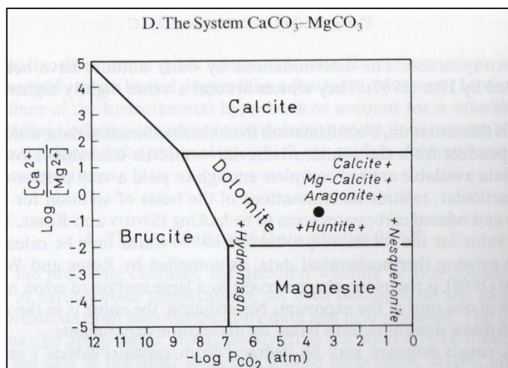
Figure 4. Phase diagram of the system CaCO 3 -MgCO 3 -H 2 O for zero ionic strength at 25°C. The metastable phases occurring in the system are indicated in italics. The black dot corresponds to the conditions of seawater. (Lippman, 1973, p:158)
