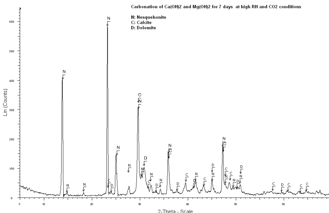
Figure 48. XRD traces of carbonation products of \text{Ca(OH)}_2 and \text{Mg(OH)}_2 nanoparticles dispersed in ethanol, at high RH and high \text{CO}_2 pressure for 7 days. N: Nesquehonite, C: Calcite, D: Dolomite.
