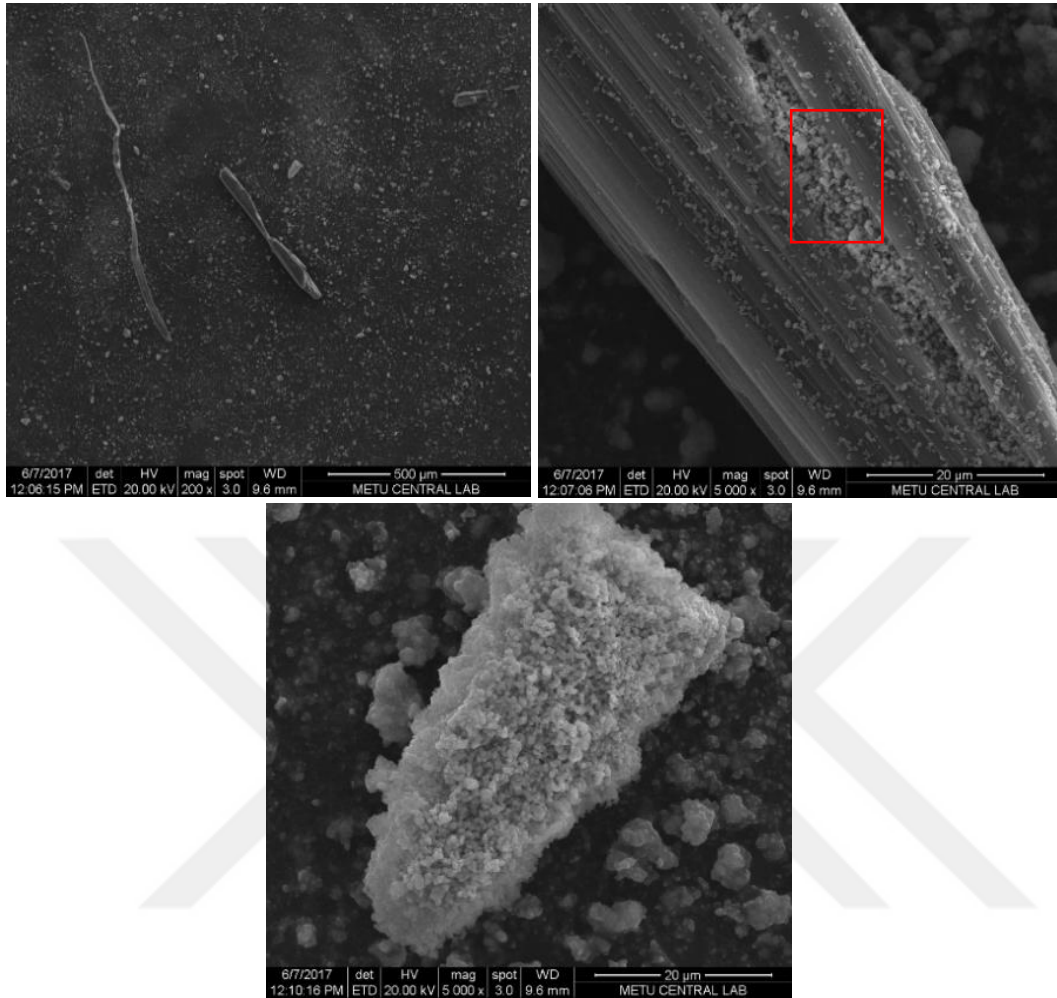
Figure 66. SEM images of carbonation products at 28th day 200x (up, left), 5000x of elongated aggregate (up, right) showing newly formed crystals on nesquehonite, 5000x of smaller aggregates belonging to calcite or dolomite (down).
