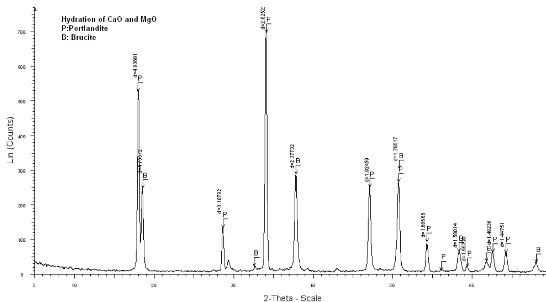
Figure 31. XRD traces of slaking products of CaO and MgO. B: Brucite ( \text{Mg}(\text{OH})_2 ), P: Portlandite ( \text{Ca}(\text{OH})_2 )
