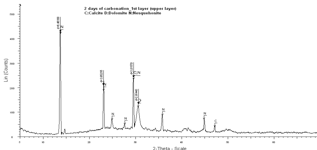
Figure 76. XRD traces of carbonation products in petri dish, upper layer, 2 days of carbonation
