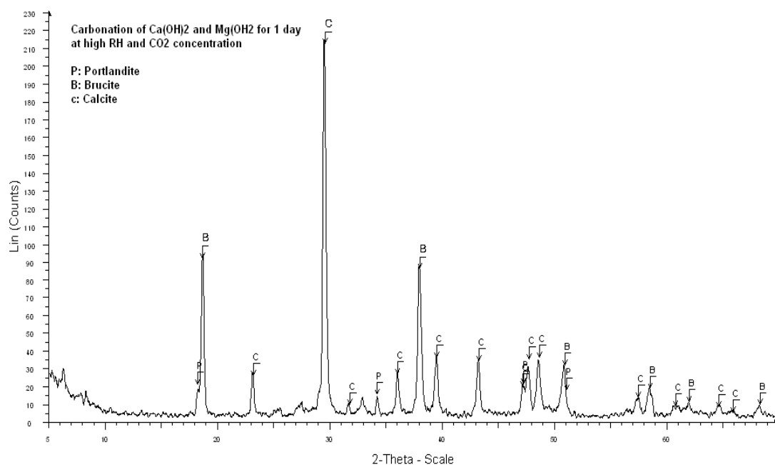
Figure 46. XRD traces of carbonation products of \text{Ca}(\text{OH})_2 and \text{Mg}(\text{OH})_2 nanoparticles dispersed in ethanol, at high RH and high \text{CO}_2 pressure for 1 day. P: Portlandite, B: Brucite, C: Calcite.
