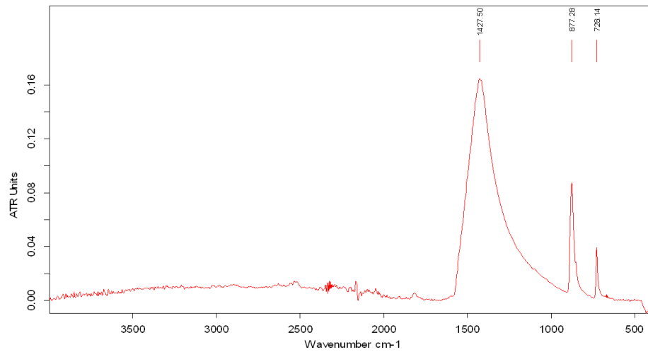
Figure 11. FTIR spectrum of Midyat dolostone
