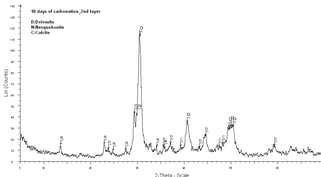
Figure 85. XRD traces of carbonation products in petri dish, bottom layer, 10 days of carbonation
