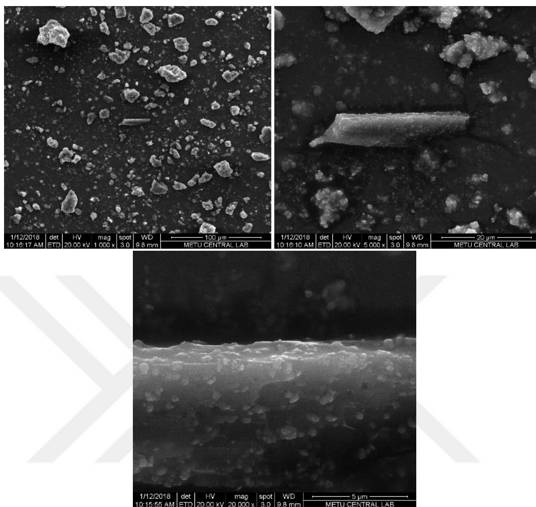
Figure 60. SEM image of carbonation products at the 7th day: Nesquehonite aggregates with calcite aggregates associated with it: 1000x (up, left), 5000x (up, right), 20000x (down)
