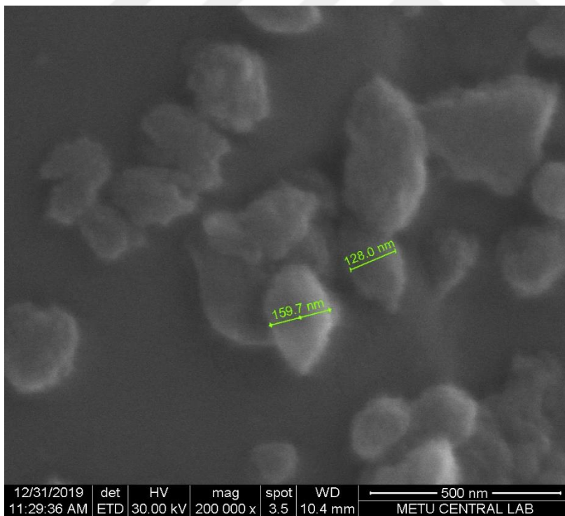
Figure 111. SEM view of the cross-section surface from the area close to the treatment surface (100000x-up, 200000x-down showing newly formed dolomite particles around 100-200nm)
