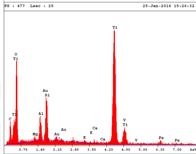
Figure 16. SEM-EDAX image of acid-insoluble part of the dolostone sample at 5000x magnification: showing the presence of oxides of titanium and silicon
