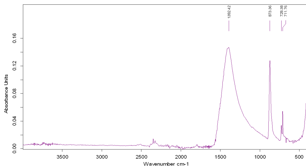
Figure 71. FTIR of Calcite and Dolomite mixture with a ratio of 0.5:0.5.
