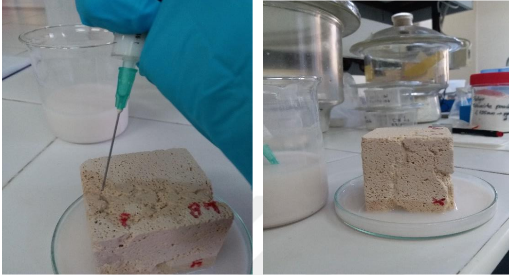
Figure 19. Application methods of alcohol dispersion of \text{Ca}(\text{OH})_2 and \text{Mg}(\text{OH})_2 nanoparticles for consolidation/treatment of deteriorated dolostone sample
