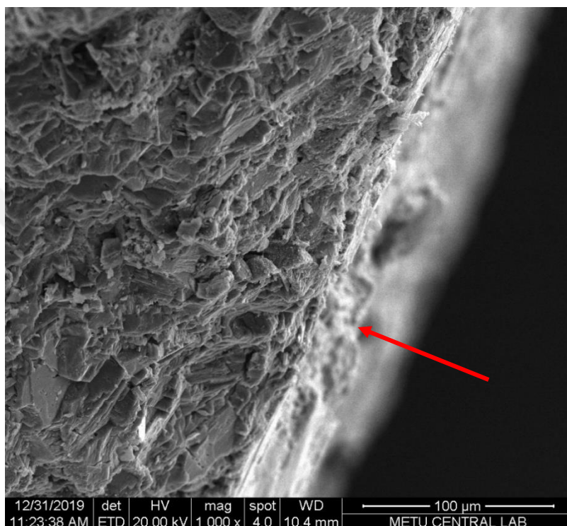
Figure 107. A general view from the cross-section surface of the treated dolostone sample. The red arrow at the right of the image corresponds to the side from where alcohol dispersion was applied: 1000x
