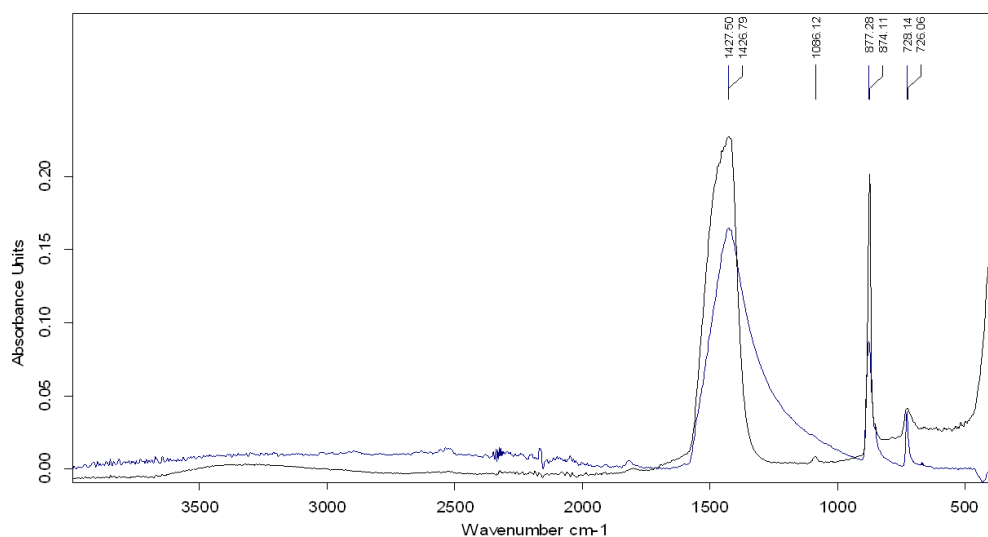
Figure 88. FTIR spectrum of dolomite formed at the upper layer (black) and FTIR spectrum of Midyat dolomite (blue)
