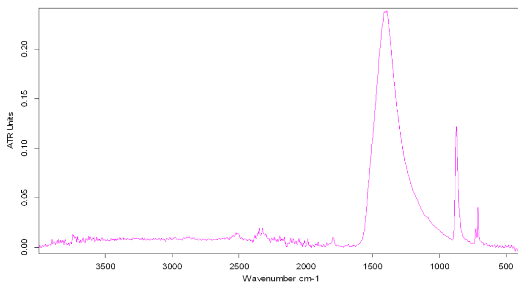
Figure 72. FTIR of Calcite and Dolomite mixture with a ratio of 0.6:0.4
