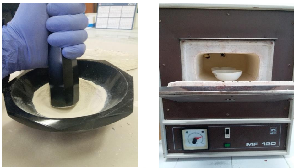
Figure 18. Pulverization and thermal decomposition stages of dolostone.
