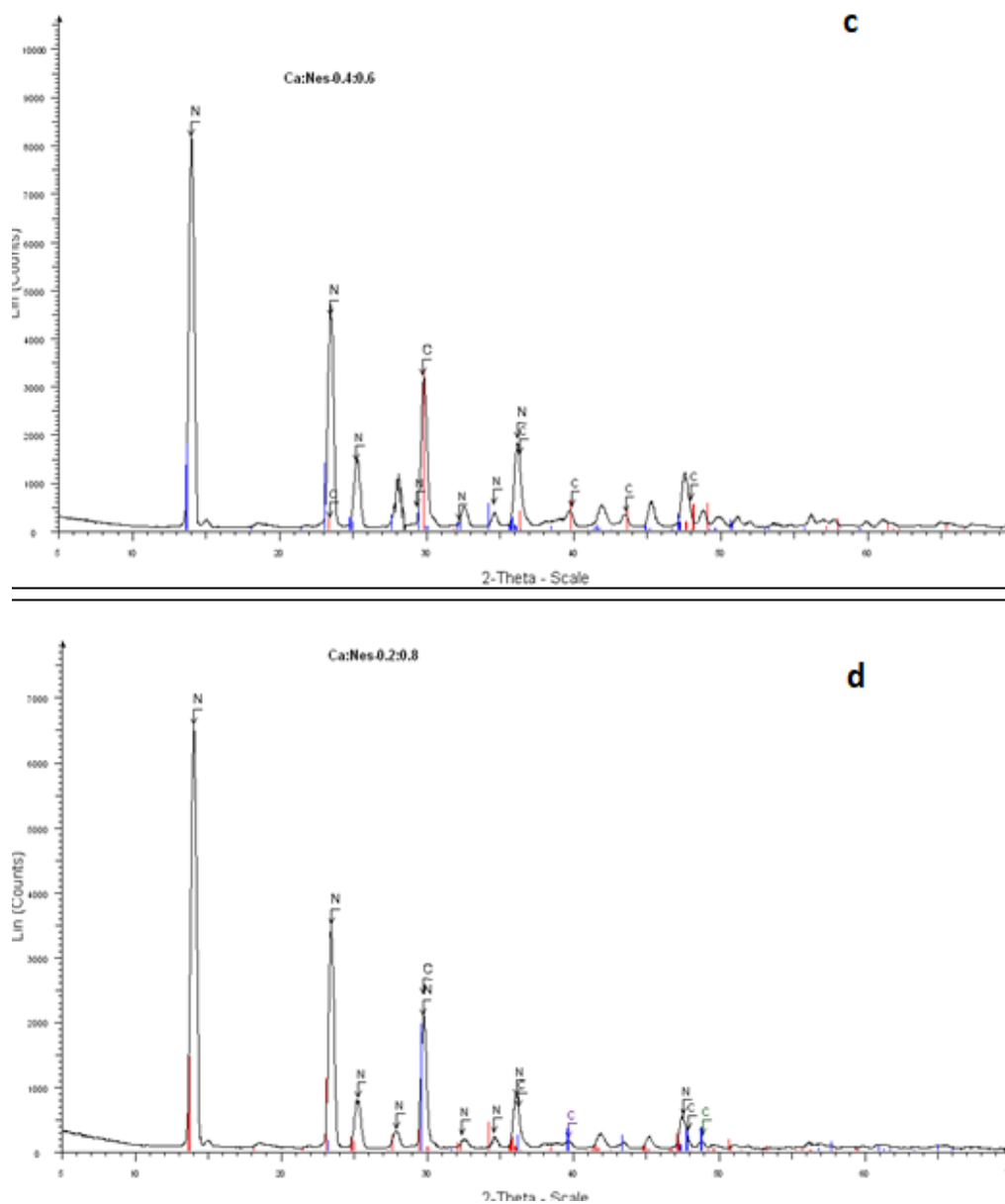
Figure 68 (continued). XRD traces of Calcite and Nesquehonite mixtures with the ratios c) Ca:Nes-0.4:0.6, d) Ca:Nes-0.2:0.8
