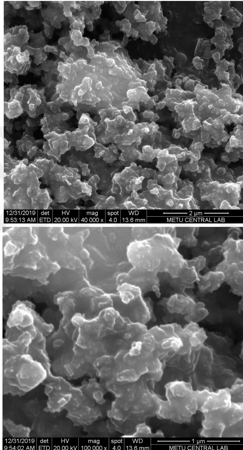
Figure 90. SEM image of carbonation products of upper layer at the first day. Hydroxide particles seems as aggregates integrated within each other (40000x-up and 100000x-down)
