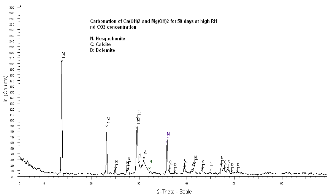
Figure 52. XRD traces of carbonation products of Ca(OH) 2 and Mg(OH) 2 nanoparticles dispersed in ethanol, at high RH and high CO 2 pressure for 58 days. N: Nesquehonite, C: Calcite, D: Dolomite.
