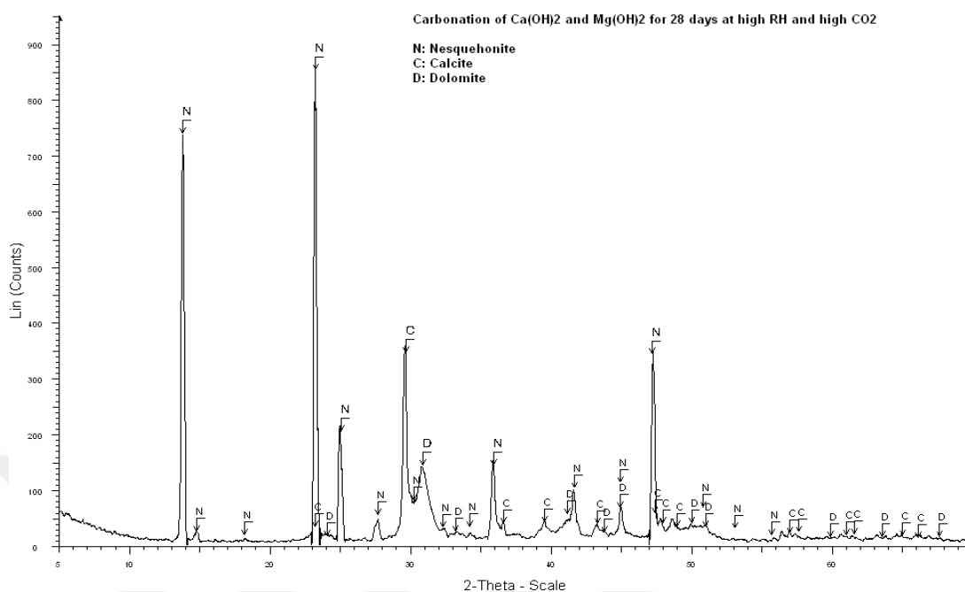
Figure 51. XRD traces of carbonation products of Ca(OH) 2 and Mg(OH) 2 nanoparticles dispersed in ethanol, at high RH and high CO 2 pressure for 28 days. N: Nesquehonite, C: Calcite, D: Dolomite.
