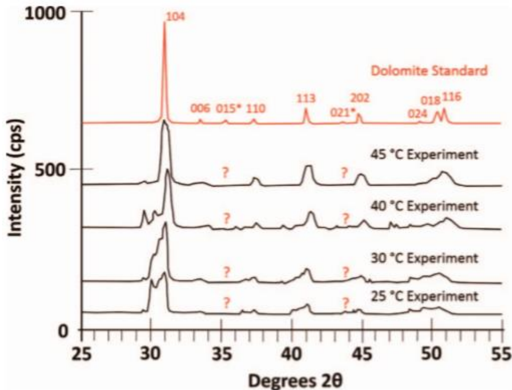
Figure 7. Comparison of XRD reflections of standard dolomite with a series of products made in low-temperature (25–45 °C) microbial experiments (modified by the author after Vasconcelos et al. , 1995).
