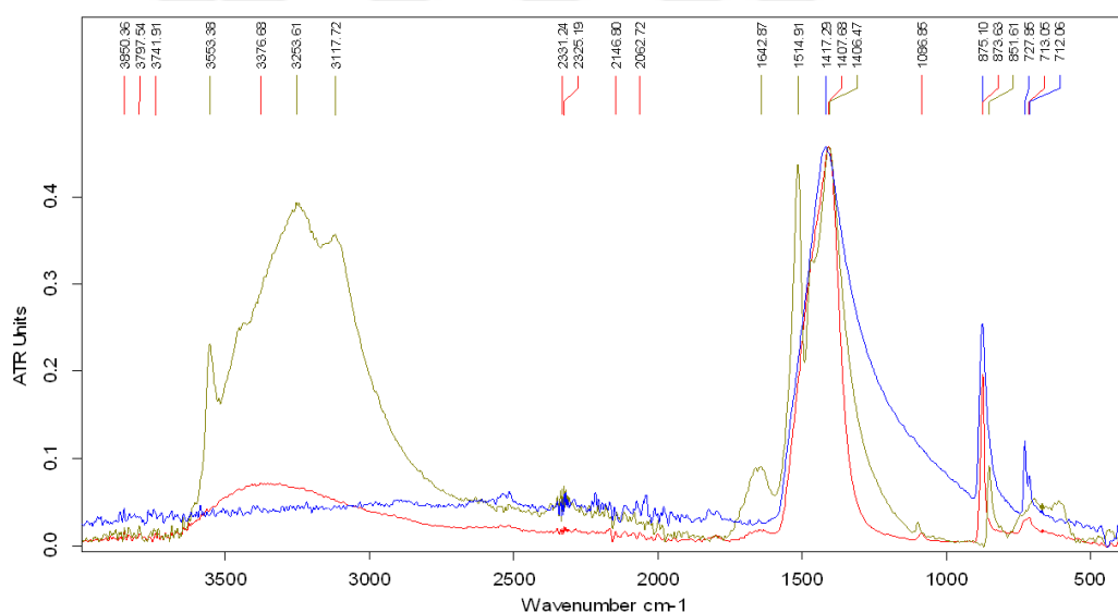
Figure 58. FTIR spectra of control mixture of dolomite and calcite (blue), nesquehonite (green) and carbonation products (red)
