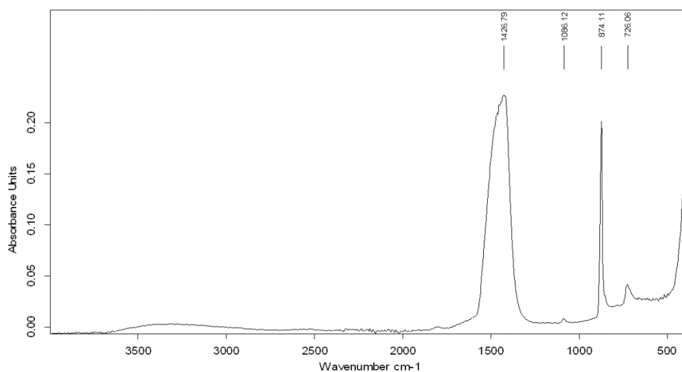
Figure 87. FTIR spectra of dolomite formed at the upper layer at the tenth day.
