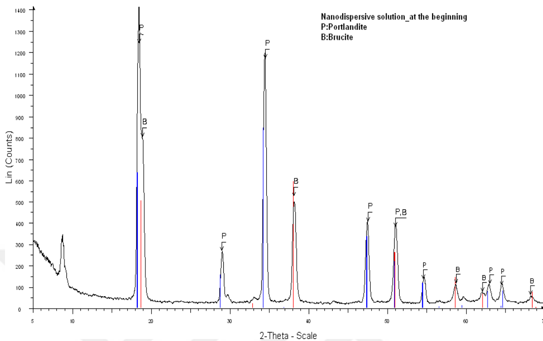
Figure 37. XRD traces of \text{Ca}(\text{OH})_2 and \text{Mg}(\text{OH})_2 nanoparticles dispersed in ethanol, in the beginning-no settlement: P: Portlandite \text{Ca}(\text{OH})_2 and B: Brucite \text{Mg}(\text{OH})_2
