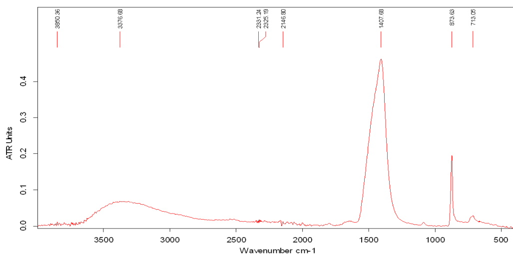
Figure 57. FTIR spectrum of carbonation products of \text{Ca(OH)}_2 and \text{Mg(OH)}_2 nanoparticles after 28 days.
