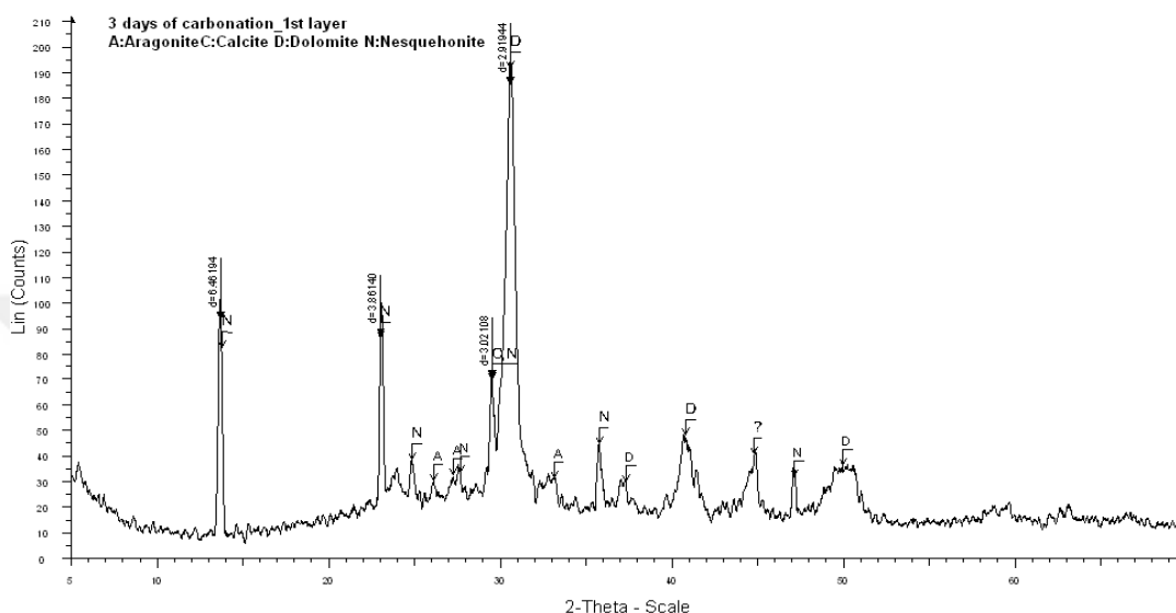
Figure 78. XRD traces of carbonation products in petri dish, upper layer, 3 days of carbonation
