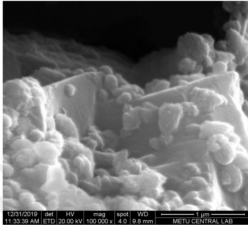
Figure 110. SEM view of the cross-section surface of treated dolostone sample showing the newly formed dolomite crystals on original dolomite crystals' edges and integration of them at 100000x magnification.
