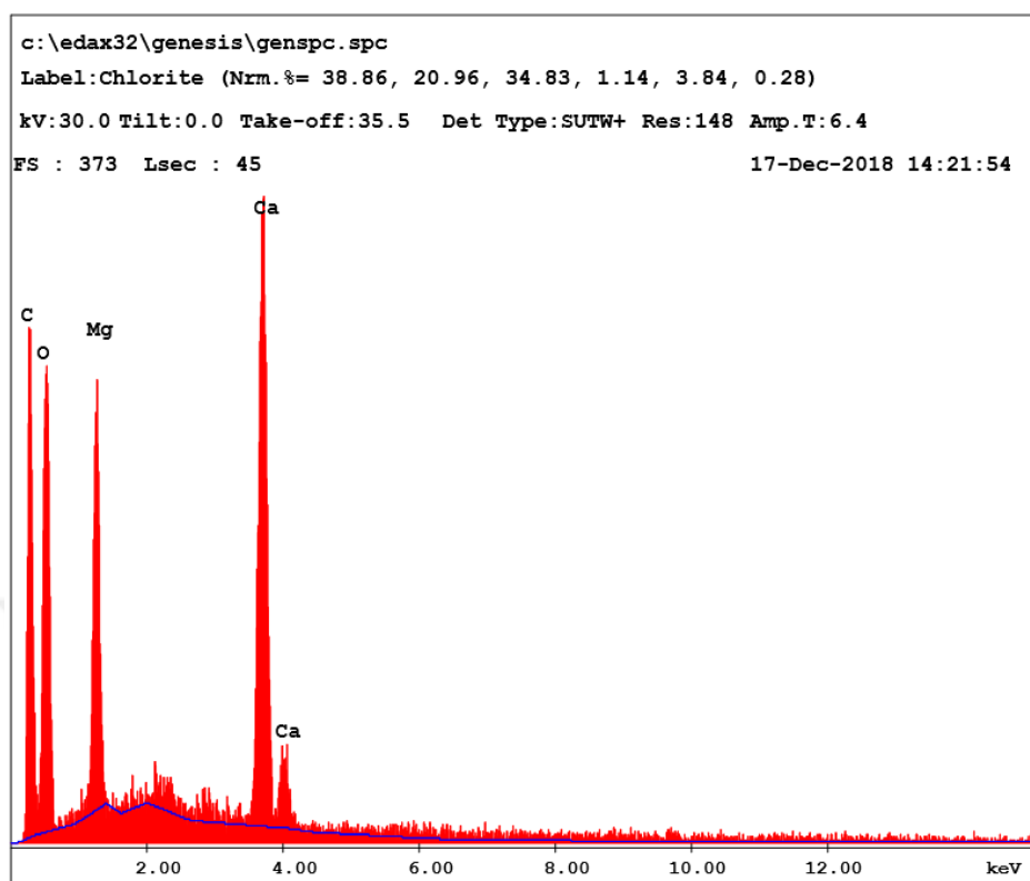
Figure 97. EDAX analysis of nanoparticle aggregates at the upper layer (at 200000x) (yellow squared part).
