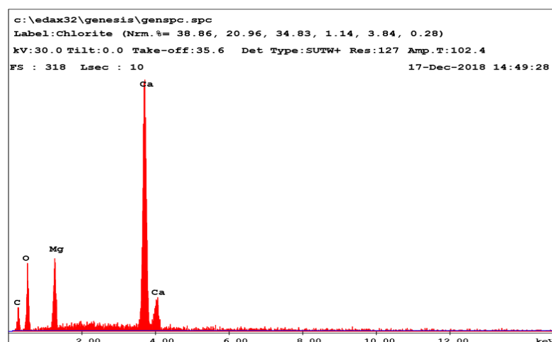
Figure 99. EDAX analysis of aggregates at the bottom layer (at 100000x).
