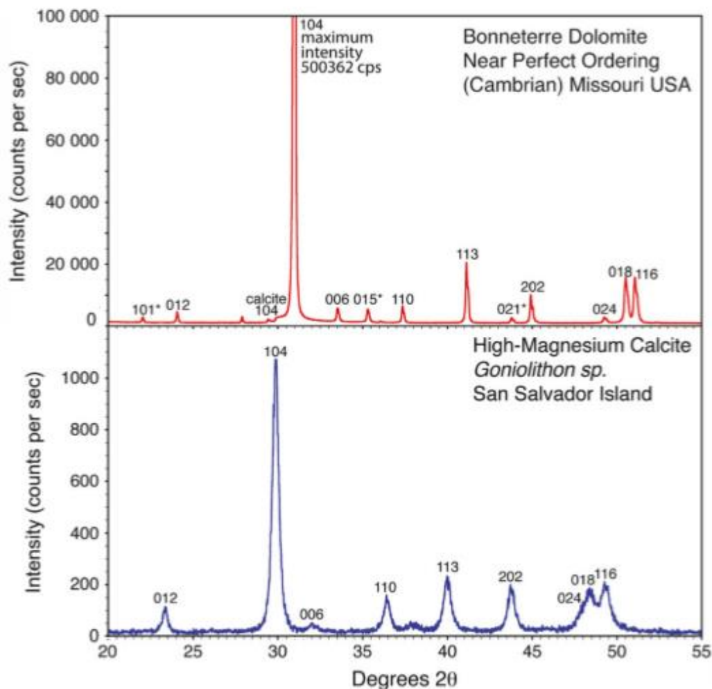
Figure 6. “X-ray diffraction patterns of dolomite and very high magnesium calcite. Dolomite from the ‘back reef’ facies of the Bonneterre Dolomite (Cambrian) Missouri (up). HMC from a coralline algae ( Goniolithon sp.) San Salvador Island, Bahamas(down). Calcite reflections are labeled. Note the pronounced shift of the 104 reflection towards a lower d-value. This shift is caused by a contraction of the calcite unit cell resulting from Mg^{2+} substitution for Ca^{2+} . Broadening of the reflections relative to those in calcite may be due to the exceptionally small crystallite size that is typical of HMC precipitated by coralline algae” Modified from Greg,2015, p:1756.
