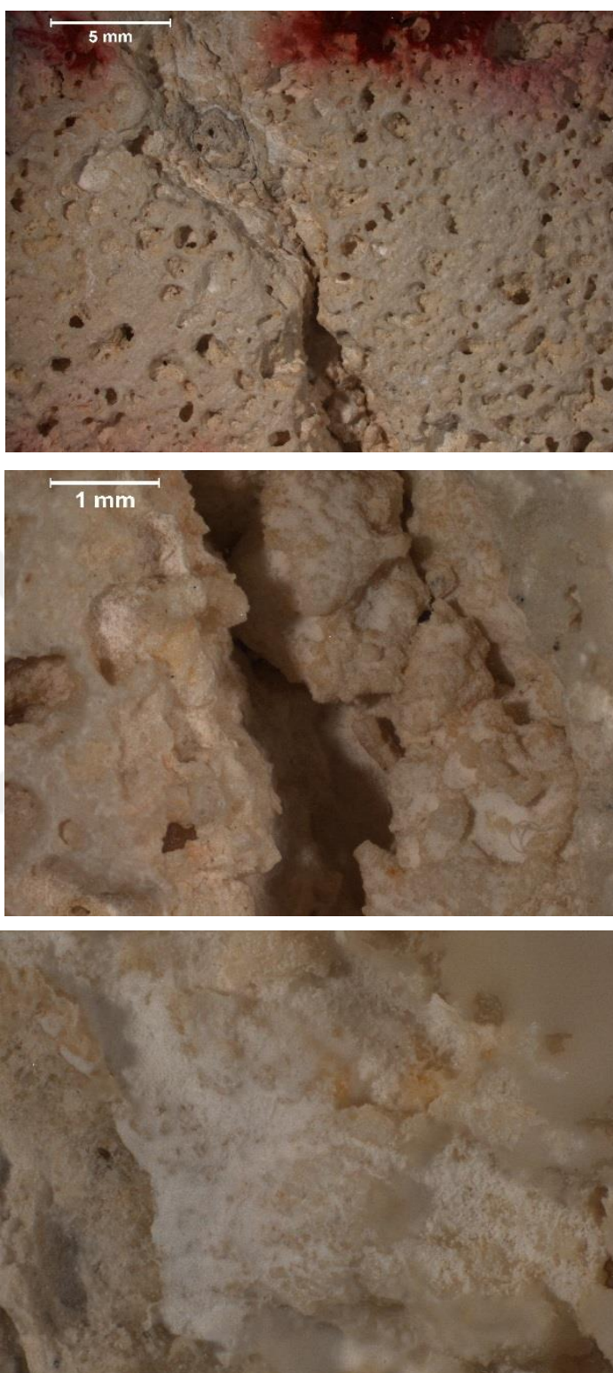
Figure 102. Stereomicroscope images of cracks of dolostone sample after treatment: 10x (up), 40x (middle), 145x (bottom).
