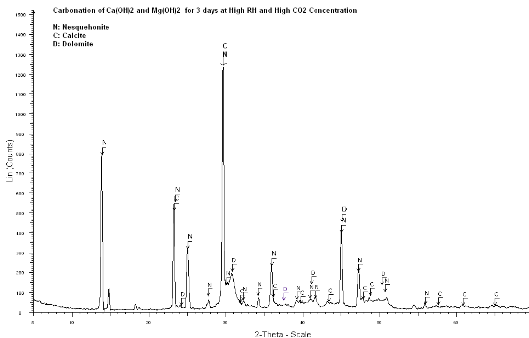
Figure 47. XRD traces of carbonation products of \text{Ca}(\text{OH})_2 and \text{Mg}(\text{OH})_2 nanoparticles dispersed in ethanol, at high RH and high \text{CO}_2 pressure for 3 days. N: Nesquehonite, C: Calcite, D: Dolomite.
