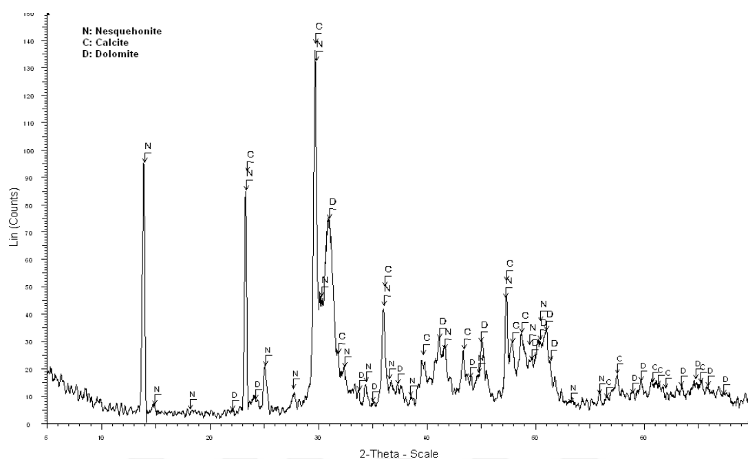
Figure 49. XRD traces of carbonation products of \text{Ca}(\text{OH})_2 and \text{Mg}(\text{OH})_2 nanoparticles dispersed in ethanol, at high RH and high \text{CO}_2 pressure for 17 days. N: Nesquehonite, C: Calcite, D: Dolomite.
