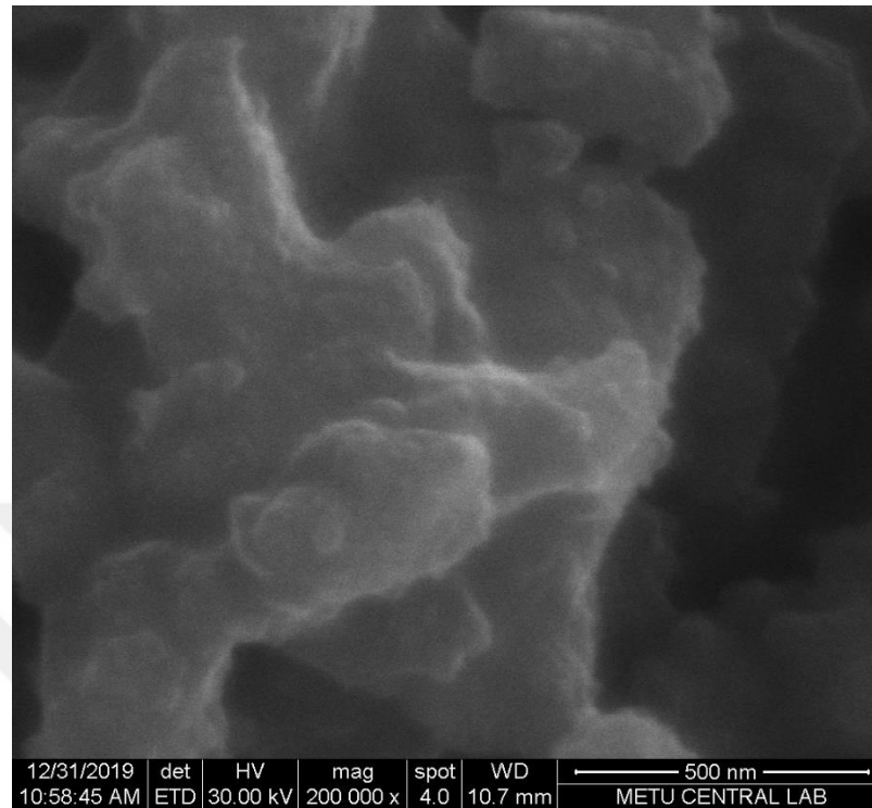
Figure 94. Closer view showing dolomite aggregates around 500 nm and smaller ones down to around 100 nm (200000x magnification)
