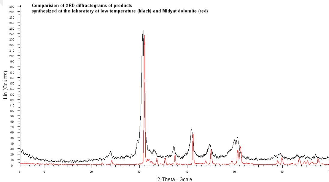
Figure 86. XRD traces of synthesized dolomite compared with the Midyat dolostone sample(red).
