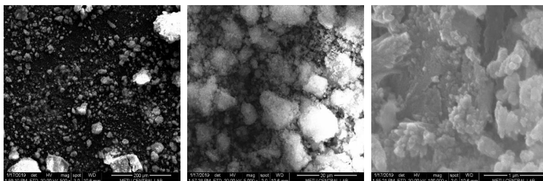
Figure 98. SEM images of carbonation products in petri dish at the bottom layer at the tenth day: 500x (left), 5000x (middle), 100000x (right).
