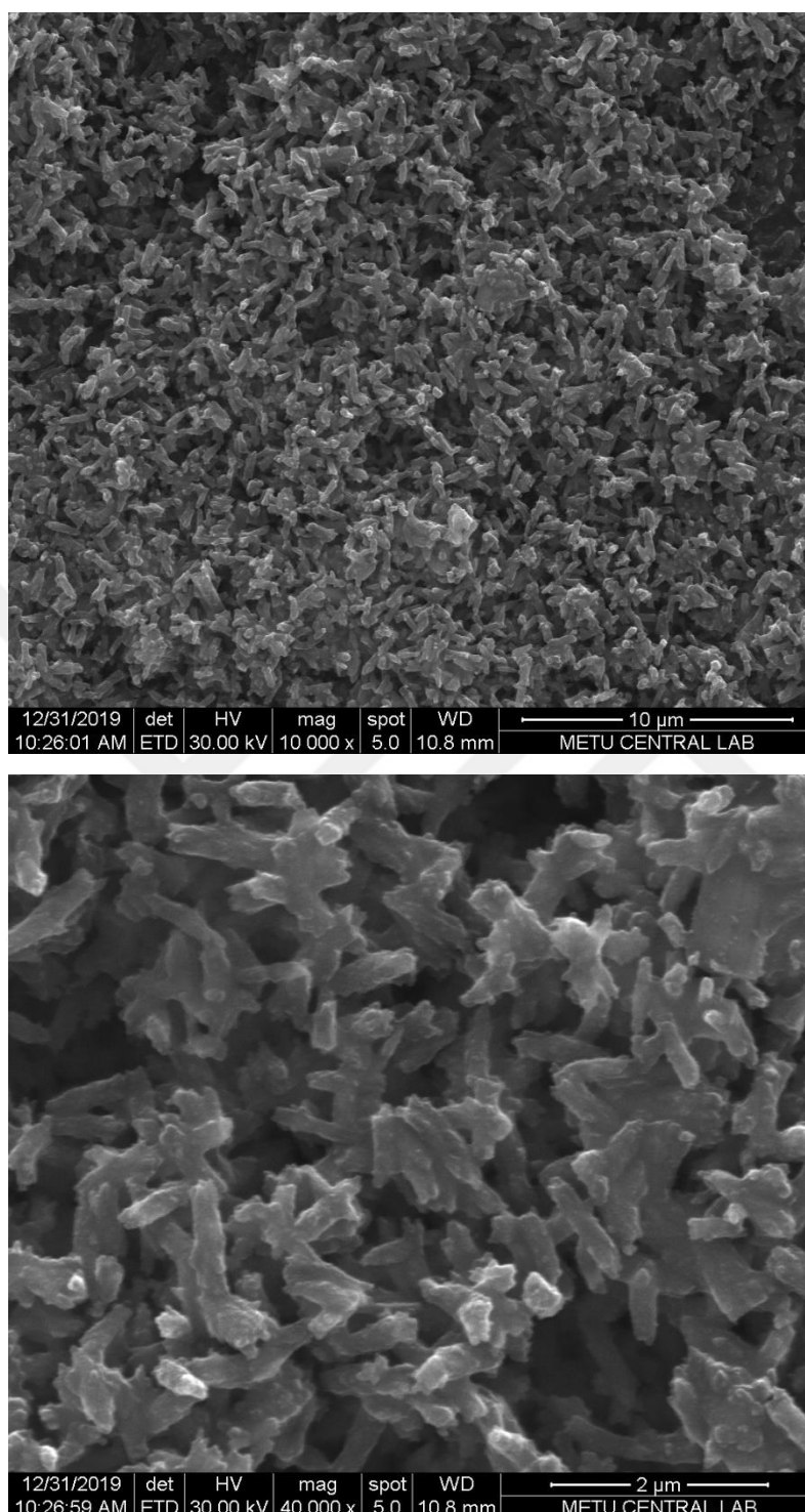
Figure 91. SEM image of carbonation products of upper layer at the second day. In that layer hydroxide nanoparticles seems to be carbonated as aggregates of calcite, dolomite (or maybe magnesium calcite) and nesquehonite (10000x-up and 40000x-down)
