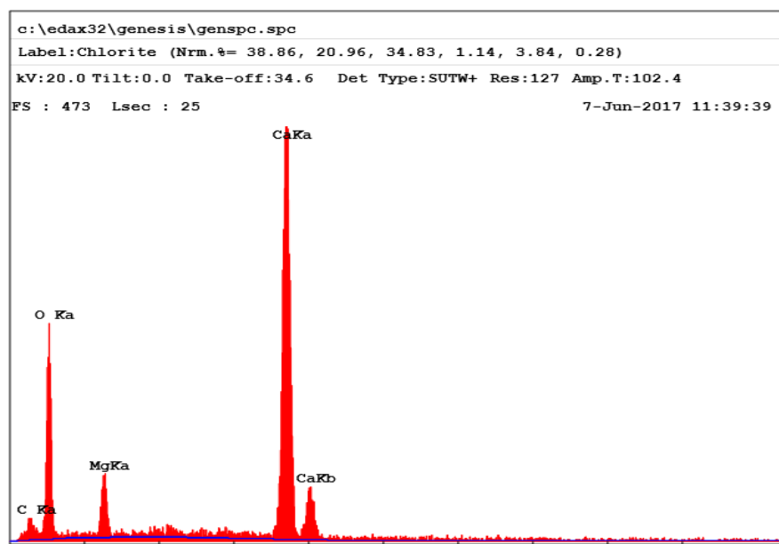
Figure 35. SEM-EDAX of large clusters belonging to \text{Ca}(\text{OH})_2 :EDAX analysis of yellow squared part.
