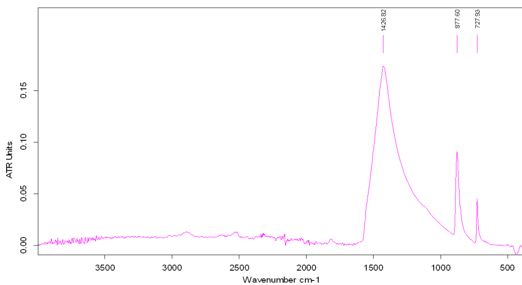
Figure 55. FTIR Spectrum of Midyat dolomite
