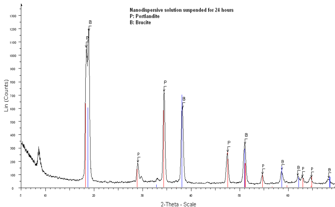
Figure 39. XRD traces of \text{Ca}(\text{OH})_2 and \text{Mg}(\text{OH})_2 nanoparticles dispersed in ethanol ,after 24 hours of settlement: P:Portlandite \text{Ca}(\text{OH})_2 and B:Brucite \text{Mg}(\text{OH})_2
