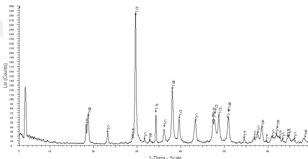
Figure 43. Carbonation of \text{Ca}(\text{OH})_2 and \text{Mg}(\text{OH})_2 nanoparticles dispersed in ethanol, at room condition for 4 weeks. B: Brucite; C: Calcite; P: Portlandite
