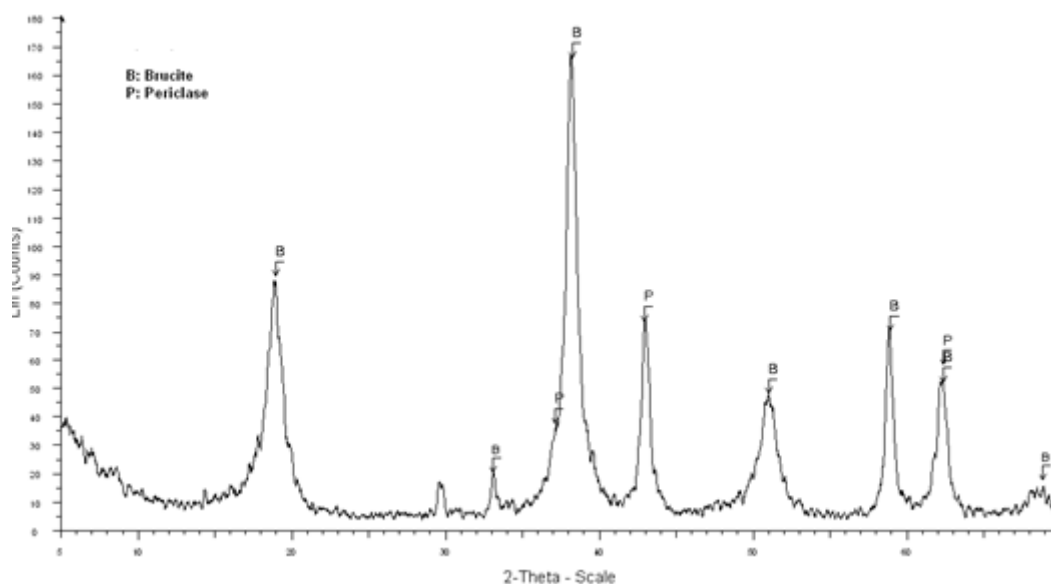
Figure 26. XRD trace of slaked product of \text{MgO} : B: Brucite ( \text{Mg}(\text{OH})_2 ), P: Periclase ( \text{MgO} )
