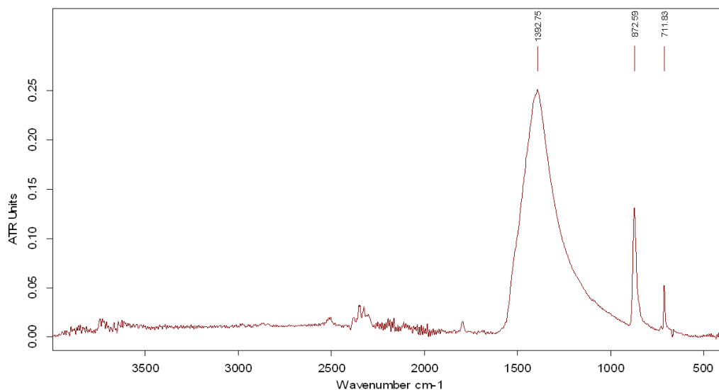
Figure 73. FTIR of Calcite and Dolomite mixture with a ratio of 0.8:0.2.
