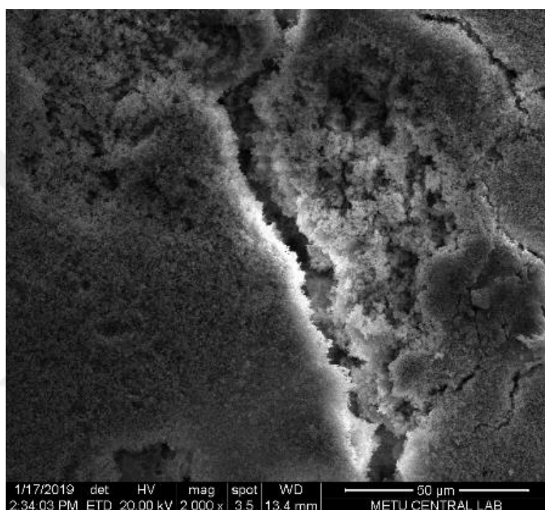
Figure 105. SEM image of dolostone surface after consolidation treatment: 2000x (dolomite layer)
