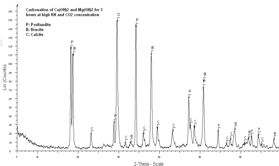
Figure 45. XRD traces of carbonation products of \text{Ca}(\text{OH})_2 and \text{Mg}(\text{OH})_2 nanoparticles dispersed in ethanol, at high RH and high \text{CO}_2 pressure for 3 hours. P: Portlandite, B: Brucite, C: Calcite.
