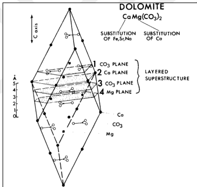
Figure 1. Representation of rhombohedral unit cell of dolomite (Morrow, 1982, p:5).
