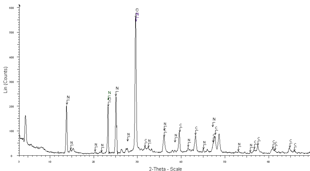
Figure 44. Carbonation of \text{Ca}(\text{OH})_2 and \text{Mg}(\text{OH})_2 nanoparticles dispersed in ethanol, at high RH and low \text{CO}_2 pressure for 4 weeks. C: Calcite, N: Nesquehonite
