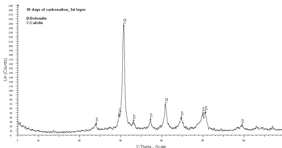
Figure 84. XRD traces of carbonation products in petri dish, upper layer, 10 days of carbonation
