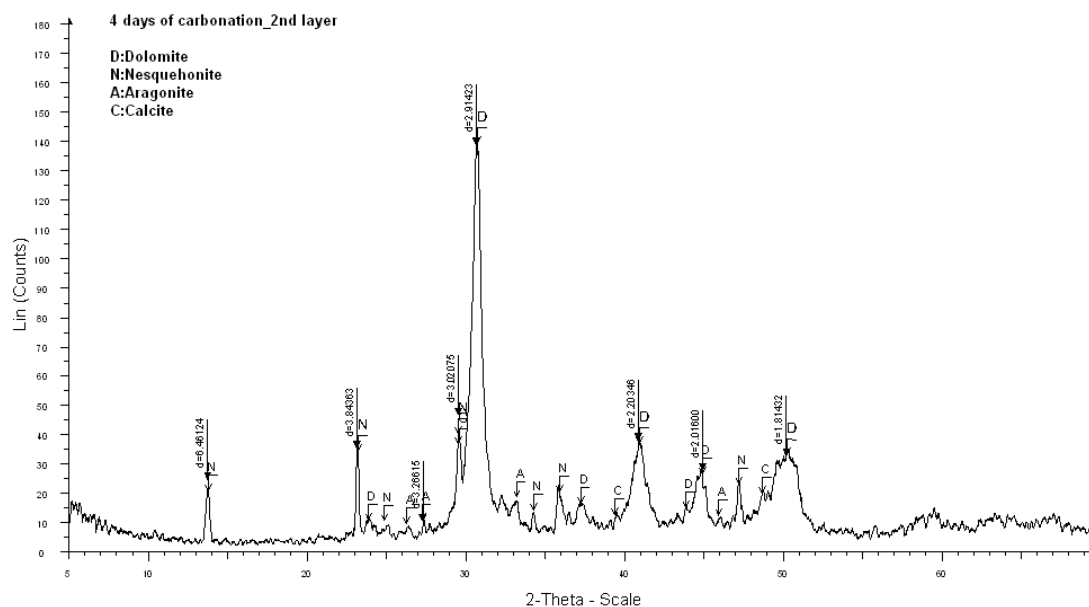
Figure 81. XRD traces of carbonation products in petri dish, bottom layer, 4 days of carbonation
