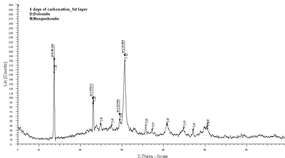
Figure 80. XRD traces of carbonation products in petri dish, upper layer, 4 days of carbonation
