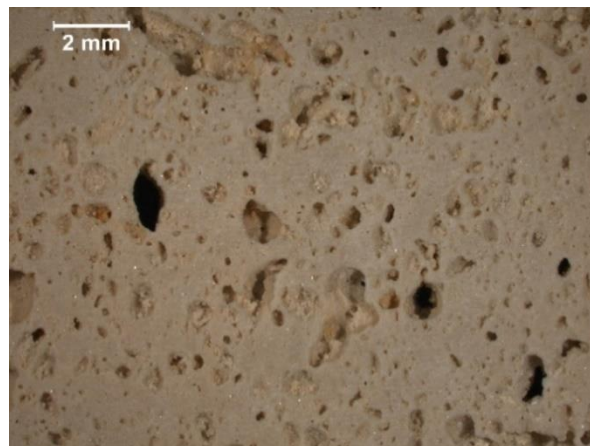
Figure 12. Stereomicroscopic view of macro-pores of Midyat dolostone in a cross-section at 20x magnification
