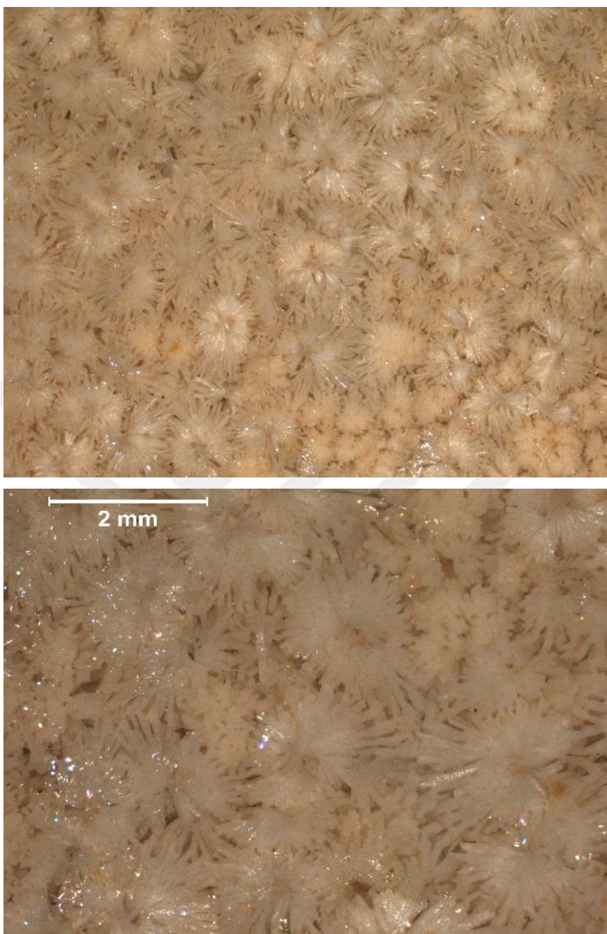
Figure 27. Stereomicroscope images of nesquehonite crystals formed after carbonation of \text{Mg}(\text{OH})_2 at high relative humidity and high \text{CO}_2 partial pressure: 10x (up) and 30x (down).
