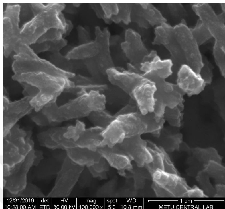
Figure 92. Closer view of aggregates having calcite, dolomite and nesquehonite aggregates integrated within each other (100000x magnification)
