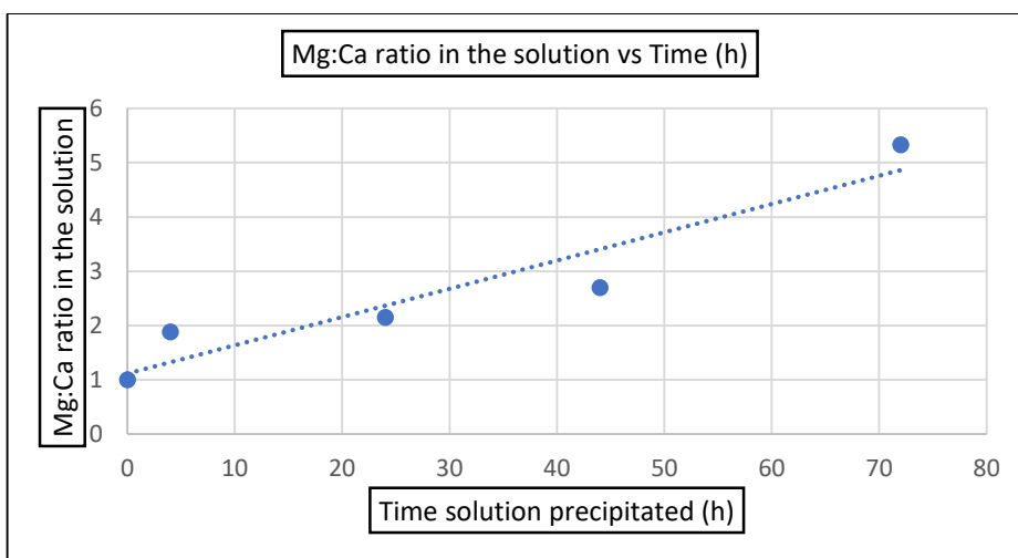
Figure 42. Mg:Ca ratio in the alcohol dispersion vs time of settlement
