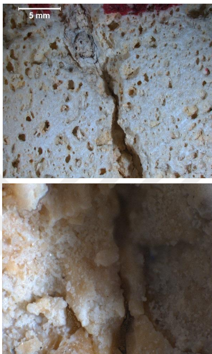
Figure 101. Stereomicroscope images of the main crack of dolostone sample before treatment: 10x (up) and 145x (down).
