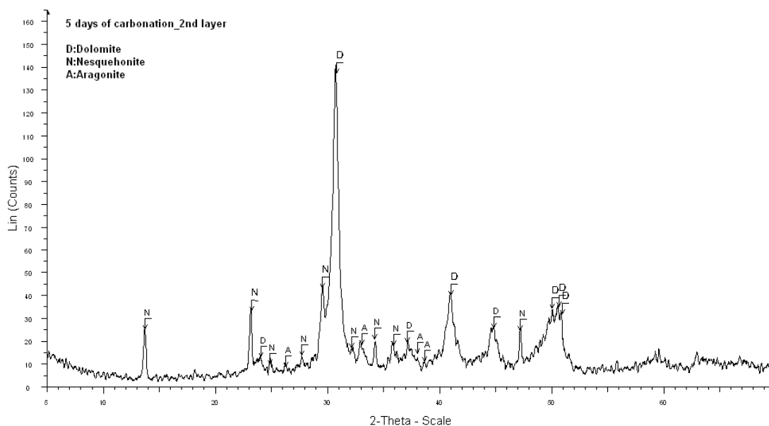
Figure 83. XRD traces of carbonation products in petri dish, bottom layer, 5 days of carbonation
