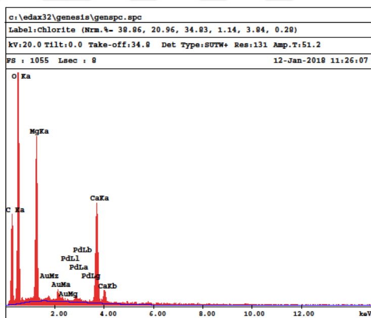
Figure 63. SEM EDAX results of the red squared region, nanoparticle aggregates on nesquehonite.
