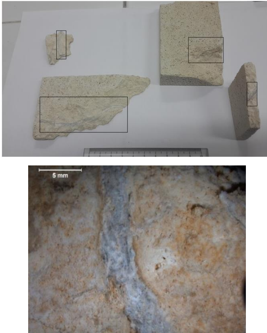
Figure 13. Photographic image of Midyat dolostone samples where veins appear (up) and Stereomicroscope image of the vein and orange colors around veins (down)
