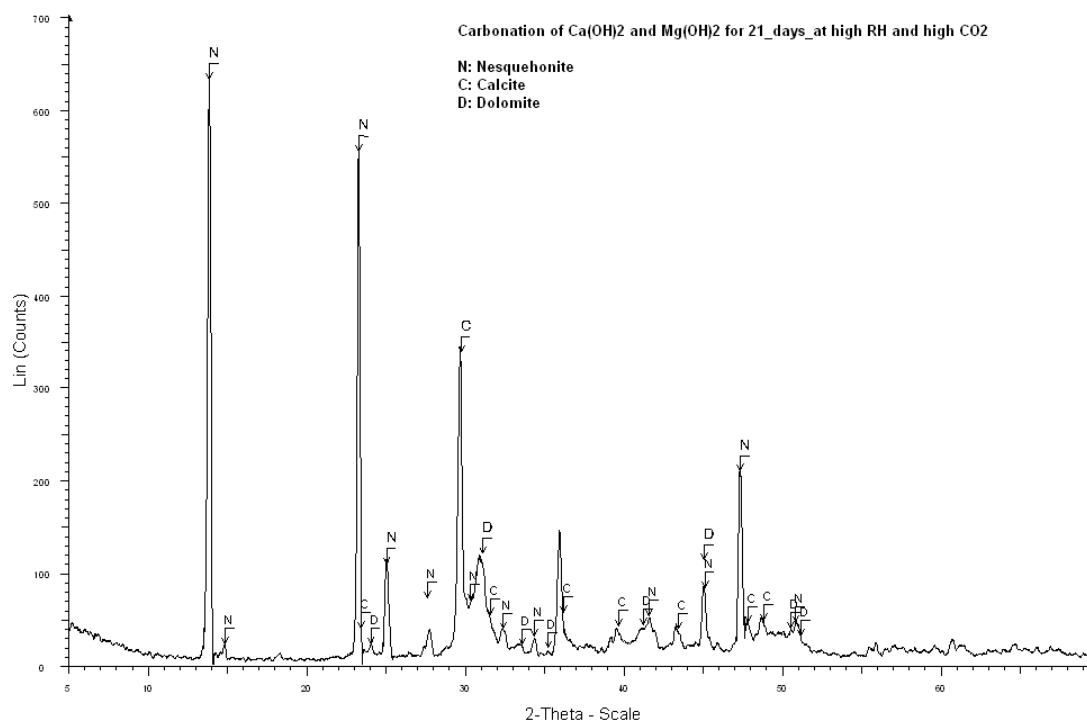
Figure 50. XRD traces of carbonation products of \text{Ca}(\text{OH})_2 and \text{Mg}(\text{OH})_2 nanoparticles dispersed in ethanol, at high RH and high \text{CO}_2 pressure for 21 days. N: Nesquehonite, C: Calcite, D: Dolomite.
