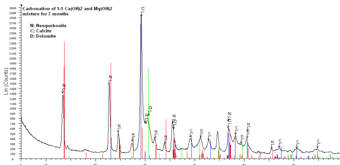
Figure 53. XRD traces of carbonation products of \text{Ca}(\text{OH})_2 and \text{Mg}(\text{OH})_2 nanoparticles dispersed in ethanol, at high RH and high \text{CO}_2 pressure for 7 months. N: Nesquehonite, C: Calcite, D: Dolomite.
