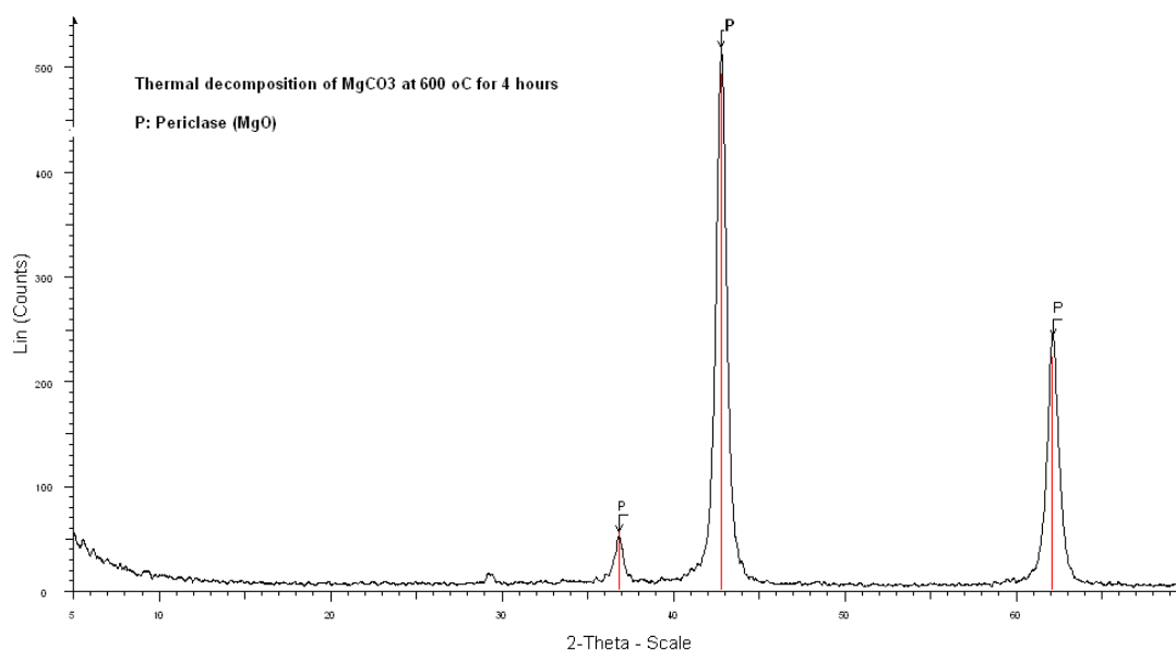
Figure 25. XRD analysis of calcination product of \text{MgCO}_3 : P: Periclase ( \text{MgO} )
