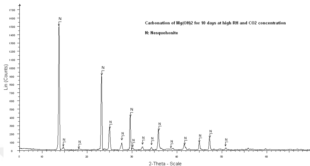
Figure 28. XRD analysis of carbonation product of \text{Mg}(\text{OH})_2 at the 10th day: N: Nesquehonite ( \text{MgCO}_3 \cdot 3\text{H}_2\text{O} )
