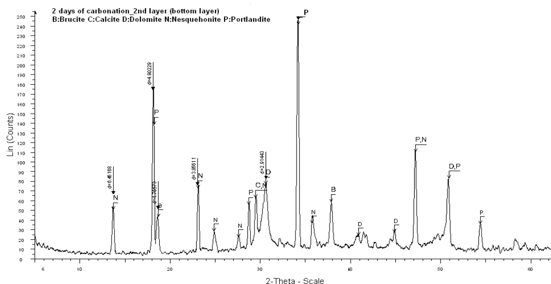
Figure 77. XRD traces of carbonation products in petri dish, bottom layer, 2 days of carbonation
