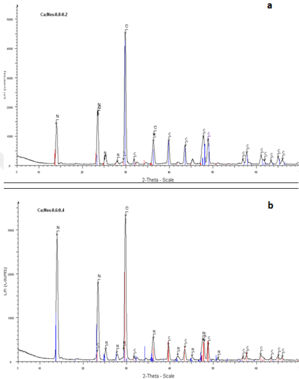
Figure 68. XRD traces of Calcite and Nesquehonite mixtures with the ratios a) Ca:Nes-0.8:0.2, b) Ca:Nes-0.6:0.4
