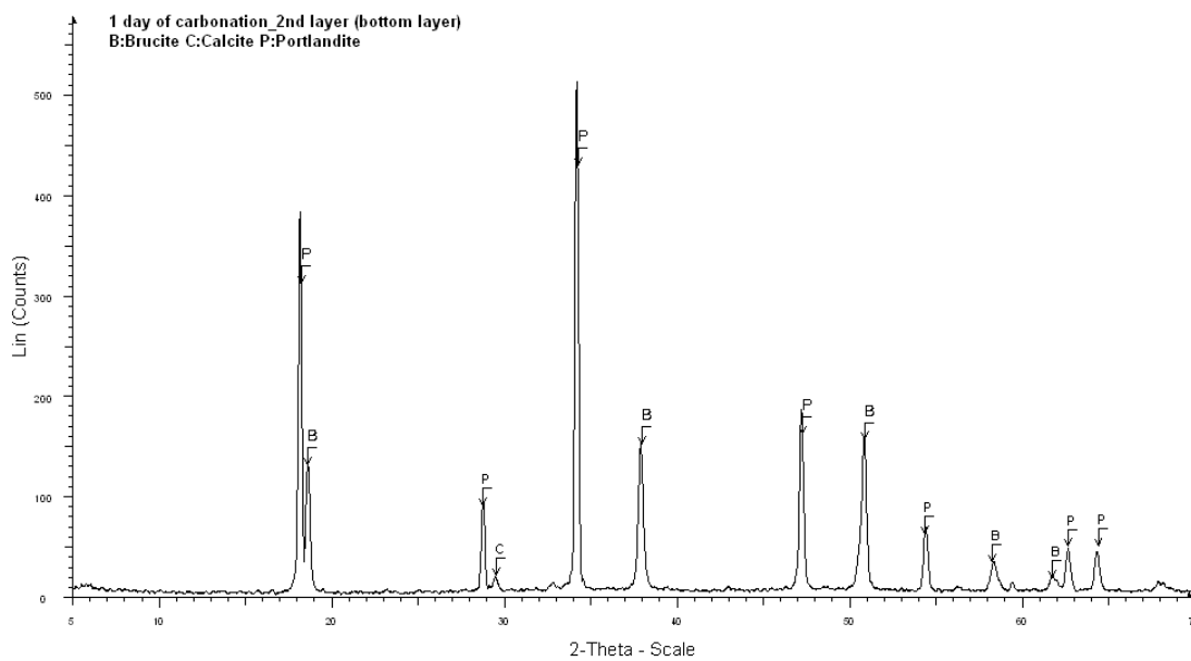
Figure 75. XRD traces of carbonation products in petri dish, bottom layer, 1 day of carbonation
