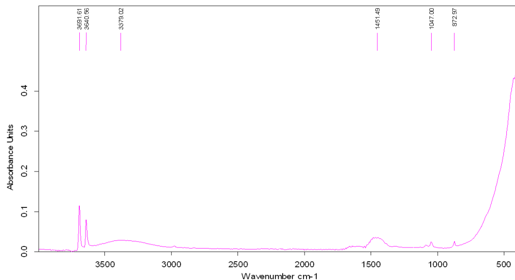
Figure 33. FTIR Spectrum of \text{Ca(OH)}_2 and \text{Mg(OH)}_2 hydroxide nanoparticles after dispersion in alcohol
