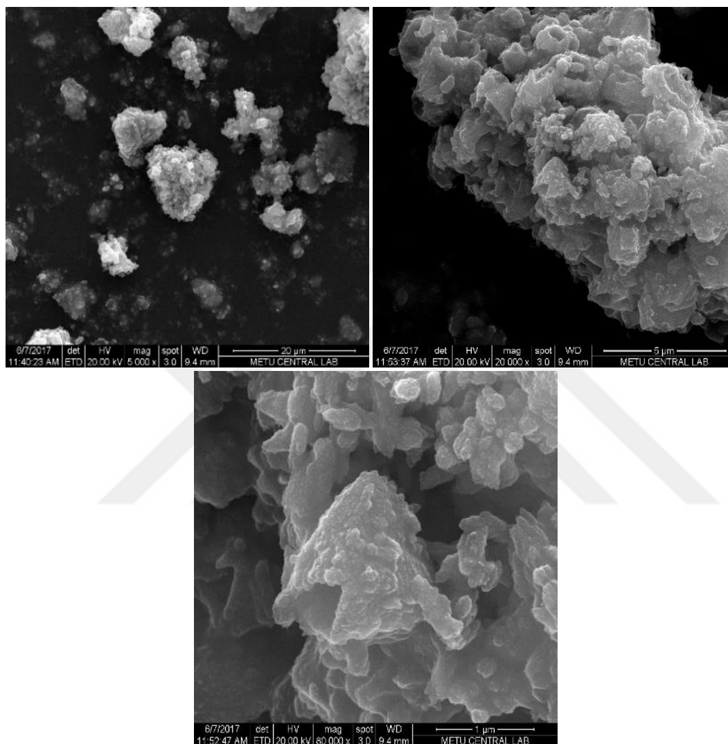
Figure 59. SEM images of carbonation products at the 7th day: calcite aggregates 5000x (up, left), 20000x (up, right), 80000x (down).
