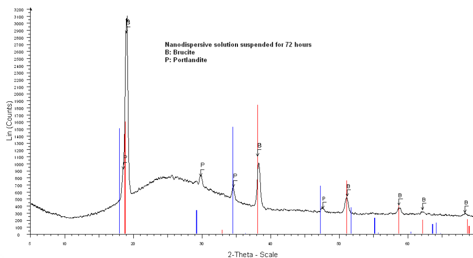
Figure 41. XRD traces of \text{Ca(OH)}_2 and \text{Mg(OH)}_2 nanoparticles dispersed in ethanol, after 72 hours of settlement: P:Portlandite \text{Ca(OH)}_2 and B:Brucite \text{Mg(OH)}_2
