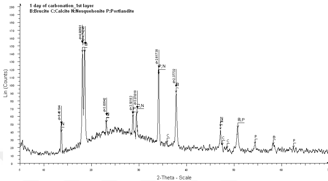
Figure 74. XRD traces of carbonation products in petri dish, upper layer, 1 day of carbonation
