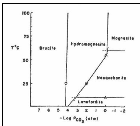
Figure 2. Probable stability relations in the system \text{MgO-CO}_2\text{-H}_2\text{O} between 0^{\circ}\text{C} and 100^{\circ}\text{C} as a function of p\text{CO}_2 and assuming a\text{H}_2\text{O} = 1 (Langmuir, 1965, p:248)
