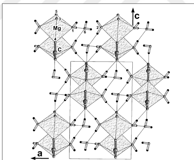
Figure 3. Crystal structure of nesquehonite in projections parallel to b. Drawings were obtained using the ATOMS program (Dowty, 1999)
