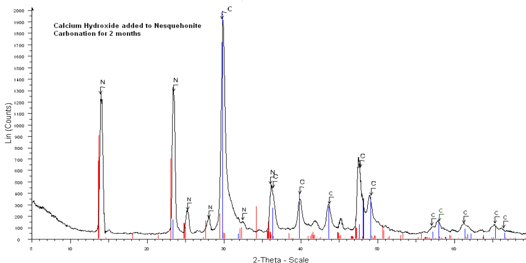
Figure 100. XRD traces of carbonation products of \text{Ca}(\text{OH})_2 nanoparticles added onto nesquehonite crystals for two months.
