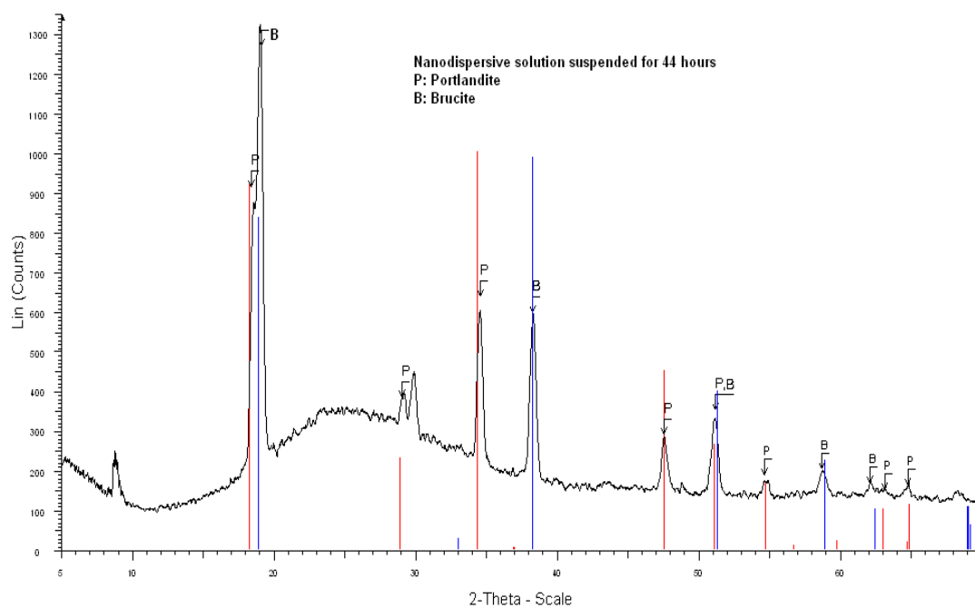
Figure 40. XRD traces of \text{Ca}(\text{OH})_2 and \text{Mg}(\text{OH})_2 nanoparticles dispersed in ethanol, after 44 hours of settlement: P:Portlandite \text{Ca}(\text{OH})_2 and B:Brucite \text{Mg}(\text{OH})_2
