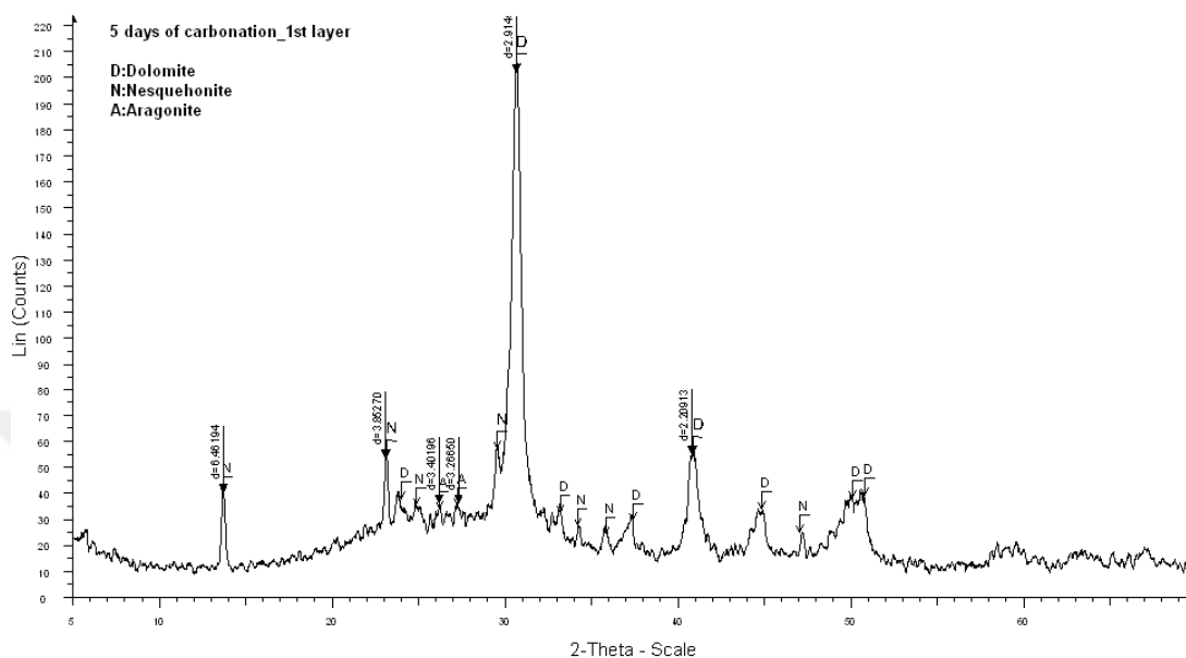
Figure 82. XRD traces of carbonation products in petri dish, upper layer, 5 days of carbonation
