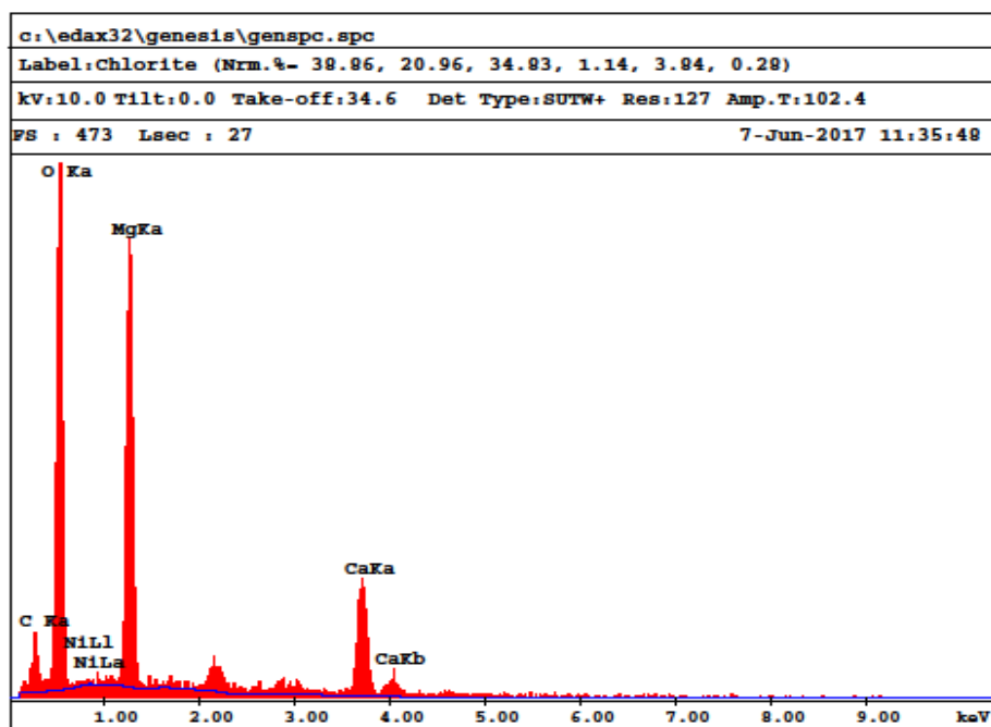
Figure 36. SEM-EDAX of smaller clusters belonging to \text{Mg}(\text{OH})_2 : EDAX analysis of red squared part.
