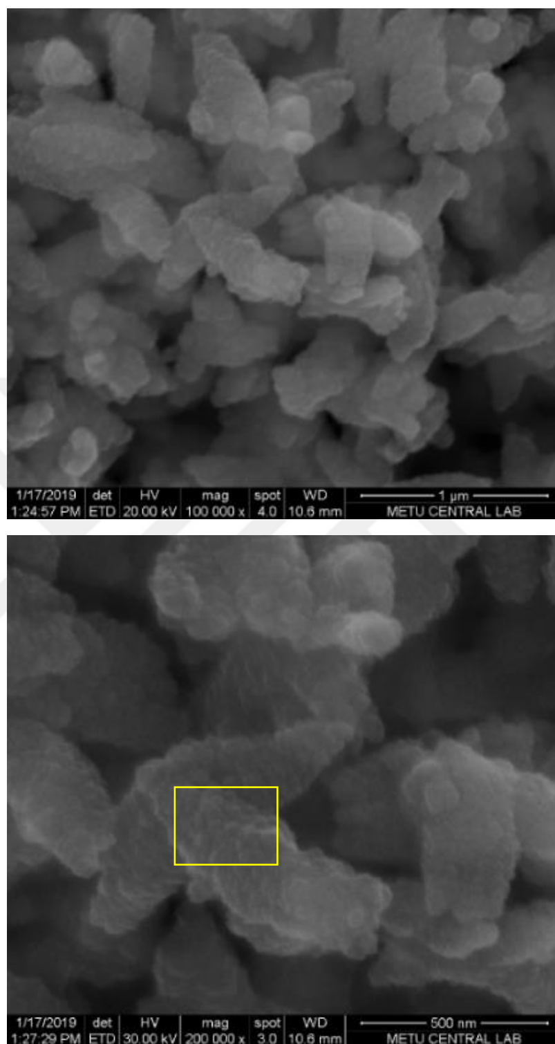
Figure 96. Closer SEM view showing dolomite aggregates around 500 nm and smaller ones having down to around 25-50 nm particles.
