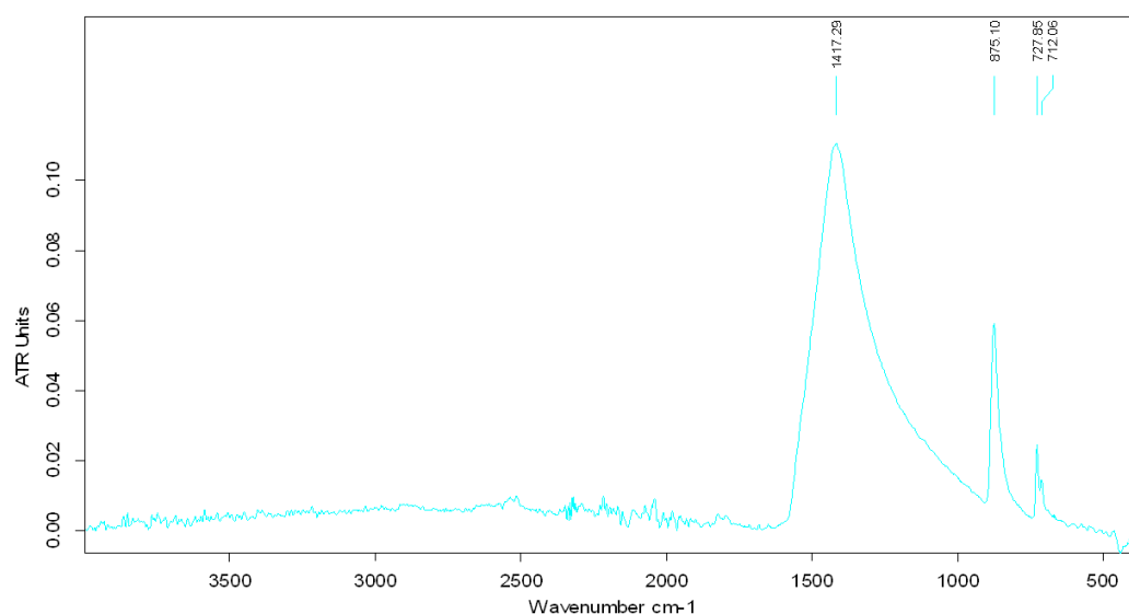
Figure 56. FTIR Spectrum of the mixture of standard calcite and dolomite.
