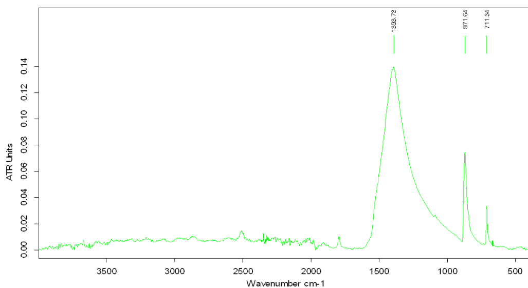
Figure 54. FTIR Spectrum of standard calcite.
