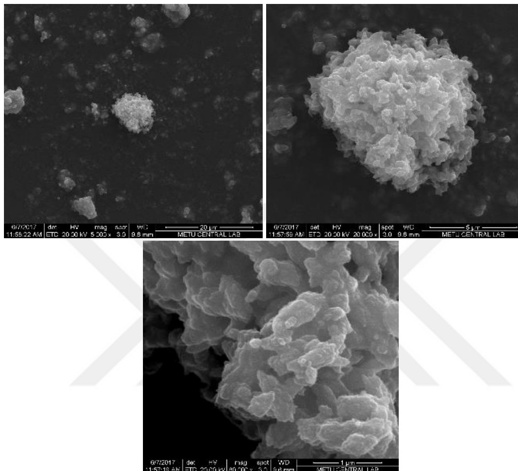
Figure 61. SEM images of carbonation products in the 17th day: calcite or dolomite aggregates 5000x (up, left), 20000x (up, right), 80000 (down).
