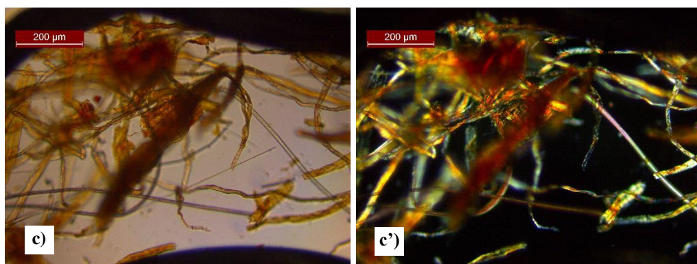
Figure 4.15. Macro to micro photographs of the sample E-44; a) sample's general view b) SM view, c&c') PLM view
