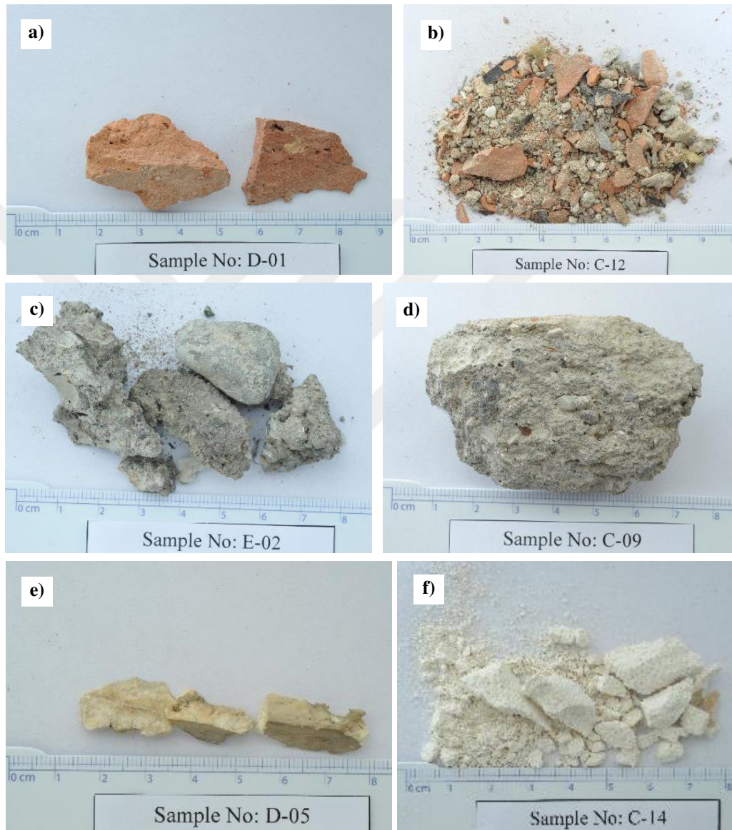
Figure 3.8. Representative macro-photographs of wall materials; a) brick, b) materials fragmented from the main bodies, c) exposed concrete, d) concrete, e) marble, f) plasterboard
