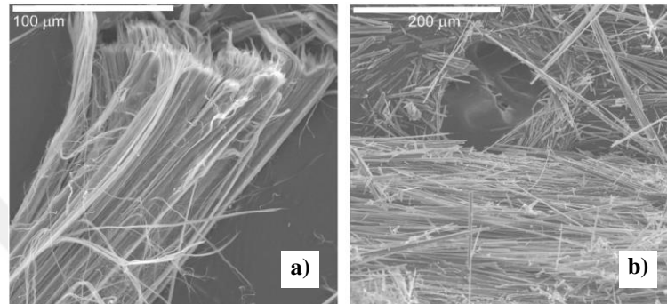
Figure 1.4. SEM views of asbestiform minerals; a) Chrysotile, b) Anthophyllite (Van Gosen, 2007)
