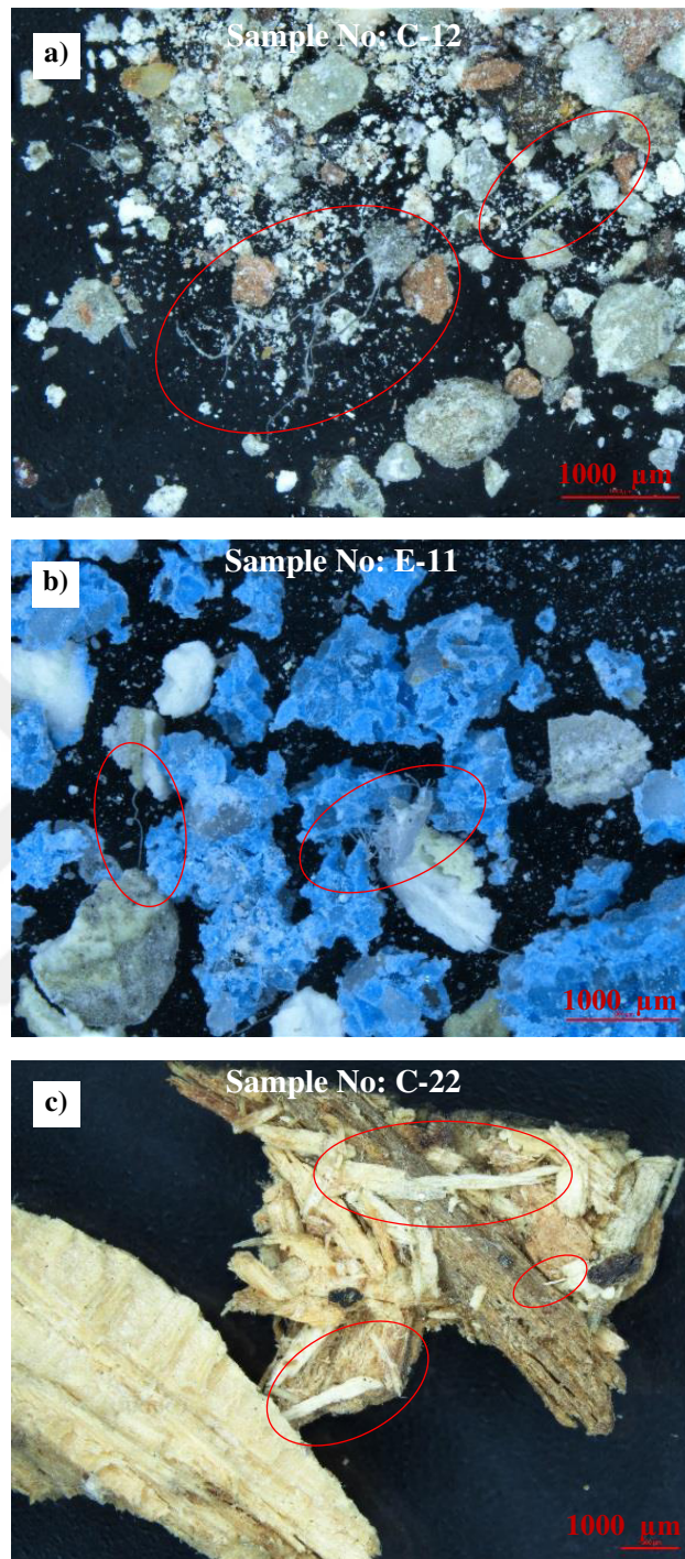
Figure 3.17. Representative micro-photographs by stereo microscope showing the samples with the fibrous form (marked by three check marks in Table 3.8); a) Wall (materials fragmented from main bodies), b) Floor (epoxy), c) Insulation (melamine coated chipboard ceiling cladding) [red circled area displays fibrous materials]
