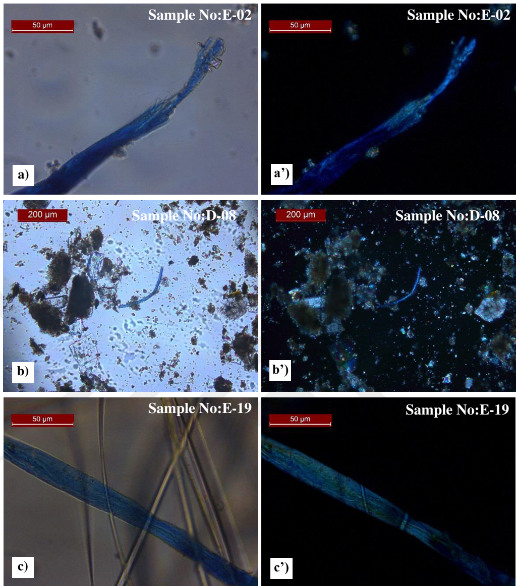
Figure 3.28. Representative micro-photographs for Crocidolite in; a) Wall (exposed concrete), b) Floor (concrete tile) c) Insulation (pipe insulation) [ a, b, c are plane polarized light, a', b', c' are cross polarized lights ]
