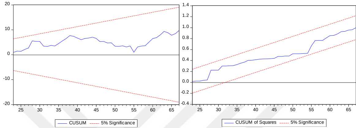
Figure 2.8. Tests of CUSUM and CUSUM of Square – HQ
