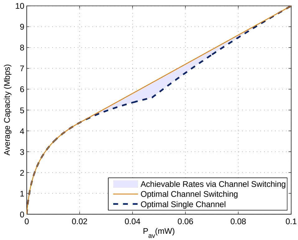
Figure 2.4: Average capacity versus average power limit for the optimal channel switching and the optimal single channel strategies for the scenario in Fig. 2.3, where P_{\text{pk}} = 0.1 \text{ mW} . The shaded area indicates the achievable rates via channel switching that are higher than those achieved by the optimal single channel strategy.
