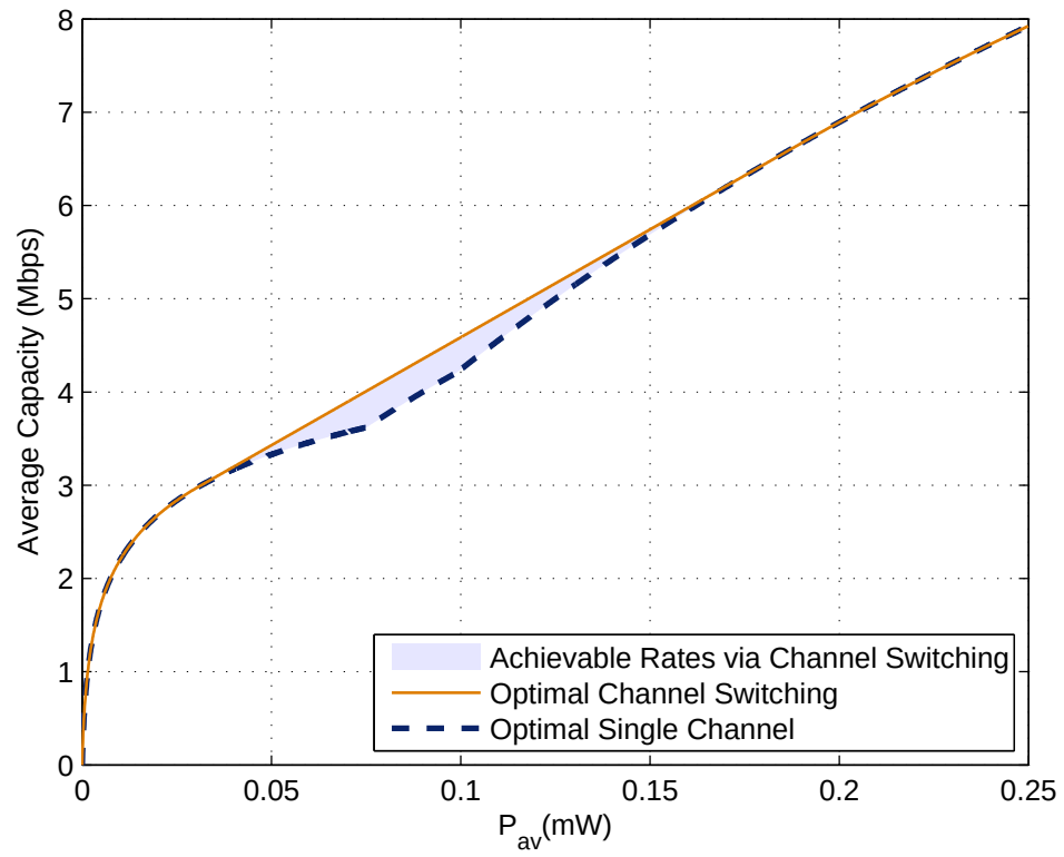
Figure 2.7: Average capacity versus average power limit for the optimal channel switching and the optimal single channel approaches for P_{\text{pk}} = 0.25 \text{ mW} . The shaded area indicates the achievable rates via channel switching that are higher than those achieved by the optimal single channel strategy.
