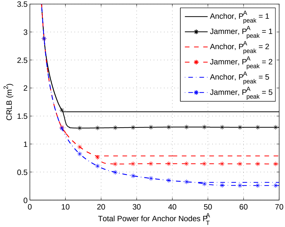
Figure 5.7: Minimum and maximum CRLBs (i.e., absolute utility values for the jammer and anchor nodes, respectively) of the target nodes versus total power of the anchor nodes for the scenario in Fig. 5.1, where P_T^J = 20 , P_{\text{peak}}^J = 10 , and the anchor nodes and the jammer nodes operate at Nash equilibrium in power control game \bar{\mathcal{G}} .
