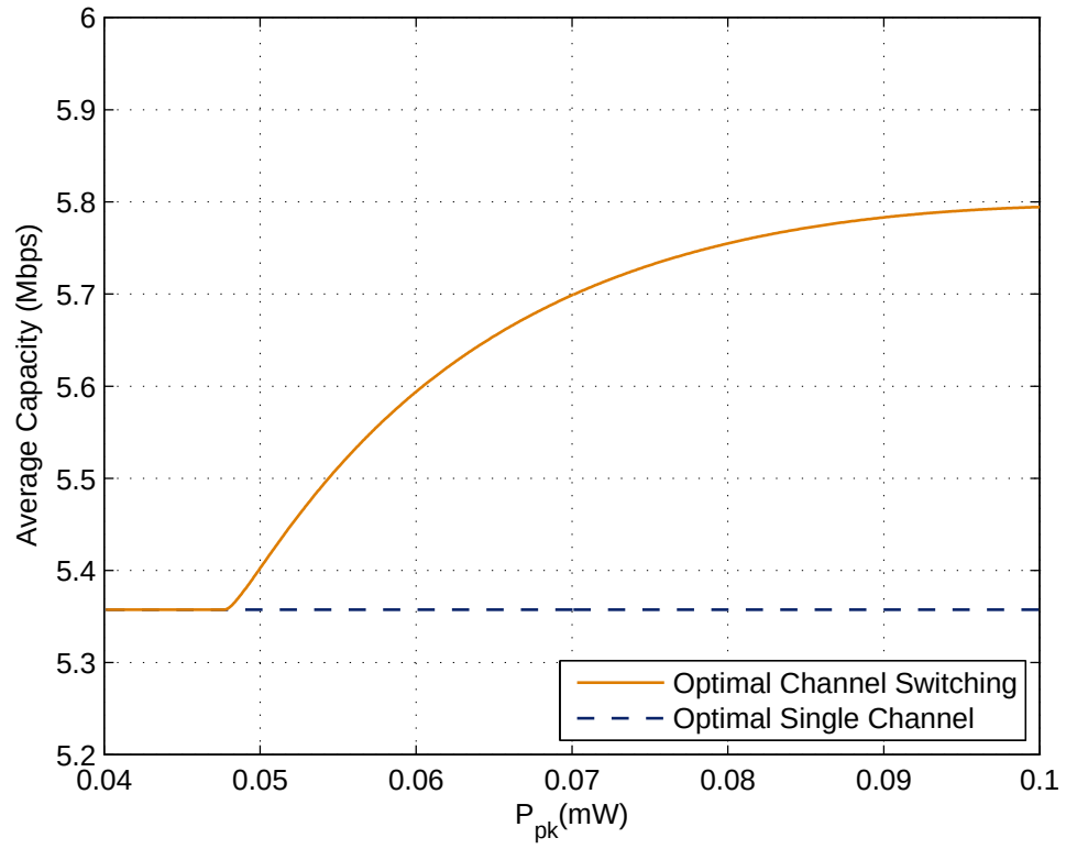
Figure 2.5: Average capacity versus peak power limit for the optimal channel switching and the optimal single channel strategies for the scenario in Fig. 2.3, where P_{av} = 0.04 mW.
