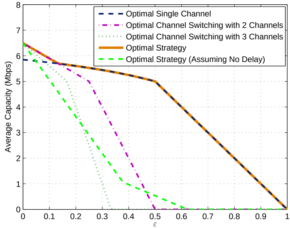
Figure 3.6: Average capacity versus channel switching delay factor for various optimal strategies for the scenario in Fig. 3.3, where P_{\text{av}} = 0.05 \text{ mW} and P_{\text{pk}} = 0.1 \text{ mW} .
