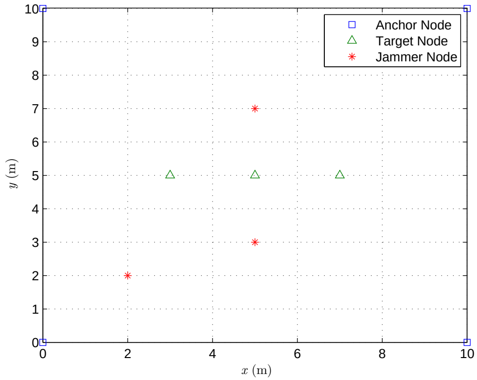
Figure 5.6: The simulated network including four anchor nodes positioned at [0\ 0] , [10\ 0] , [0\ 10] , and [10\ 10] m., three jammer nodes positioned at [5\ 3] , [5\ 7] , and [2\ 2] m., and three target nodes positioned at [3\ 5] , [5\ 5] , and [7\ 5] m.
