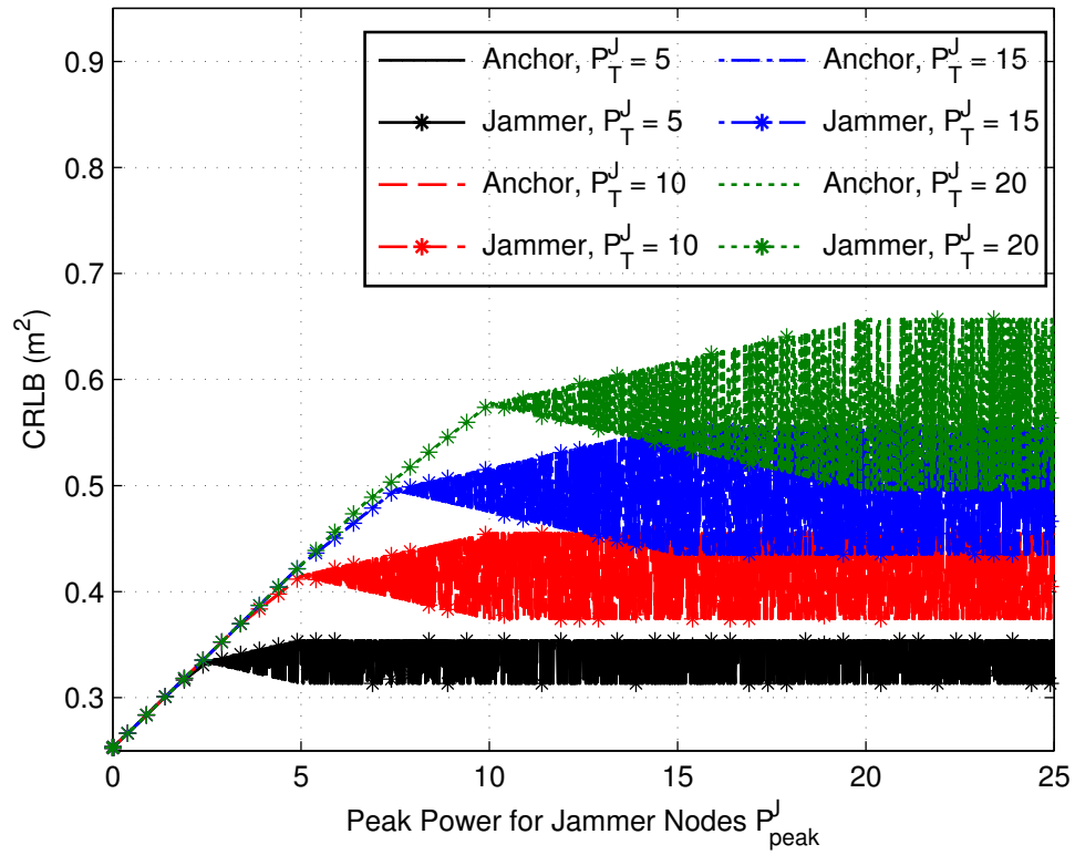
Figure 5.10: Minimum and maximum CRLBs (i.e., absolute utility values for the jammer and anchor nodes, respectively) of the target nodes versus peak power of the jammer nodes for the scenario in Fig. 5.1, where P_T^A = 20 , P_{\text{peak}}^A = 10 , and the anchor nodes and the jammer nodes operate at Nash equilibrium in power control game \bar{\mathcal{G}} .
