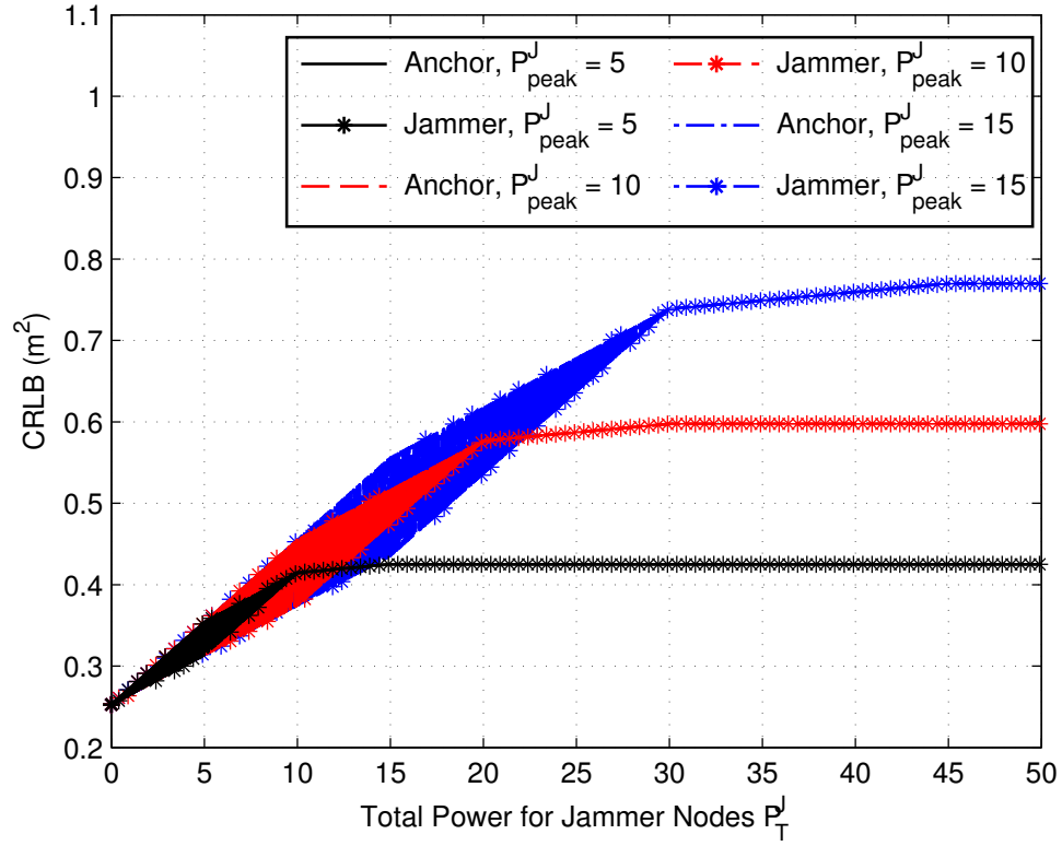
Figure 5.9: Minimum and maximum CRLBs (i.e., absolute utility values for the jammer and anchor nodes, respectively) of the target nodes versus total power of the jammer nodes for the scenario in Fig. 5.1, where P_T^A = 20 , P_{\text{peak}}^A = 10 , and the anchor nodes and the jammer nodes operate at Nash equilibrium in power control game \bar{\mathcal{G}} .
