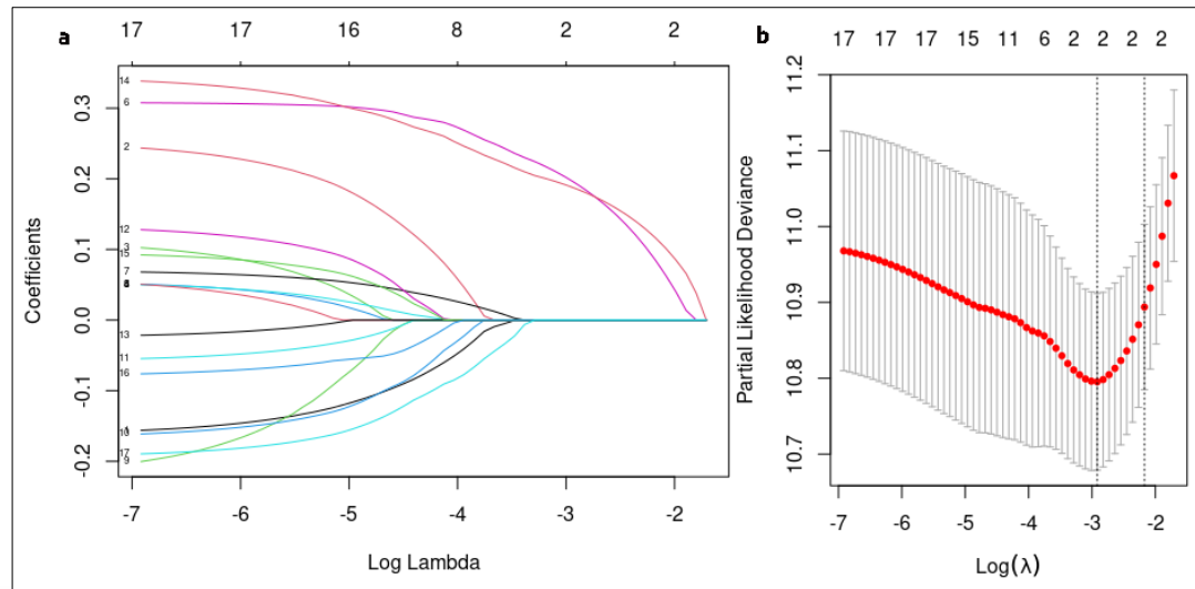
Figure 3.63 LASSO Regularization.
