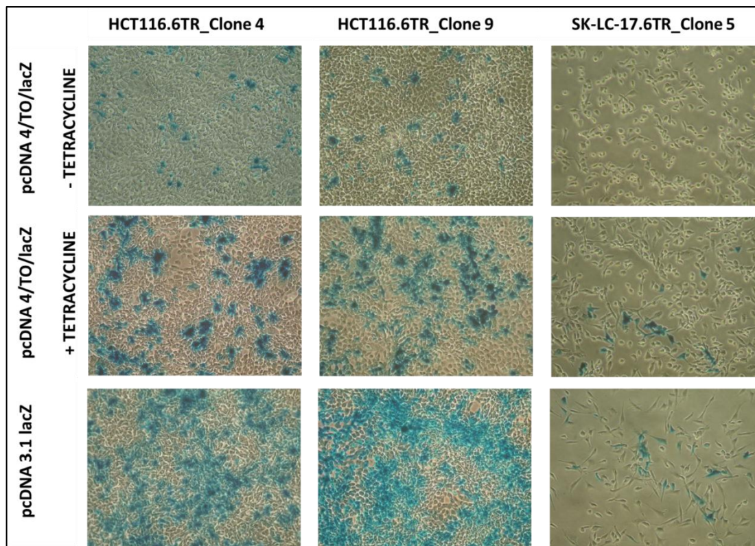
Figure 3.2.7 1: 3 candidate clones are identified as a result of \beta -Galactosidase staining experiment performed after pcDNA4/TO/lacZ transfection to stable clones expressing Tet repressor.
