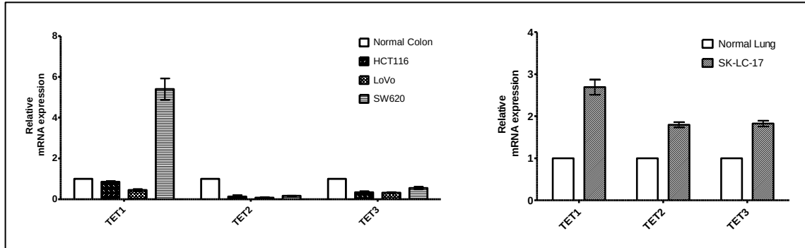
Figure 3.2.6 1: The mRNA levels of TET genes ( TET1 , TET2 , TET3 ) in colon cancer and lung cancer cell lines with respect to normal counterparts.
