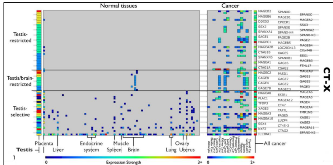
Figure 1.1.1 1: The expression pattern of CT-X genes in normal tissues and cancer CT genes on chromosome X are mainly expressed in testis and placenta among normal tissues. CT-X gene expression is detected in brain and in some of the normal tissues at very low levels albeit. Various CT genes are induced and detected in cancer tissues. Adopted from [6]. (Hofmann et al. PNAS, 105, 51, 2008 Genome-wide analysis of cancer/testis gene expression. Copyright (2008) National Academy of Sciences, U.S.A.)
