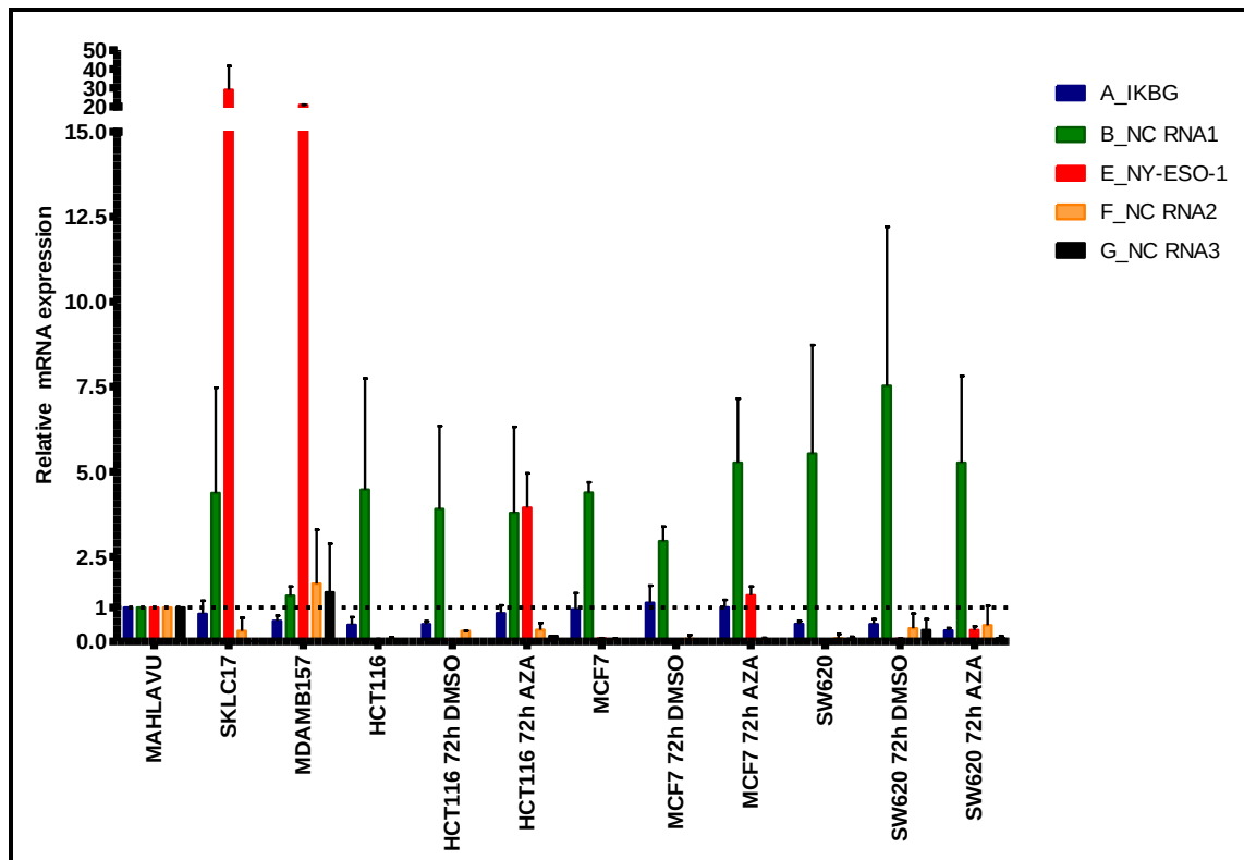
Figure 3.3.1 2: The expressions of noncoding RNAs in repeat region, IkBG and NY-ESO-1 in NY-ESO-1 positive (Mahlavu, SK-LC-17 and MDA-MB157) and negative cell lines (HCT116, SW20 and MCF-7) are analyzed by q RT-PCR.
