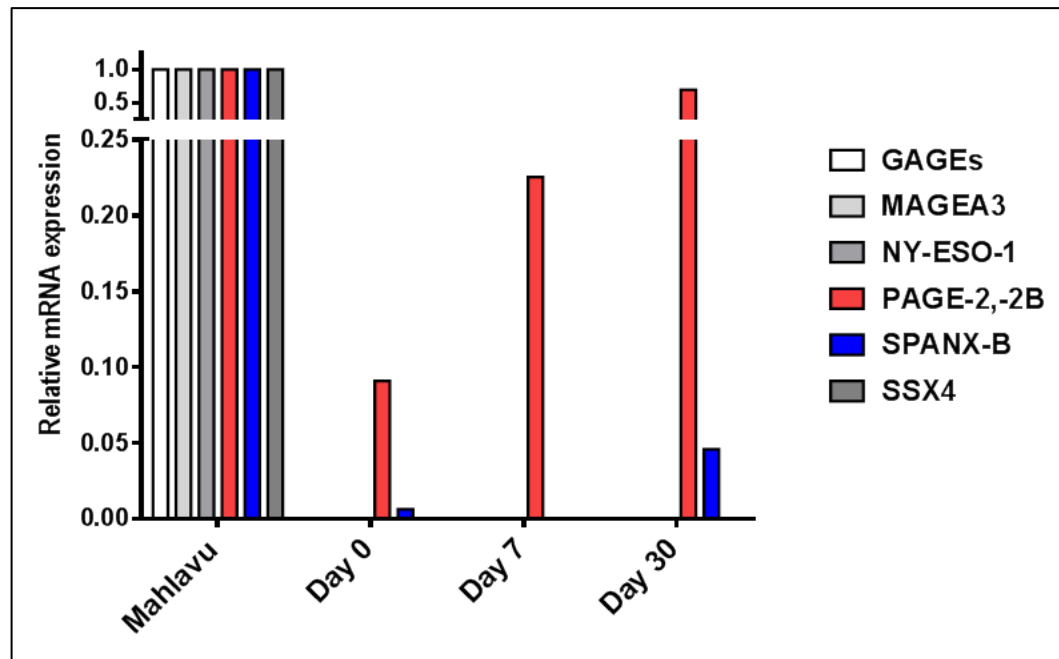
Figure 3.1.1 3: Among 6 CT gene families; the gene expressions of PAGE-2,-2B and SPANX-B increase in Caco-2 spontaneous differentiation.
