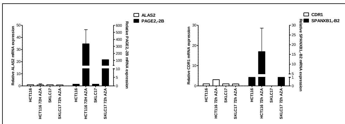
Figure 3.2.4 1: The response of CT genes and CT proximal genes to 5-aza-2'-deoxycytidine treatment is showed by q RT-PCR.
