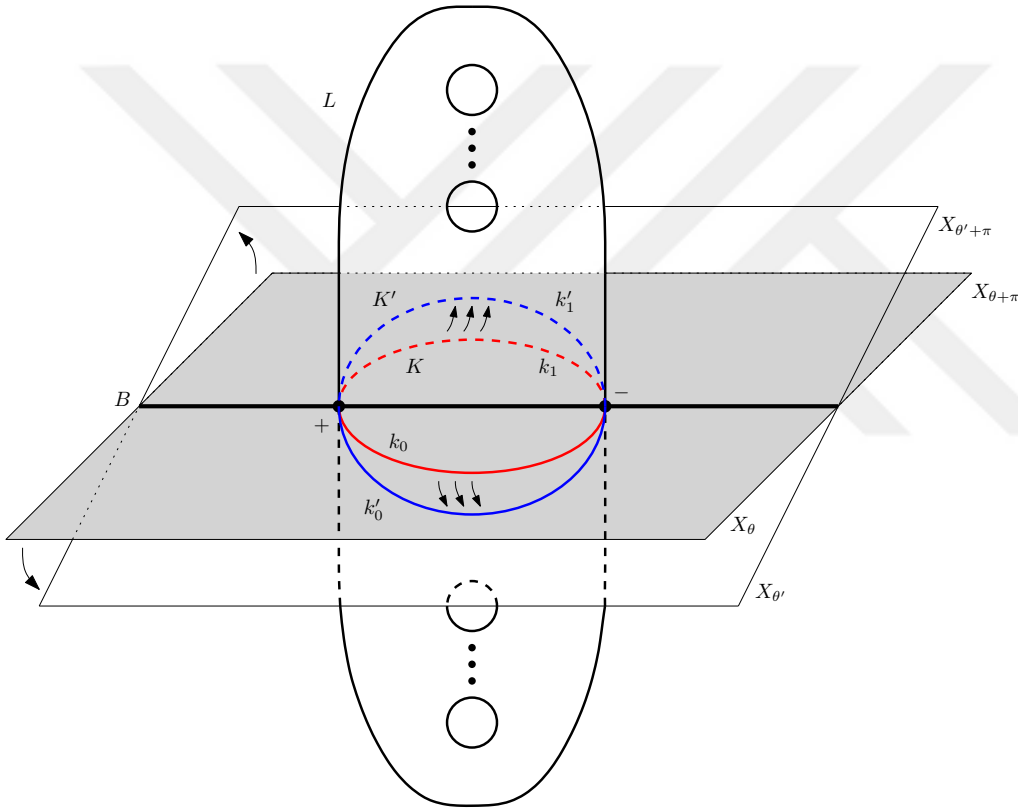
Figure 5.1: Replacing X_0 = X_\theta (resp. X_1 = X_{\theta+\pi} ) with a nearby (Stein) page X_{\theta'} (resp. X_{\theta'+\pi} ) which are still intersecting L' transversely. A new knot component K' = k'_0 \cup k'_1 (isotopic to older one K ) of the link of intersection of L' with the new double X_{\theta'} \cup_{\partial} X_{\theta'+\pi} .
