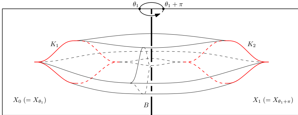
Figure 6.1: A schematic picture of the front projection of the Legendrian Clifford torus T_k \subset (\mathbb{S}^3, \xi_3) onto \mathbb{R}^3 with coordinates z, y_1, y_2 . The components K_1, K_2 (in red) of the (un)link of intersection of T_k with the double X_0 \cup_{\partial} X_1 \approx \mathbb{S}^4 of a page X \approx D^4 of the trivial open book on \mathbb{S}^5 . (Note: B \approx \mathbb{S}^3 and T_k \pitchfork B = \emptyset .)
