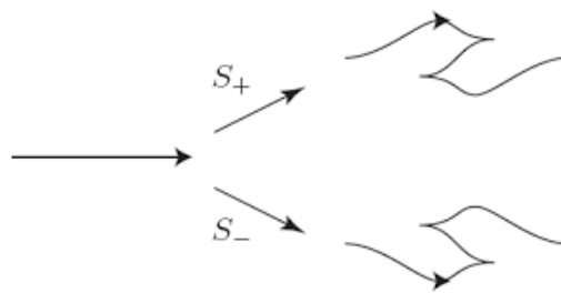
Figure 2.8: The positive and negative stabilizations of L .
