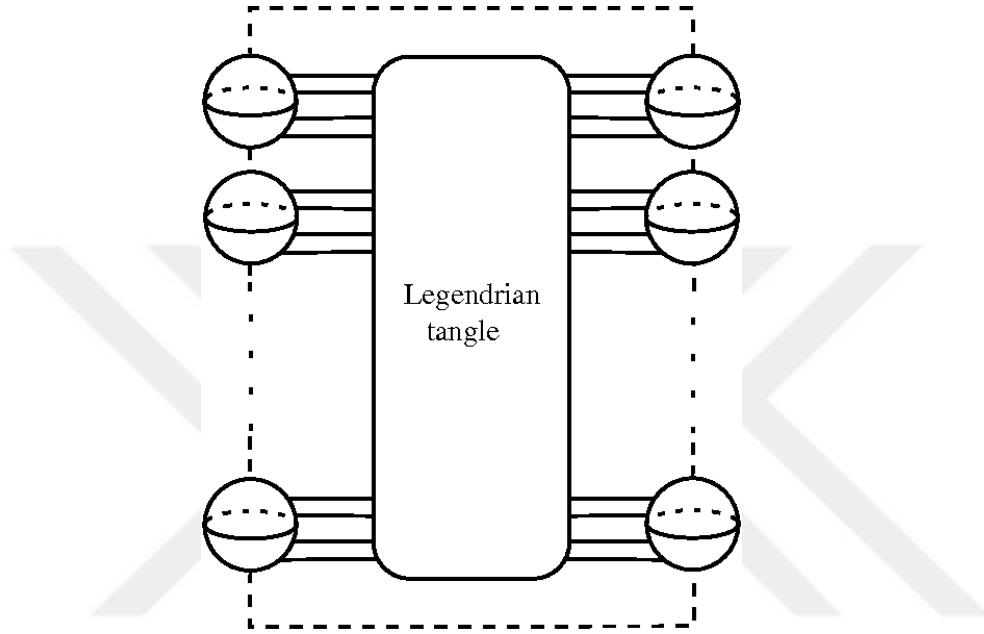
Figure 2.9: A Legendrian link diagram.
