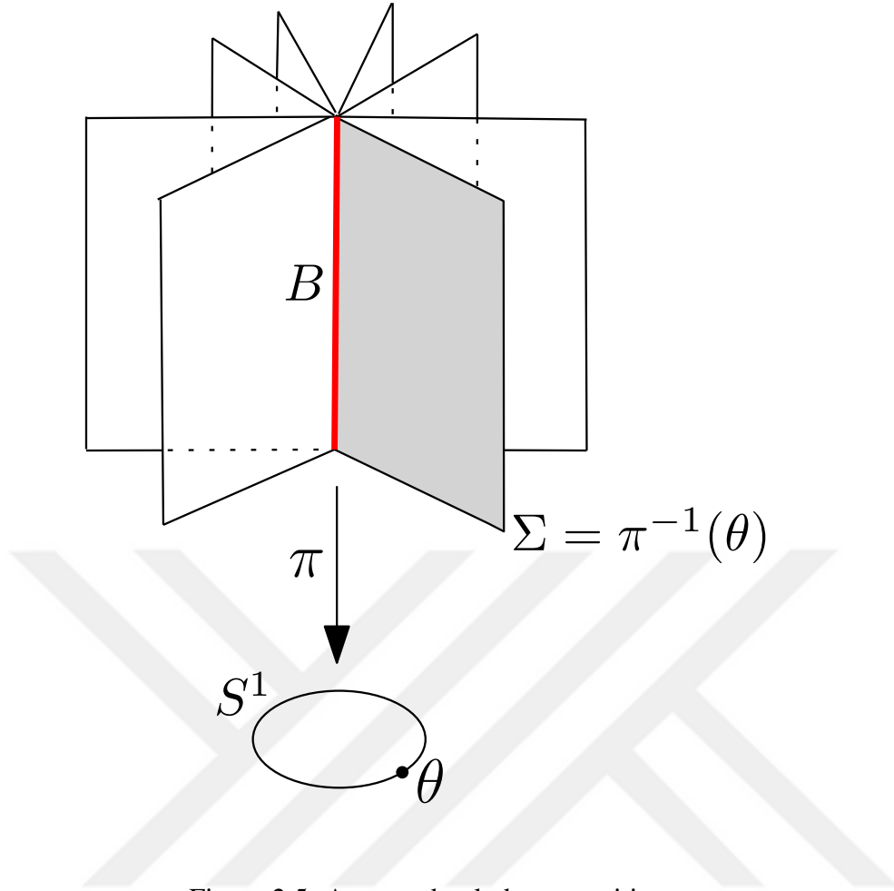
Figure 2.5: An open book decomposition.
