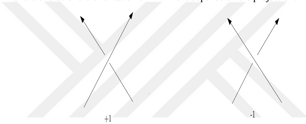
Figure 2.6: Positive and negative crossings.
