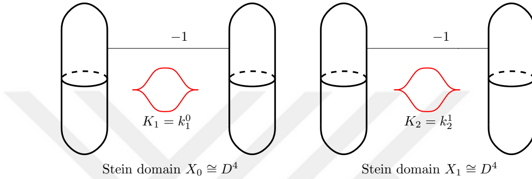
Figure 6.2: Realizing the (un)link of transverse intersection of the Legendrian Clifford torus T_k with the double X_0 \cup_{\partial} X_1 \approx \mathbb{S}^4 of a page X \approx D^4 in the Stein diagrams of (X_0, d\alpha_5|_{X_0}) and (X_1, d\alpha_5|_{X_1}) .
