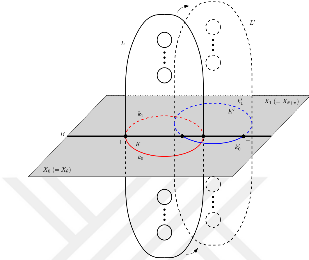
Figure 4.1: A regular Legendrian isotopy L_t taking L_0 = L to another Legendrian L_1 = L' which is still intersecting the double D(X) = X_0 \cup_\partial X_1 transversally, but the new points of intersection in L' \cap B are possibly different than the older ones.
