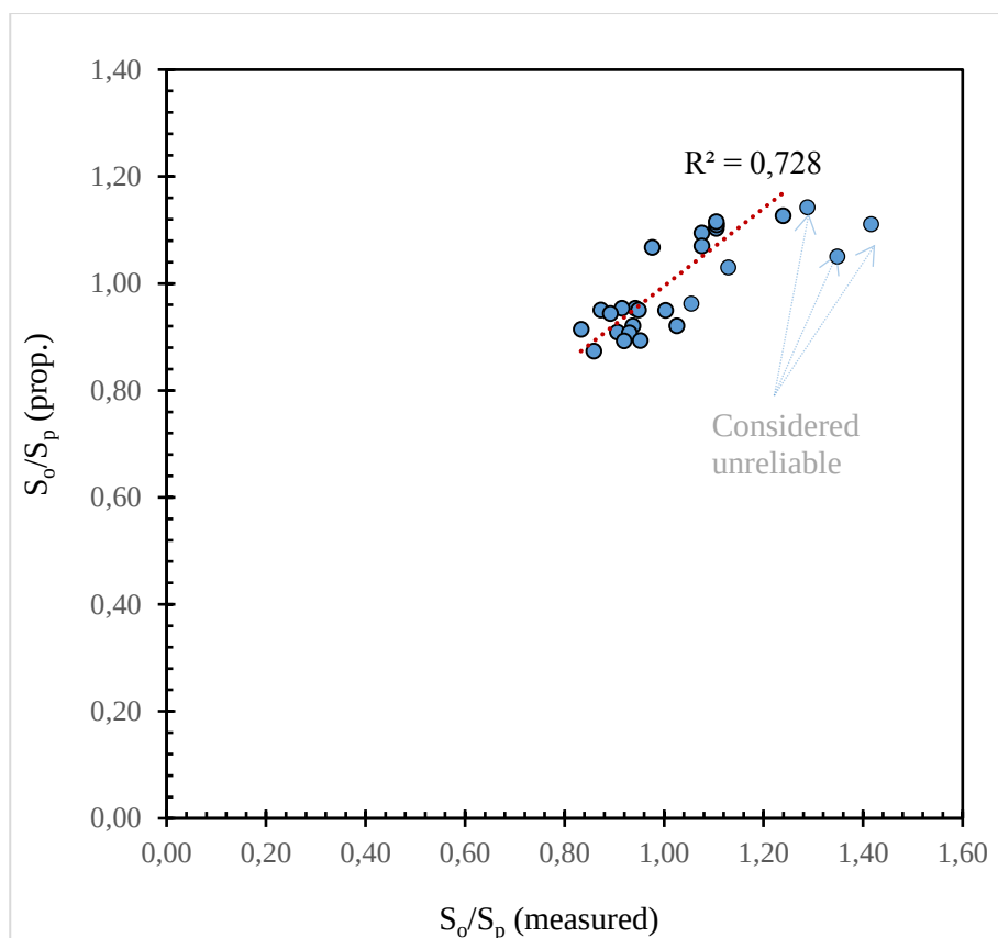
Figure 4.70. S_o/S_p (measured) vs. S_o/S_p (proposed) graph
