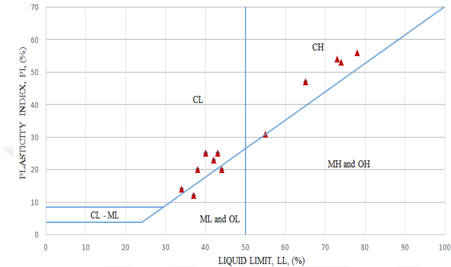
Figure A.23. Plasticity chart for BSSK-461
