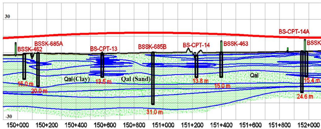
Figure 3.46. The longitudinal geological section of Km: 150+500
