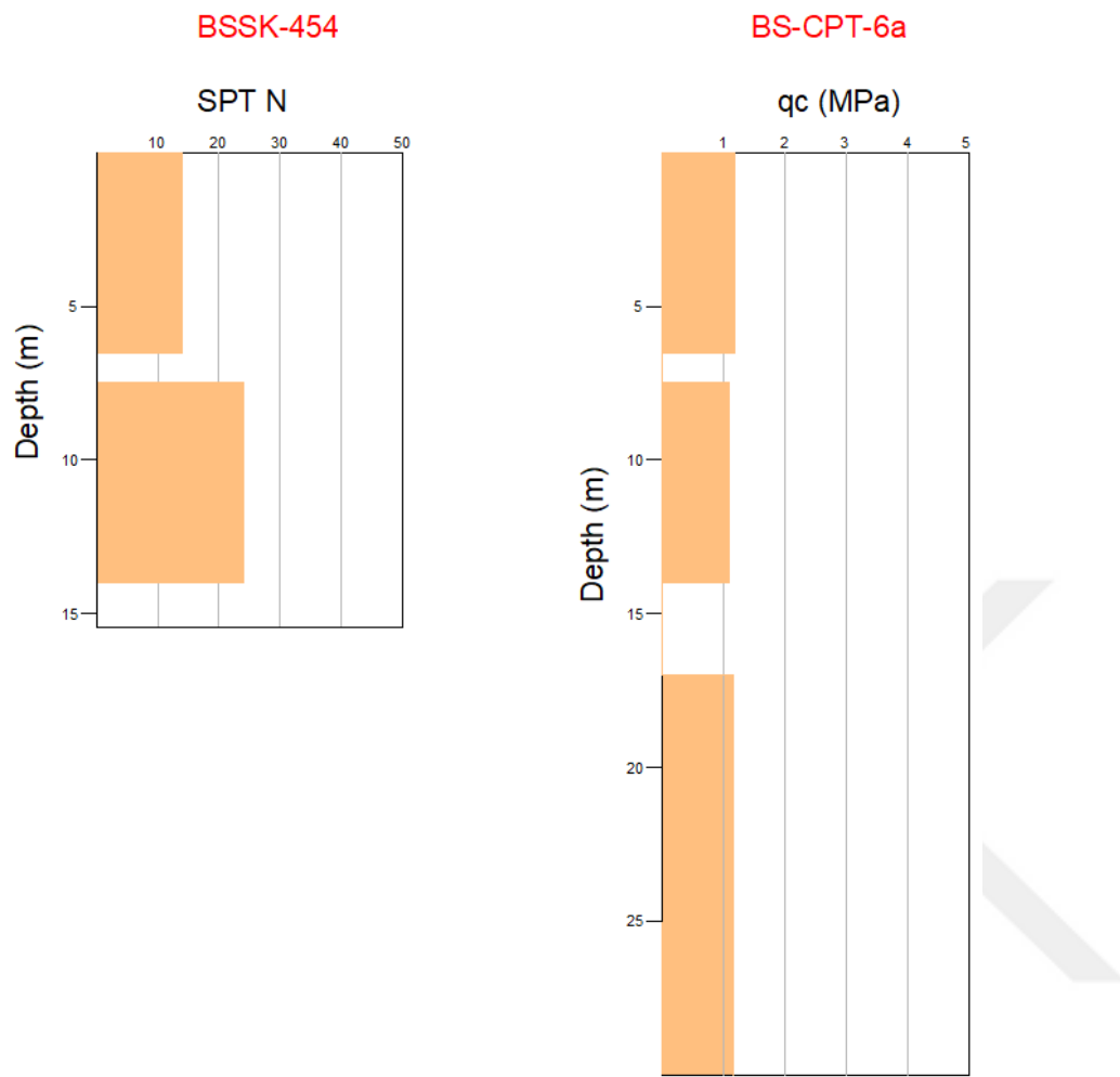
Figure 3.29. SPT N vs. Depth (m) and q_c (MPa) vs. Depth (m) graphs for clay layers
