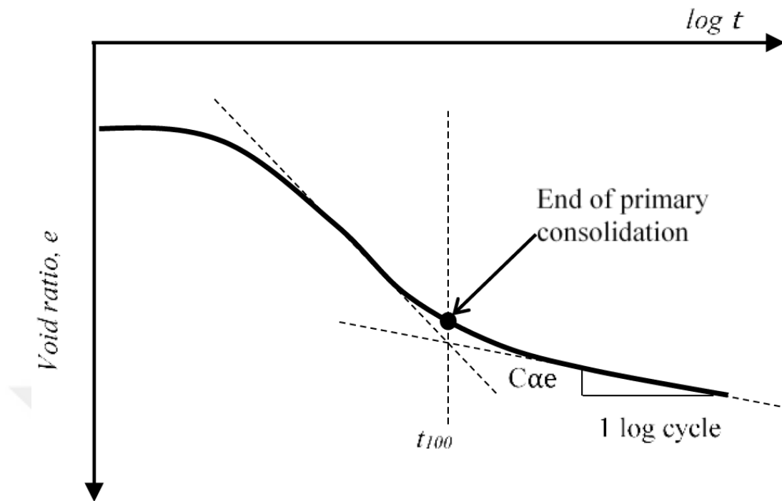
Figure 2.9. Identification of secondary compression coefficient (Zhao, 2017)
