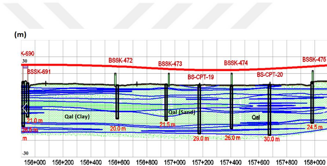
Figure 3.67. The longitudinal geological section of Km: 157+400
