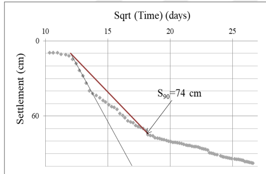
Figure 4.34. Primary consolidation settlement amounts for Station 11 at Km: 147+000 and for Station 12 at Km: 149+000
