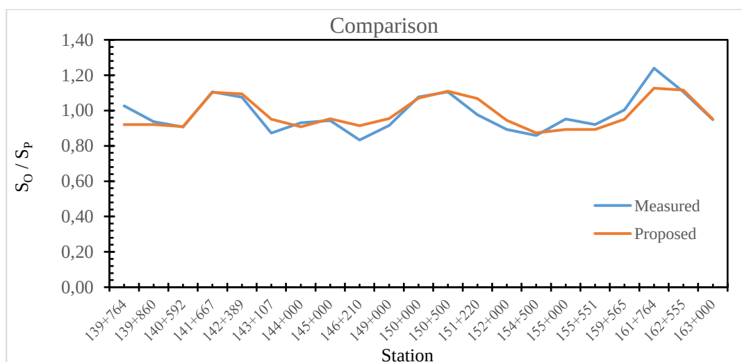
Figure 4.71. Comparison graph for the measured and proposed S_o/S_p for each station
