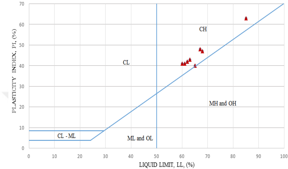
Figure A.15. Plasticity chart for BSSK-454
