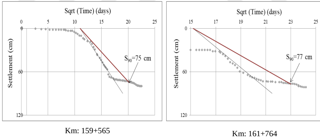
Figure 4.40. Primary consolidation settlement amounts for Station 23 at Km: 159+565 and for Station 24 at Km: 161+764
