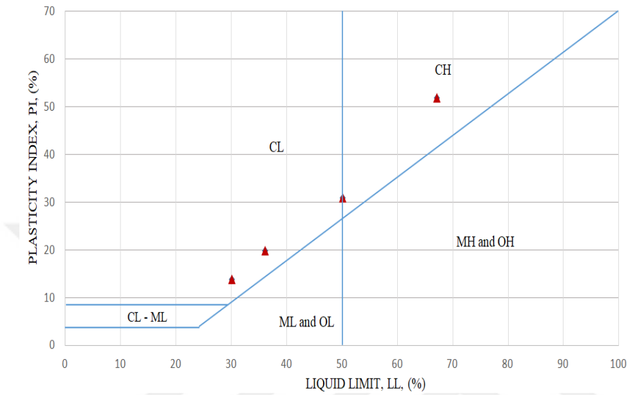
Figure A.19. Plasticity chart for BSSK-457
