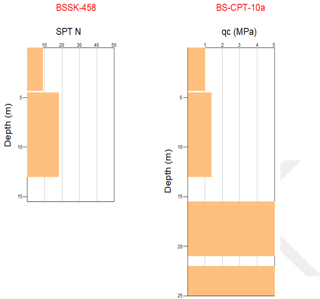
Figure 3.38. SPT N vs. Depth (m) and q_c (MPa) vs. Depth (m) graphs for clay layers
