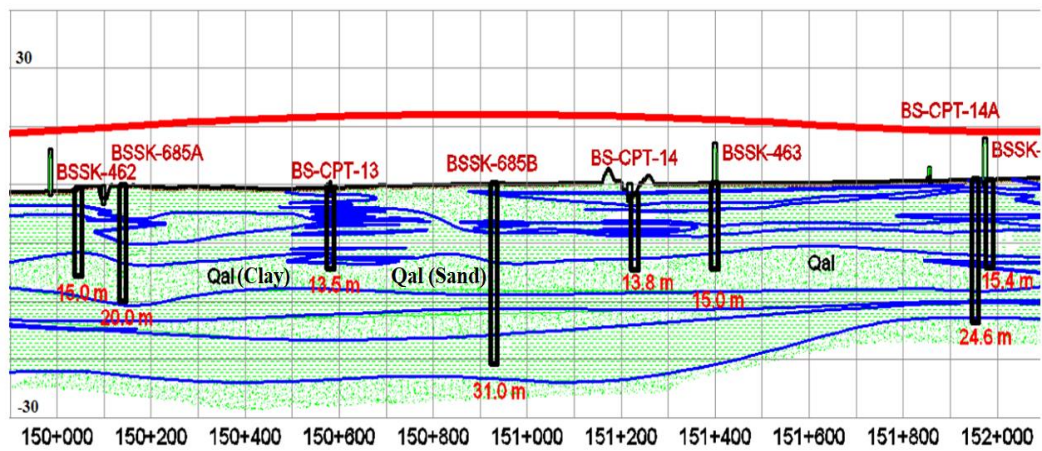
Figure 3.43. The longitudinal geological section of Km: 150+000
