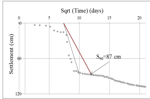
Figure 4.33. Primary consolidation settlement amounts for Station 9 at Km: 145+000 and for Station 10 at Km: 146+210
