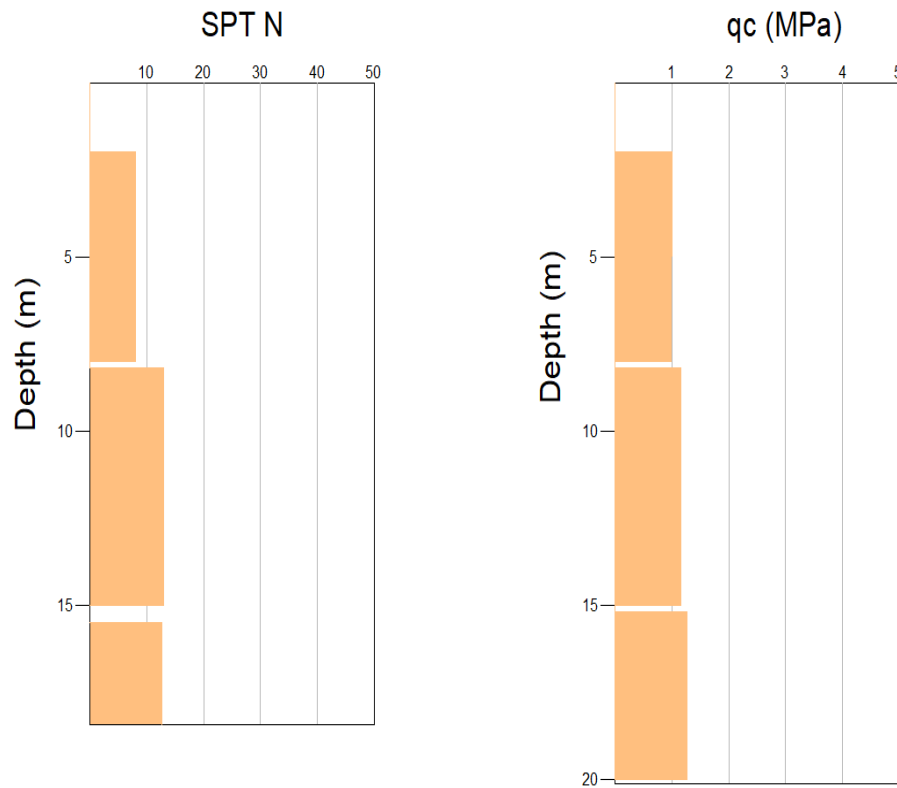
Figure 3.83. SPT N vs. Depth (m) and q_c (MPa) vs. Depth (m) graphs for clay layers
