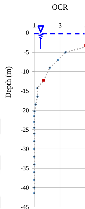
OCR vs. Depth (m) Graph
