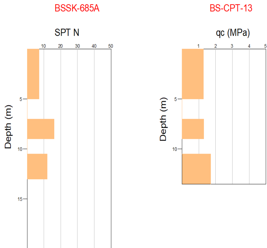
Figure 3.47. SPT N vs. Depth (m) and q_c (MPa) vs. Depth (m) graphs for clay layers
