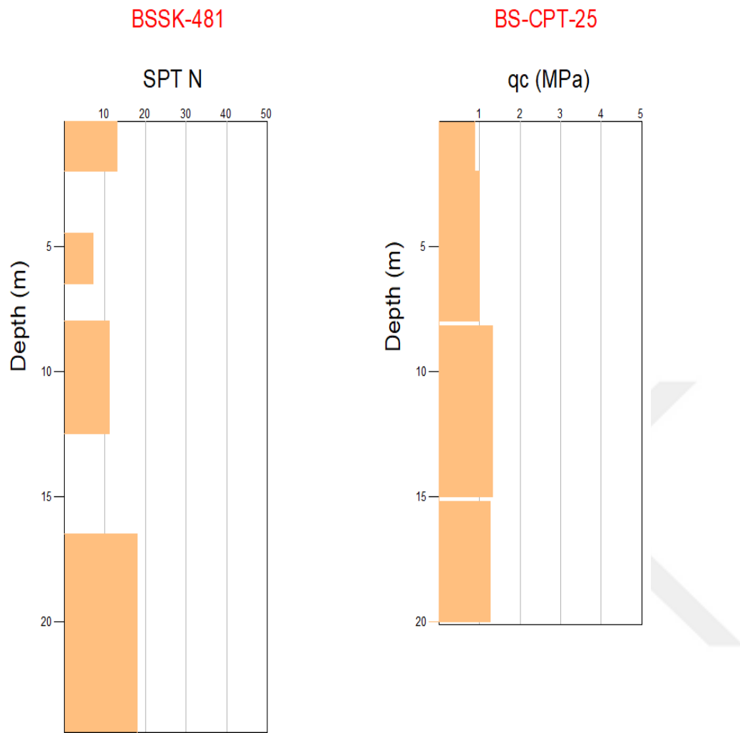
Figure 3.80. SPT N vs. Depth (m) and q_c (MPa) vs. Depth (m) graphs for clay layers
