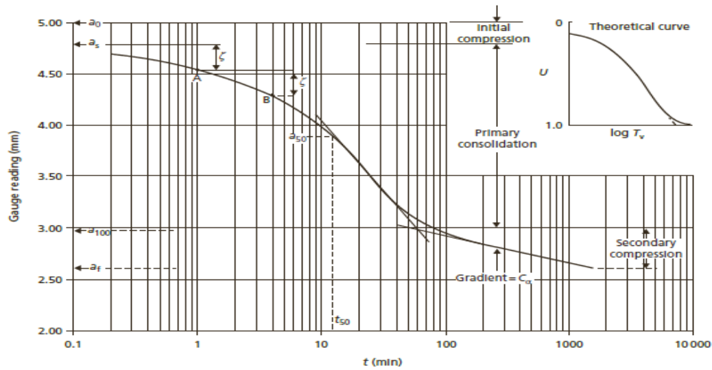
Figure 2.6. Casagrande's Log of Time Method (Craig, 1997)
