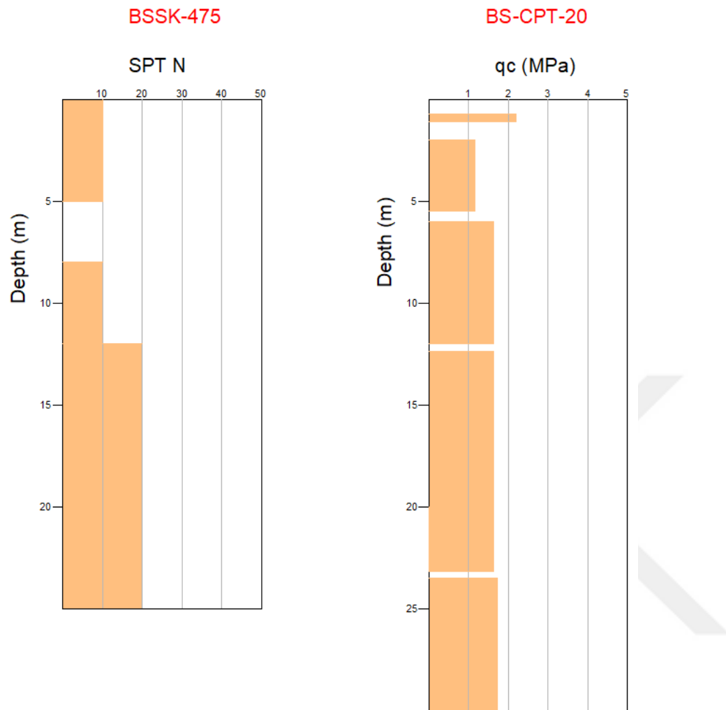
Figure 3.71. SPT N vs. Depth (m) and q_c (MPa) vs. Depth (m) graphs for clay layers
