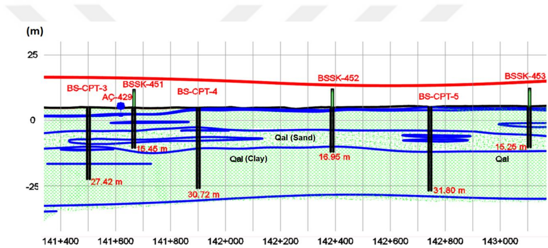
Figure 3.19. The longitudinal geological section of Km: 142+000
