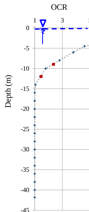
OCR vs. Depth (m) Graph
