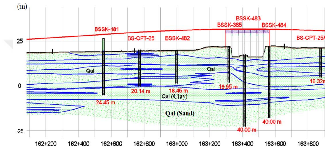
Figure 3.82. The longitudinal geological section of Km: 163+000
