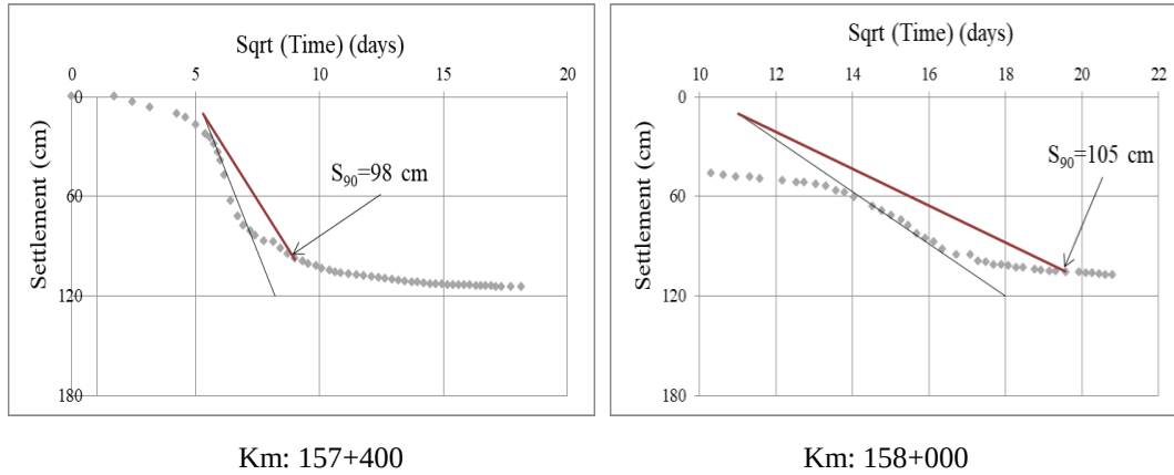
Figure 4.39. Primary consolidation settlement amounts for Station 21 at Km: 157+400 and for Station 22 at Km: 158+000
