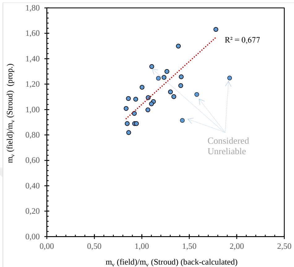
Figure 4.76 m_v \text{ (field)}/m_v \text{ (Stroud)} (back-calculated) vs. m_v \text{ (field)}/m_v \text{ (Stroud)} (proposed) graph
