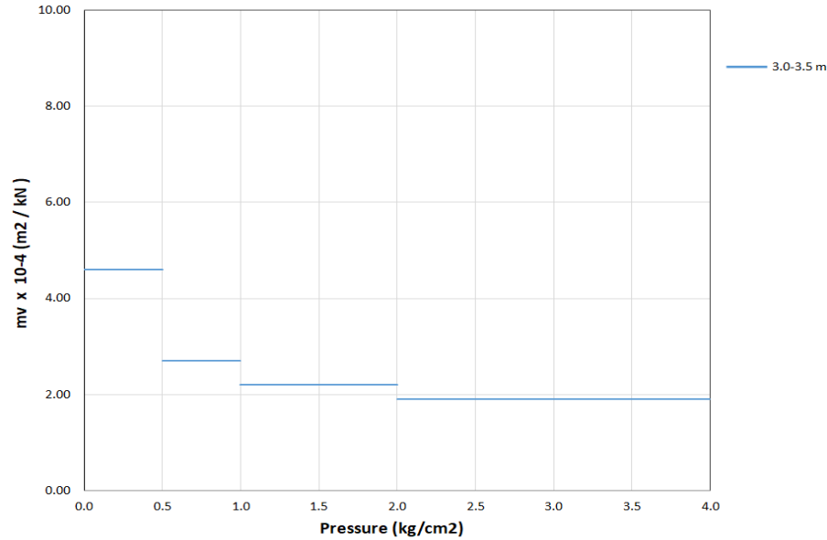
Figure A.8. The coefficient of volume compressibility ( m_v ) chart for BSSK-451
