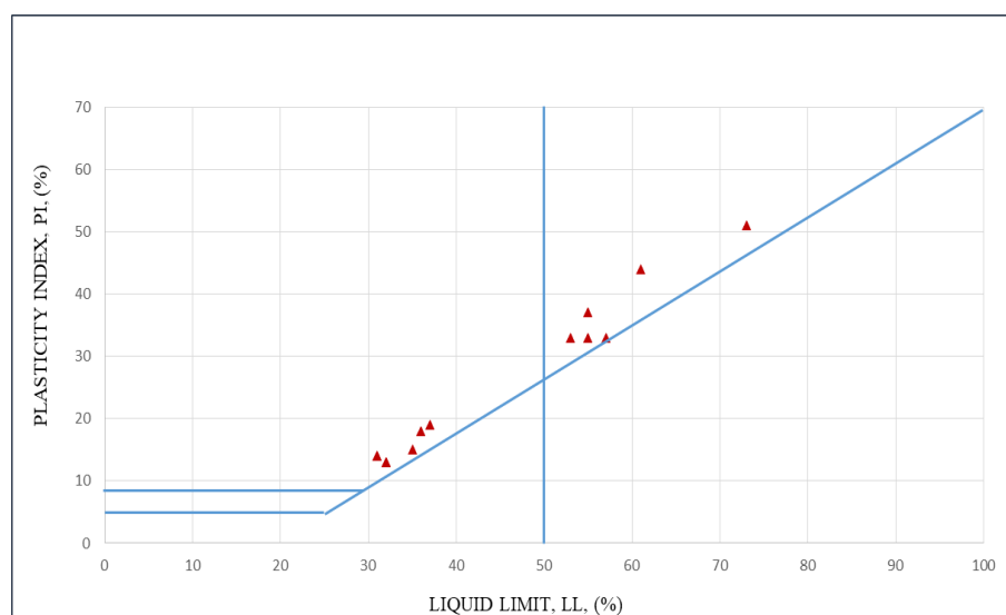
Figure A.46. Plasticity chart for BSSK-477
