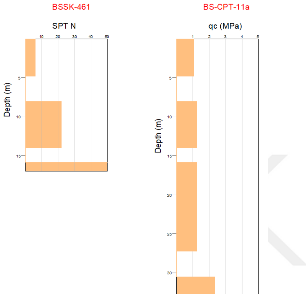
Figure 3.41. SPT N vs. Depth (m) and q_c (MPa) vs. Depth (m) graphs for clay layers
