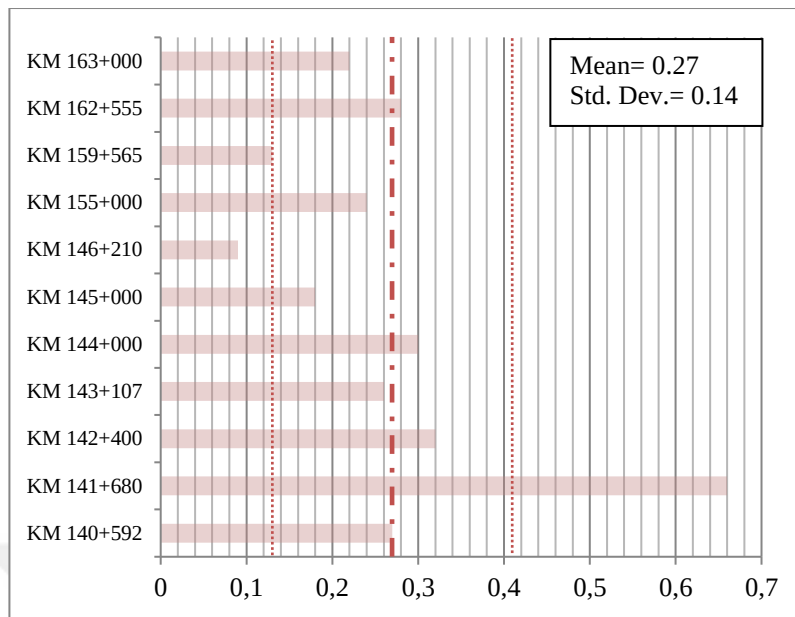
Figure 4.57. C_t/C_c graph for each station
