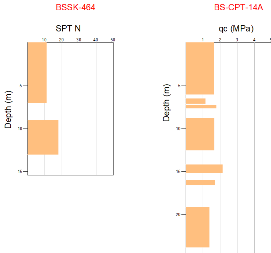
Figure 3.53. SPT N vs. Depth (m) and q_c (MPa) vs. Depth (m) graphs for clay layers
