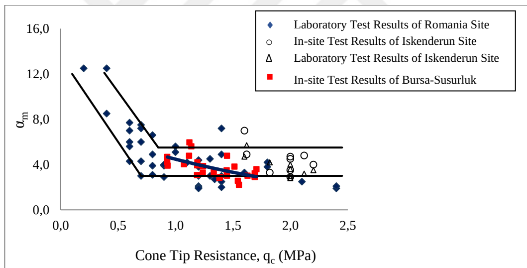
Figure 4.69. The variation of \alpha_m values from cone tip resistance, q_c (MPa) (Erol et al., 2004)
