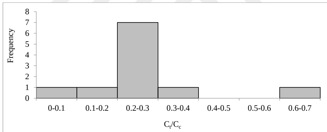
Figure 4.58. Histogram graph for C_t/C_c
