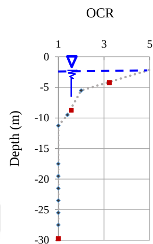
OCR vs. Depth (m) Graph
