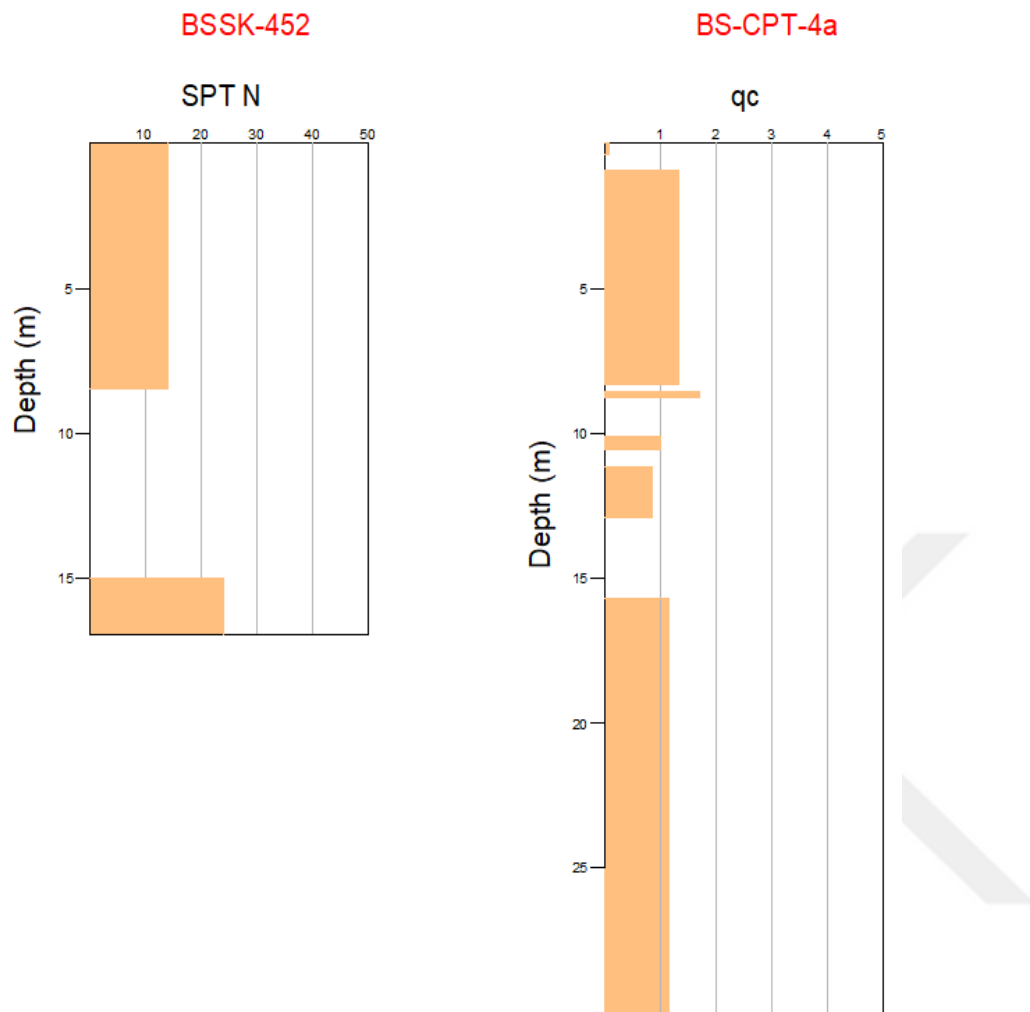
Figure 3.23. SPT N vs. Depth (m) and q_c (MPa) vs. Depth (m) graphs for clay layers
