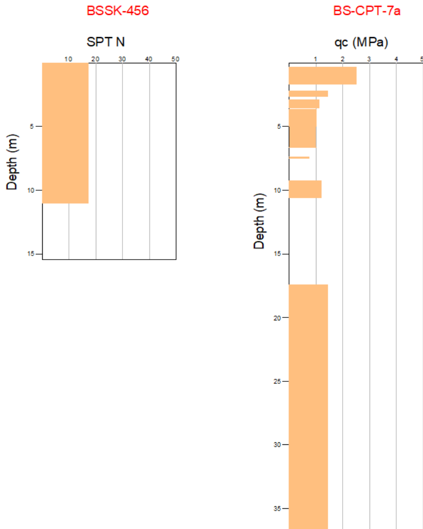
Figure 3.32. SPT N vs. Depth (m) and q_c (MPa) vs. Depth (m) graphs for clay layers
