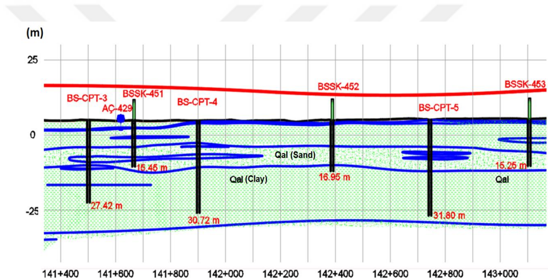
Figure 3.22. The longitudinal geological section of Km: 142+400
