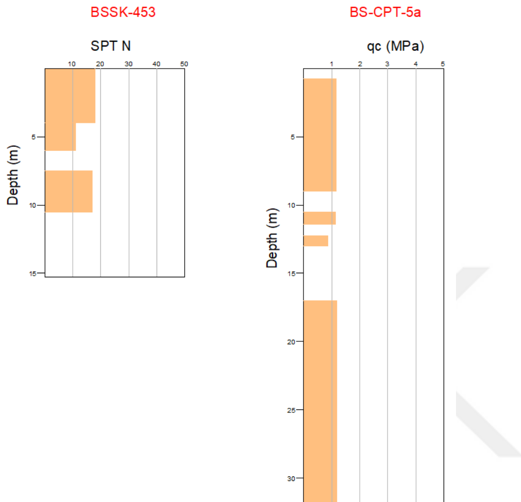
Figure 3.26. SPT N vs. Depth (m) and q_c (MPa) vs. Depth (m) graphs for clay layers
