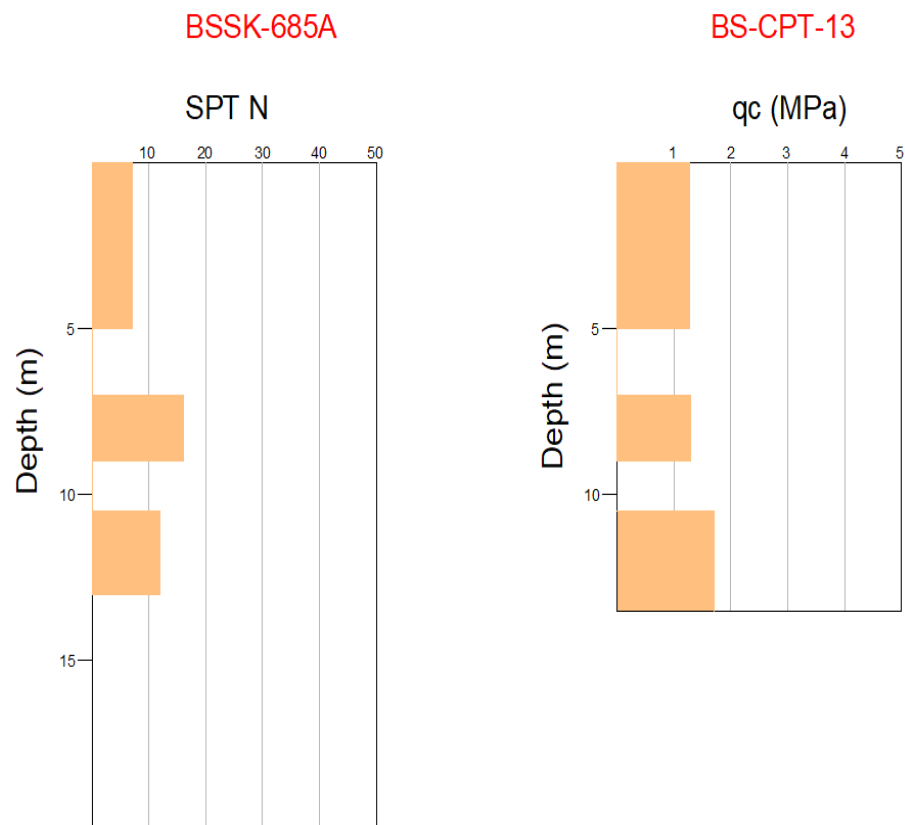
Figure 3.44. SPT N vs. Depth (m) and q_c (MPa) vs. Depth (m) graphs for clay layers
