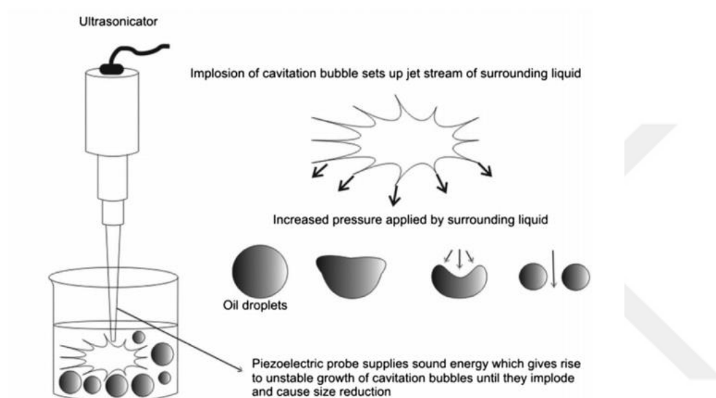
Figure 1.10: Schematic representation of ultrasonication method (Cheaburu-Yilmaz, Karasulu, & Yilmaz, 2018)
