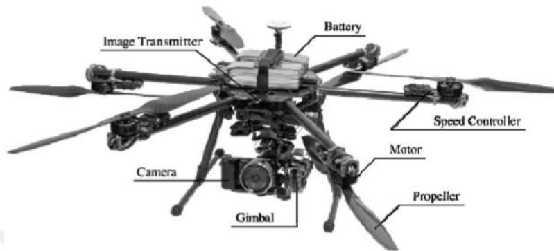
Figure 2.3. A representative Digital Camera Mounted UAV (Liu et al., 2014)
