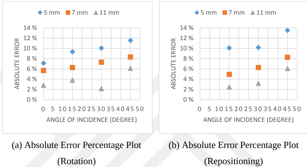
Figure 5.6. AEP Plot for RC Specimen
