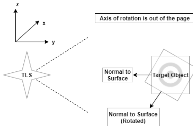
Figure 5.2. Top View of Rotation Method
