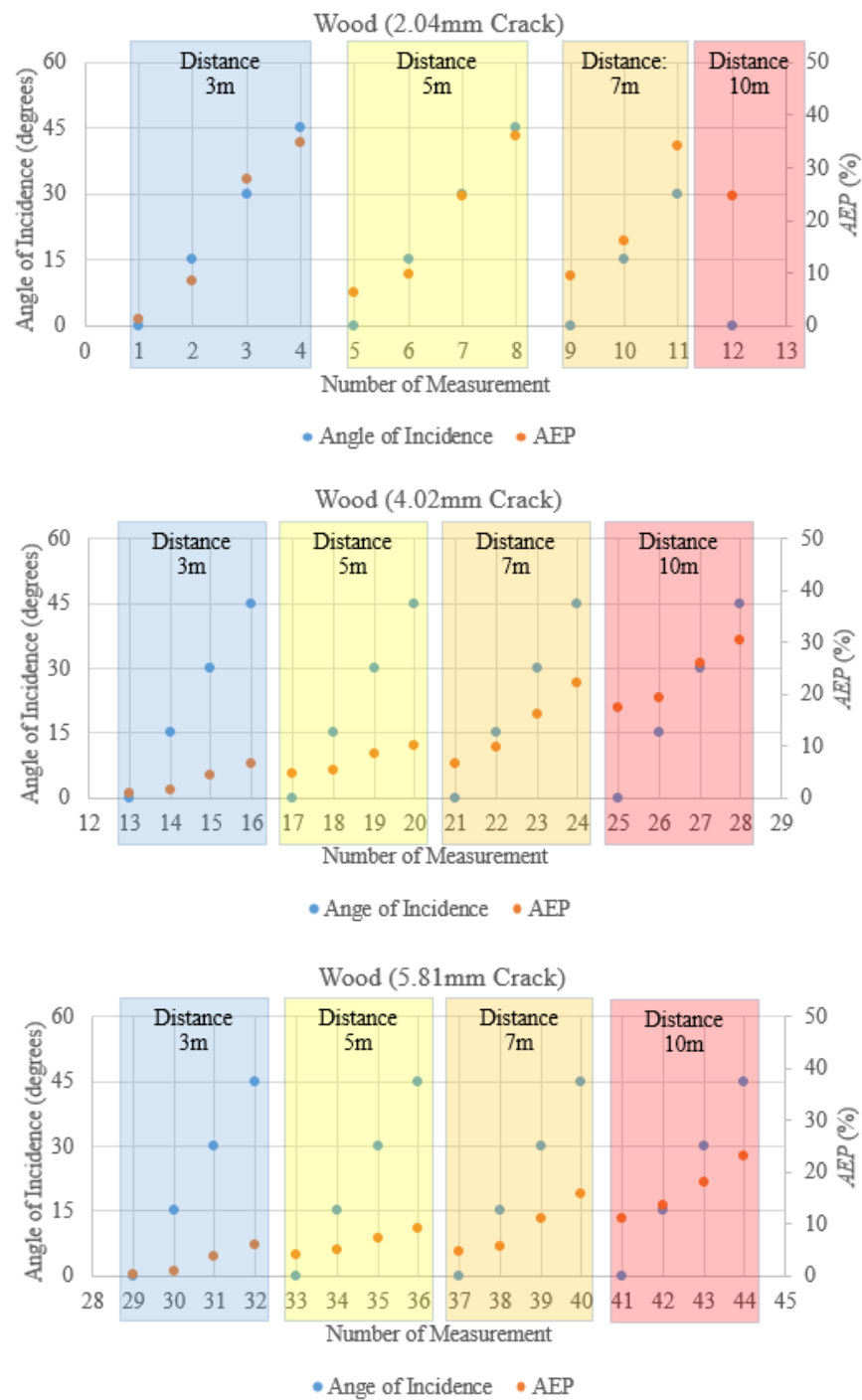
Figure 5.13. Dispersion of Values for Wooden Specimen
