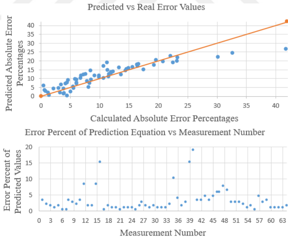
Figure 5.22. Error Performance of the Equation Derived (Coated RC Specimen)
