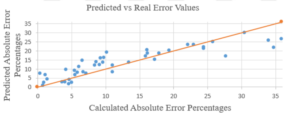
Figure 5.19. Error Performance of the Equation Derived (RC Specimen)
