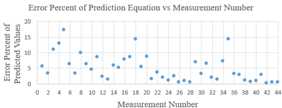
Figure 5.20. Error Performance of the Equation Derived (Wooden Specimen)
