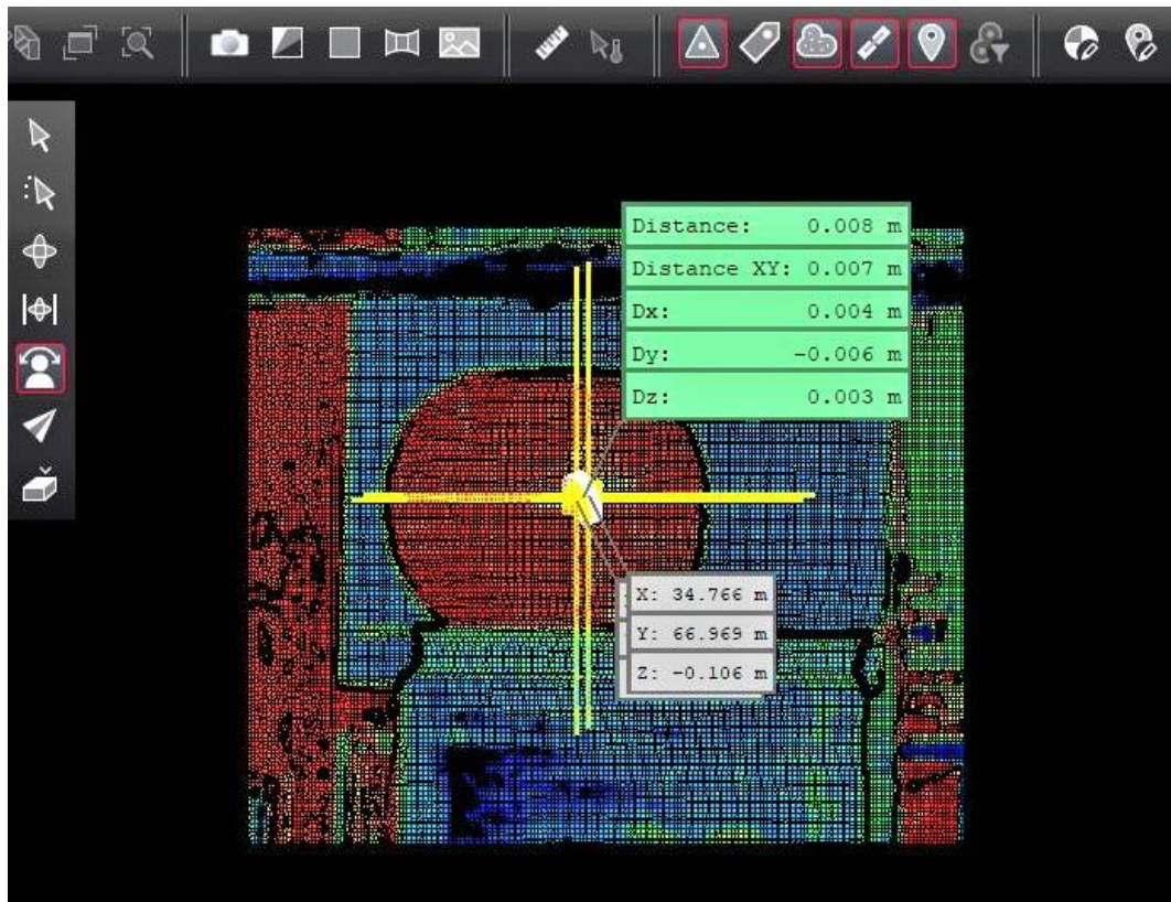
Figure 4.8. Measurement in Software Scan Number 7, Case Study-1, Stage-2
