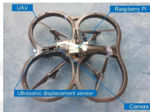
Figure 2.4. UAV-Based Prototype for Crack Identification (H. Kim et al., 2015)
