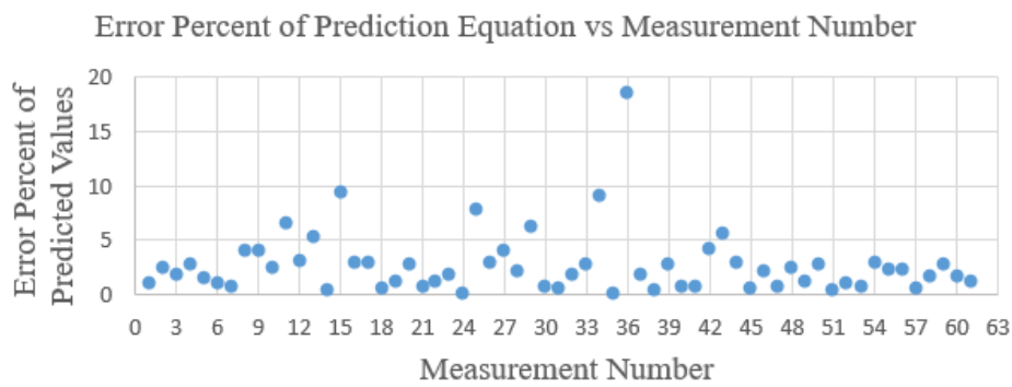
Figure 5.19. Error Performance of the Equation Derived (RC Specimen)
