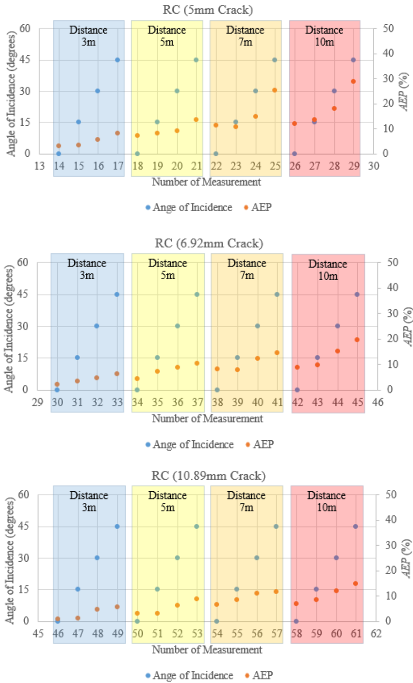
Figure 5.11. Dispersion of Values for RC Specimen
