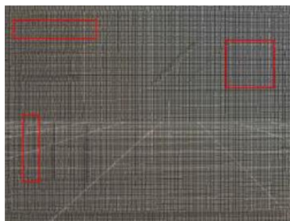
Figure 4.11. The Cracks Captured, Resolution 6.1 mm, Scanning Distance 7 m (Shi & Ergan, 2019)
