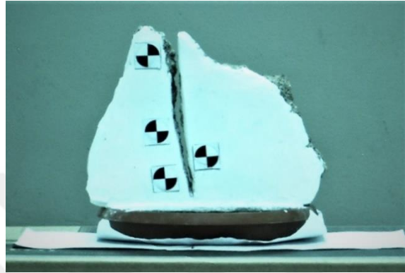
Figure 5.16. Satin Plaster Coated RC Specimen Used in Case Study-4
