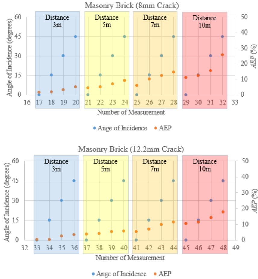
Figure 5.15. Dispersion of Values for Masonry Brick Specimen
