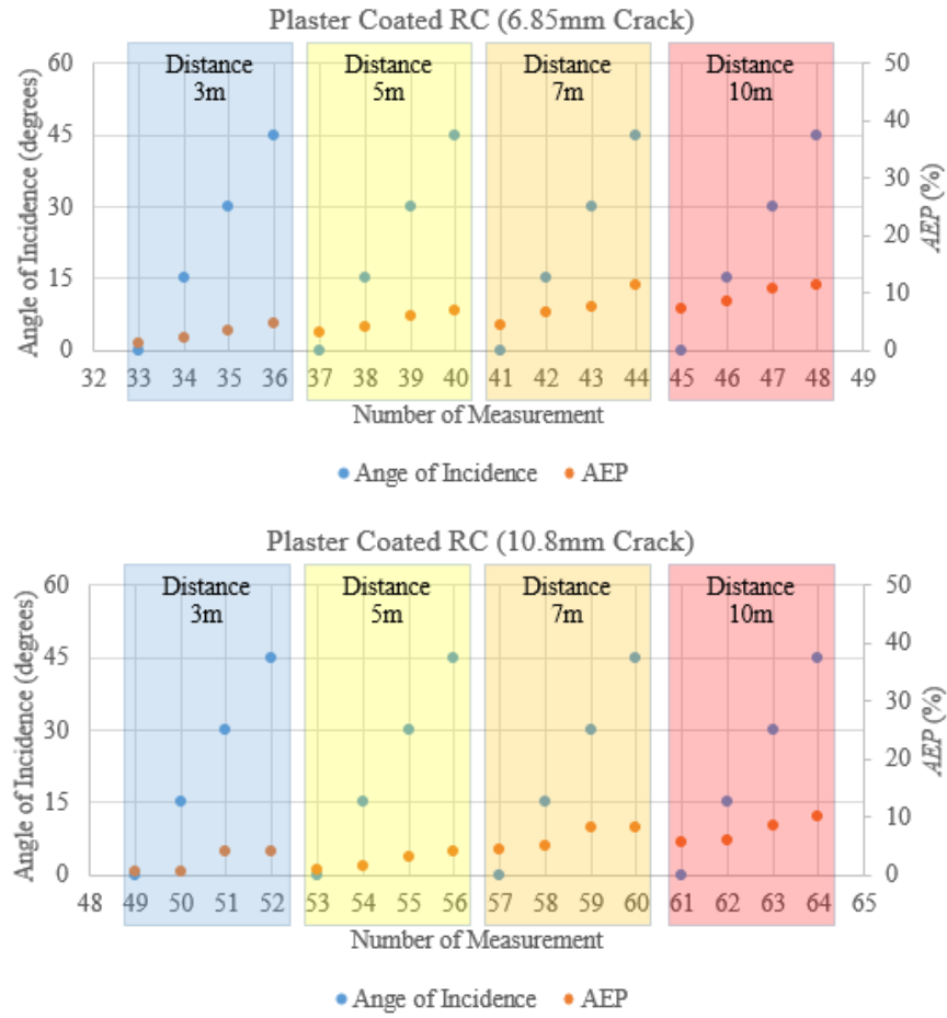
Figure 5.18. Dispersion of Values for Plaster Coated RC Specimen
