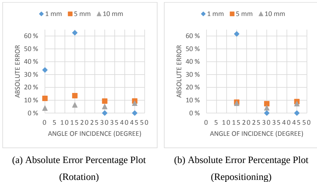
Figure 5.7. AEP Plot for Foam Board Specimen
