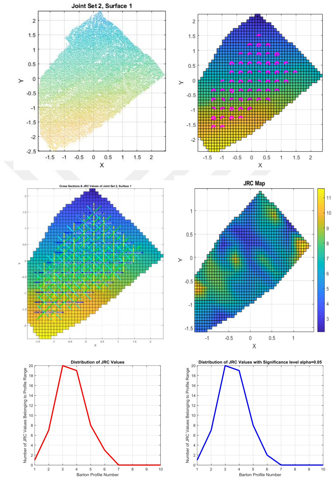
Figure 8.9. JRC estimation process of Joint Set 2, Surface 1.
