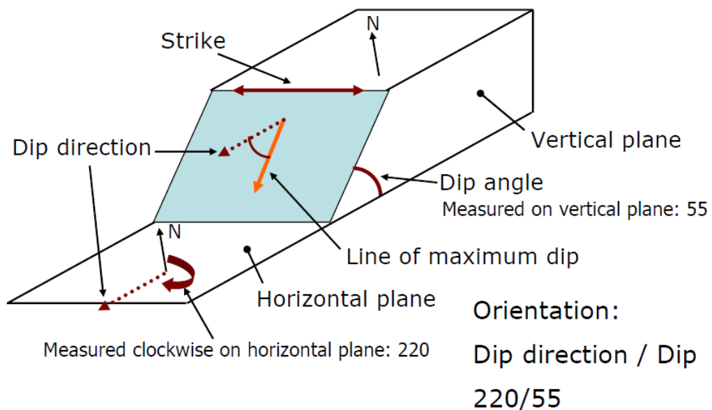
Figure 3.1. Plane orientation and its defining properties, Zhang (2017).
