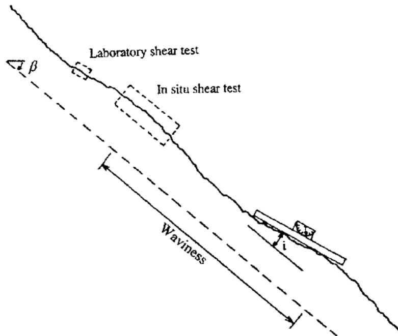
Figure 3.11. Different scales of discontinuity roughness are sampled by different scales of tests. The waviness can be characterized by the angle i , ISRM (1978c).
