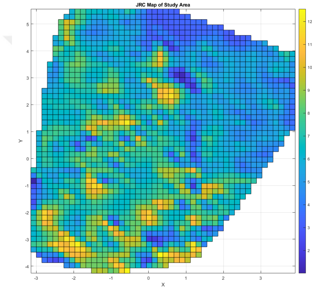
Figure 8.5. JRC map of Joint Set 1 Surface 1.
