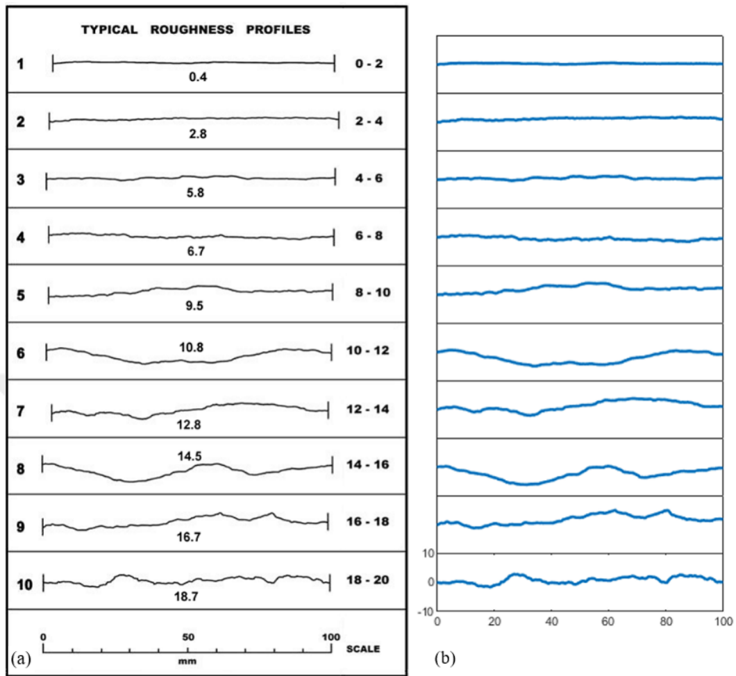
Figure 6.1. Reference profiles from Barton and Choubey (1977) (a) and their digitized plots (b).
