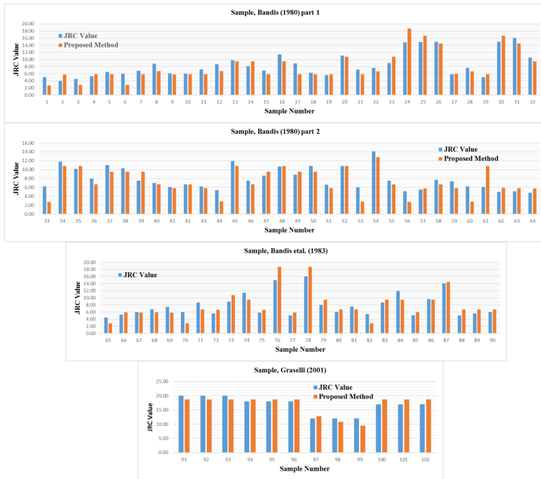
Figure 6.6. Comparison of back-calculated and estimated JRC values.
