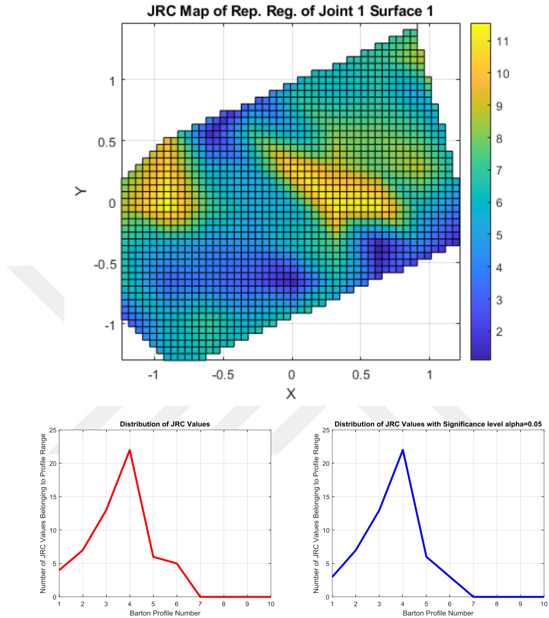
Figure 8.12. JRC map and value distribution of Joint Set 1, Surface 1.
