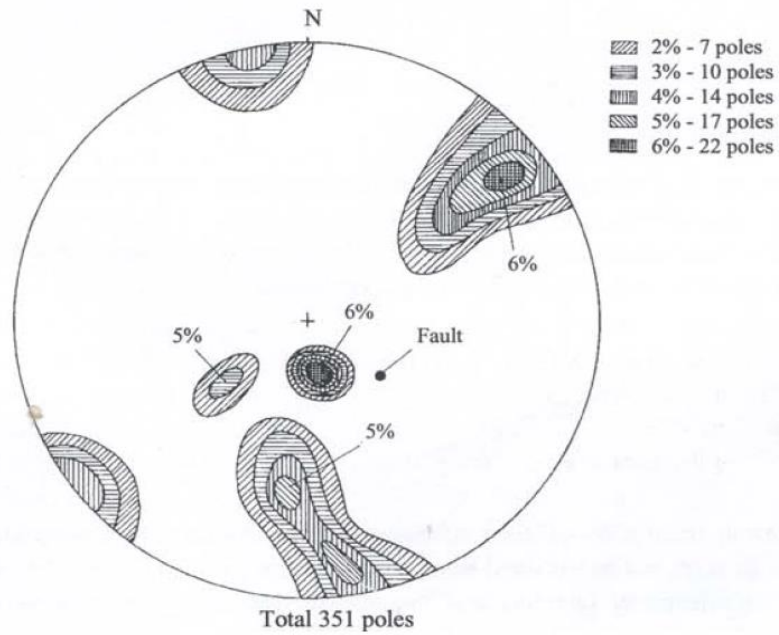
Figure 3.5. Contours of pole concentrations for the data plotted in Fig. 3.3., Hoek and Brown (1980a).
