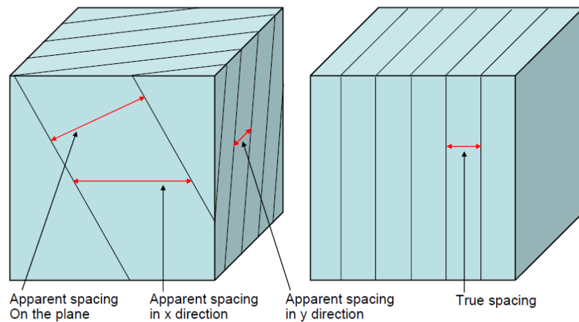
Figure 3.6. Joint spacing, apparent spacing, and true spacing, Zhang (2017).
