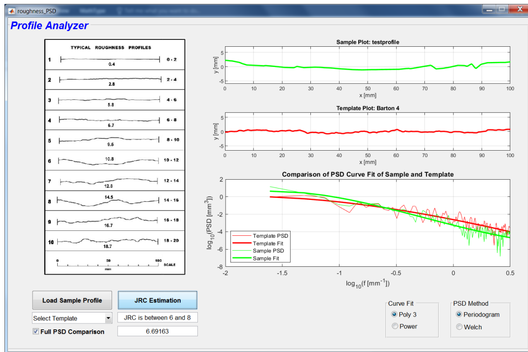
Figure 7.18. Sample profile obtained from the Surface Roughness section.
