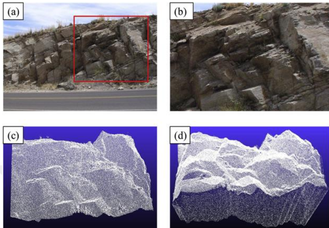
Figure 3.14. Three-dimensional presentation of a discontinuity surface. (Chen et. al., 2017)
