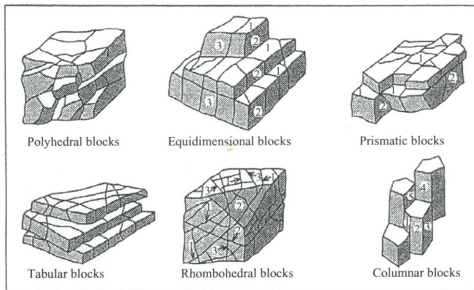
Figure 3.10. Examples of block shapes, Dearman (1991).
