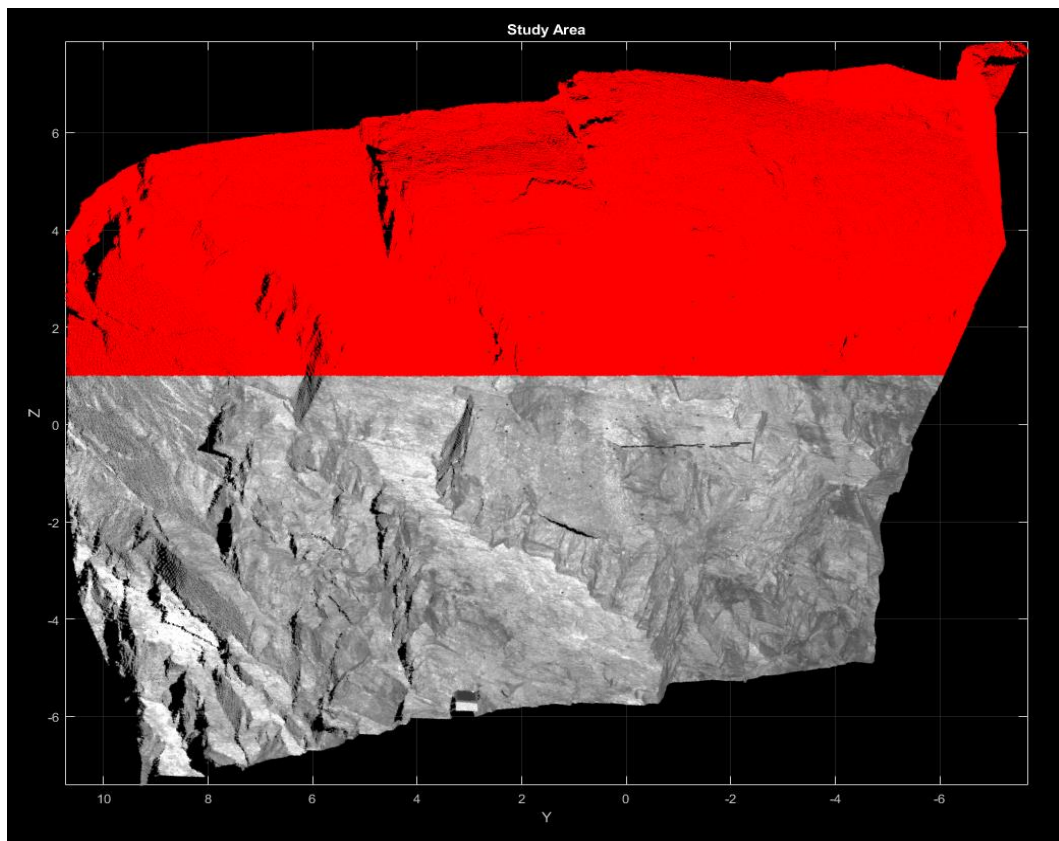
Figure 8.1. Region (red) was selected for JRC estimation.
