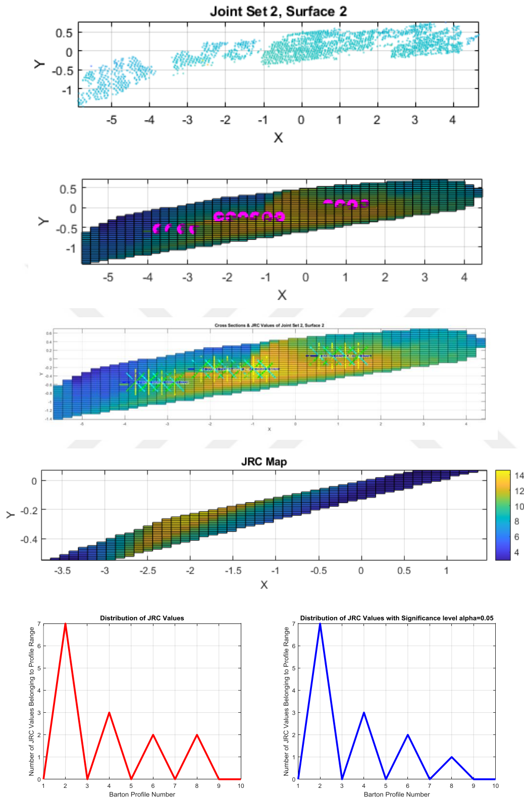
Figure 8.10. JRC estimation process of Joint Set 2, Surface 2.
