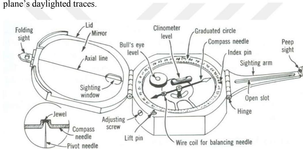
Figure 3.2. The standard Brunton compass and its most essential parts. (University at Buffalo, 2020)
