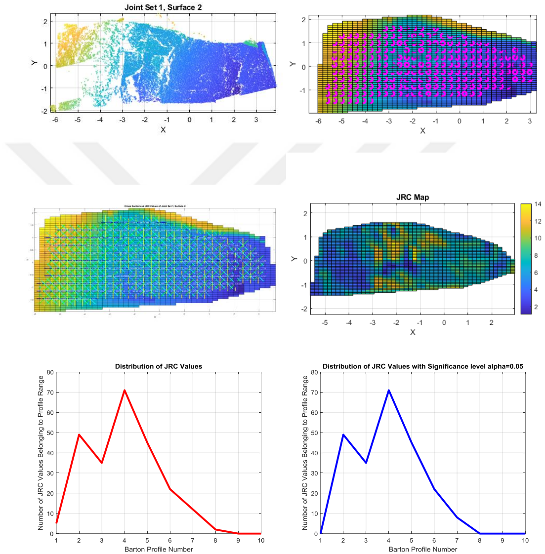
Figure 8.7. JRC estimation process of Joint Set 1, Surface 2.
