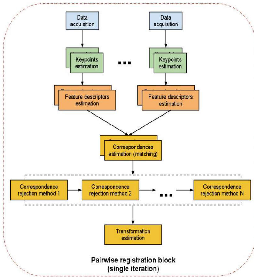
Figure 4.6. Process chart of point cloud registration (PCL, 2016).
