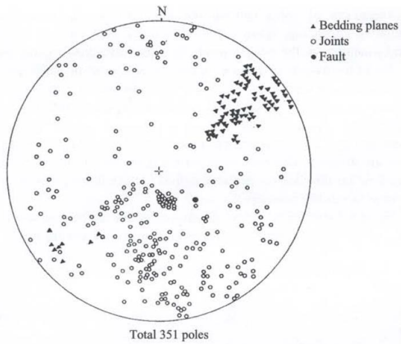
Figure 3.4. The plot of poles of 351 discontinuities, Hoek and Brown (1980a).
