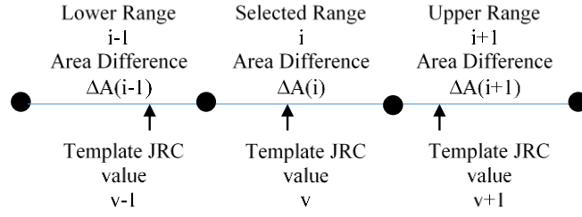
Figure 6.5. Interpolation structure.
