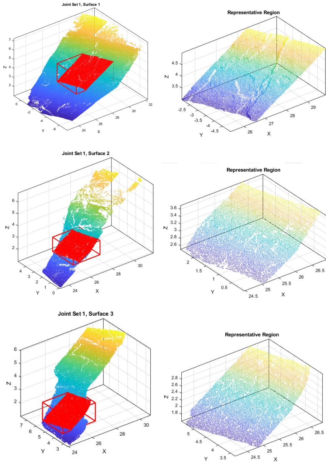
Figure 8.11. Representative regions selected from the three surfaces of the first joint set.
