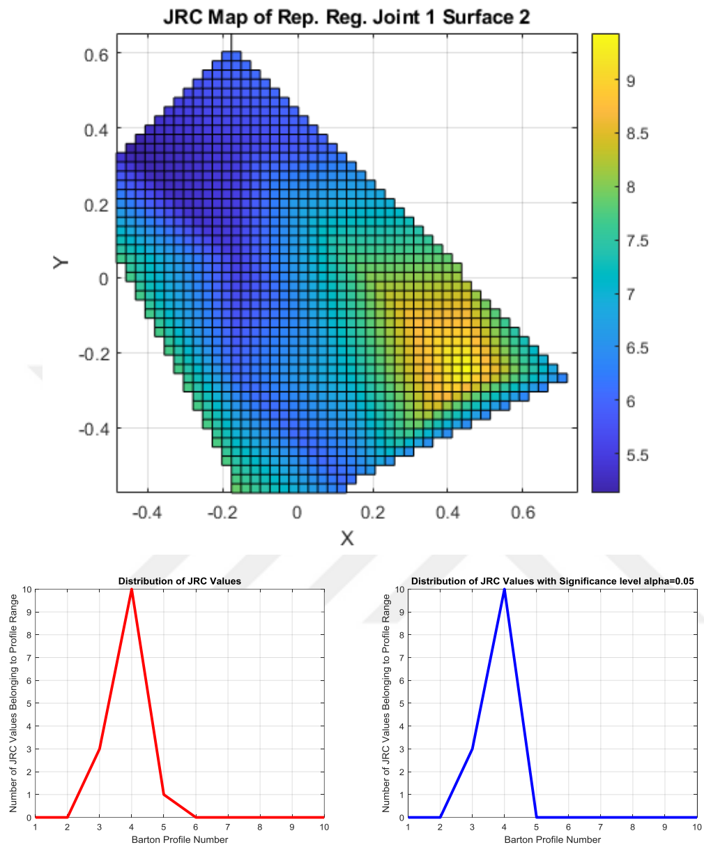
Figure 8.13. JRC map and value distribution of Joint Set 1, Surface 2.
