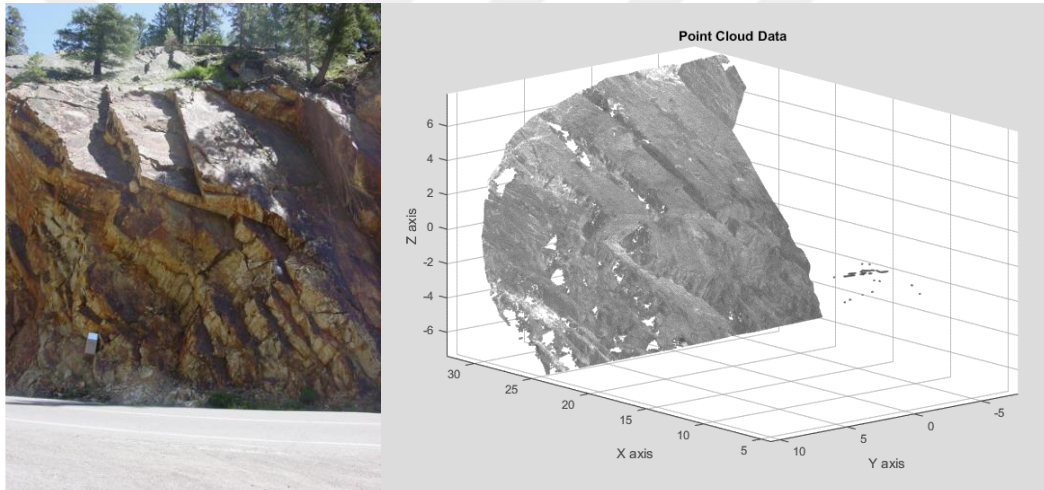
Figure 7.2. Point Cloud data used for Matlab case study and its photograph, Riquelme et al. (2014).
