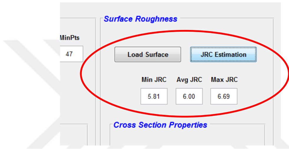
Figure 7.16. Result of JRC estimation for six cross-sections.
