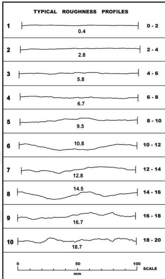
Figure 3.13. Template JRC profiles, Barton and Choubey (1977).
