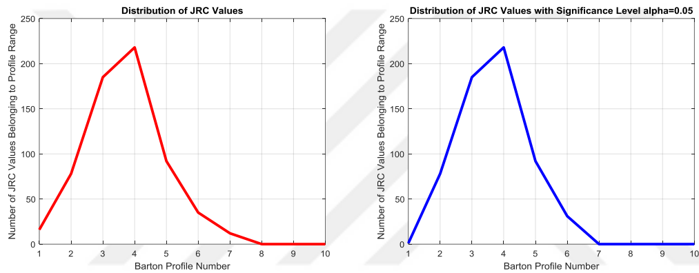
Figure 8.6. Distribution of JRC values of study area according to reference profiles of Barton and Choubey (1977) and same data for significance level \alpha=0.05 .
