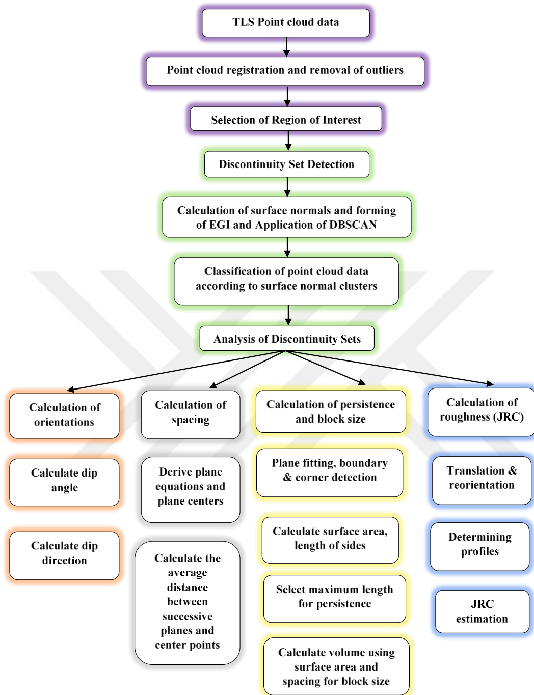
Figure 1.3. Block diagram of the main body of the study.
