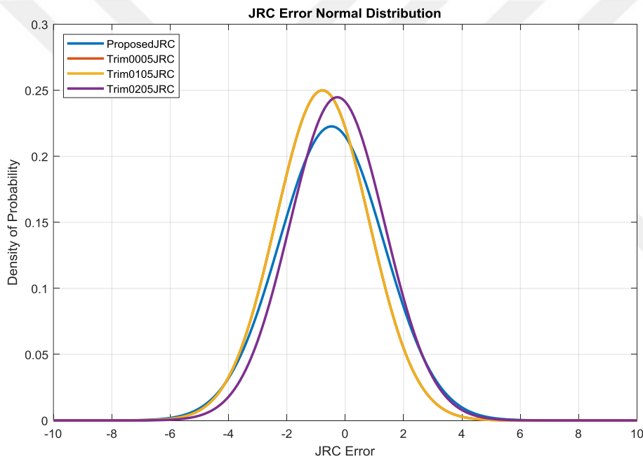
Figure 6.10. Normal probability density distribution of estimation errors for the proposed method and trimmed PSD plots 5% at low frequency and 0%, 1%, and 2% at high frequency ends. Red and yellow plots overlap.
