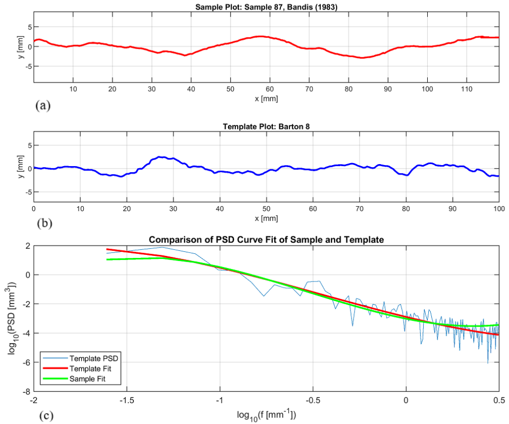
Figure 6.3. Sample (a) and template (b) profiles and polynomial fit superimposed on the template PSD (c).
