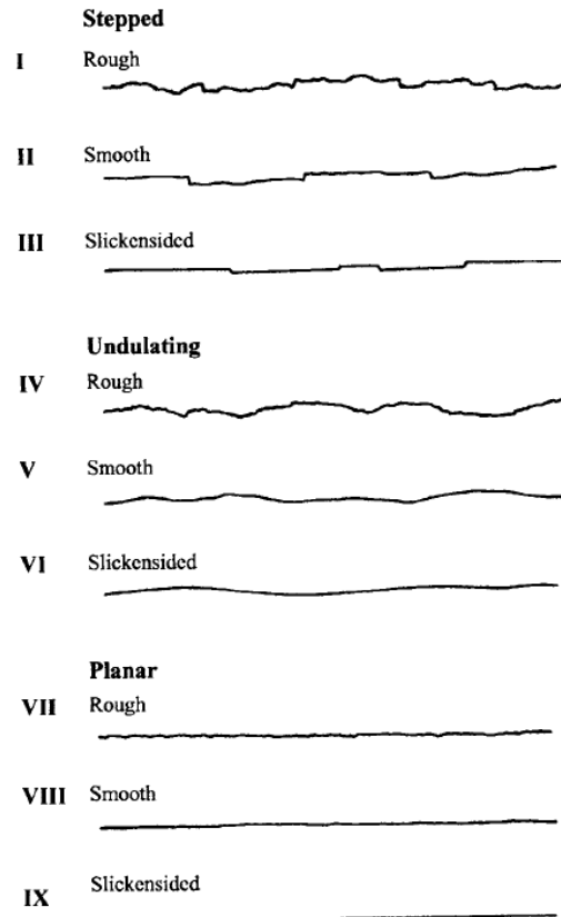
Figure 3.12. Typical roughness profiles and suggested nomenclature. The length of each profile is in the range of 1 to 10 meters. The vertical and horizontal scales are equal, ISRM (1978c).
