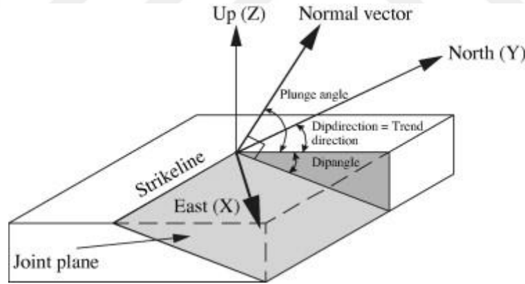
Figure 3.3. The relation between dip direction, trend direction, dip angle, and plunge angle. (Ge et. al., 2014)
