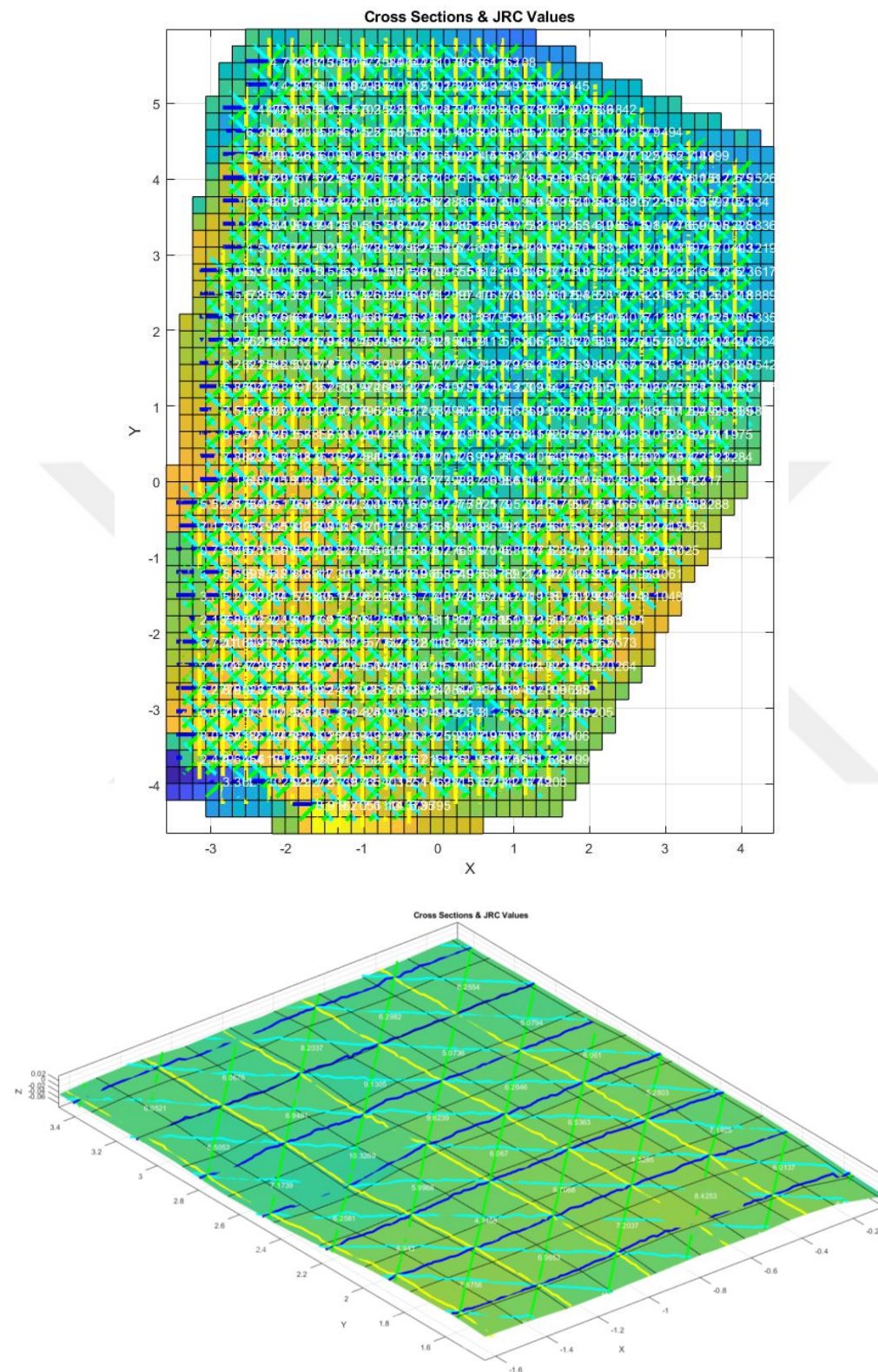
Figure 8.4. JRC estimation areas of the whole study area and a close-up of a section.
