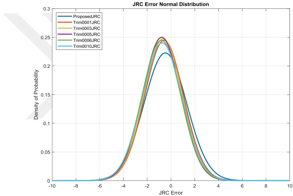
Figure 6.9. Normal probability density distribution of estimation errors for the proposed method and trimmed PSD plots of low frequency (1%, 3%, 5%, 6%, and 10%).
