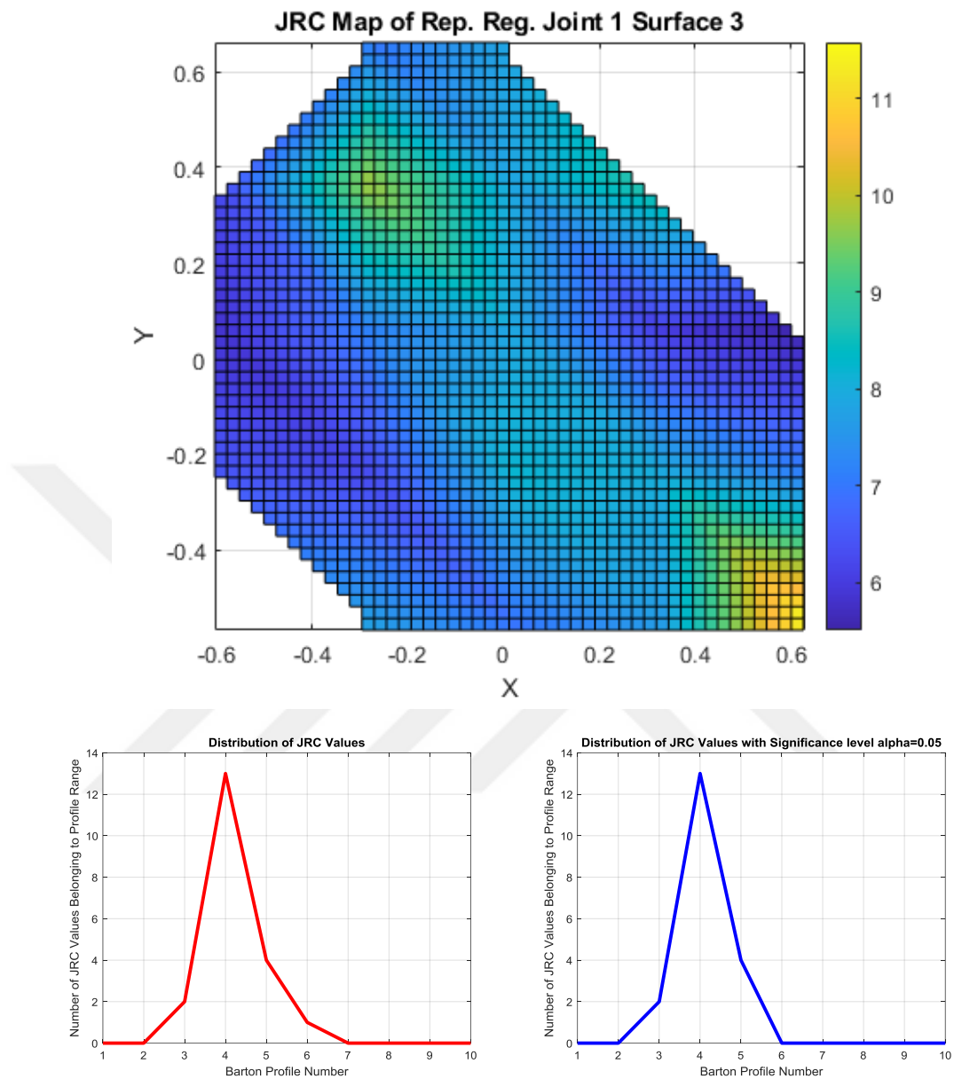
Figure 8.14. JRC map and value distribution of Joint Set 1, Surface 3.
