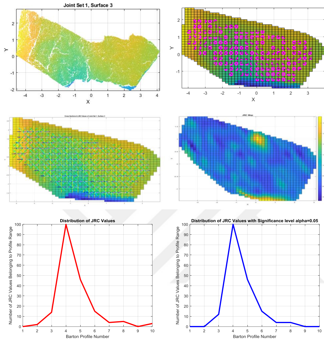
Figure 8.8. JRC estimation process of Joint Set 1, Surface 3.
