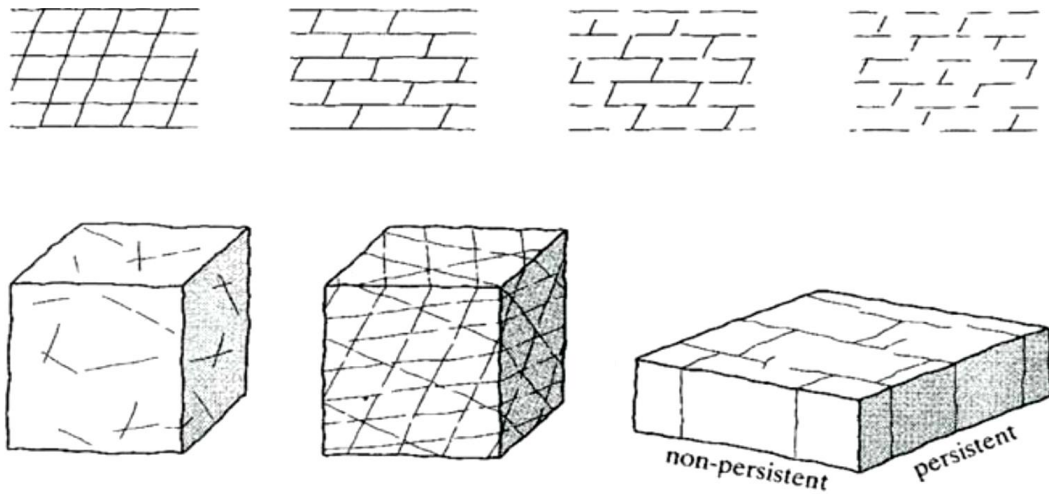
Figure 3.7. Sketches and block diagrams displaying persistence of various sets of discontinuities, ISRM (1978c).
