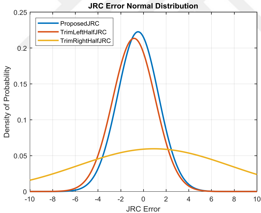
Figure 6.8. Normal probability density distribution of estimation errors for the proposed method (blue) and trimmed PSD plots of high frequency (red) and low frequency (yellow).
