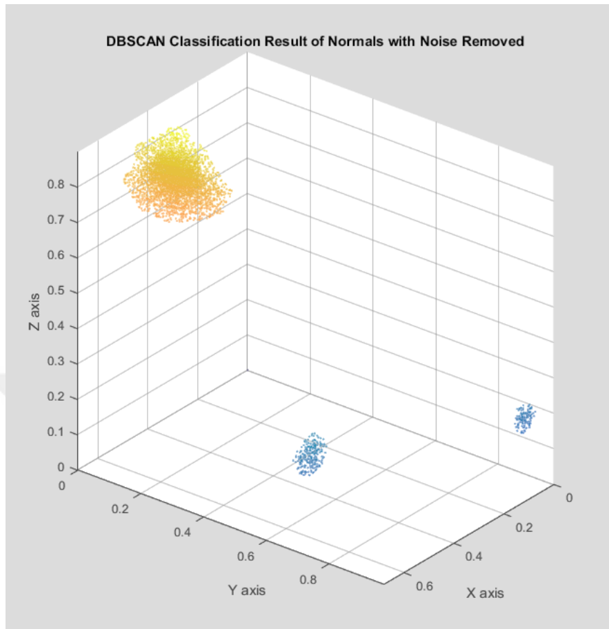
Figure 5.8. DBSCAN clustering result after the noise cluster was removed.
