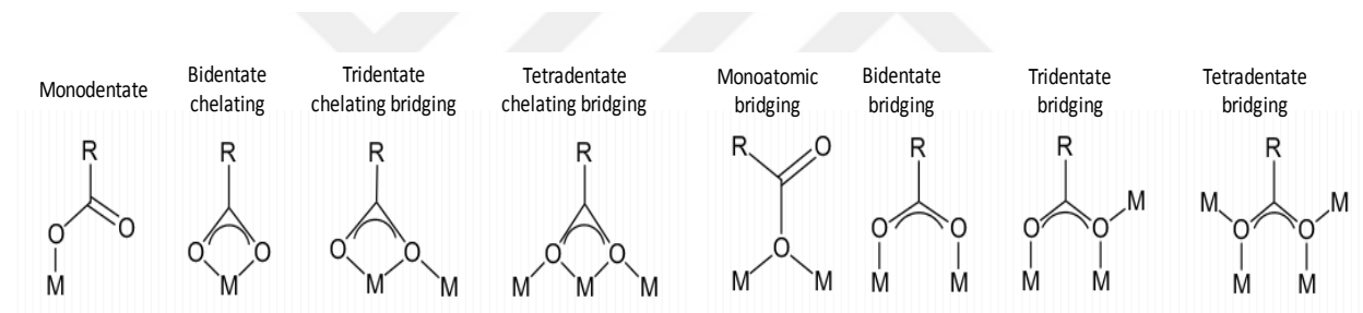
Figure 8. Possible ways of adsorption of an adsorbate onto a metal surface with various geometries [35].
