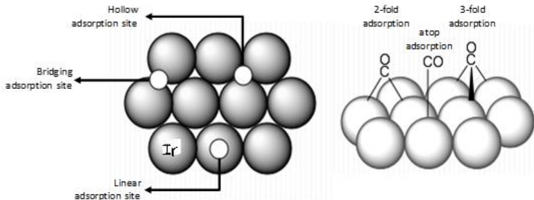
Figure 7. Typical adsorption geometries of CO on a face-centered-cubic (FCC) (111) surface (e.g. Pt(111), Pd(111), Ir(111) etc.) [12].
