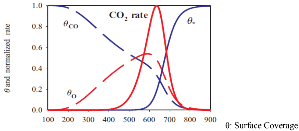
Figure 10. Surface coverage of CO ( \theta_{CO} ) and O ( \theta_O ) species and the CO 2 formation rate as a function of temperature in a typical CO oxidation reaction following Langmuir-Hinshelwood kinetics [32].
