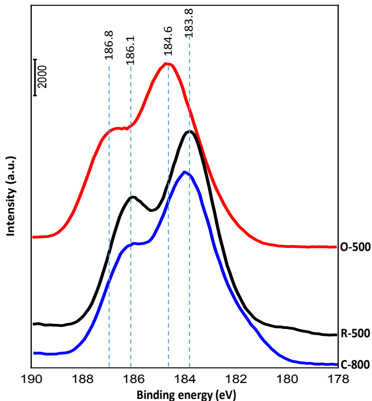
Figure 63. Zr3d XPS spectra for 1 wt% IrCl 3 -CeO 2 (IWI) samples. R-500: Reduced in H 2 at 500 °C, O-500: Oxidized in O 2 at 500 °C, C-800: Calcined in air at 800 °C.
