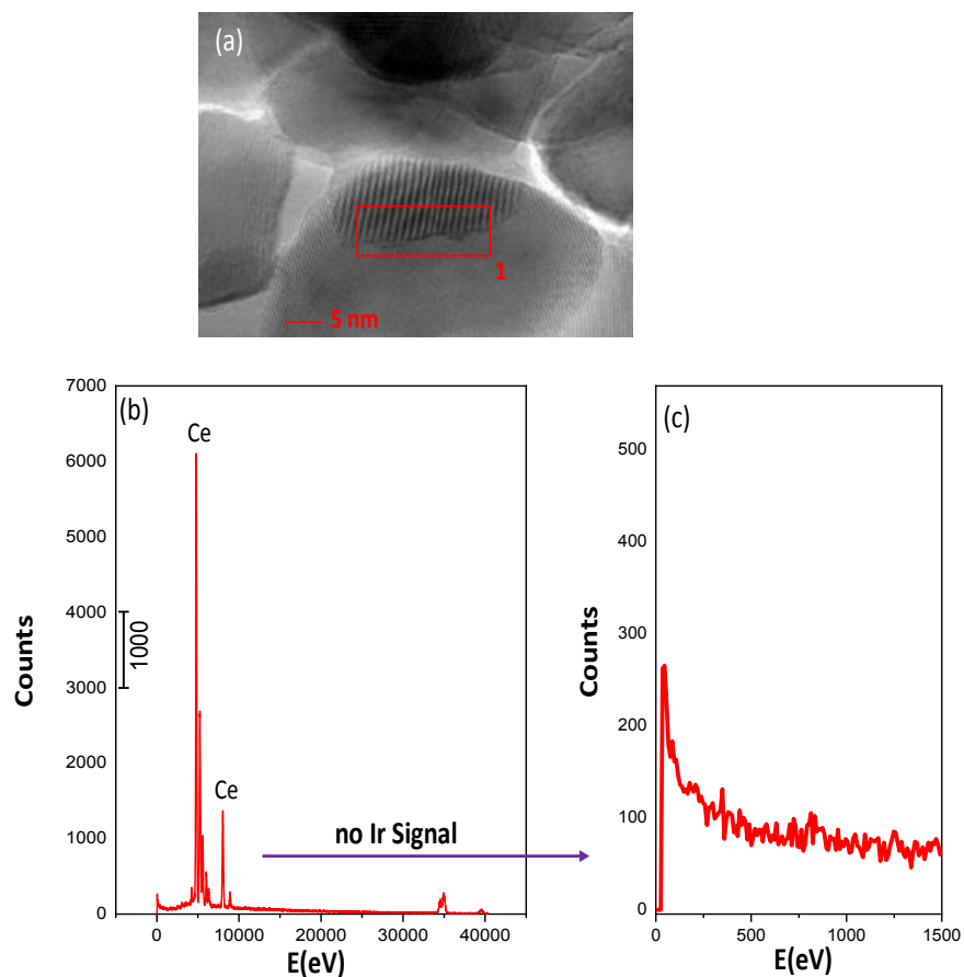
Figure 39. HAADF-TEM image (a) and TEM-EDX spectra (b and c) collected from specified point of 1 wt% \text{IrCl}_3\text{-CeO}_2 annealed in \text{O}_2 .
