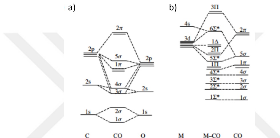
Figure 9. Molecular orbitals of (a) gas phase (free) CO and (b) linear M-CO adsorption system [14].
