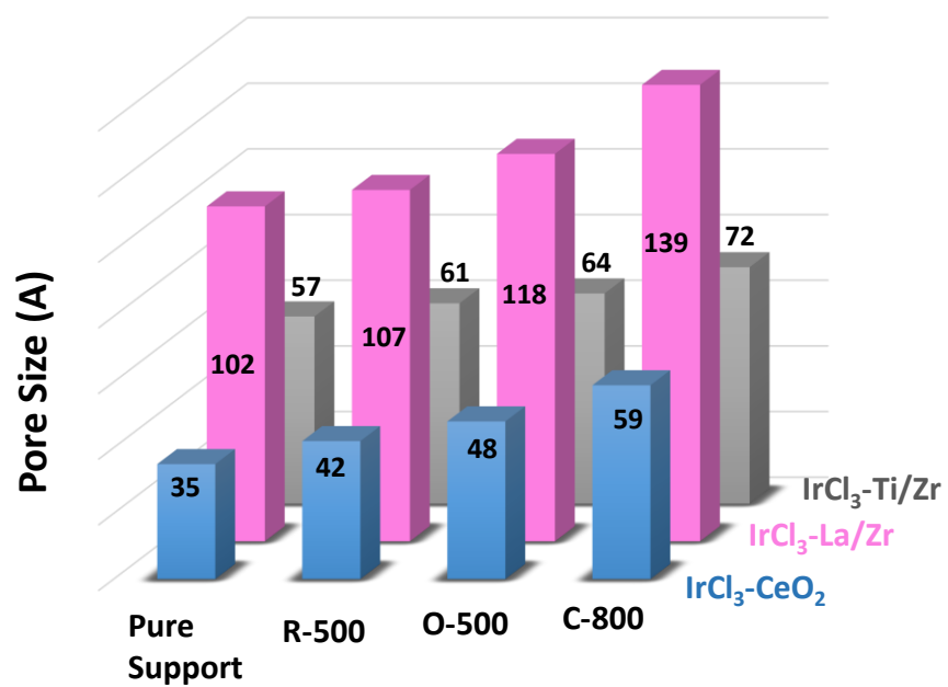
Figure 68. Average pore size of three different family of samples (1 wt%-IWI) under different treatment conditions. R-500: Reduced in H 2 at 500 °C, O-500: Oxidized in O 2 at 500 °C, C-800: Calcined in air at 800 °C.
