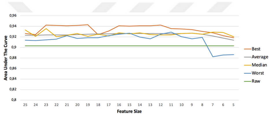
Figure 5.2.3.5 The AUC of LDA classifiers when different numbers of features are used on Z-Alizadehsani data set
