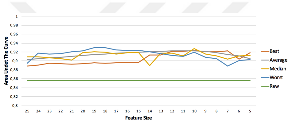
Figure 5.2.4.5 The AUC of NB classifiers when different numbers of features are used on Z-Alizadehsani data set
