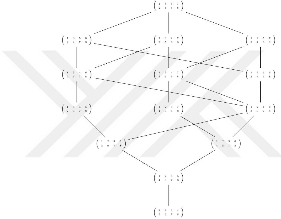
Figure 5.1: Hasse diagram of \mathbf{DP}(8)
