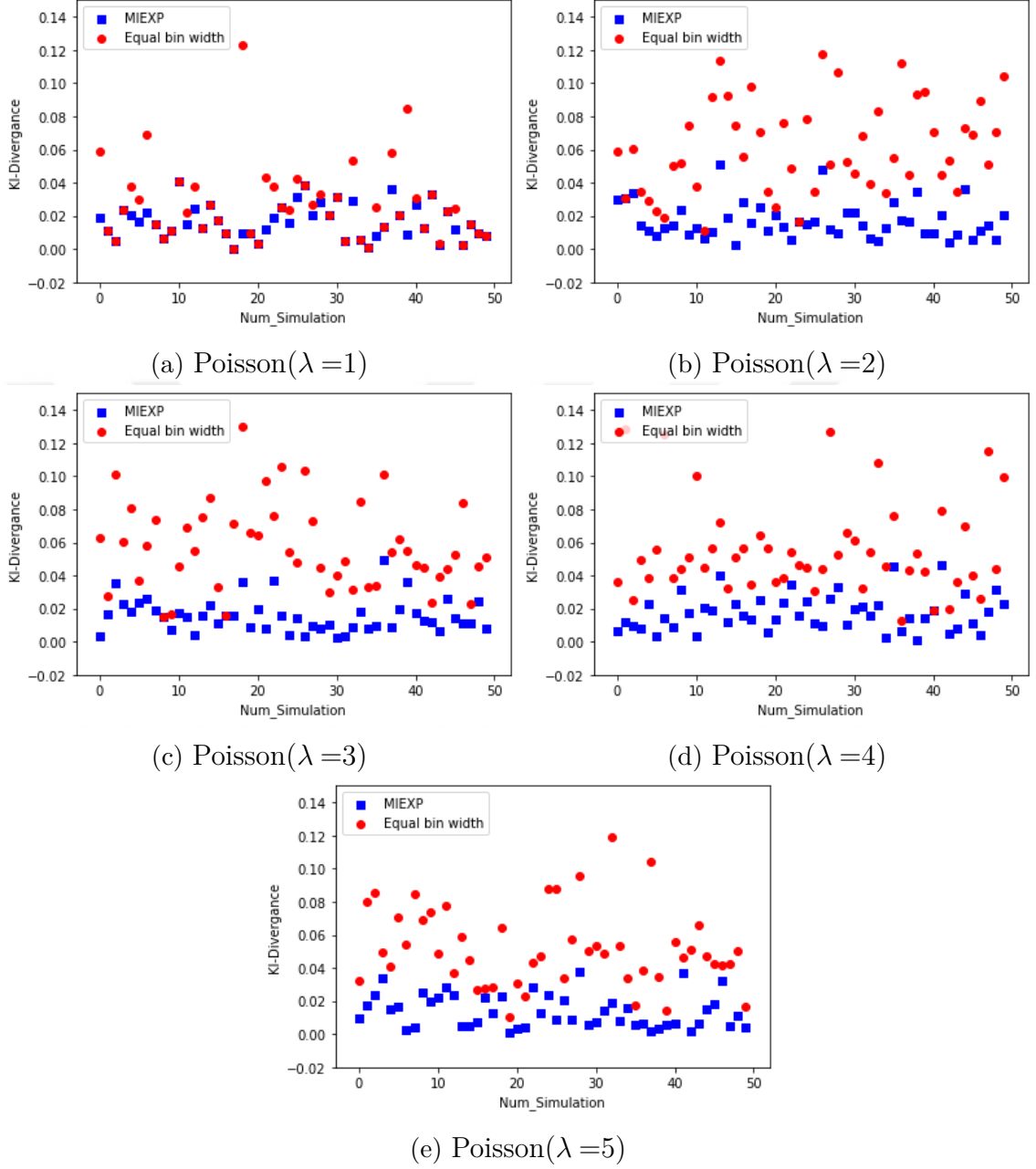
Figure 3.12 KL-divergence of MIEXP method and Equal bin widths for Poisson distributions.
