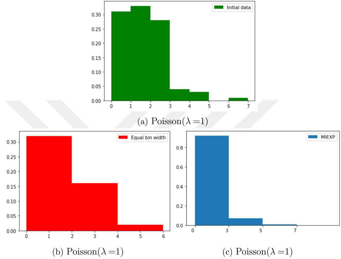
Figure 3.13 Histograms of initial data, MIEXP model, and Equal bin widths for the 18th simulation of \text{Poisson}(\lambda=1) .
