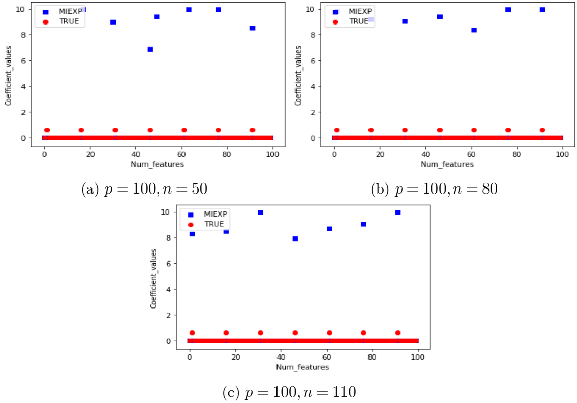
Figure 3.6 Performance of the model in terms of selecting the true coefficients for Scenario 3.
