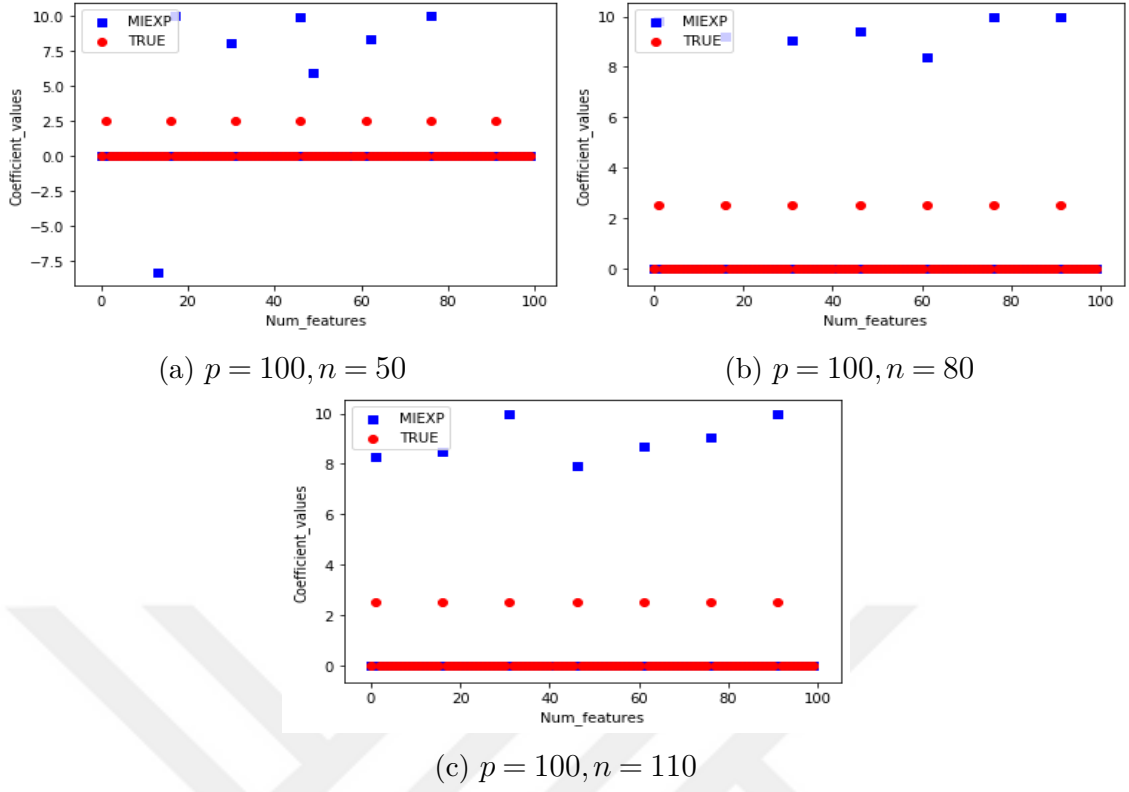
Figure 3.5 Performance of the model in terms of selecting the true coefficients for Scenario 2.
