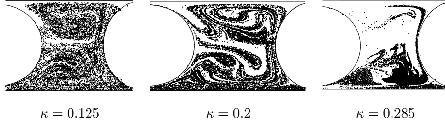
Figure 4.17: The mixing patterns at the exit of the channel as a function of the nondimensional corrugation wavelength of the channel, \kappa . ( Ca = 0.005 , Re = 0.64 , \lambda = 0.014 , \Lambda = 2.0 , \eta = 0.75 , r = 0.1 , Grid: 1728 \times 64 .)
