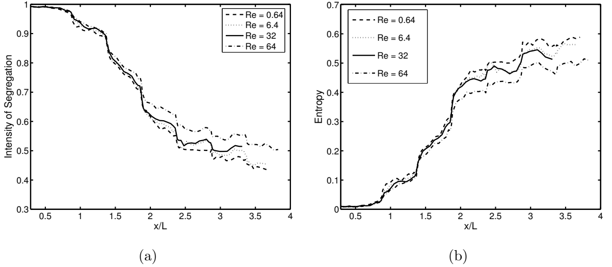
Figure 4.12: Effect of the Reynolds number on mixing. (a) Intensity of segregation (b) Entropy. ( Ca = 0.005 , \lambda = 0.014 , \Lambda = 2.0 , \eta = 0.75 , \kappa = 0.125 , r = 0.1 , Grid: 1728 \times 64 .)
