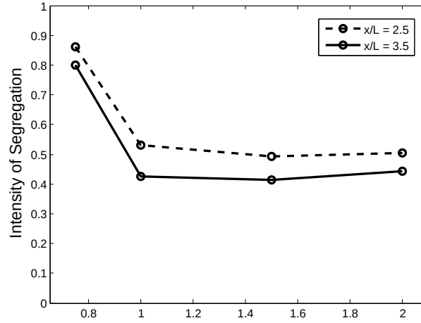
Figure 4.7: The intensity of segregation against the nondimensional bubble size at times when slug centroid, x/L = 2.5 and x/L = 3.5 . The mixing is essentially independent of the bubble size when \Lambda \geq 1 . ( Ca = 0.005 , Re = 0.64 , \lambda = 0.014 , \eta = 0.75 , \kappa = 0.125 , r = 0.1 , Grid: 1728 \times 64 .)
