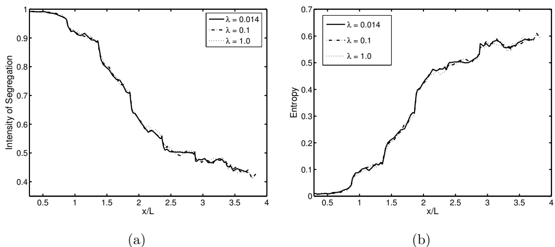
Figure 4.9: Effect of the viscosity ratio on mixing. (a) Intensity of segregation (b) Entropy. ( Ca = 0.005 , Re = 0.64 , \Lambda = 2.0 , \eta = 0.75 , \kappa = 0.125 , r = 0.1 , Grid: 1728 \times 64 .)
