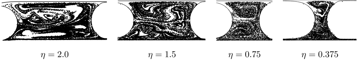
Figure 4.14: The mixing patterns at the exit of the channel as a function of the initial distance between bubbles. ( Ca = 0.005 , Re = 0.64 , \lambda = 0.014 , \Lambda = 2.0 , \kappa = 0.125 , r = 0.1 , Grid: 1728 \times 64 .)
