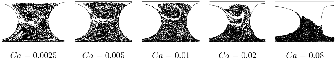
Figure 4.2: Effects of capillary number ( Ca ) on mixing. The mixing patterns at the exit of the channel. ( Re = 0.64 , \lambda = 0.014 , \Lambda = 2.0 , \eta = 0.75 , \kappa = 0.125 , r = 0.1 , Grid: 1728 \times 64 .)
