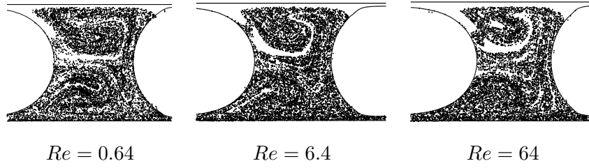
Figure 4.11: Effects of Reynolds number on mixing. The mixing patterns at the exit of the channel for Re = 0.64, 6.4 and 64 . ( Ca = 0.005 , \lambda = 0.014 , \Lambda = 2.0 , \eta = 0.75 , \kappa = 0.125 , r = 0.1 , Grid: 1728 \times 64 .)
