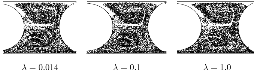
Figure 4.8: Effects of viscosity ratio on the mixing. The mixing patterns at the exit of the channel for \lambda = 0.014, 0.1 and 1 . ( Ca = 0.005 , Re = 0.64 , \Lambda = 2.0 , \eta = 0.75 , \kappa = 0.125 , r = 0.1 , Grid: 1728 \times 64 .)
