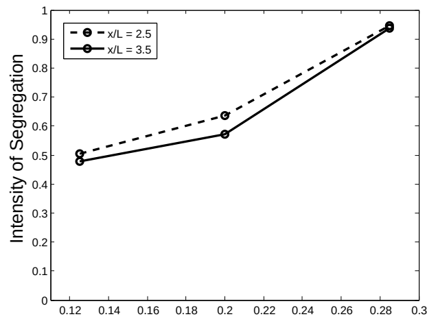
Figure 4.19: The intensity of segregation against the nondimensional channel corrugation wavelength at times when slug centroid, x/L = 2.5 and x/L = 3.5 . The mixing increases as \kappa decreases. ( Ca = 0.005 , Re = 0.64 , \lambda = 0.014 , \Lambda = 2.0 , \eta = 0.75 , r = 0.1 , Grid: 1728 \times 64 .)
