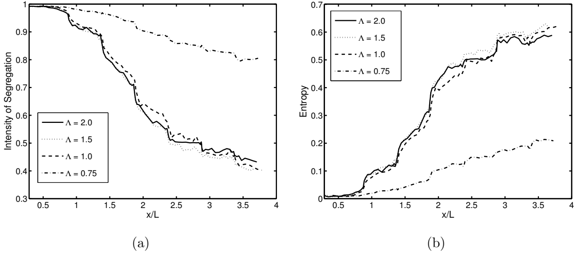
Figure 4.6: Effect of bubble size on mixing. (a) Intensity of segregation (b) Entropy. ( Ca = 0.005 , Re = 0.64 , \lambda = 0.014 , \eta = 0.75 , \kappa = 0.125 , r = 0.1 , Grid: 1728 \times 64 .)
