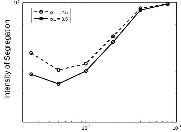
Figure 4.4: The intensity of segregation against the capillary number at times when slug centroid, x/L = 2.5 and x/L = 3.5 . The best mixing occurs at about Ca = 0.005 . ( Re = 0.64 , \lambda = 0.014 , \Lambda = 2.0 , \eta = 0.75 , \kappa = 0.125 , r = 0.1 , Grid: 1728 \times 64 .)
