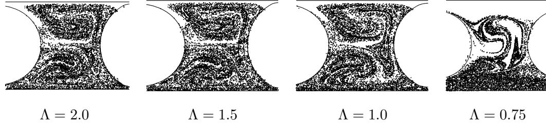
Figure 4.5: Effects of the non-dimensional bubble size on the mixing. The mixing patterns at the exit of the channel for \Lambda = 2.0, 1.5, 1.0 and 0.75 from left to right, respectively. ( Ca = 0.005 , Re = 0.64 , \lambda = 0.014 , \eta = 0.75 , \kappa = 0.125 , r = 0.1 , Grid: 1728 \times 64 .)
