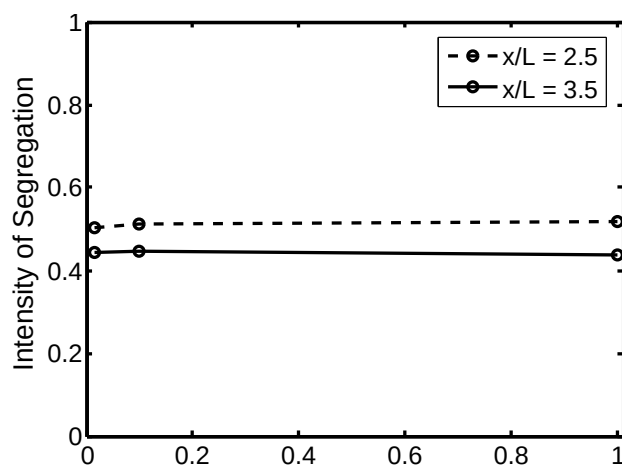
Figure 4.10: The intensity of segregation against the viscosity ratio at times when slug centroid, x/L = 2.5 and x/L = 3.5 . The mixing is nearly independent of the viscosity ratio, \lambda . ( Ca = 0.005 , Re = 0.64 , \Lambda = 2.0 , \eta = 0.75 , \kappa = 0.125 , r = 0.1 , Grid: 1728 \times 64 .)
