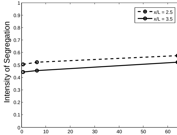
Figure 4.13: The intensity of segregation against the Reynolds Number at times when slug centroid, x/L = 2.5 and x/L = 3.5 . The mixing slightly increases as the Re decreases. ( Ca = 0.005 , \lambda = 0.014 , \Lambda = 2.0 , \eta = 0.75 , \kappa = 0.125 , r = 0.1 , Grid: 1728 \times 64 .)
