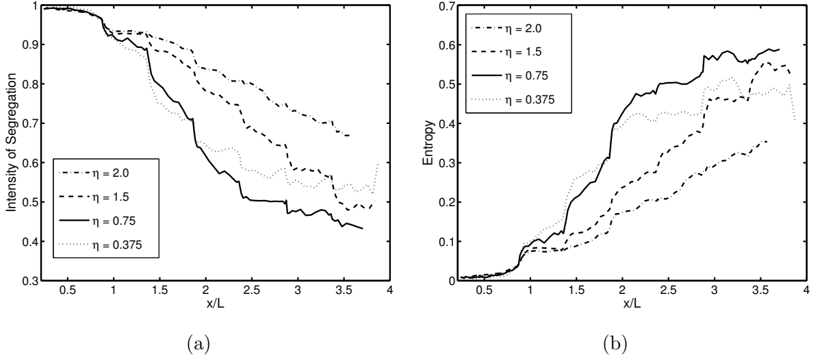
Figure 4.15: Effect of the initial distance between bubbles on mixing. (a) Intensity of segregation (b) Entropy. ( Ca = 0.005 , Re = 0.64 , \lambda = 0.014 , \Lambda = 2.0 , \kappa = 0.125 , r = 0.1 , Grid: 1728 \times 64 .)
