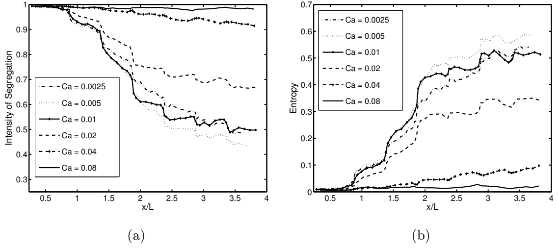
Figure 4.3: Effects of the capillary number on mixing. (a) Intensity of segregation (b) Entropy. ( Re = 0.64 , \lambda = 0.014 , \Lambda = 2.0 , \eta = 0.75 , \kappa = 0.125 , r = 0.1 , Grid: 1728 \times 64 .)
