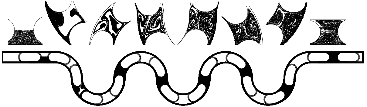
Figure 4.1: Snapshots of mixing patterns for a two-bubble system taken at the nondimensional times from left to right t^* = 0, 5, 11, 16, 21.5, 27, 32.5 and 38.5 , respectively. The top plots are the enlarged versions of the corresponding scatter plots shown in the channel (lower plots). ( Ca = 0.005 , Re = 0.64 , \lambda = 0.014 , \Lambda = 2.0 , \eta = 0.75 , \kappa = 0.125 , r = 0.1 , Grid: 1728 \times 64 .)
