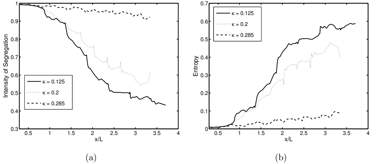
Figure 4.18: Effect of the channel geometry on mixing. (a) Intensity of segregation (b) Entropy. ( Ca = 0.005 , Re = 0.64 , \lambda = 0.014 , \Lambda = 2.0 , \eta = 0.75 , r = 0.1 , Grid: 1728 \times 64 .)
