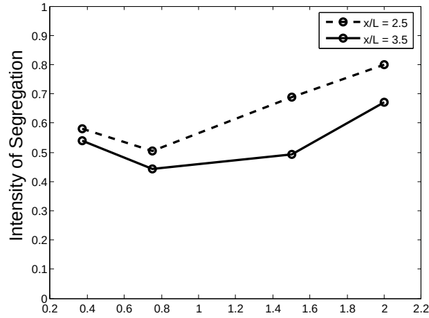
Figure 4.16: The intensity of segregation against the nondimensional distance between bubbles at times when slug centroid, x/L = 2.5 and x/L = 3.5 . The best mixing occurs for the base case, i.e., \eta = 0.75 . ( Ca = 0.005 , Re = 0.64 , \lambda = 0.014 , \Lambda = 2.0 , \kappa = 0.125 , r = 0.1 , Grid: 1728 \times 64 .)
