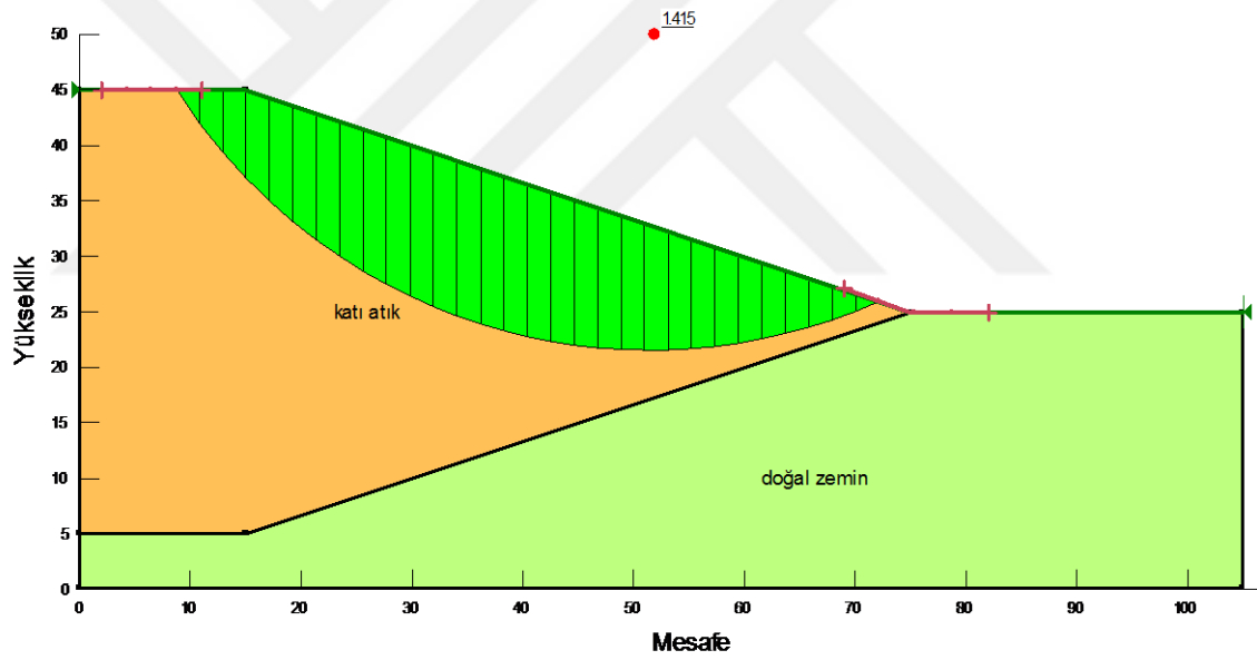
d) Janbu
