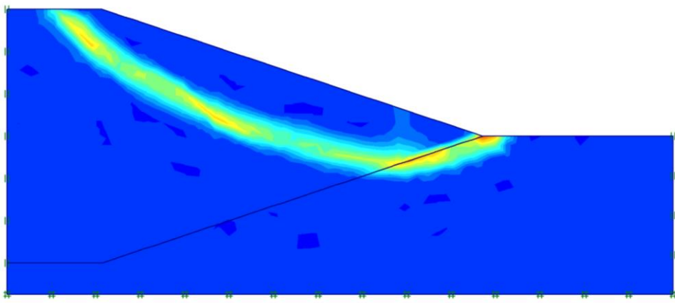
d) \phi=50^\circ
