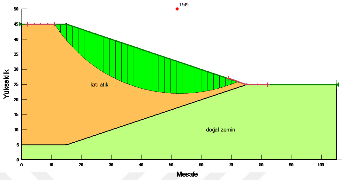
c) Morgenstern-Price
