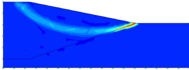
d) \beta=14.04^\circ
