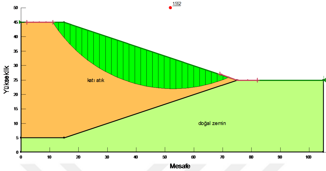
e) Bishop
