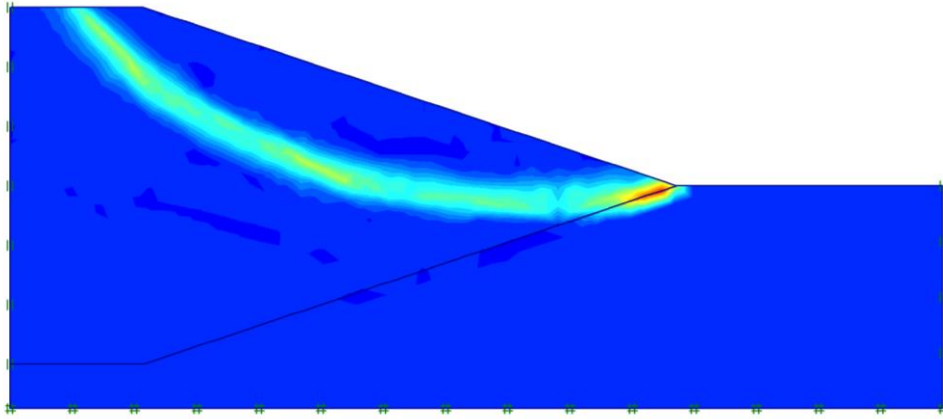
c) \gamma=13 \text{ kN/m}^3
