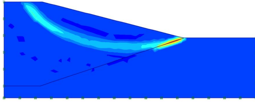
d) \beta=14.04^\circ
