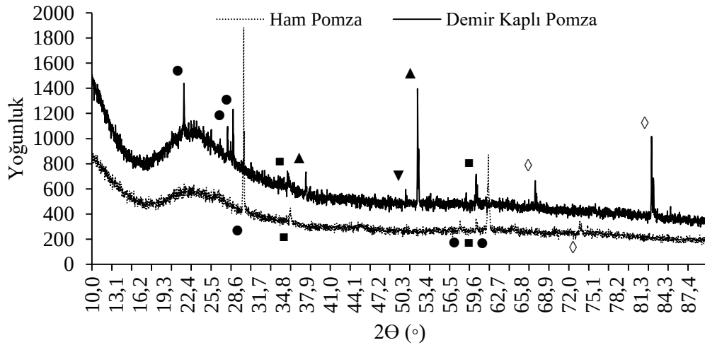
Şekil 4.2: XRD grafiği (•: (\text{Ca}, \text{Na})(\text{Si}, \text{Al})_4\text{O}_8 , ▼: \text{Na}(\text{Si}_3\text{Al})\text{O}_8 , ▲: \alpha\text{-Fe}_2\text{O}_3 , ■: \alpha\text{-FeOOH} , ◇: Fe).
