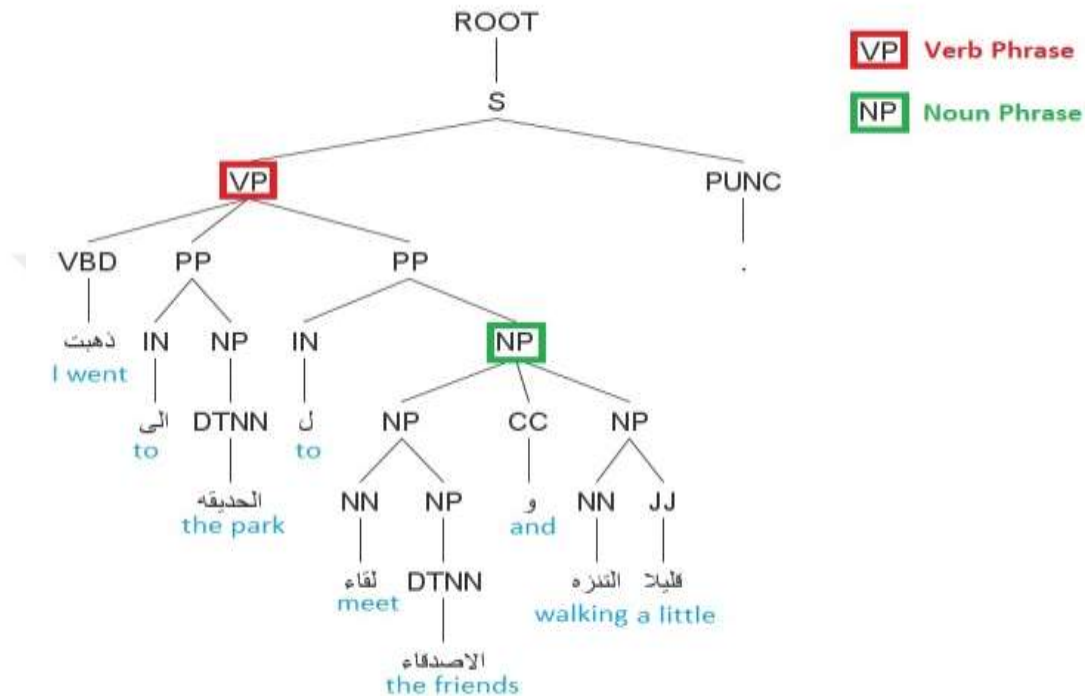
Figure 3.8 An example of Arabic sentence parse tree with PoS tags which generated by using both of Stanford Arabic Parser and Tagger tools
