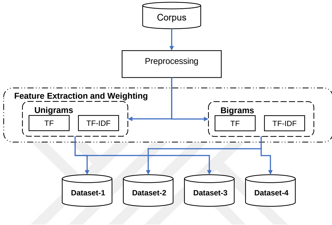
Figure 4.4 Datasets generation process
