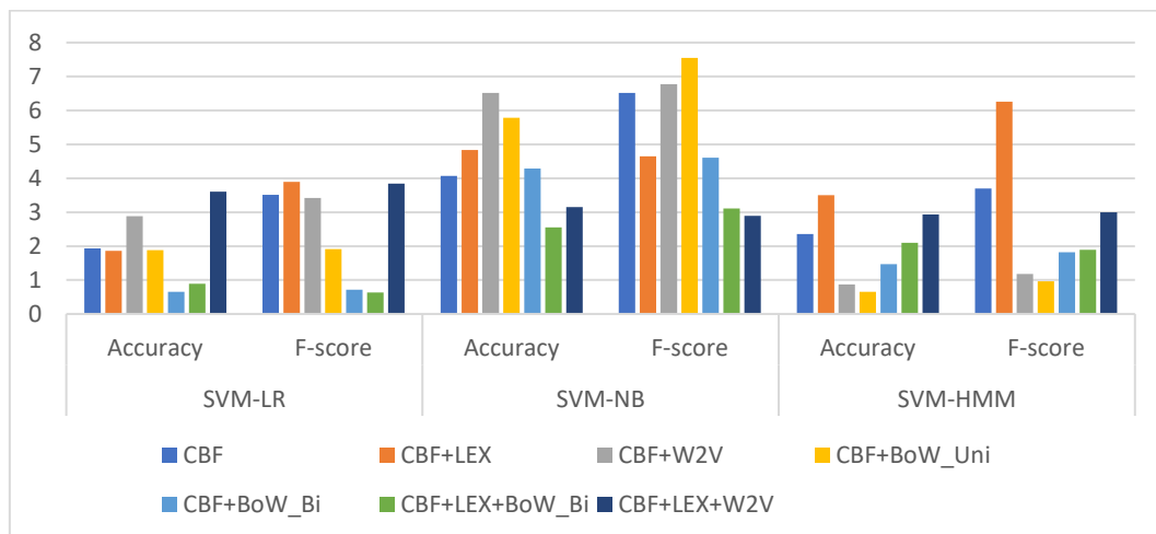
Figure 4.17 The percentage of improvement in the average of classification accuracy and F-score for each combined learner using stacking method for different features combinations
