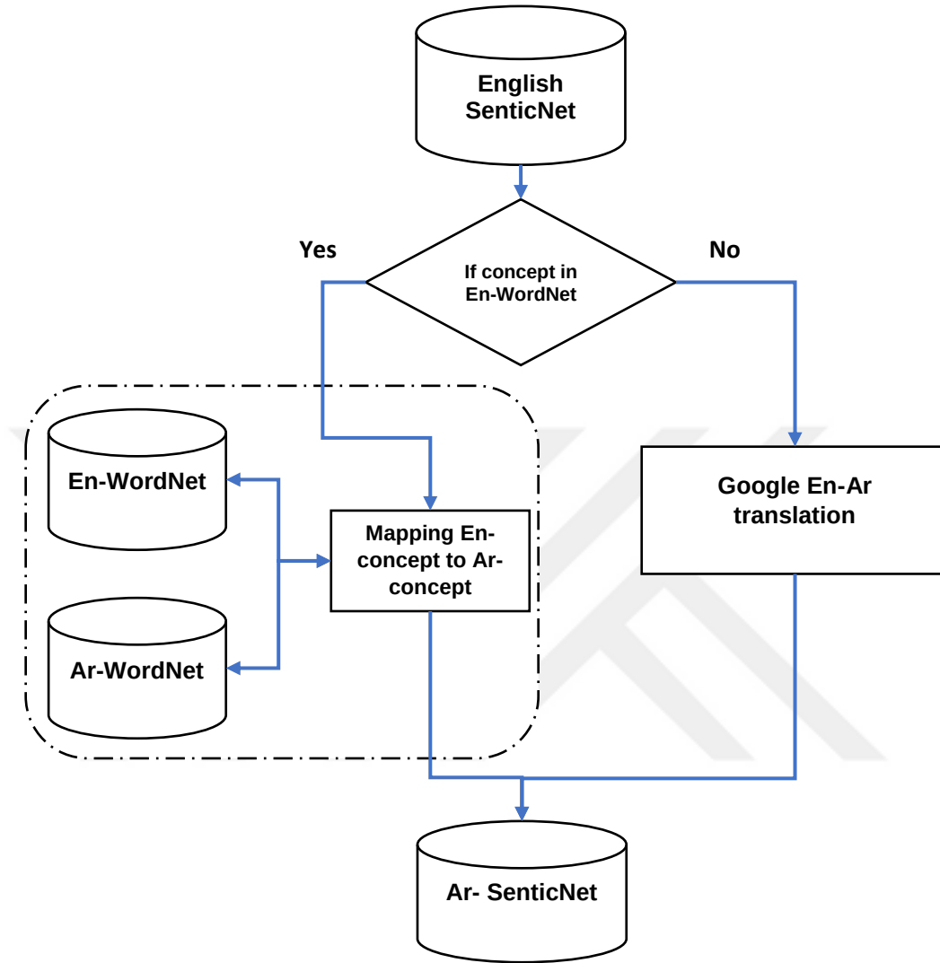
Figure 3.5 The proposed approach for translating English SenticNet to the Arabic language
