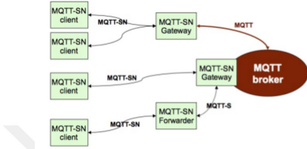
Figure 2.4: MQTT-SN Architecture [5]
