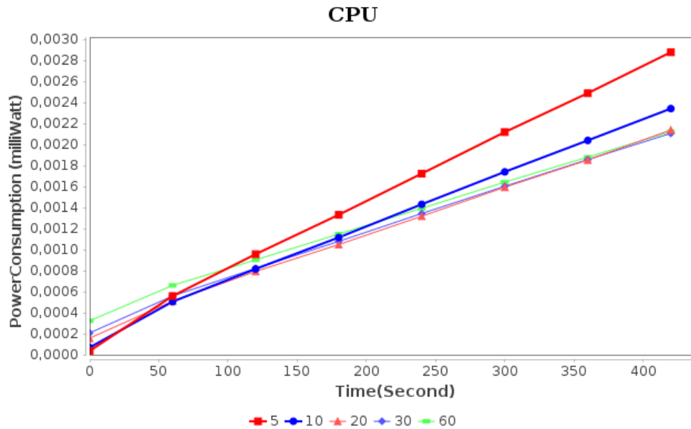
Figure 4.17: The total power consumption in milliwatt in first 450 seconds for CPU
