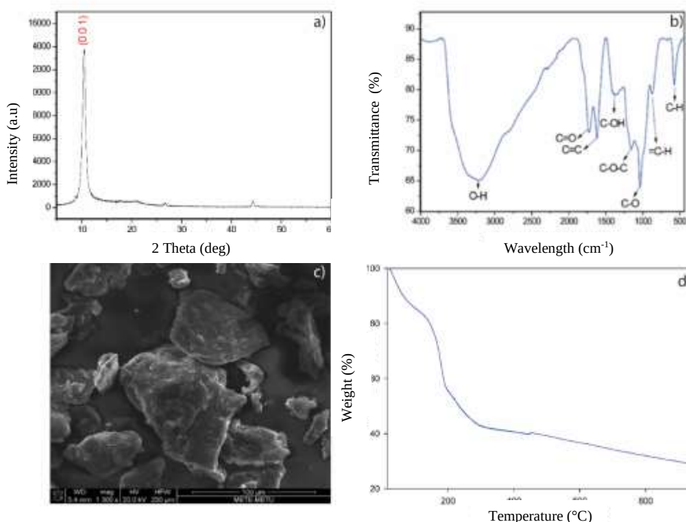
Figure 4.20. a) XRD pattern, b) FTIR spectra, c) Micrograph image and d) TGA analysis of GO synthesized using Tour method.
