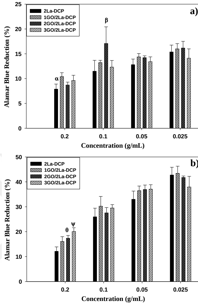
Figure 4.28. Percent Alamar Blue reduction of cells result of indirect cell viability study after a) 1 and b) 4 days of incubation. \alpha : Indicates statistically significant difference between results of 1GO/2La-DPC and 2La-DPC groups ( P < 0.05 ). \beta : Indicates statistically significant difference between results of 2GO/2La-DPC and La-DPC groups ( P < 0.05 ). \theta : Indicates statistically significant difference between results of 2GO/2La-DPC and 2La-DPC groups ( P < 0.05 ). \Psi : Indicates statistically significant difference between results of 3GO/La-DPC and 2La-DPC groups ( P < 0.01 ).
