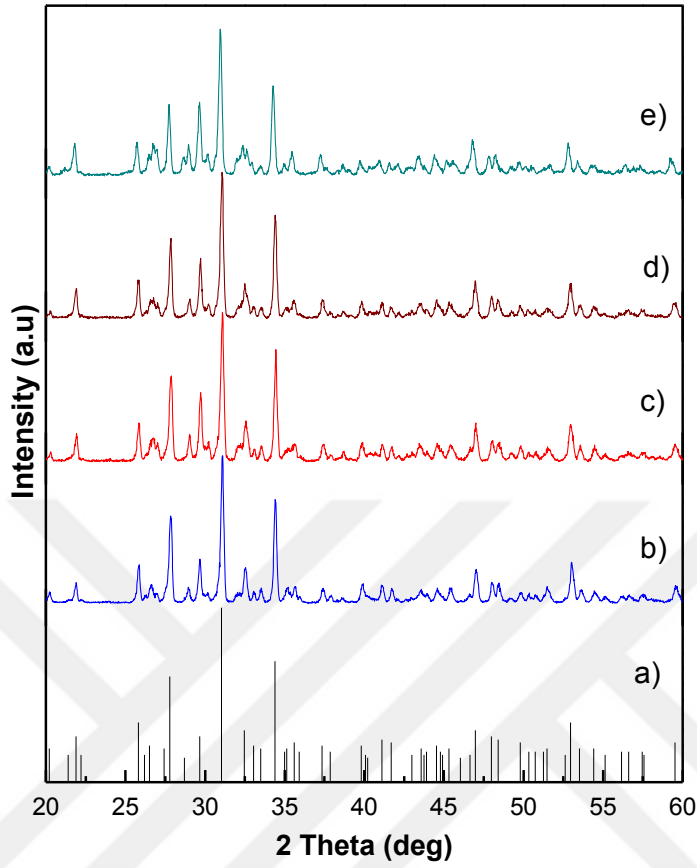
Figure 4.1. XRD patterns of \beta TCP and \text{La}^{3+} doped \beta TCP, calcined at 1000°C for 2 h, a) \beta TCP (JCPDS No: 09-0169), b) \beta TCP, c) 1La- \beta TCP, d) 2La- \beta TCP, e) 3La- \beta TCP.
