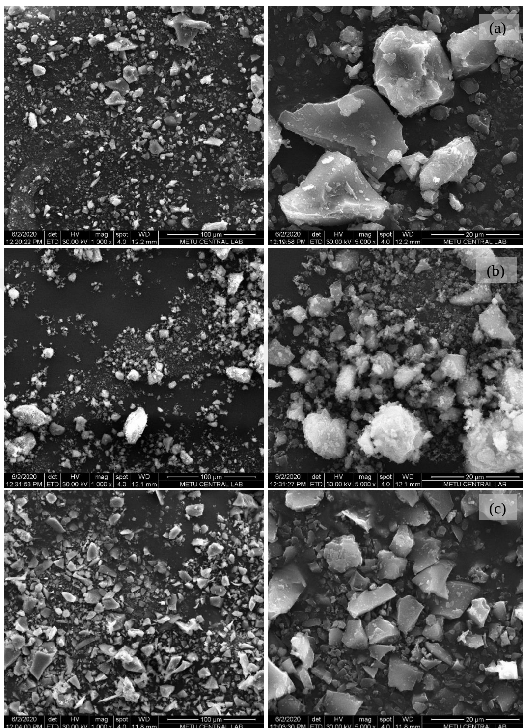
Figure 3.5. Scanning electron microscopy images of glass waste (a), concrete waste (b) and slag (c), (images on left and right side have magnifications of 1000× and 5000× respectively)
