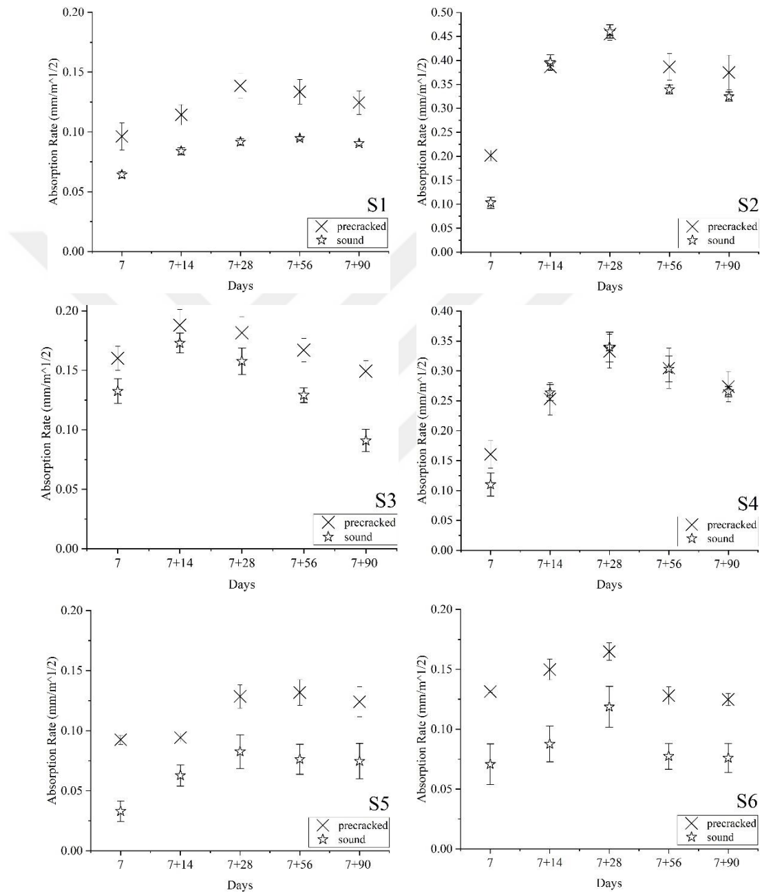
Figure 4.11. Absorption results of EGCs
