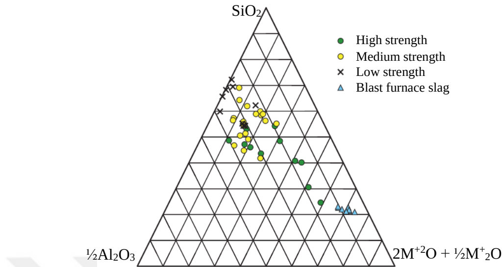
Figure 2.4. Alkali-activated fly-ashes' ternary diagram showing the relationship between compressive strength and chemical content (Provis and Bernal, 2014)
