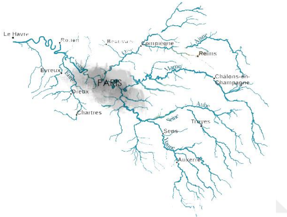
Figure 3.1. The Seine River Basin. Edited by the author (Flipo, Lestel, Labadie, Meybeck, & Garnier, 2021).
