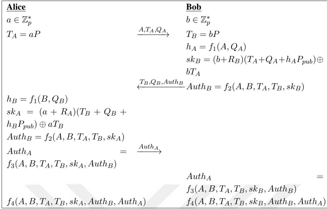
Figure 3.2: Tseng, Huang and You's Protocol
