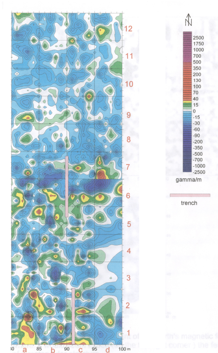
Map.15. High resolution map of vertical gradient
