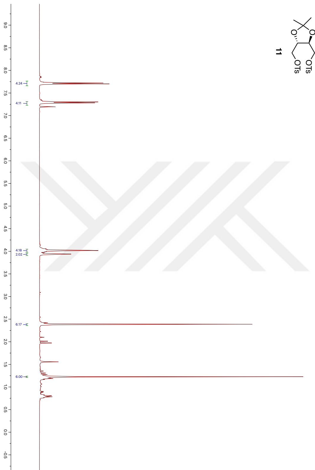
Figure 44. 1 H NMR spectrum of Compound 11
