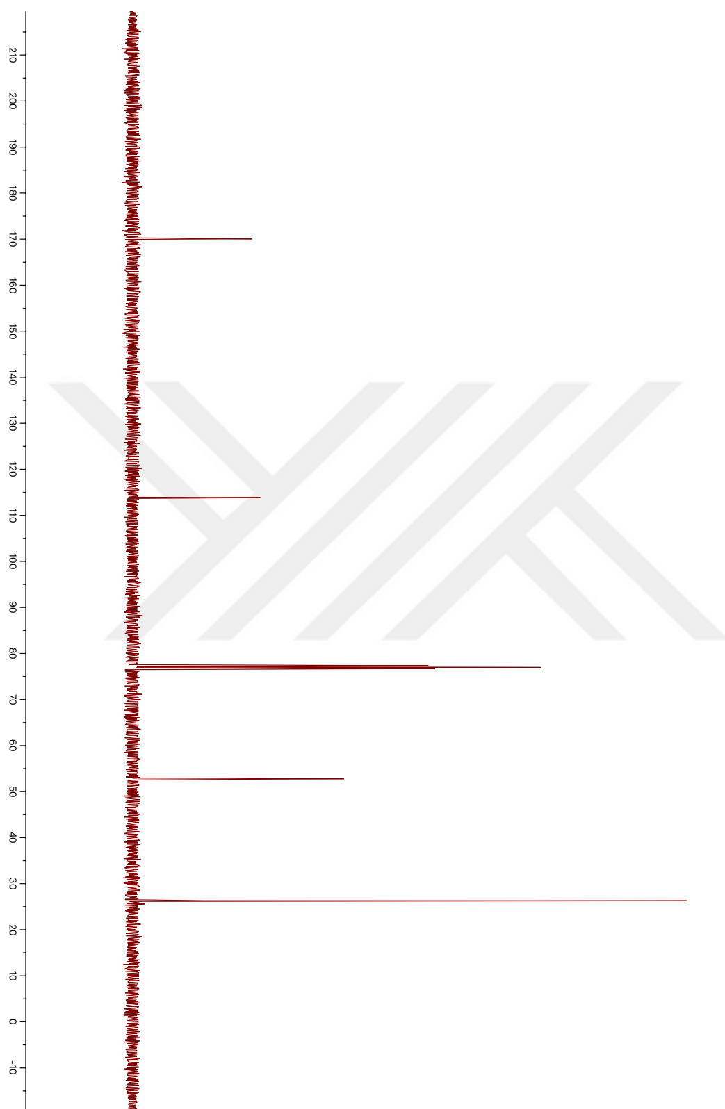
Figure 42. ^{13}\text{C} NMR spectrum of compound 9
