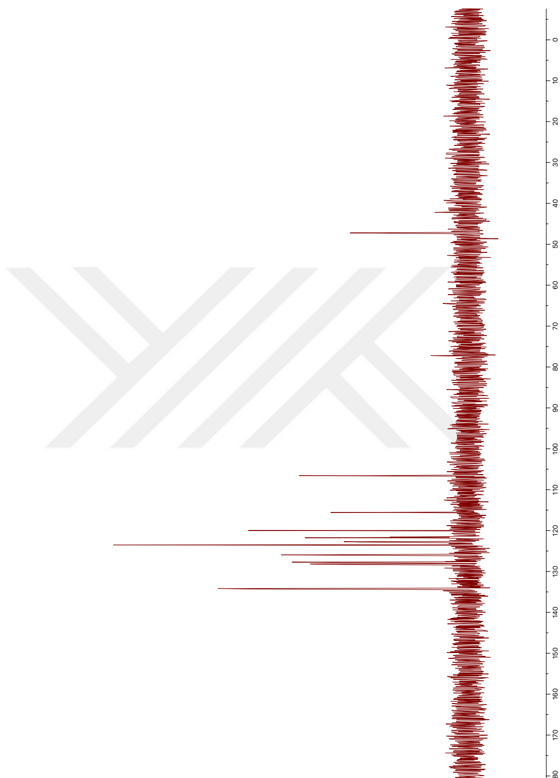
Figure 57. DEPT90 NMR spectrum of SPA-I
