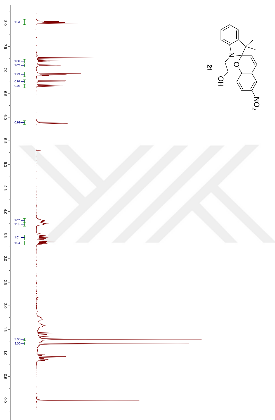
Figure 50. 1 H NMR spectrum of Compound 21
