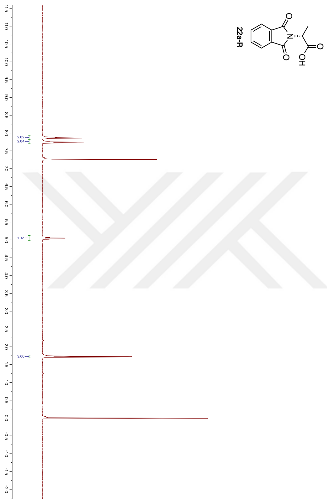
Figure 52. ^1\text{H} NMR spectrum of Compound 22a-R
