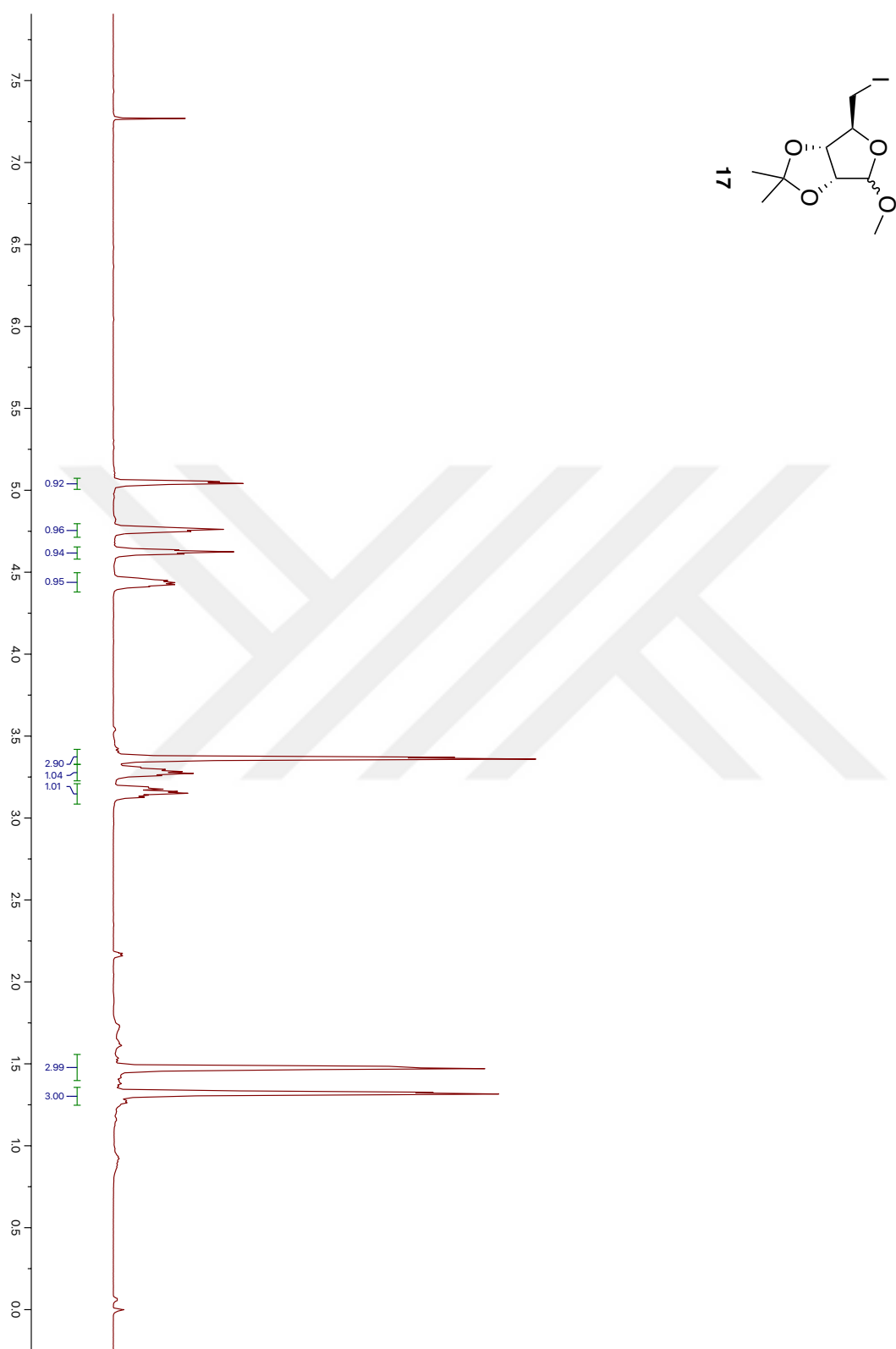
Figure 48. 1 H NMR spectrum of Compound 17
