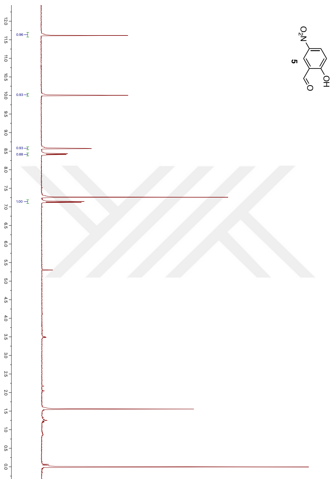
Figure 38. ^1\text{H} NMR spectrum of 2-hydroxy-5-nitrobenzaldehyde (5)
