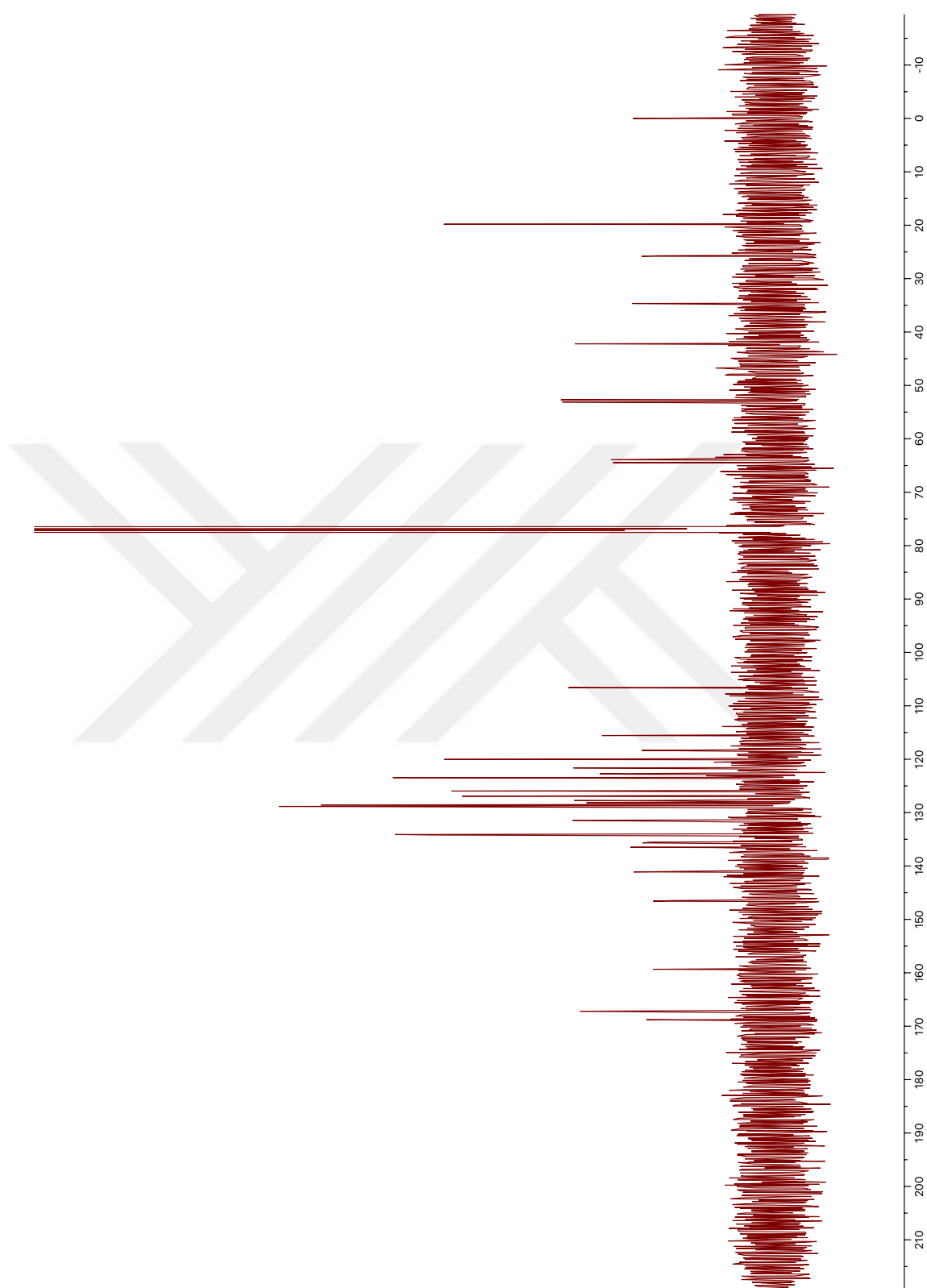
Figure 69. ^{13}\text{C} NMR spectrum of SPA-IV
