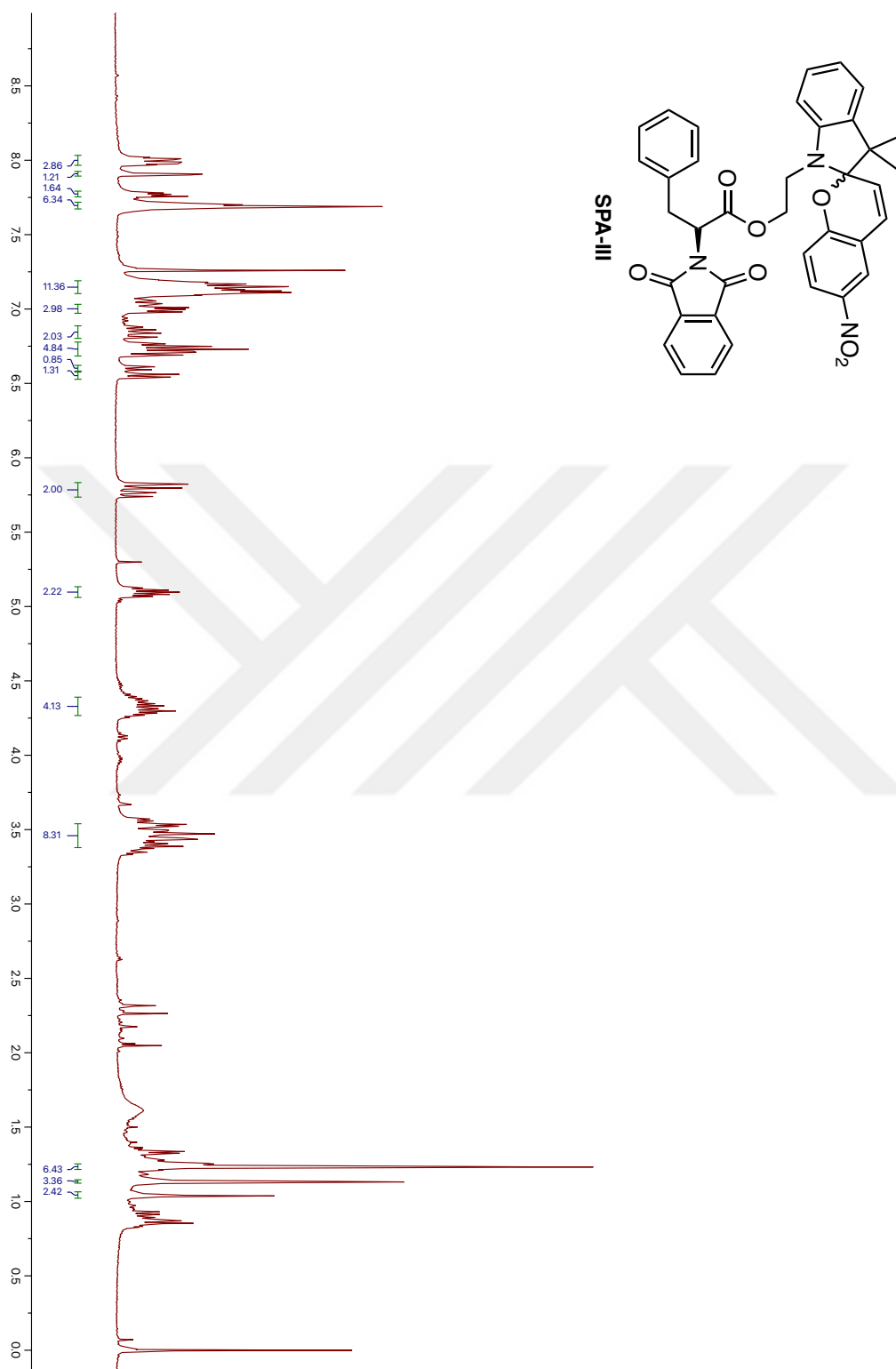
Figure 64. 1 H NMR spectrum of SPA-III
