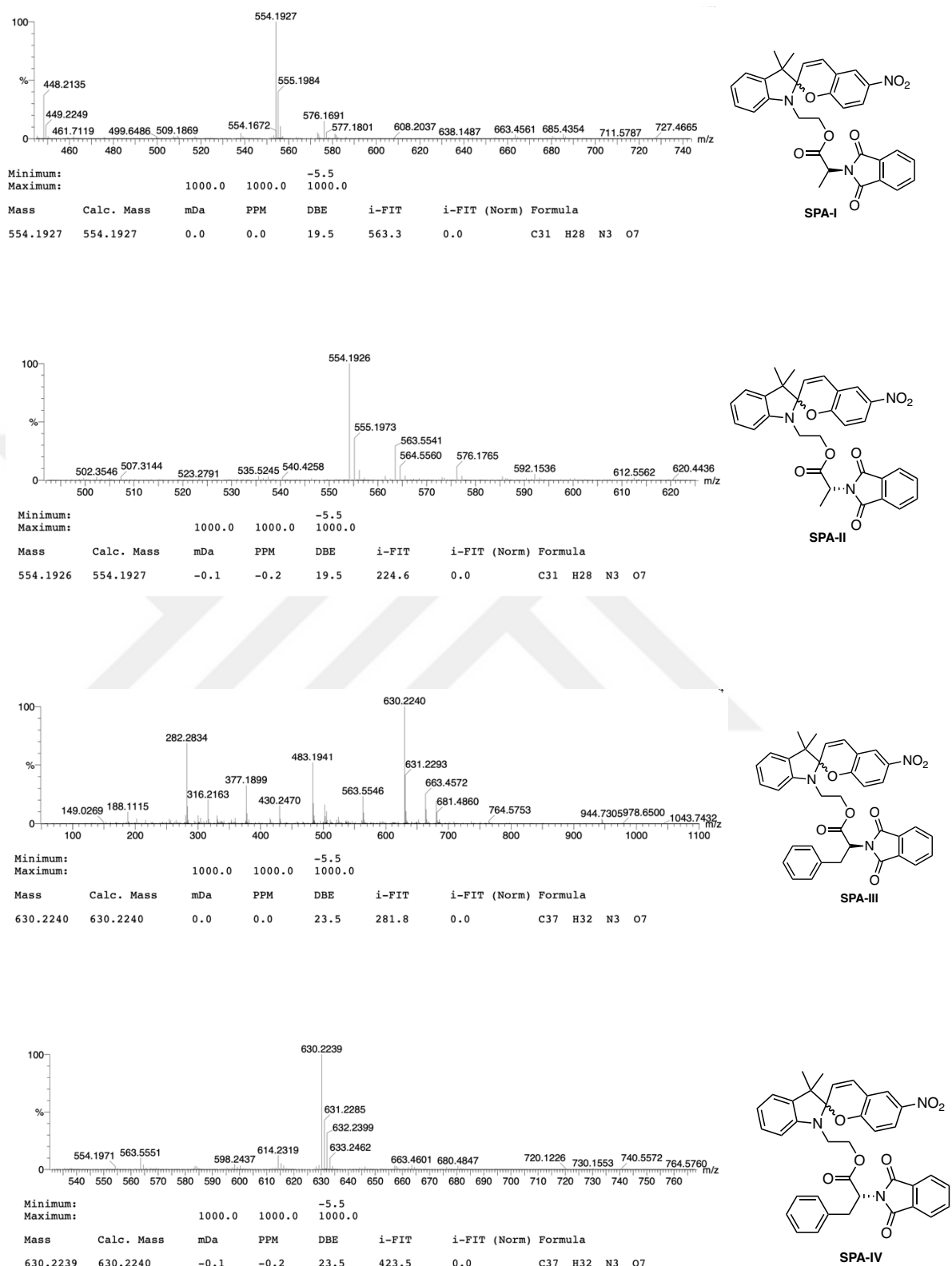
Figure 77. HRMS spectra of SPA-I, SPA-II, SPA-III, and SPA-IV
