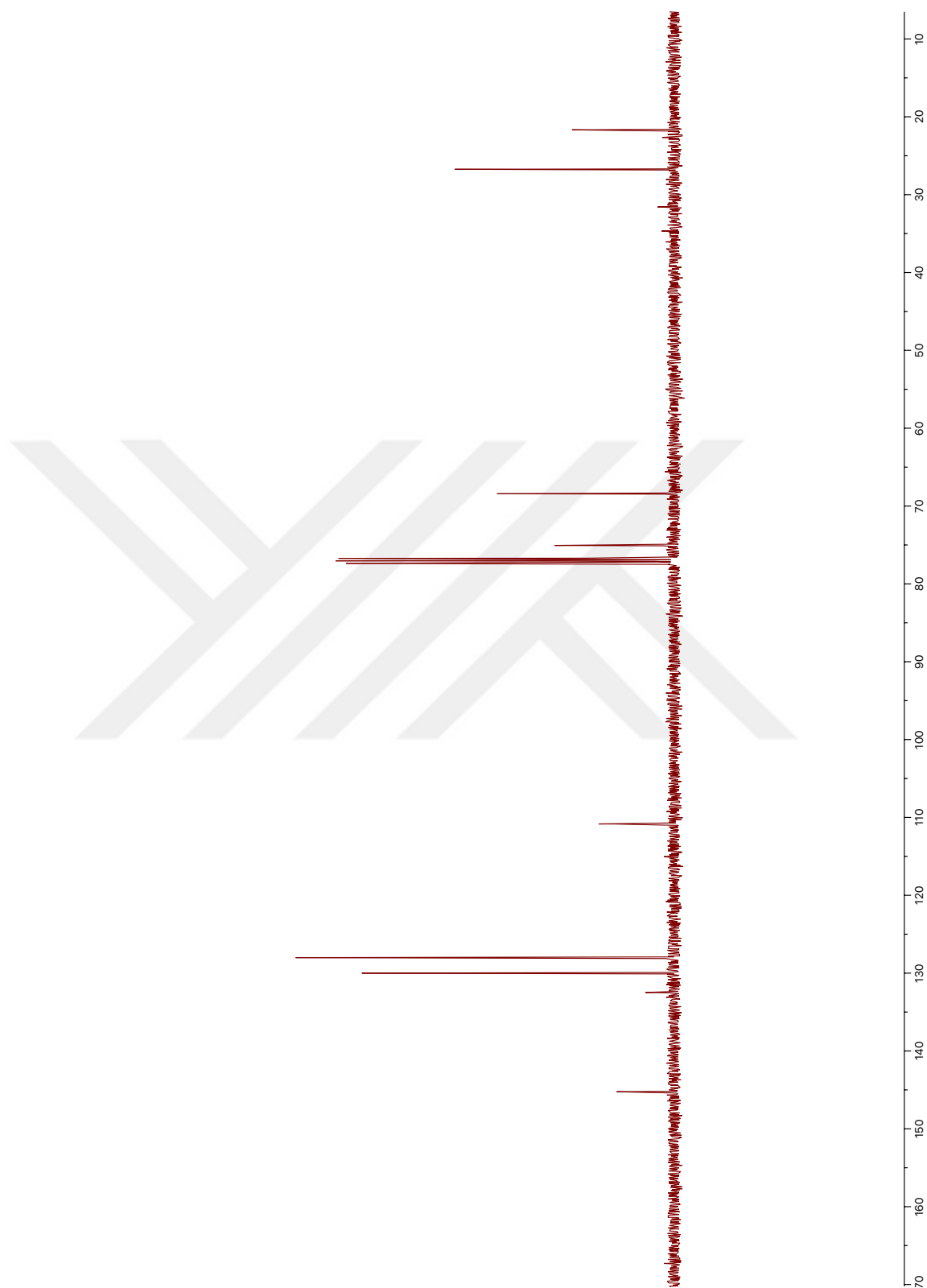
Figure 45. ^{13}\text{C} NMR spectrum of Compound 11
