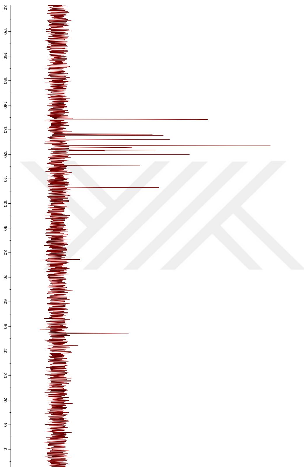
Figure 62. DEPT90 NMR spectrum of SPA-II
