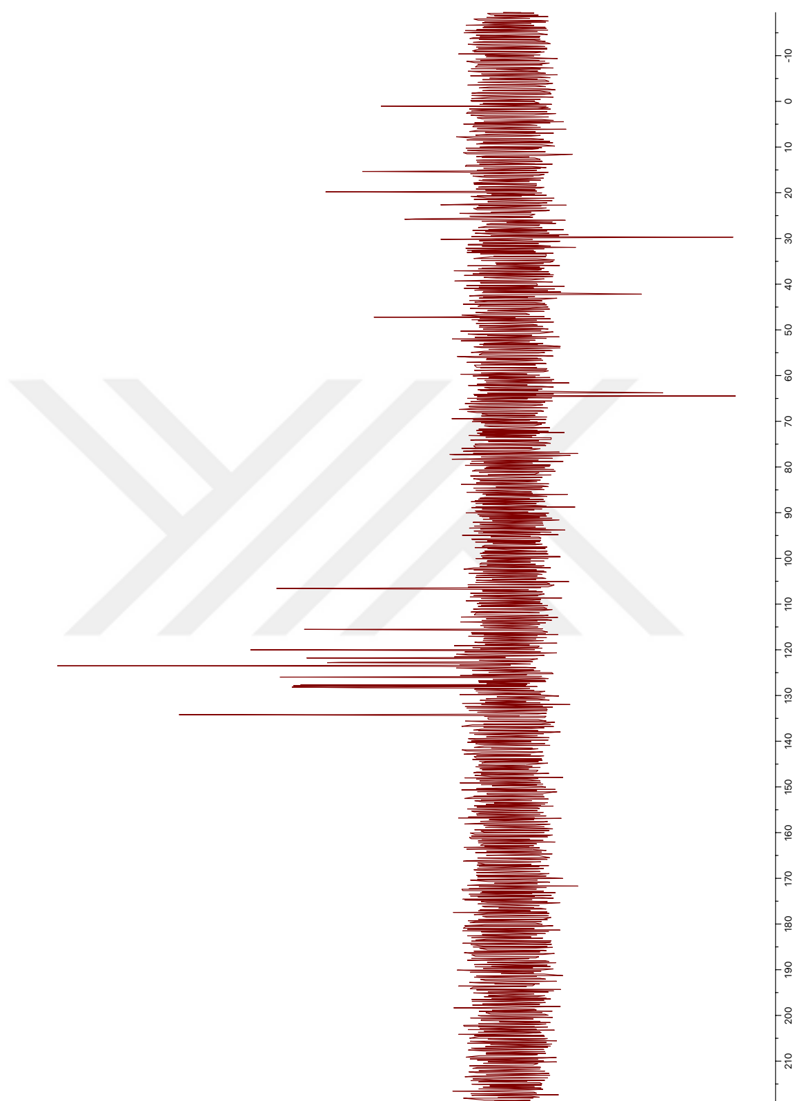
Figure 67. DEPT135 NMR spectrum of SPA-III
