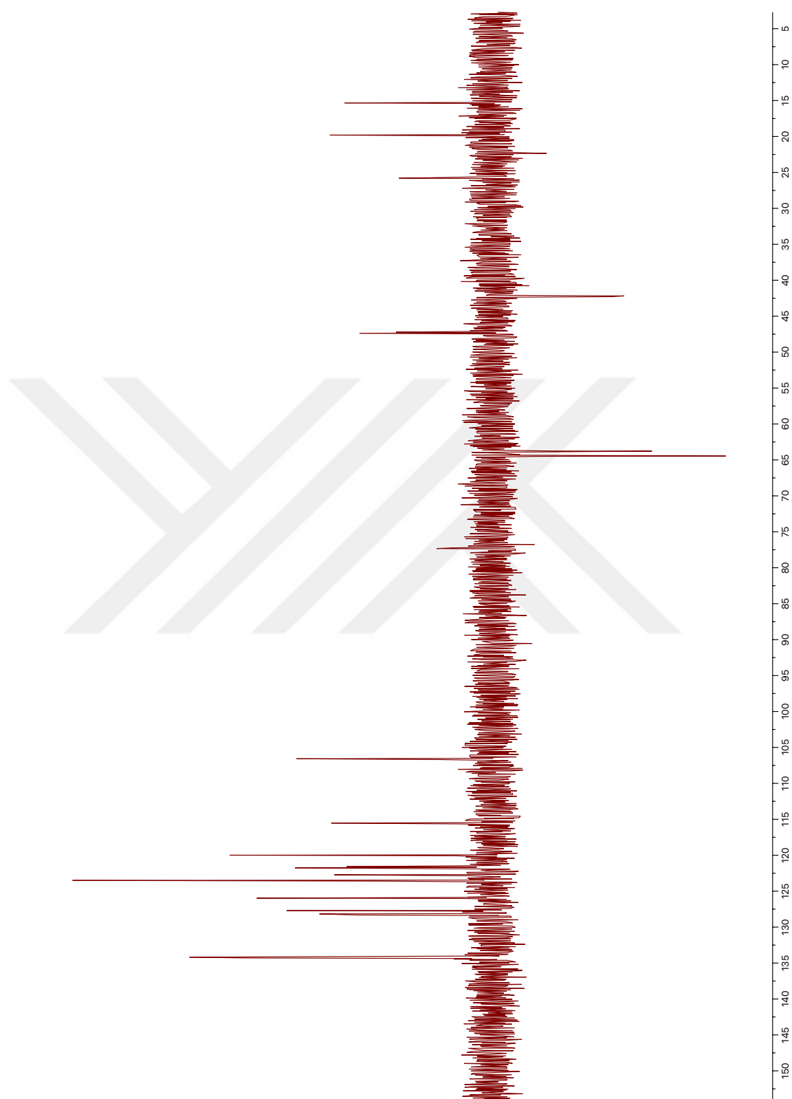
Figure 63. DEPT135 NMR spectrum of SPA-II
