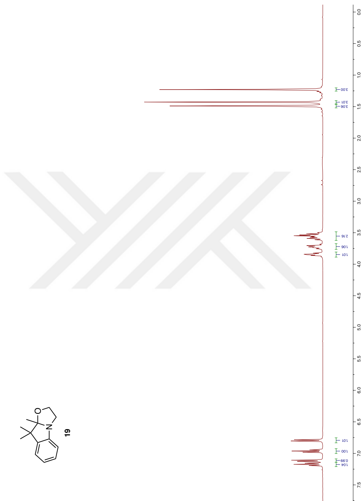
Figure 49. 1 H NMR spectrum of Compound 19
