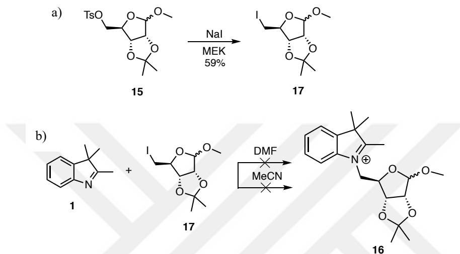
Scheme 21. Alternative way for the synthesis of compound 16
