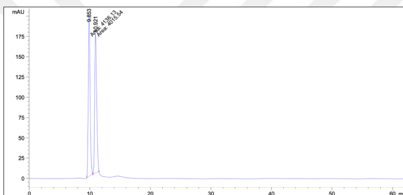
Figure 31. HPLC chromatogram of compound 21 (Chiralcel OD-H, eluent 90:10 n-hexane:isopropanol, flow rate 1.0 mL/min, t_R :9.8, 10.9)
