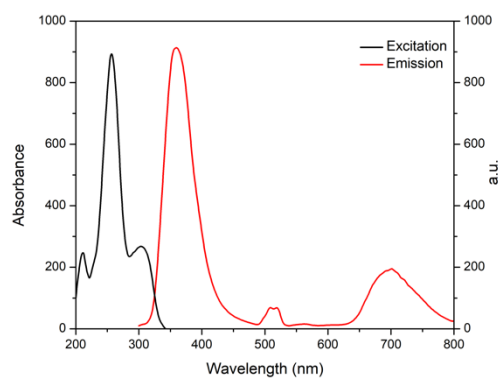
Figure 79. Fluorescence absorption and emission spectra SPA-II in isopropanol
