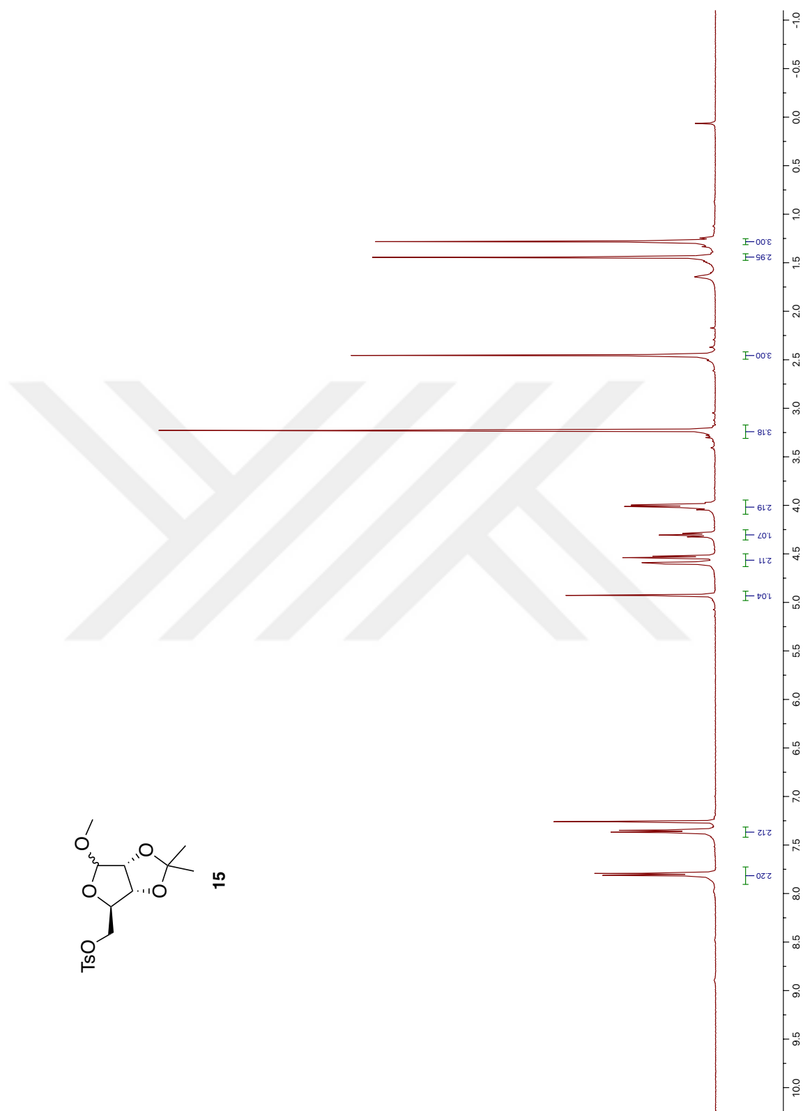
Figure 47. 1 H NMR spectrum of Compound 15
