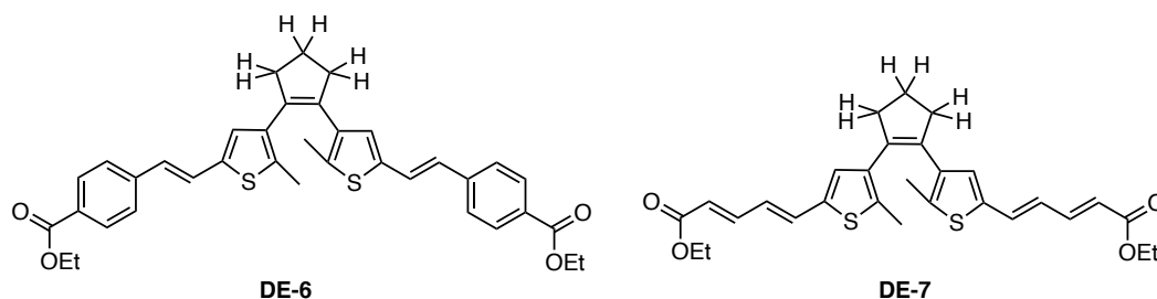
Figure 4. The ditithienylethenes with unsaturated ethyl benzoate moiety and tetraalkene derivatives
