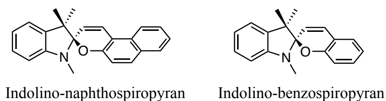
Figure 7. The spiropyrans reported by Fischer and Hirshberg
