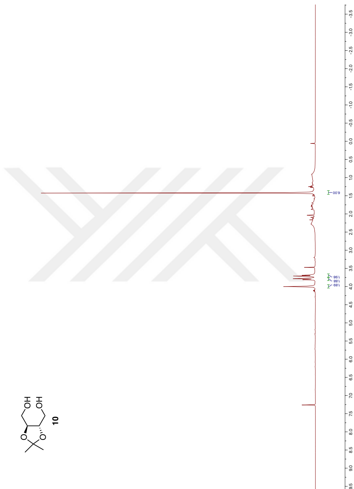
Figure 43. 1 H NMR spectrum of Compound 10
