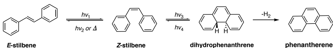
Scheme 3. Photoisomerization of stilbenes and its irreversible oxidation to phenanthrene
