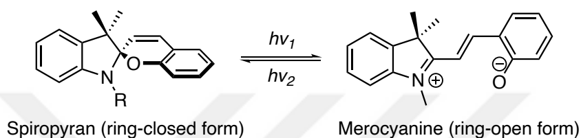
Scheme 4. The conversion between spiropyran and merocyanine
