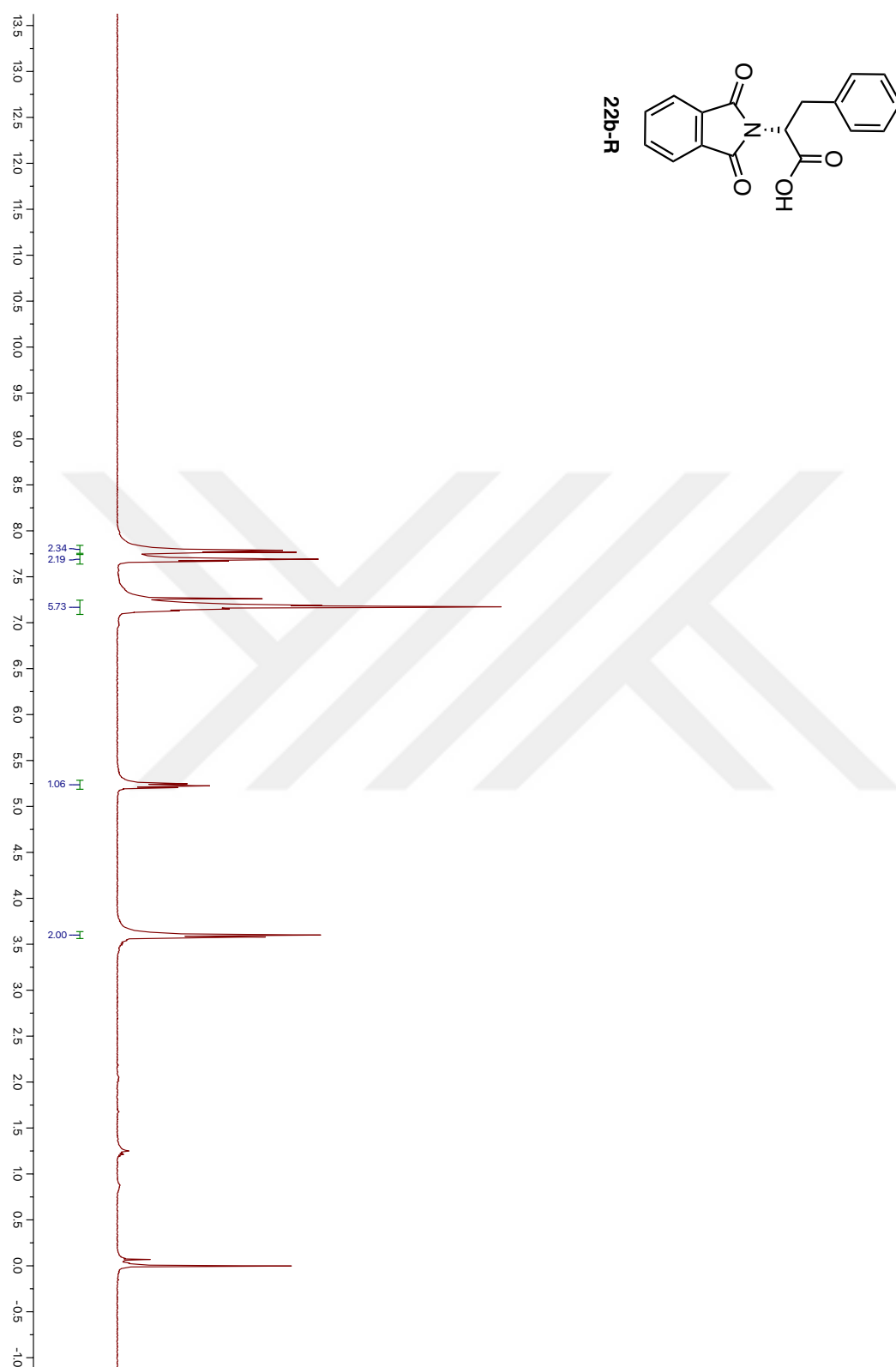
Figure 54. 1 H NMR spectrum of Compound 22b-R
