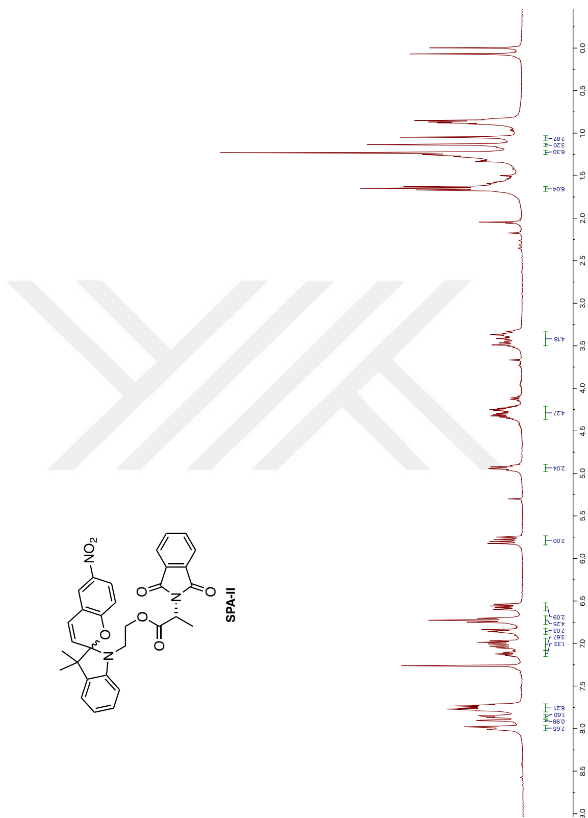
Figure 59. 1 H NMR spectrum of SPA-II
