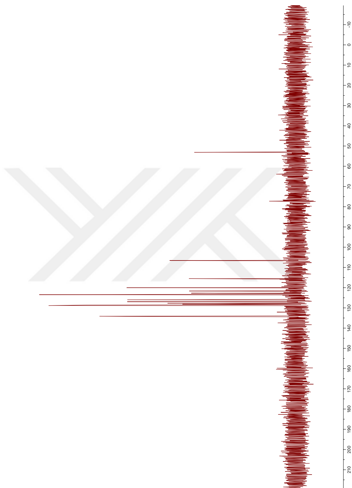
Figure 71. DEPT90 NMR spectrum of SPA-IV
