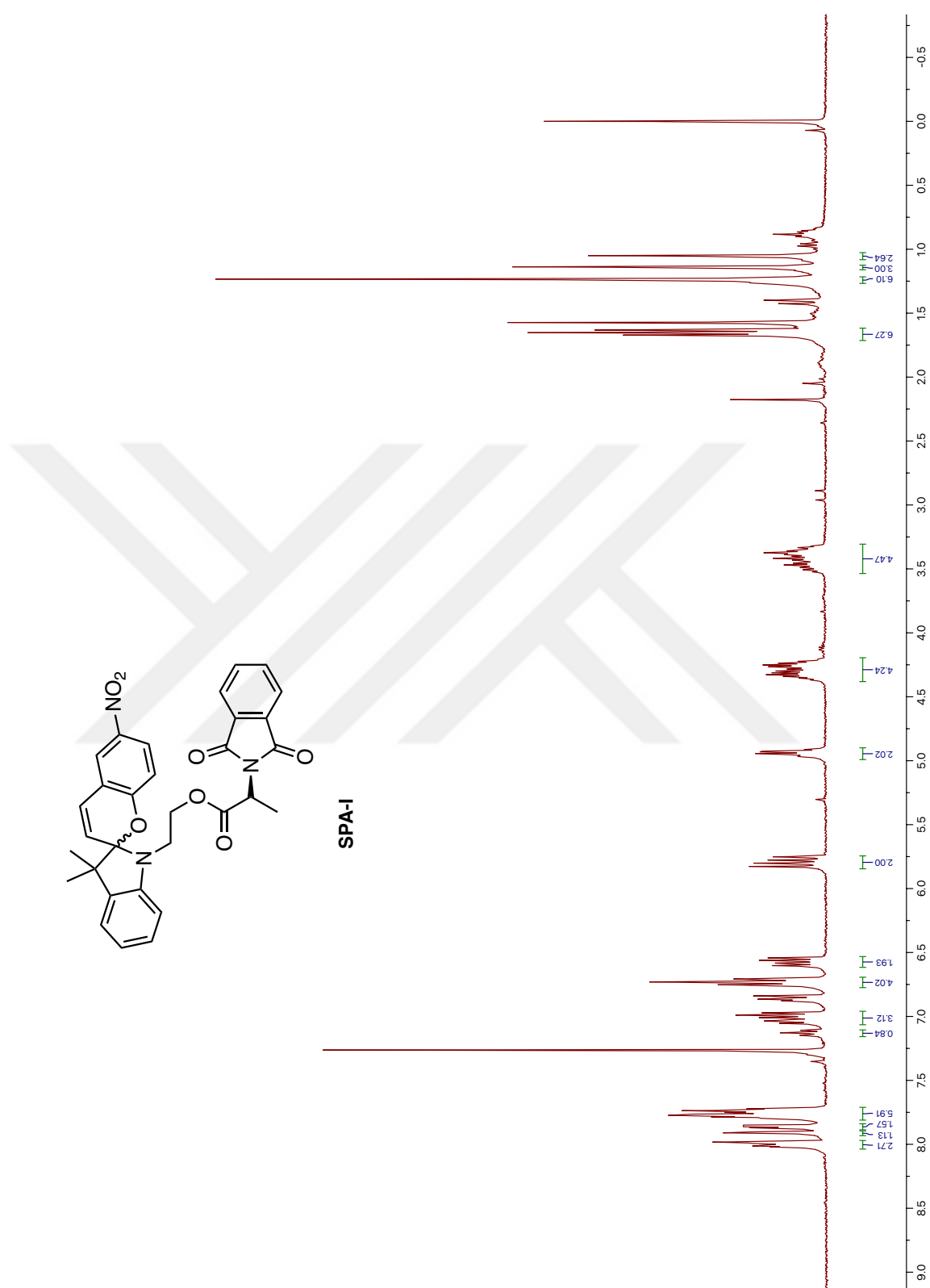
Figure 55. 1 H NMR spectrum of SPA-I
