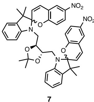
Figure 16. The designed spiropyran containing chiral moiety derived from tartaric acid
