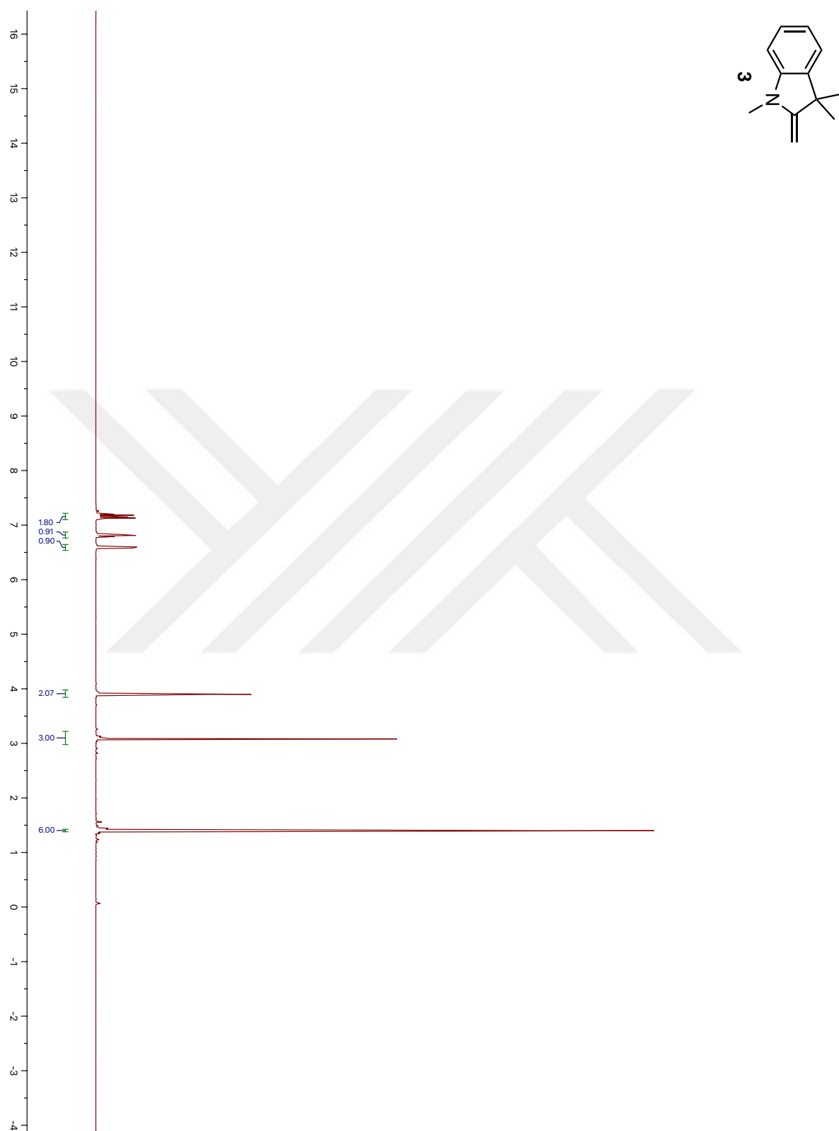
Figure 36. ^1\text{H} NMR spectrum of Compound 3
