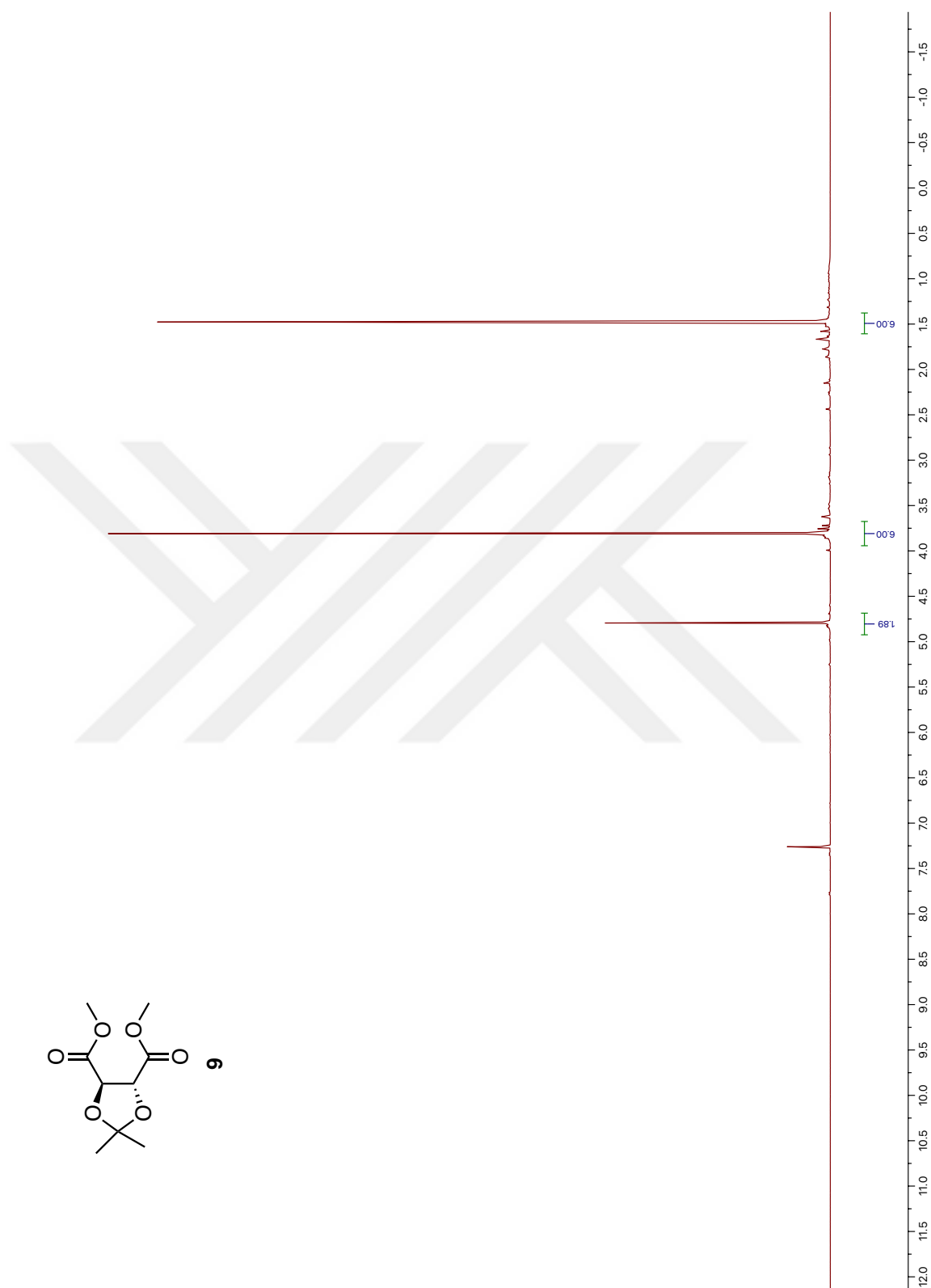
Figure 41. 1 H NMR spectrum of Compound 9
