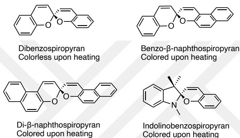
Figure 11. Spiropyrans derivatives exhibiting thermochromism
