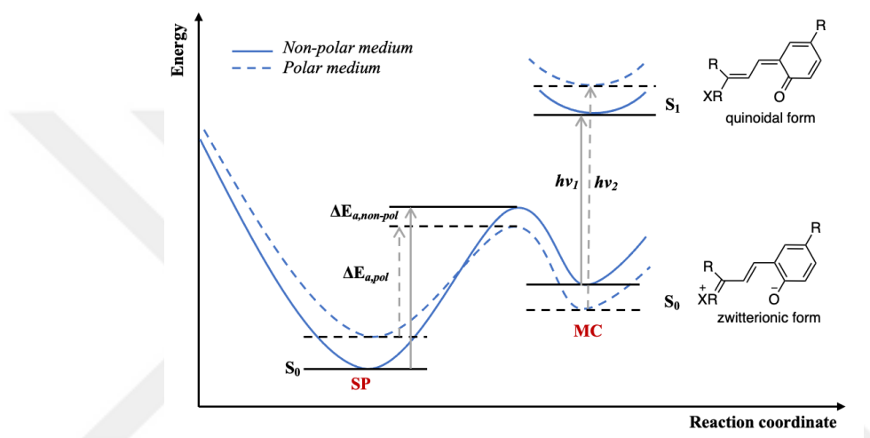
Figure 10. Potential energy diagram displaying solvatochromism of merocyanines redrawn inspired from reference 41
