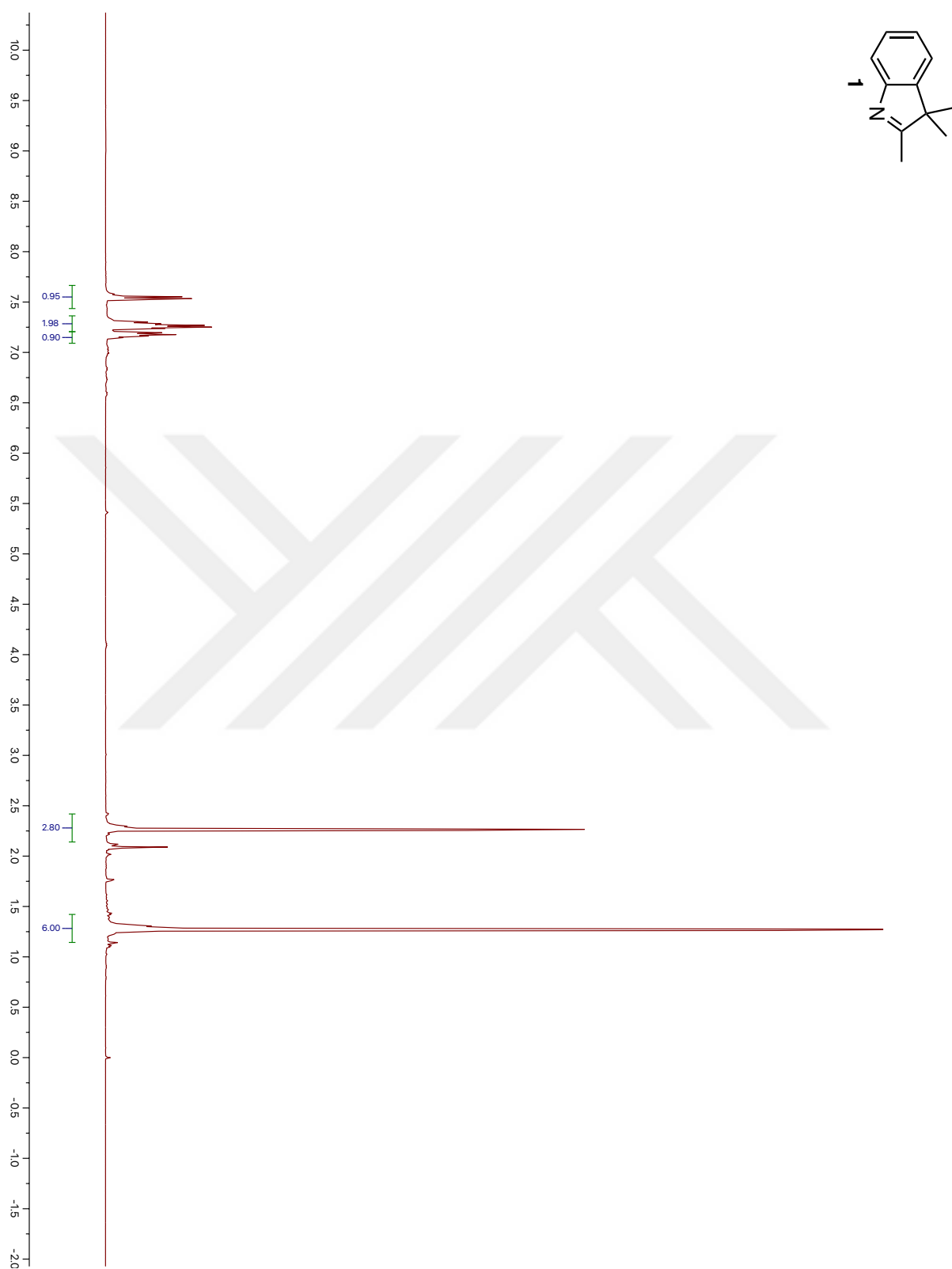
Figure 34. ^1\text{H} NMR spectrum of Compound 1
