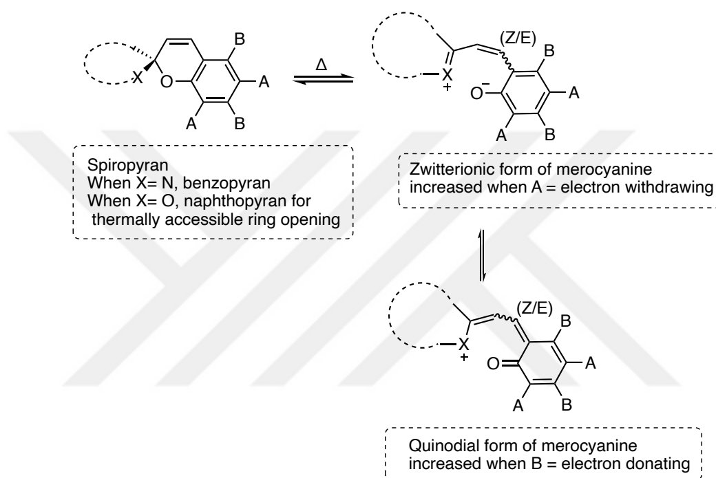
Scheme 13. Thermochromism of spiropyrans with different substituents
