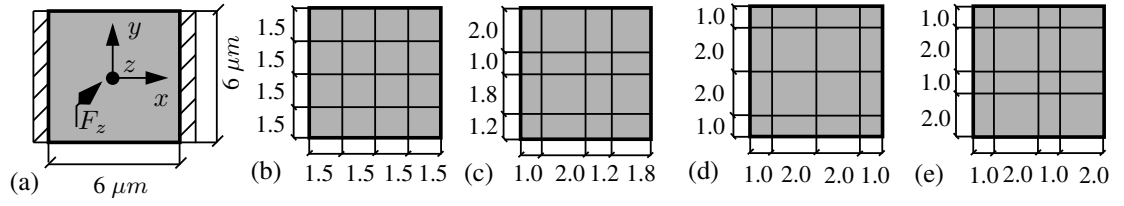
Figure 4.4: (a) Geometry and boundary conditions for square microplate. Thickness is taken as 1 \mu m and F_z = 1 mN . The problem is solved for (b) regular and (c), (d), (e) irregular mesh discretizations.
