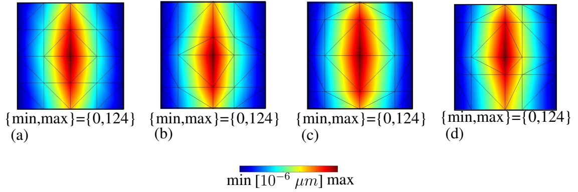
Figure 4.18: Contour plots depicting vertical displacement for the aspect ratio test given in Figure 4.4 for (a) regular mesh and (b, c, d) irregular meshes.
