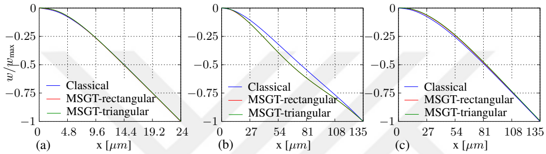
Figure 4.34: Deflection profiles from AA' sections as given in Figure 4.31. Structures are (a) from Stefanini et al. [7], and (b-c) from Patel and Rebeiz [8].
