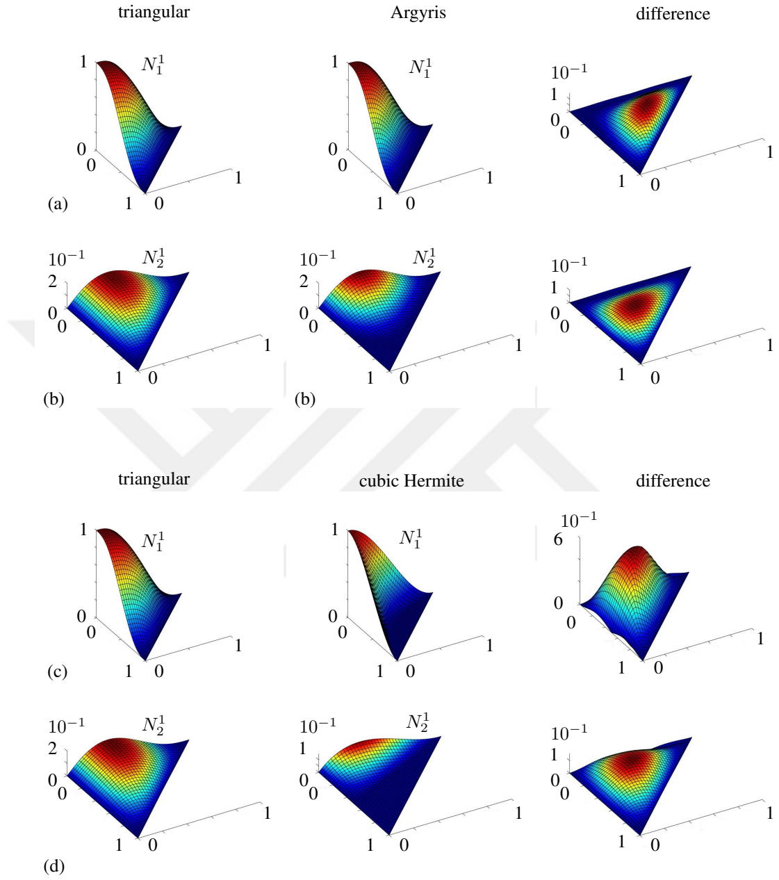
Figure 3.19: Comparison of the shape functions: (a) N_1^1 for Argyris and 18-DOF elements, (b) N_2^1 for Argyris and 18-DOF elements, (c) N_1^1 for cubic Hermite and 18-DOF elements, (d) N_2^1 for cubic Hermite and 18-DOF elements [3, 4].
