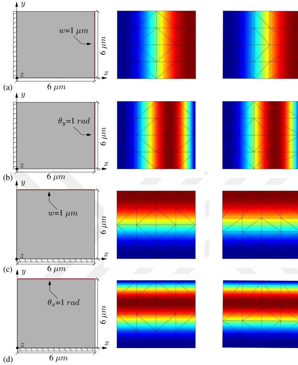
Figure 4.20: Geometry and boundary conditions (left) and corresponding displacement fields for the aspect ratio test considering response to prescribed displacements, for regular mesh (middle) and irregular mesh (right). The thickness of the plates is 1 \mu m for (a, b, c, d).
