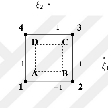
Figure 4.12: Coordinate transformation from (a) original coordinates to (b) mapped coordinates. Node numbers are indicated in bold.
