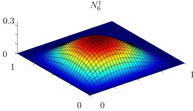
Figure 3.11: Additional twist DOF shape functions N_6^1 . Other N_6^j terms are symmetric with respect to
