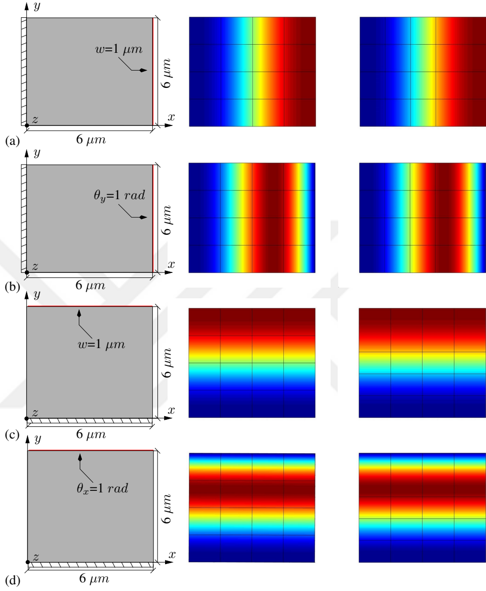
Figure 4.7: Geometry and boundary conditions (left) and corresponding displacement fields for the aspect ratio test considering response to prescribed displacements, for regular mesh (middle) and irregular mesh (right). The thickness of the plates is 1 \mu m for (a, b, c, d).
