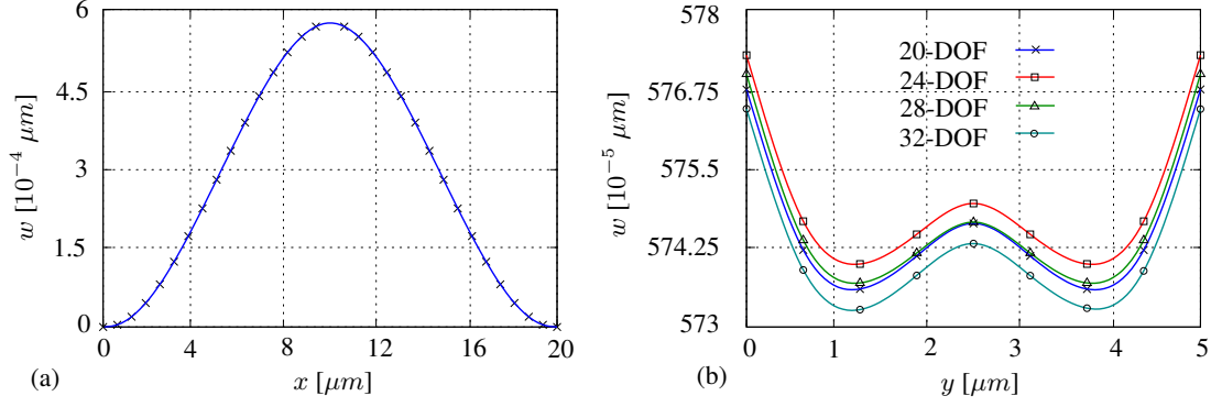
Figure 4.3: Deflection profiles of the two principal centroidal axes for the models constructed with 20-, 24-, 28-, 32-DOF elements, (a) for the principal axis along x-direction, and (b) for the principal axis along y-direction.
