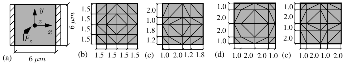
Figure 4.17: (a) Geometry and boundary conditions for square microplate. Thickness is taken as 1 \mu m and F_z = 1 mN . The problem is solved for (b) regular and (c), (d), (e) irregular mesh discretizations.
