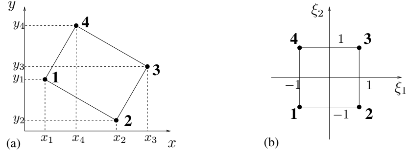
Figure 3.8: Coordinate transformation from (a) original coordinates to (b) mapped coordinates. Node numbers are indicated in bold.
