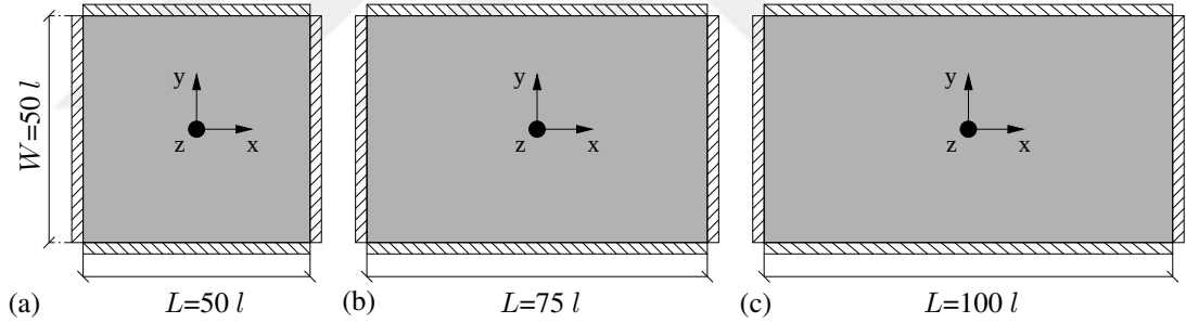
Figure 4.15: Geometry and boundary conditions for the three cases (a)-(c) in [5] replicated numerically with the proposed higher order microplate elements. The dimensions are in terms of the length scale parameters l = l_0 = l_1 = l_2 , with thickness h = l in all cases. A distributed load of 1 \text{ kN/m}^2 is applied for all cases as in the said study. Therein, the material parameters specific to epoxy are used [6], see Table 4.1.
