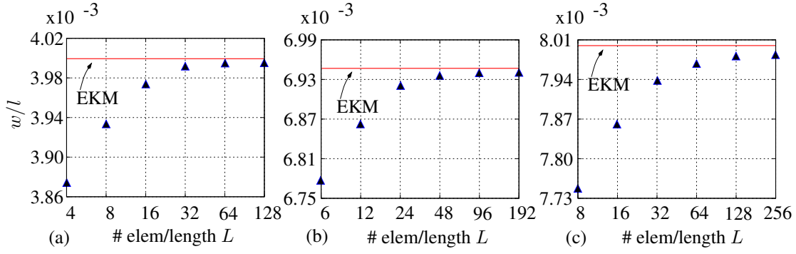
Figure 4.25: Midpoint deflections of the cases in Figure 4.15 versus number of triangular elements per element length versus results obtained with EKM in [5].
