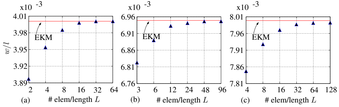
Figure 4.16: Midpoint deflections of the cases in Figure 4.15 versus number of rectangular elements per element length versus results obtained with EKM in [5].
