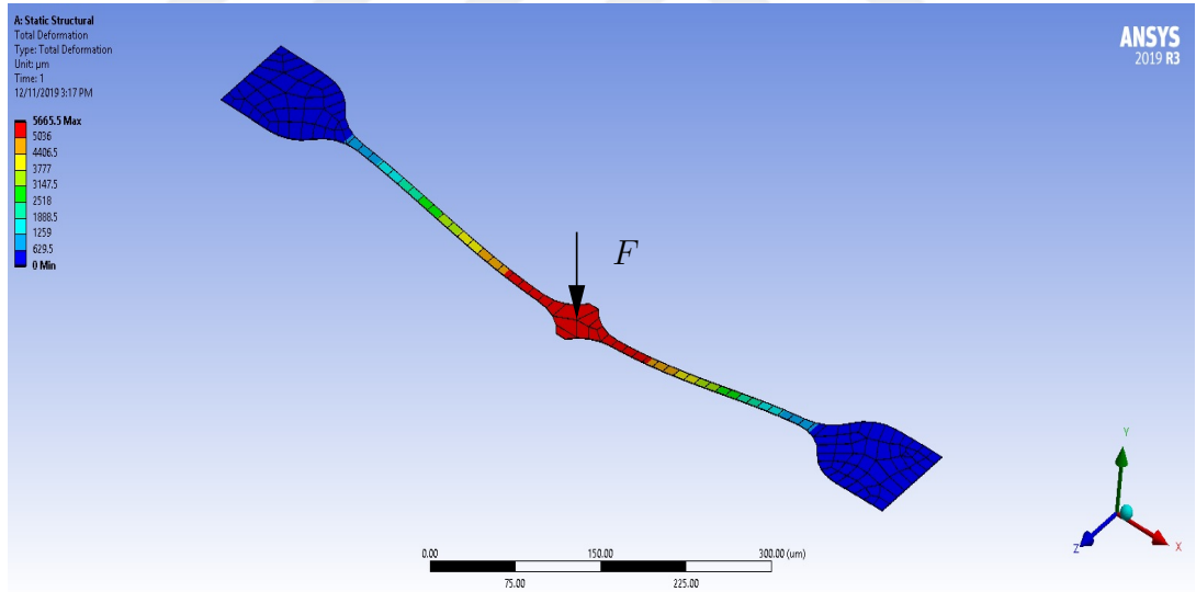
Figure 4.28: ANSYS Mechanical model of the experiments in Espinosa et al. [1]. The force applied is 0.3 mN per Table 4.2. This figure is given for specimen 2, the thickness of which is 1.0 \mu m .
