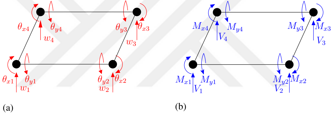
Figure 3.4: (a) Nodal degrees of freedom and (b) corresponding nodal forces for a classical Kirchhoff-Love plate formulation
