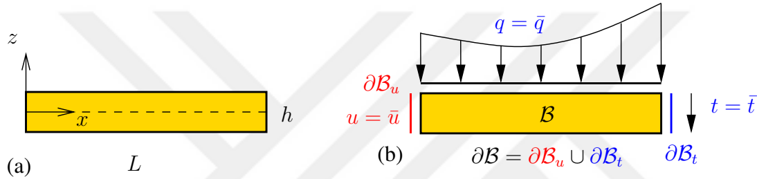
Figure 2.1: (a) Kirchhoff-Love plate geometry and (b) Dirichlet \partial\mathcal{B}_u and Neumann \partial\mathcal{B}_t boundary conditions imposed. Note that \partial\mathcal{B} = \partial\mathcal{B}_u \cup \partial\mathcal{B}_t .
