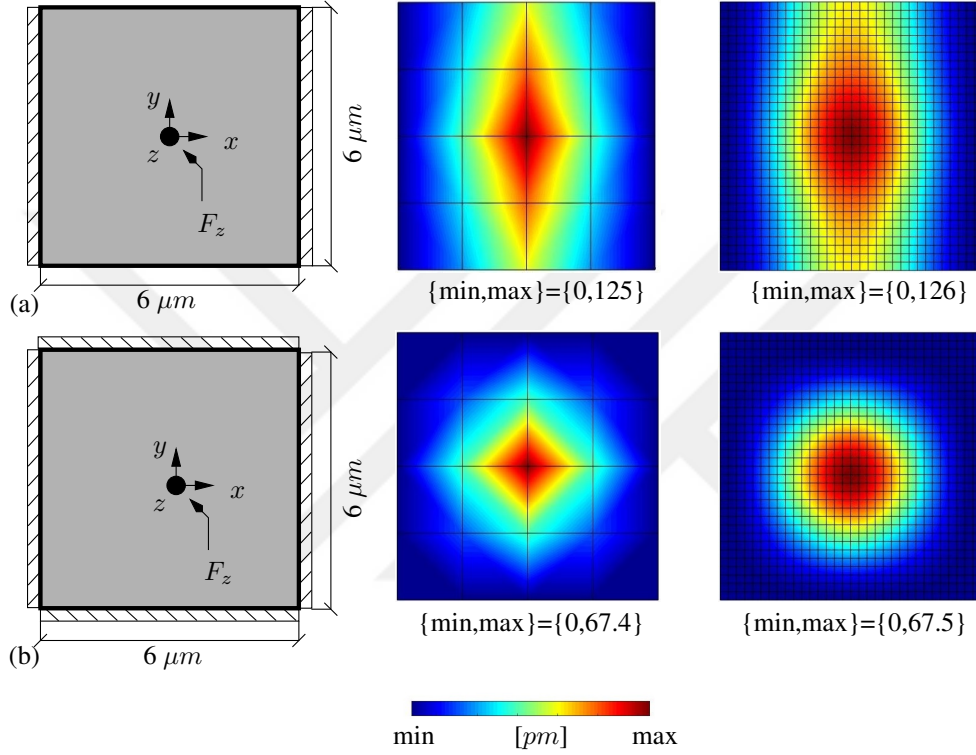
Figure 4.8: Geometry and boundary conditions (left) together with displacement profiles for deflected shapes for mesh refinement tests on a 4x4 and a 32x32 mesh, (a) fixed-fixed, and (b) all sides fixed. F_z=1 \text{ mN} . Thickness is 1 \mu m .
