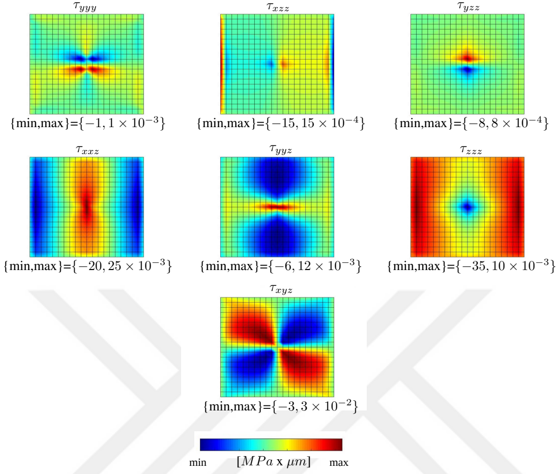
Figure 4.14: Higher order stress metrics (continued) per Equations B.51-B.57. It must be noted that \tau_{xzz}=\tau_{zxx}=\tau_{zxz} , \tau_{yzz}=\tau_{zyz}=\tau_{zzy} , \tau_{xxz}=\tau_{zxx}=\tau_{xzx} , \tau_{yyz}=\tau_{zyy}=\tau_{yzy} , \tau_{xyz}=\tau_{yxz}=\tau_{yzx}=\tau_{zxy}=\tau_{zyx} .
