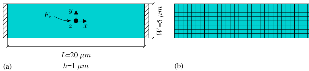
Figure 4.1: (a) Geometry and boundary conditions for the plate with dimensions L=20 \mu m , W=5 \mu m , h=1 \mu m under a load of F_z = 1 \text{ mN} applied towards +z direction at the midpoint with the material properties given as in Table 4.1, (b) relevant mesh for the comparative analysis.
