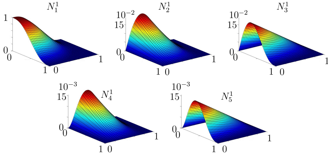
Figure 3.7: First five shape functions for the new Kirchhoff-Love plate element in MSGT (of the 1st node). l_0 = l_1 = l_2 = 3.71 \mu m as given in the forthcoming section.
