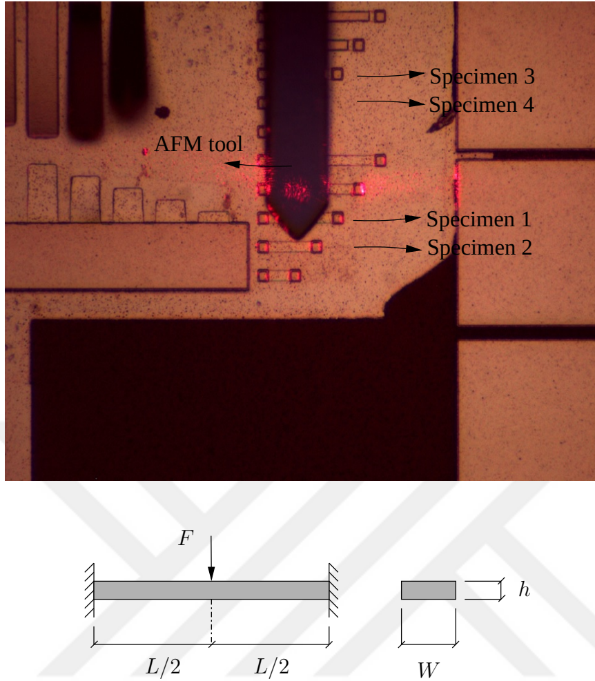
Figure 5.1: Photo of the specimens and the AFM tool from the top and relevant idealizations.
