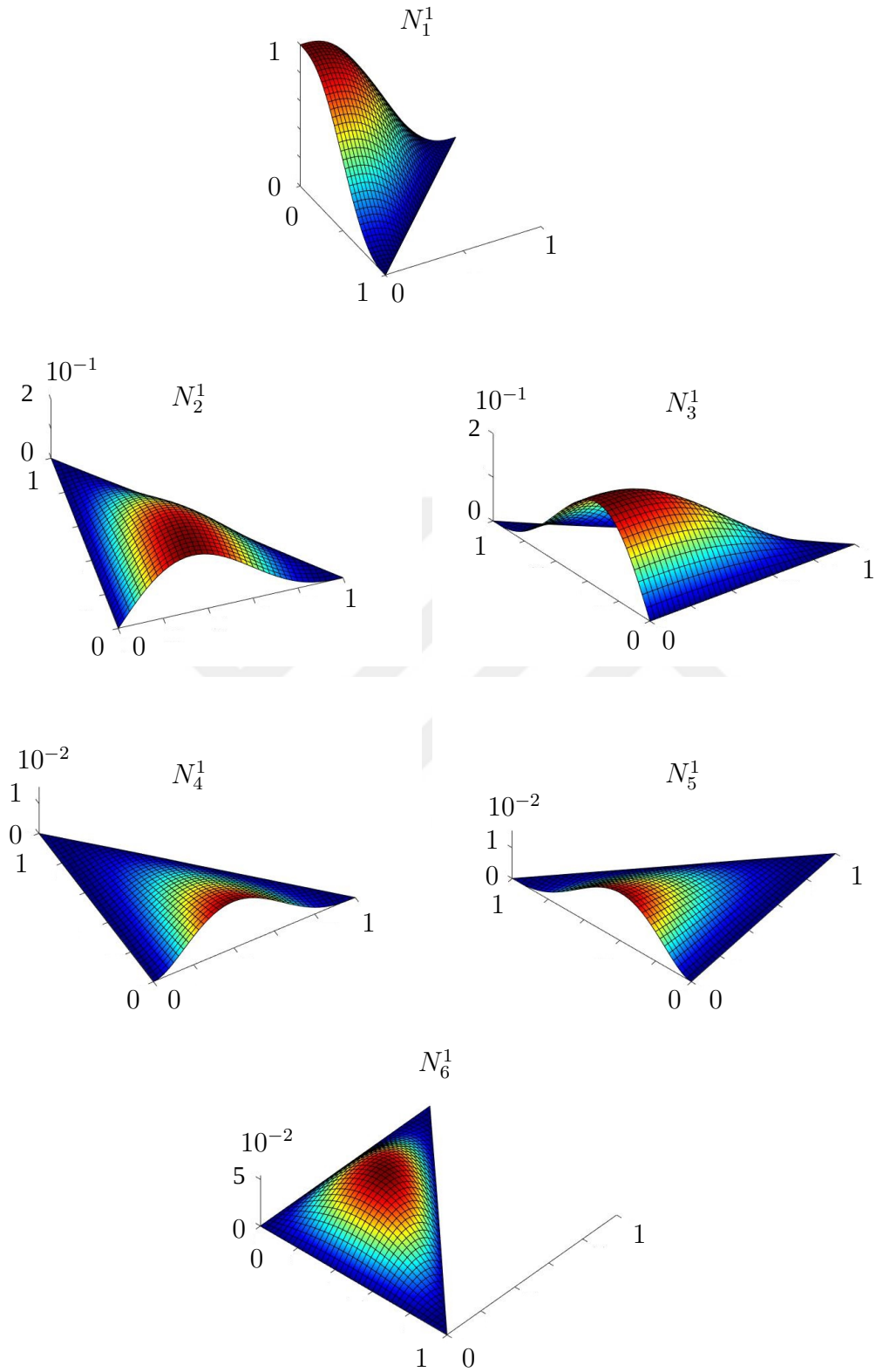
Figure 3.16: Shape functions for the first node for the newly developed 18-DOF triangular element.
