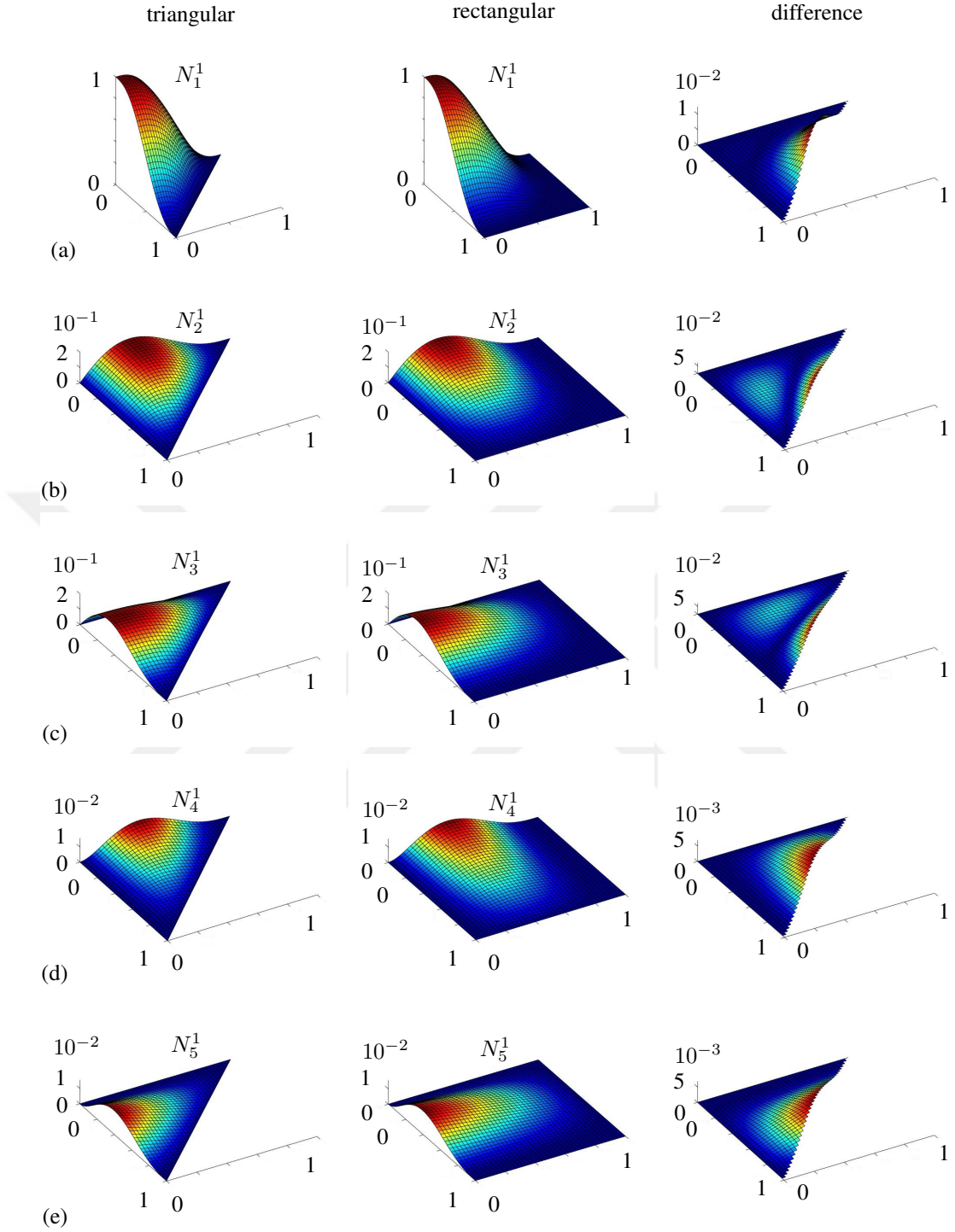
Figure 3.17: The first five shape functions for the first node (a)-(e) for the newly developed 18-DOF triangular element (left column) and for the newly developed 24-DOF rectangular element (middle column), along with the difference of two (right column).
