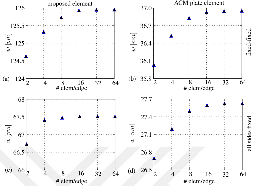
Figure 4.9: Mesh convergence of the microplate element: Loading point deflection versus element per edge for (a) MSGT-based KL solution for the fixed-fixed plate, (b) classical KL solution for the fixed-fixed plate, (c) MSGT-based KL solution for the plate with all sides fixed, (d) classical KL solution for the plate with all sides fixed.
