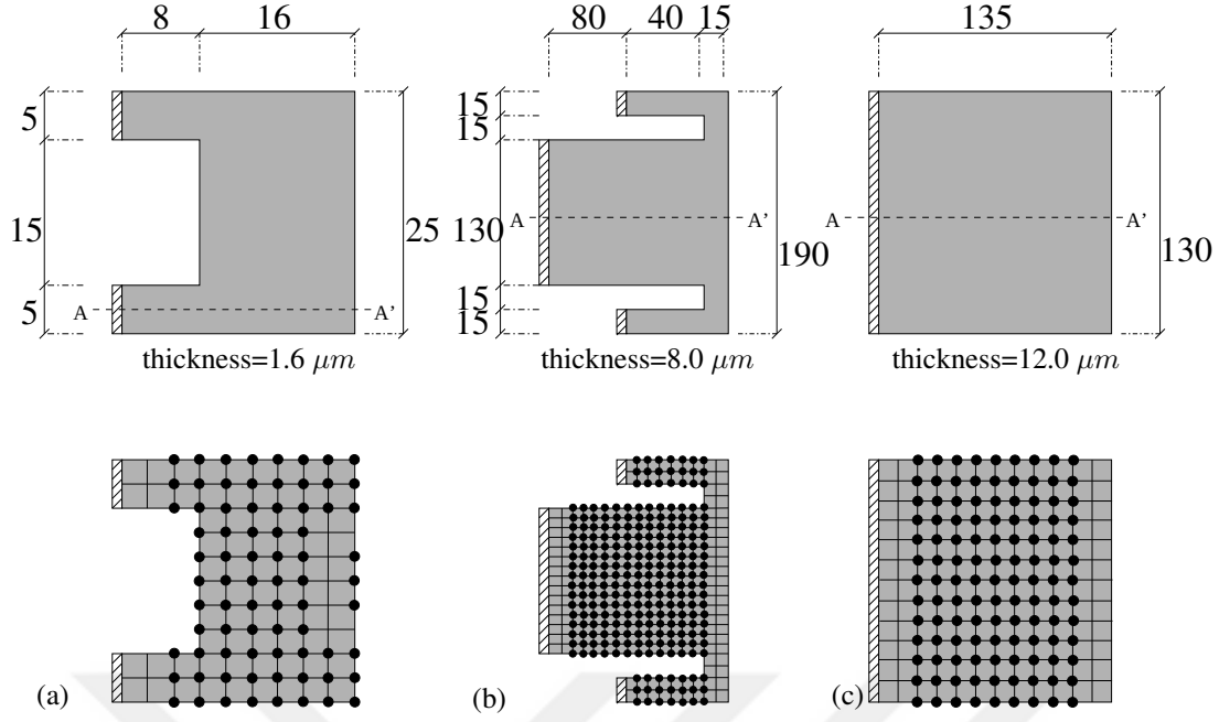
Figure 4.31: Real MEMS structures that are modelled with new plate elements from Stefanini et al. [7] (a) and from Patel and Rebeiz [8] (b and c). The total loads of F_z = 77.2 \mu N (a) and F_z = 3 mN (b and c) are distributed to the bold circled nodes as given in corresponding meshes. Note that the structure in (c) is the untethered part of the one in (b). All dimensions in \mu m .
