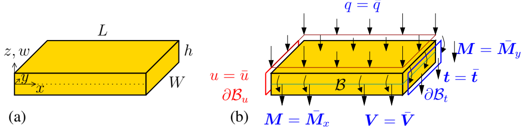
Figure 2.2: (a) Kirchhoff-Love plate geometry and (b) Dirichlet \partial\mathcal{B}_u and Neumann \partial\mathcal{B}_t boundary conditions imposed. Note that \partial\mathcal{B} = \partial\mathcal{B}_u \cup \partial\mathcal{B}_t .
