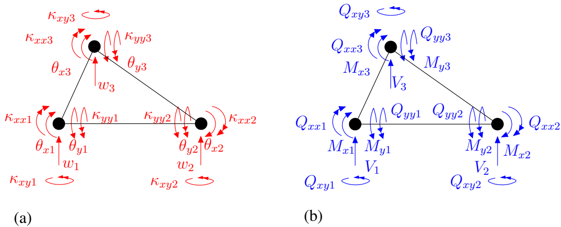
Figure 3.15: (a) Nodal degrees of freedom and (b) corresponding nodal forces for a 18-DOF higher order triangular Kirchhoff-Love plate formulation based on MSGT.
