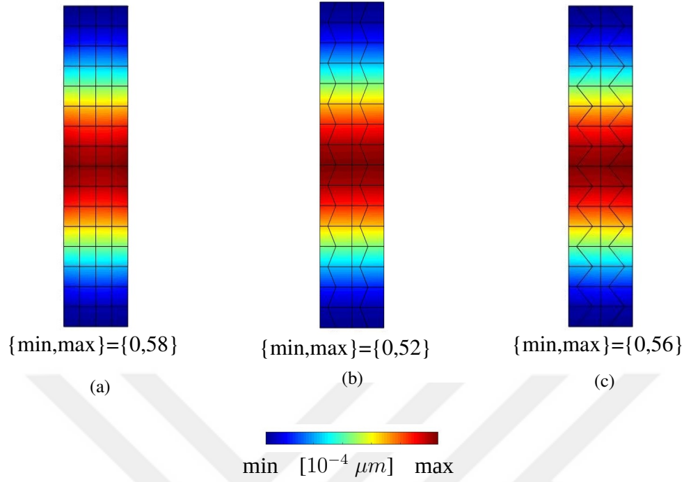
Figure 4.10: Displacement fields for (a) distorted patch (b) regular patch for a mid-point load of 1 N applied upwards. Values are in \mu m .
