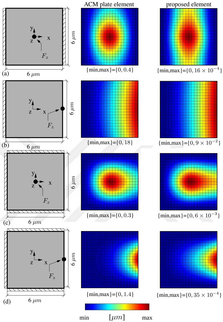
Figure 4.11: Deflected shapes for a microplate with classical theory (second column) and MSGT (third column). Boundary conditions are (a) CFCF, point load applied at midpoint, (b) CFFF, point load applied at endpoint, (c) CCCF, point load applied at midpoint of the plate, (d) CCCF, point load applied at midpoint of the free end. F_z=1 mN . Thickness is 1 \mu m .
