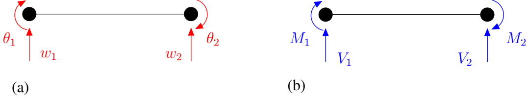
Figure 3.1: (a) Nodal degrees of freedom and (b) corresponding nodal forces for a classical Euler-Bernoulli beam formulation
