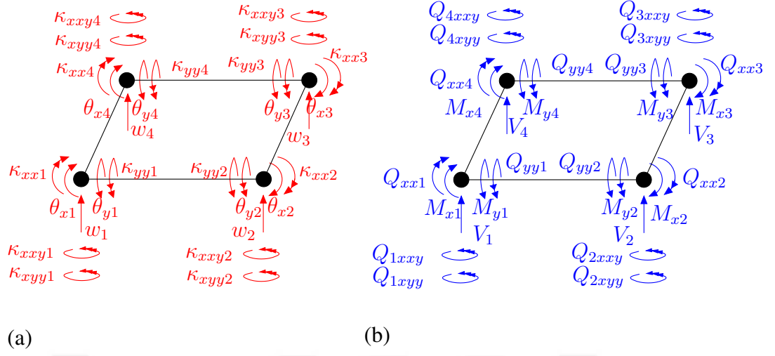
Figure 3.12: (a) Nodal degrees of freedom and (b) corresponding nodal forces for a 28-DOF higher order Kirchhoff-Love plate formulation based on MSGT.
