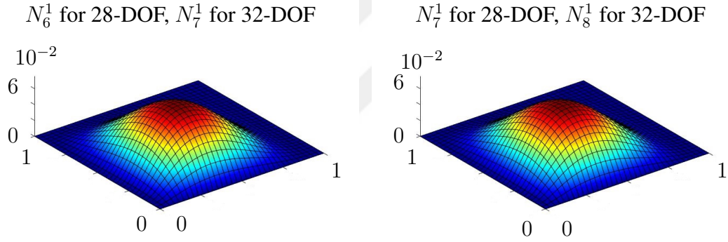
Figure 3.14: Two of the additional higher order twist DOF shape functions for 28-DOF and 32-DOF elements.
