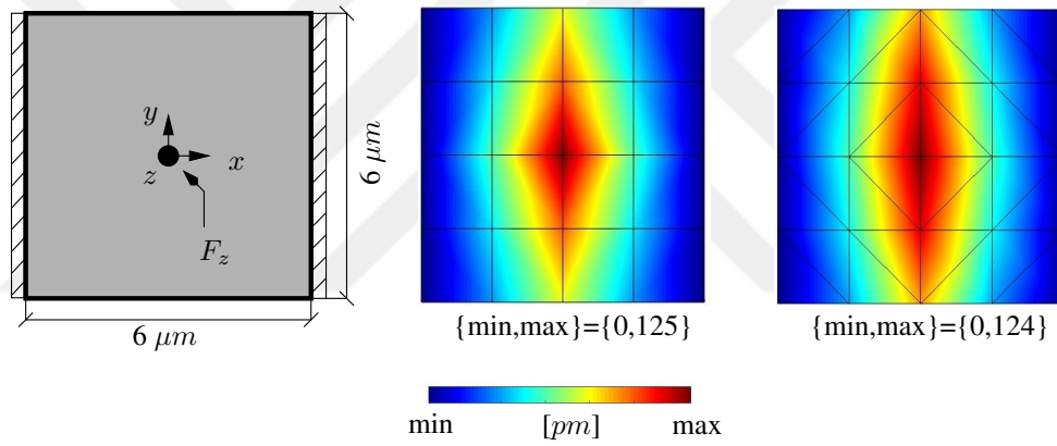
Figure 4.19: Geometry and boundary conditions (left) together with displacement profiles for rectangular elements and triangular elements. F_z = 1 \text{ mN} . Thickness is 1 \mu m .
