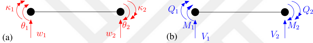
Figure 3.2: (a) Nodal degrees of freedom and (b) corresponding nodal forces for a higher order Euler-Bernoulli beam formulation based on MSGT.
