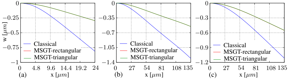
Figure 4.33: Deflection profiles from AA' sections as given in Figure 4.31. Structures are (a) from Stefanini et al. [7] and (b-c) from Patel and Rebeiz [8].
