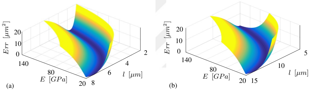
Figure 4.27: Corresponding Err , E , and l values for (a) MSGT and (b) MCST with rectangular plate elements.
