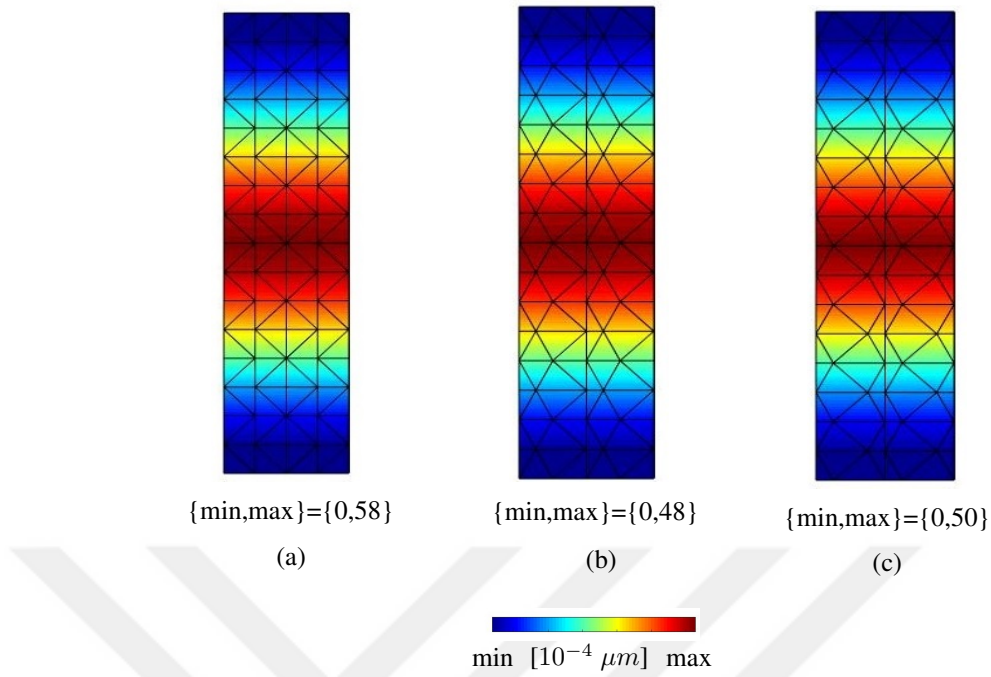
Figure 4.24: Displacement fields for (a) distorted patch (b) regular patch for a mid-point load of 1 N applied upwards. Values are in \mu m .
