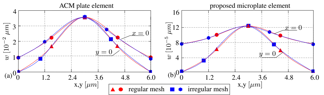
Figure 4.6: Midline deflections along x - and y -axes obtained from the regular and irregular meshes depicted in Figure 4.5 for (a) classical theory ( l_i = 0 ) and (b) proposed element formulation.
