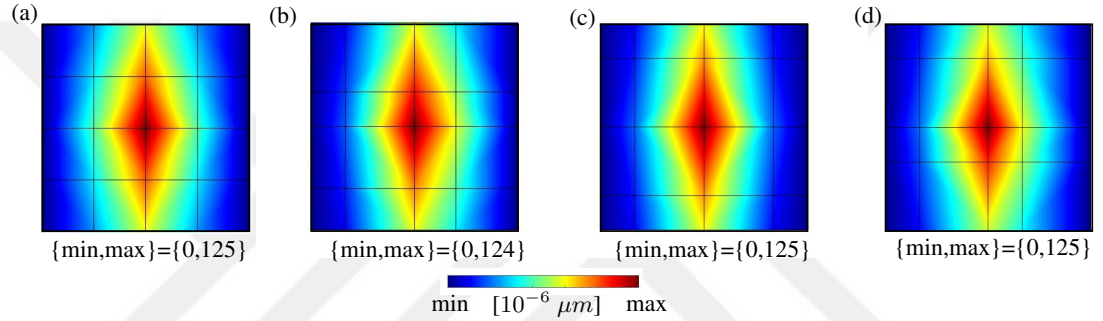
Figure 4.5: Contour plots depicting vertical displacement for the aspect ratio test given in Figure 4.4 for (a) regular mesh and (b, c, d) irregular meshes.
