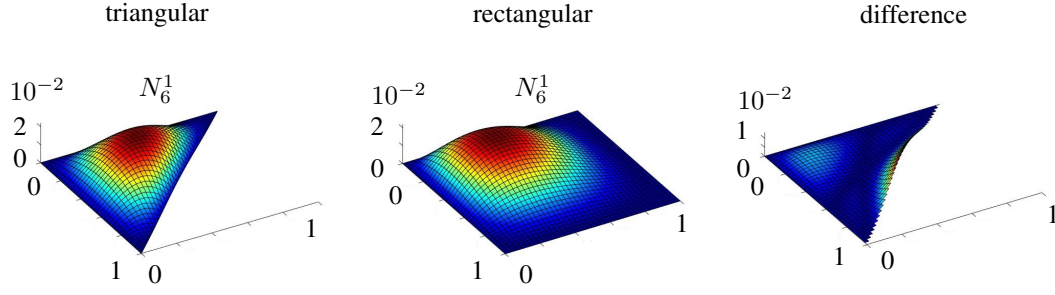
Figure 3.18: The sixth shape function for the first node for the newly developed 18-DOF triangular element (left column) and for the newly developed 24-DOF rectangular element (middle column), along with the difference of two (right column).
