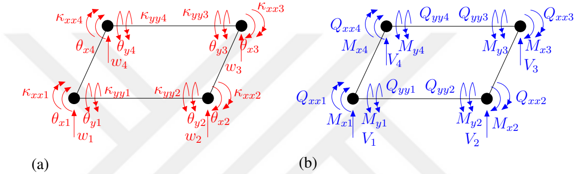
Figure 3.6: (a) Nodal degrees of freedom and (b) corresponding nodal forces for a 20-DOF higher order Kirchhoff-Love plate formulation based on MSGT.
