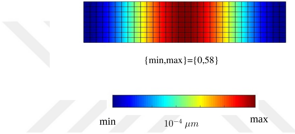
Figure 4.2: Deflection field for the 20 \times 5 \times 1 \mu m plate under a midpoint load F = 1 mN and boundary conditions given in Figure 4.1 with the material properties given as in Table 4.1.
