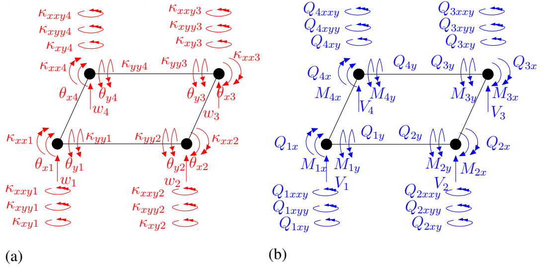
Figure 3.13: (a) Nodal degrees of freedom and (b) corresponding nodal forces for a 32-DOF higher order Kirchhoff-Love plate formulation based on MSGT.
