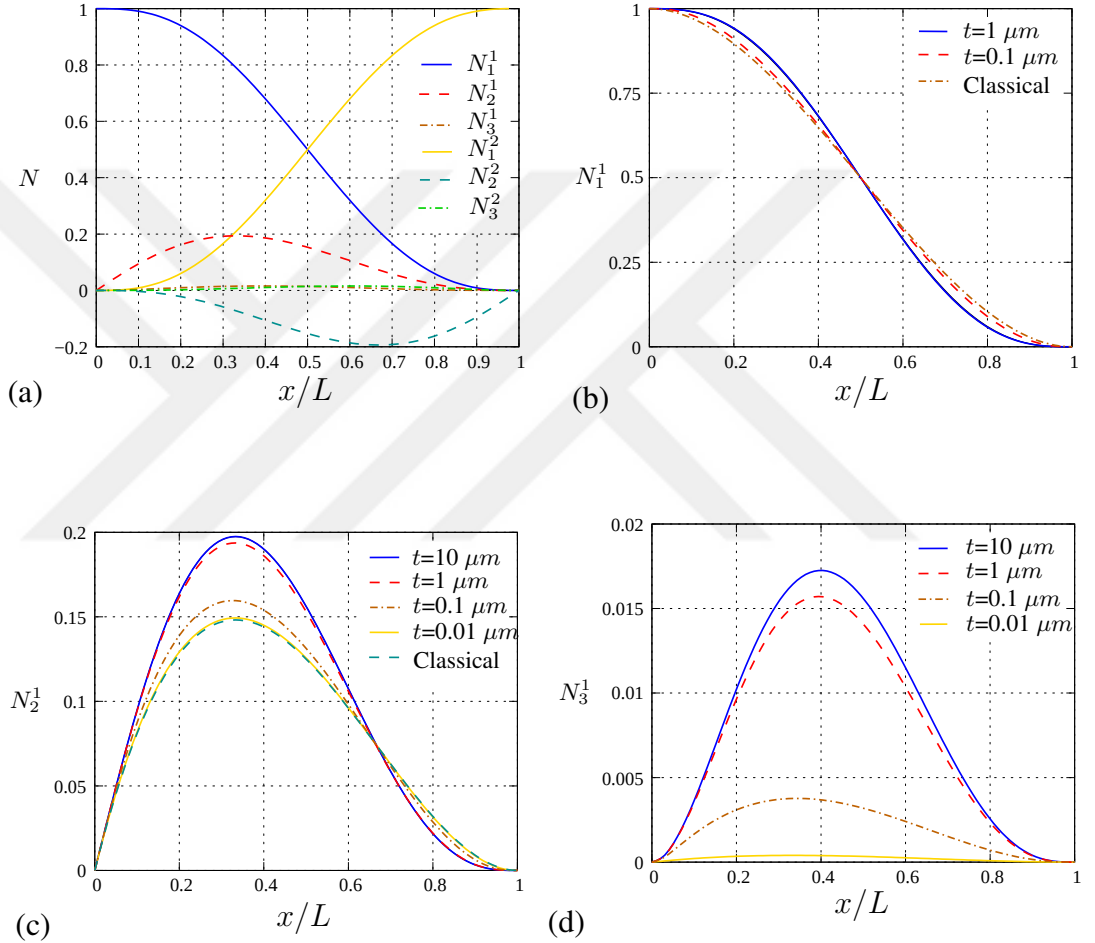
Figure 3.3: Shape functions for MSGT, (a) all elements of shape function matrix N , (b) N_1^1 , (c) N_2^1 , and (d) N_3^1 . For (b)-(d), the curves do not change significantly even if h is increased more than those given as the upper bound in the figures. They also approach to classical hermite cubic shape functions with decreasing values of h .
