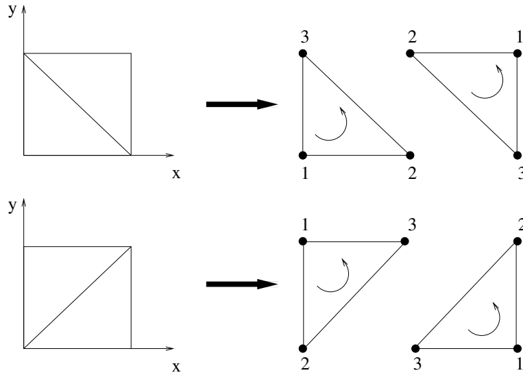
Figure 4.22: Node numbering convention for triangular elements in different orientations.
