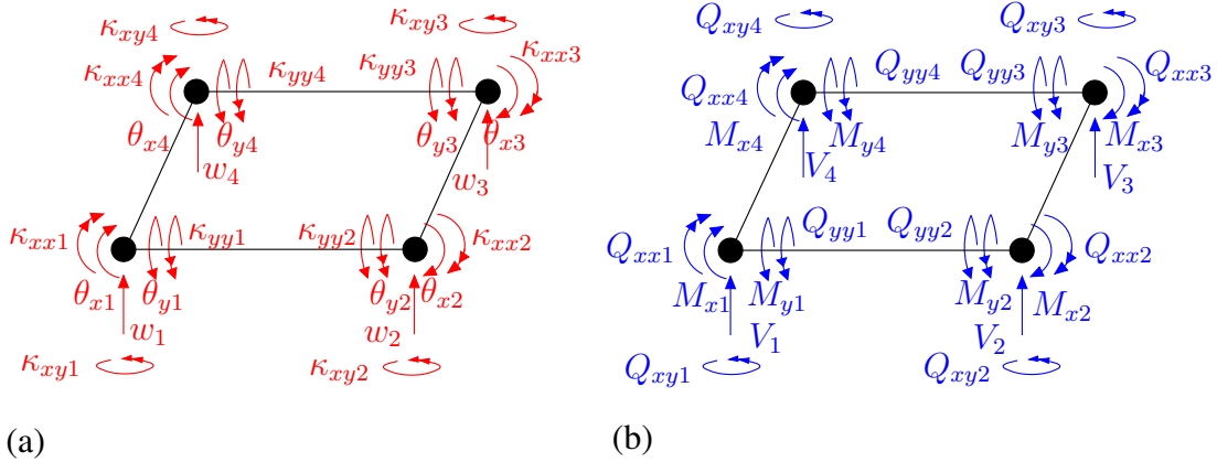
Figure 3.10: (a) Nodal degrees of freedom and (b) corresponding nodal forces for a 24-DOF higher order Kirchhoff-Love plate formulation based on MSGT.
