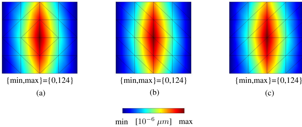
Figure 4.23: Displacement fields for different mesh orientations for triangular elements.
