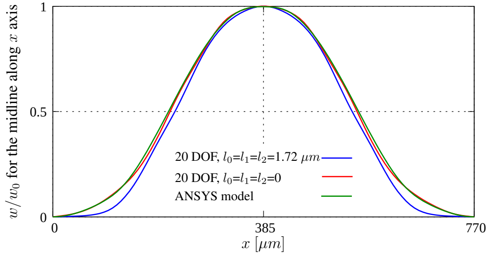
Figure 4.30: Displacement profiles for different models, normalized by dividing to the maximum displacement (of the midnode).
