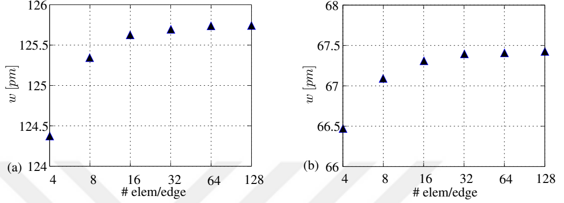
Figure 4.21: Refinement results with triangular elements, i.e. midpoint deflections per number of elements for (a) MSGT, fixed-fixed, (b) MSGT, all sides fixed.
