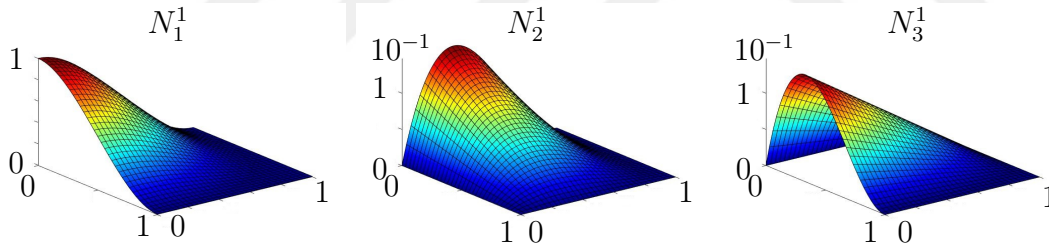
Figure 3.5: 12-DOF element shape functions from N_1 to N_3 .
