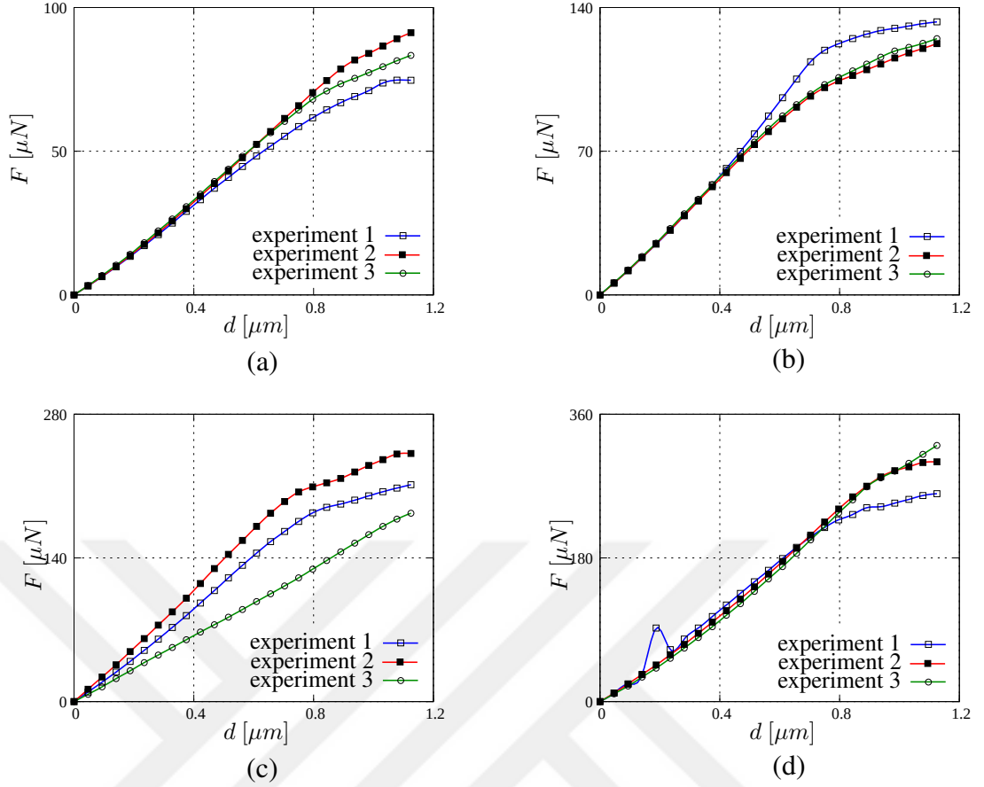
Figure 5.2: Force-displacement data from conducted experiments for (a) specimen 1, (b) specimen 2, (c) specimen 3, (d) specimen 4, per Table 5.1
