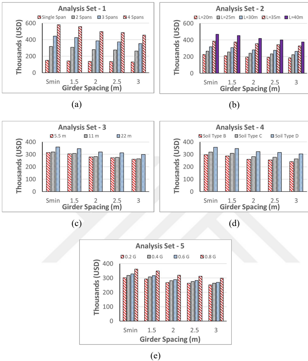
Figure 5.1. Comparison of construction costs
