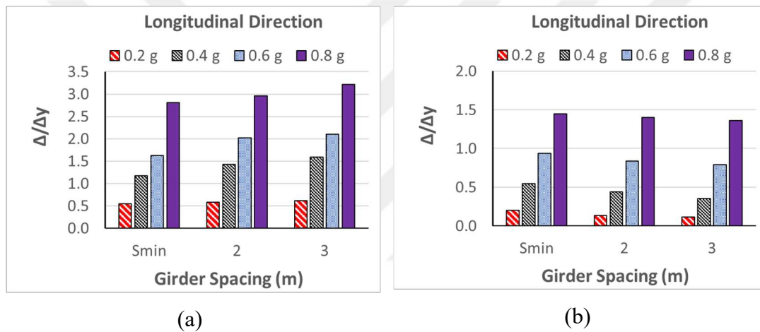
Figure 6.10. Girder spacing versus peak ground acceleration for (a) tension-controlled column section (b) compression-controlled column section
