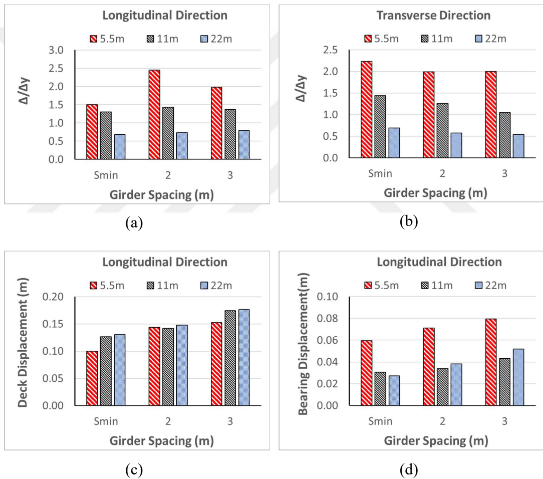
Figure 6.9. Ductility ratio ( \Delta/\Delta_y ) versus girder spacing (a) in the longitudinal direction, (b) in the transverse direction, (c) deck displacement in the longitudinal direction versus girder spacing, (d) bearing displacement in the longitudinal direction for different values of column heights
