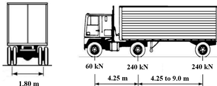
Figure 3.1. H30-S24 Truck
