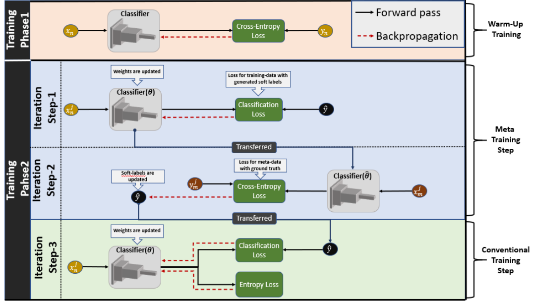
Figure 5.1: The overall framework of the proposed algorithm. x_n, y_n represents the training data and label pair. x_n^j, y_n^j represents batches of training data and label pair. x_m^j, y_m^j represents batches of meta-data and label pair. \hat{y} represents generated soft-labels. The training consists of two phases. In the first phase (warm-up training), the base classifier is trained on noisy data with the conventional cross-entropy loss. This is useful to provide a stable starting point for the second phase. Training phase-2 consists of 3 consecutive steps, which are repeated for each batch of data. In the first iteration step, classification loss for model predictions is calculated with generated soft labels. Then, updated classifier parameters \hat{\theta} are calculated by SGD. In the second iteration step, the cross-entropy loss for meta-data is calculated using the updated classifier parameters \hat{\theta} . Then, soft-labels are updated by taking an SGD step on this cross-entropy loss. In the third iteration step, the classifier parameters \theta are updated by the classification loss (with newly generated soft labels) and entropy loss.
