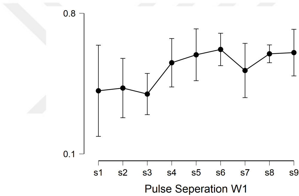
Figure 3.8: Graph for average correlation values for different separations between 1 bit wide pulses, overall subjects.
