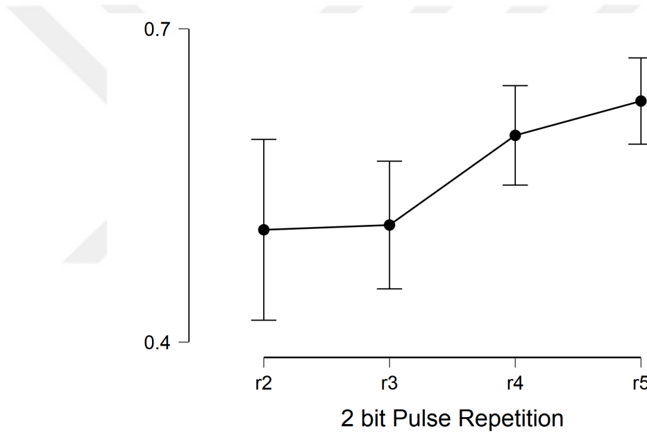
Figure 3.14: Graph for average correlation values for different repetitions of 2 bit wide pulse, overall subjects.
