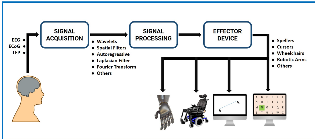
Figure 1.1: Flow diagram of a general BCI system
