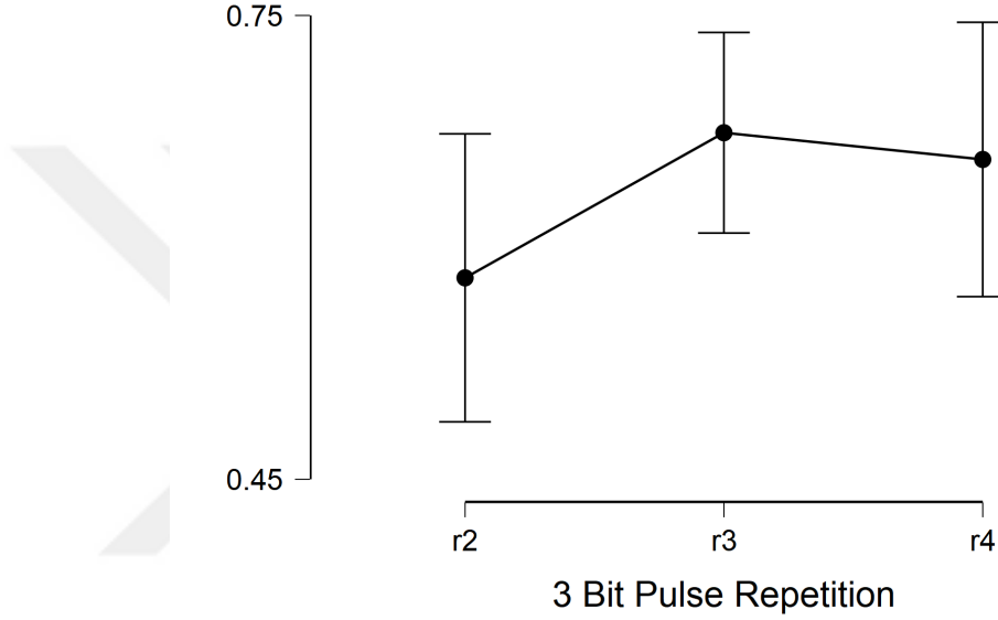
Figure 3.16: Graph for average correlation values for different repetitions of 3 bit wide pulse, overall subjects.
