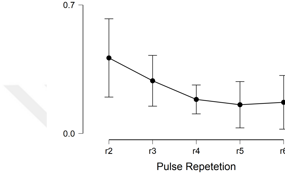
Figure 3.12: Graph for average correlation values for different repetitions of 1 bit wide pulse, overall subjects.
