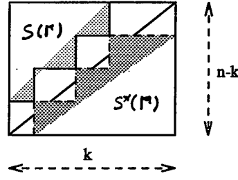
Figure 4.1: S^*(\Gamma)
