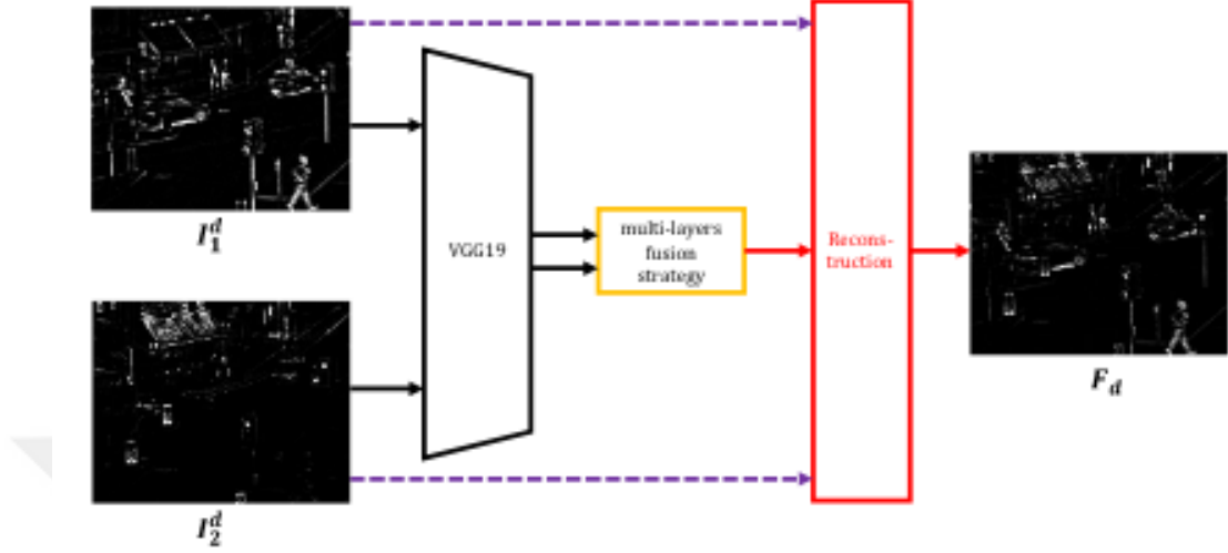
Figure 3.25: The procedure of detail content fusion taken from [22]
