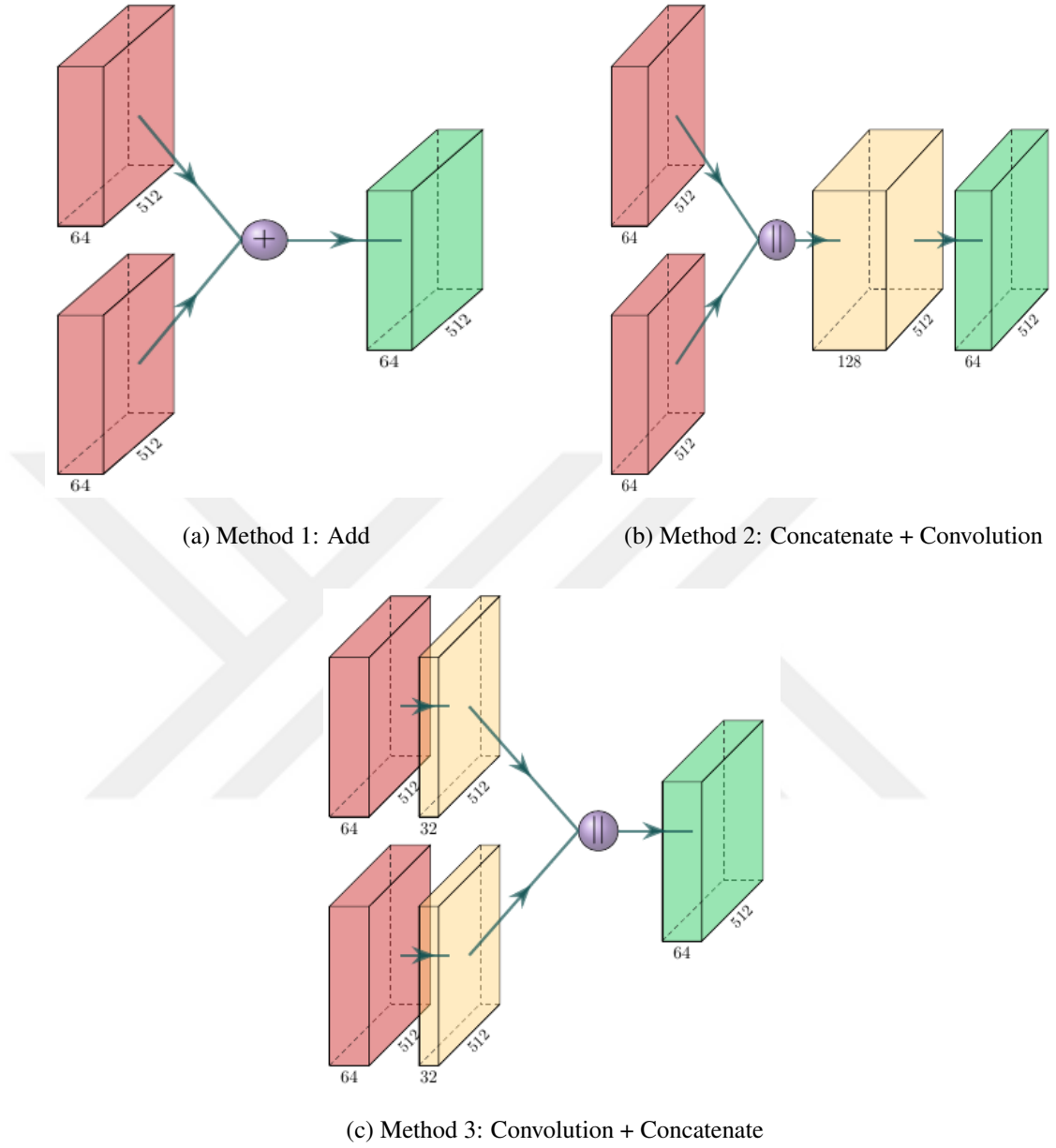
Figure 4.5: Fusion method visualizations. Yellow boxes are the result of the convolution layer. Green boxes are the results of the fusion layer. Red boxes are the inputs that came from encoder layers. Purple circles define the operation used. '+' means element-wise adding while '||' means concatenation in channel dimension.
