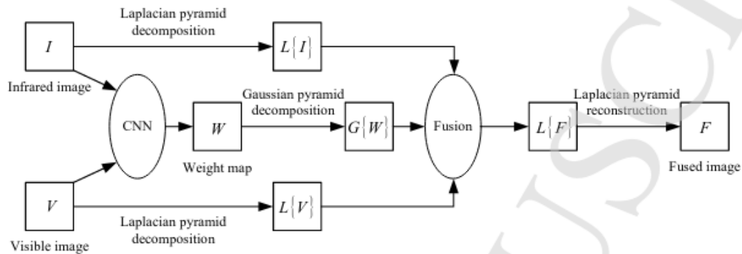
Figure 3.22: The schematic diagram of proposed CNN method taken from [21]
