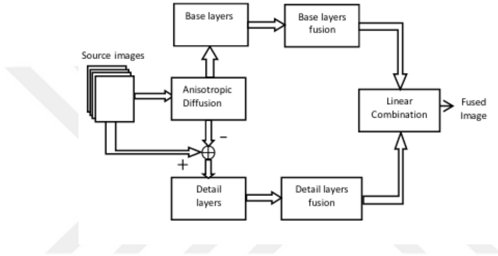
Figure 3.2: Proposed ADF Method taken from [6]
