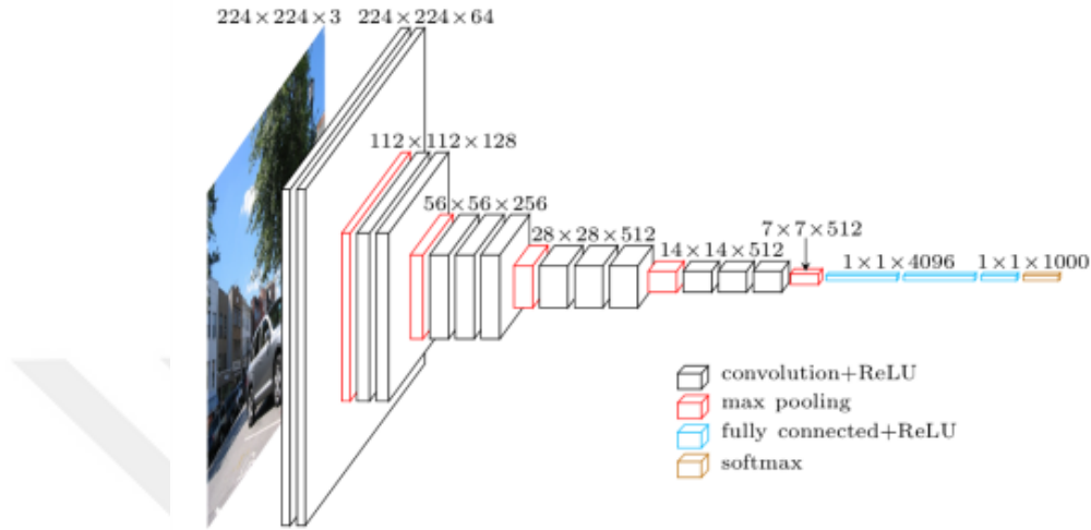
Figure 2.2: VGG-16 architecture taken from [33].
