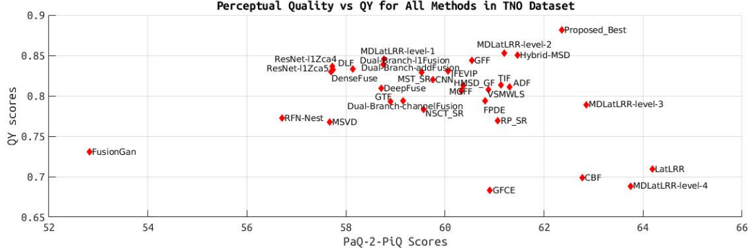
(c) Perceptual quality vs Q_Y score graph.
