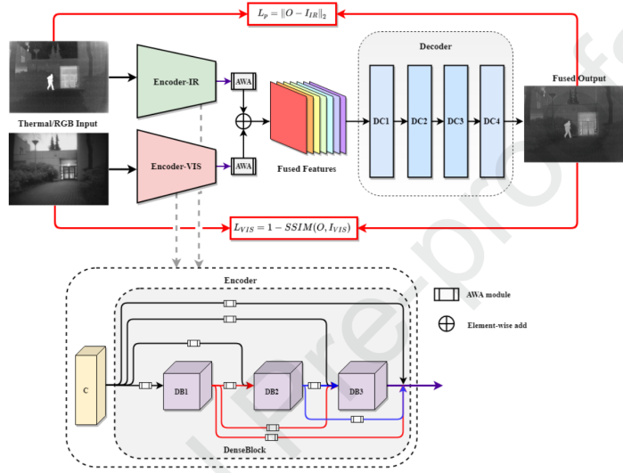
Figure 3.39: The overall architecture of TFSNet method. Image is taken from [29].
