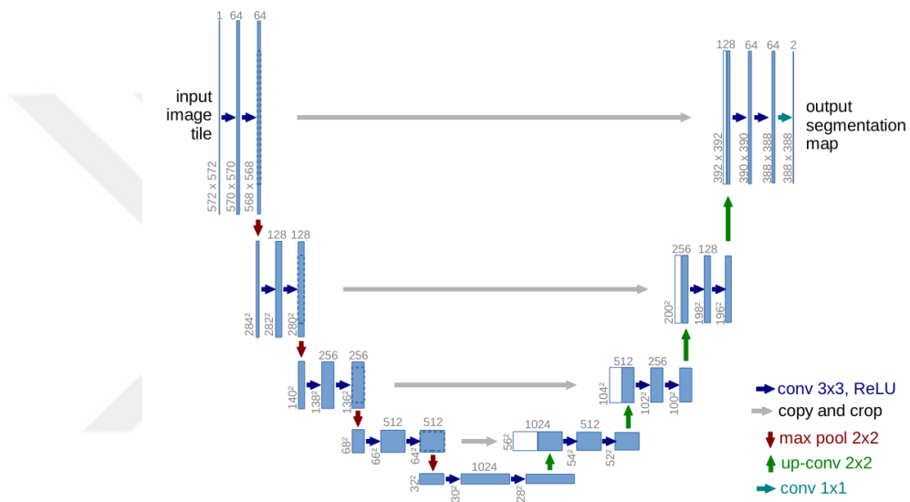
Figure 2.4: U-Net architecture. Gray arrows show skip connections of the architecture. The number of channels is denoted on top of the boxes. Image taken from [1].
