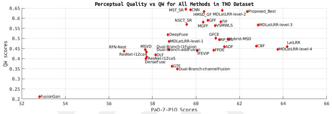
(b) Perceptual quality vs Q_W score graph.
