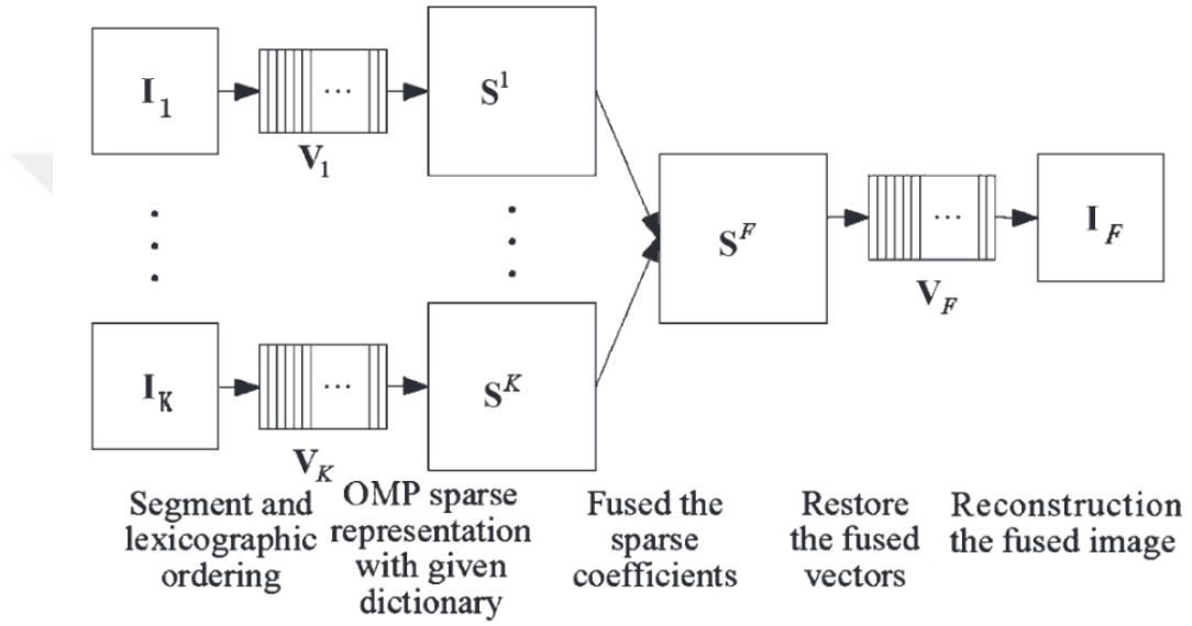
Figure 3.14: Overall architecture of SR method taken from [14]
