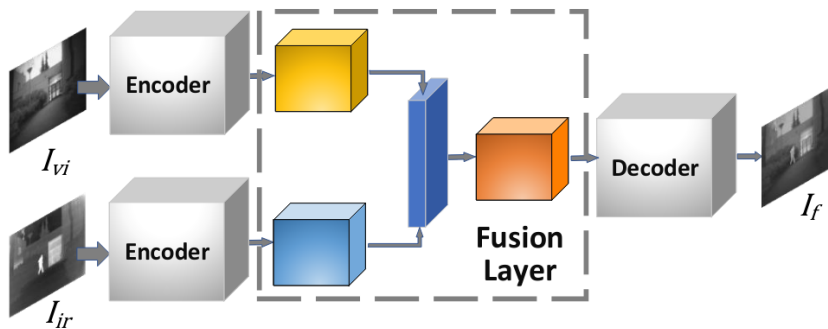
Figure 3.37: The architecture of the Dual-Branch method in the inference phase. Image is taken from [28]
