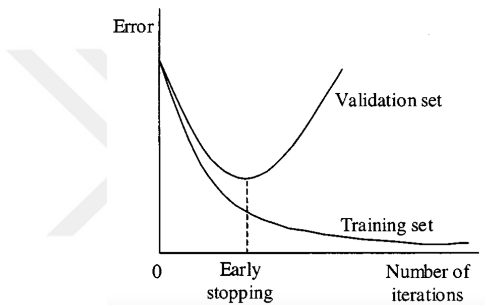
Figure A.6: Loss curves of the artificial neural network. This shows that from a point validation loss started to increase even if training loss continues to decrease.
