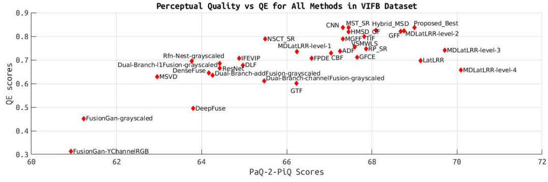
(a) Perceptual quality with Q_E score graph.
