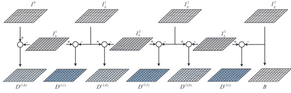
Figure 3.4: Construction of three level decomposition taken from [8]
