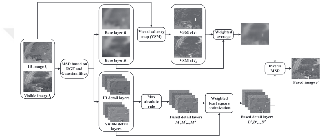
Figure 3.21: The schematic diagram of proposed VSMWLS method taken from [20]
