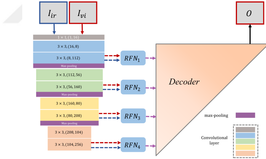
Figure 3.33: The overall architecture of the proposed method taken from [27]
