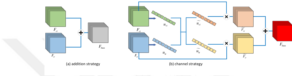
Figure 3.38: The fusion strategies of the Dual-Branch method. Image is taken from [28]
