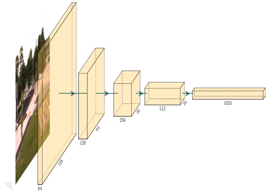
Figure 4.3: Basic encoder architecture. Includes only convolution layers.
