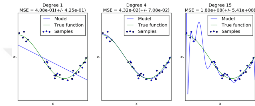
Figure A.4: Demonstration of underfitting, correct fit and overfitting from left to right respectively . It is taken from [46]
