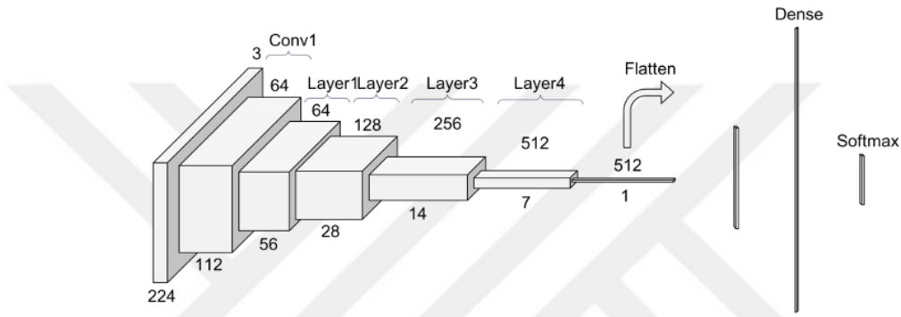
Figure 4.4: ResNet 34 architecture. Image is taken from [41]
