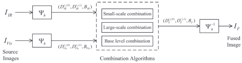
Figure 3.5: Proposed Hybrid_MSD Method taken from [8]
