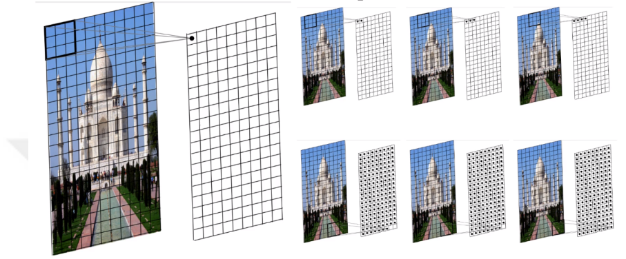
Figure 2.1: Convolution operation on an image. Image taken from [32]
