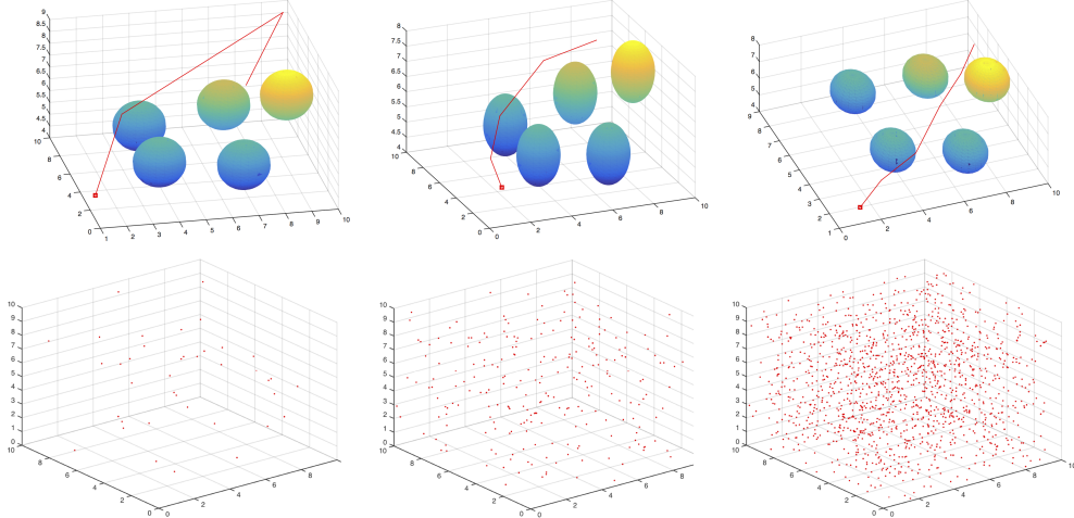
Figure 6.4 : Pseudo-random sampling and asymptotic convergence in RRT^* with 40, 120 and 400 samples
