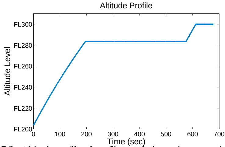
Figure 7.8 : Altitude profile of conflict resolution trajectory to the Scenario 2
