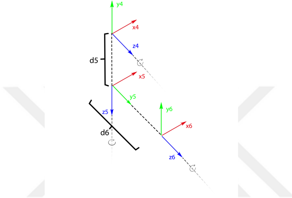
Figure 3.1: Collaborative UR5 robot last three joint frames
