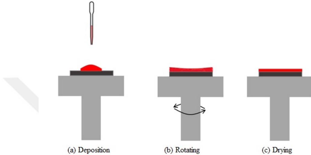
Figure 2.7: Stages in thin-film deposition using spin-coating.
