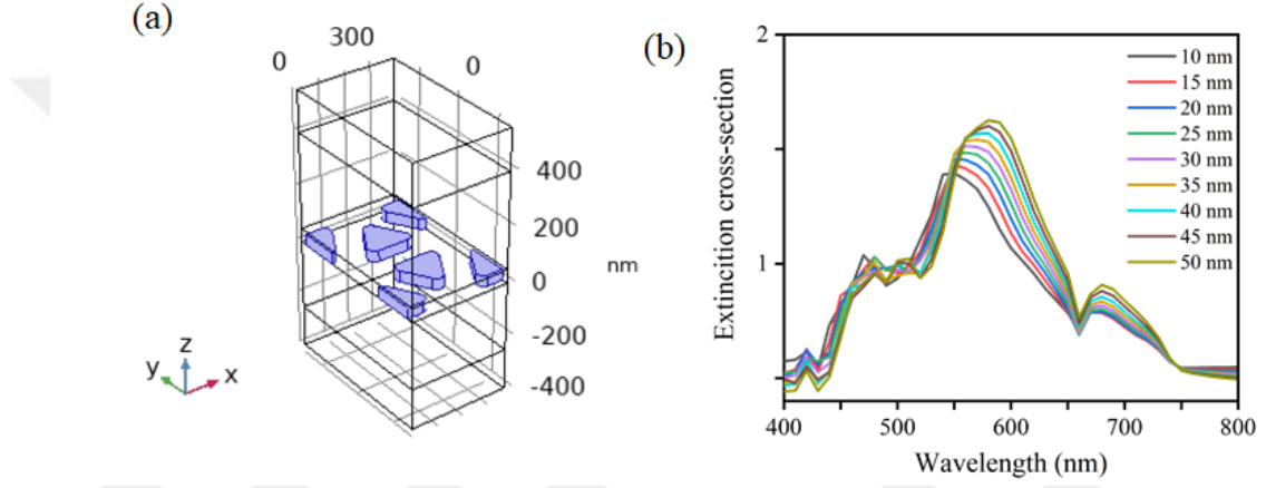
Figure 5.21: (a) Schematic illustration of the simulation setup used for finding the optical cross-sections of Ag nanoprism arrays. (b) Extinction cross-section of the Ag/substrate system with \text{SiO}_2 dielectric spacer on top.
