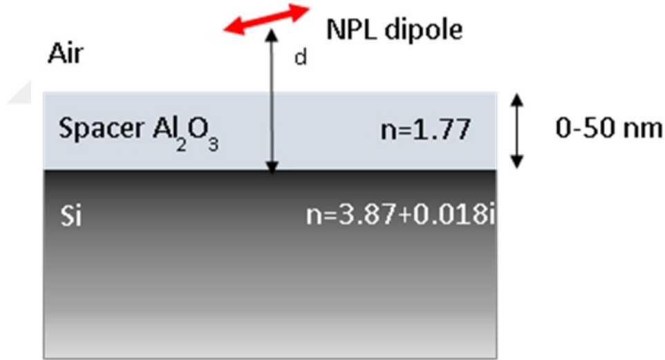
Figure 4.10: Cross-sectional diagram of the hybrid NPL- \text{Al}_2\text{O}_3 -Si system for rate modification calculations.
