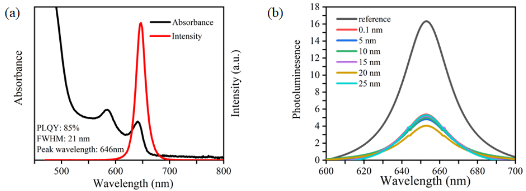
Figure 5.8: (a) Absorption and PL spectra of CdSe/CdZnS NPLs. (b) PL spectra of solid films of the NPLs-Au assembly with varying thicknesses of the Al 2 O 3 separation layer.
