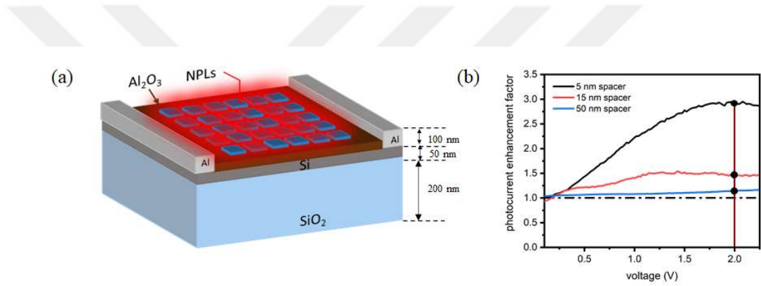
Figure 4.12: (a) Schematic of our proof-of-concept device. b) Photocurrent enhancement due to the presence of NPLs atop an ultrathin Si photodetector with respect to the negative control group device with no NPLs. Photocurrent enhancement factor as a result of the NPL deposition for the spacer thicknesses of 5, 15, and 50 nm. Reproduced with permission from Ref. [83] Copyright 2021, Wiley.
