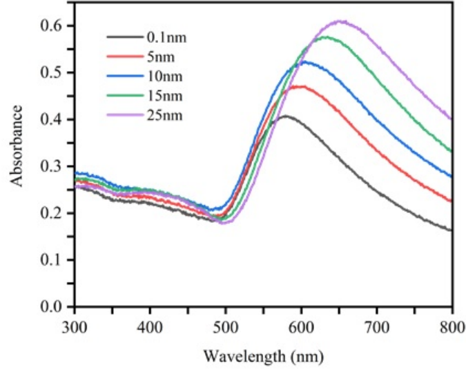
Figure 5.4: Absorption spectra of thermally evaporated Au films with initial mass-thickness of 8 nm, annealed at 650 °C for 3 minutes, followed by \text{Al}_2\text{O}_3 deposition of varying thicknesses using ALD at 200 °C.
