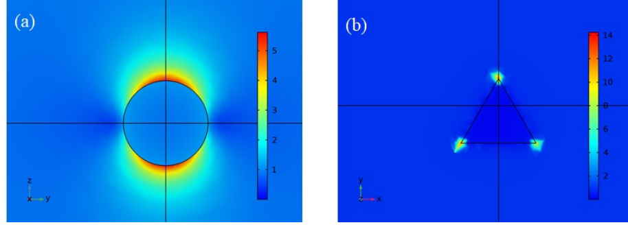
Figure 2.14: Plasmonic hotspots around the MNPs of different shapes (a) Spherical NP and (b) Metal nanoprism.
