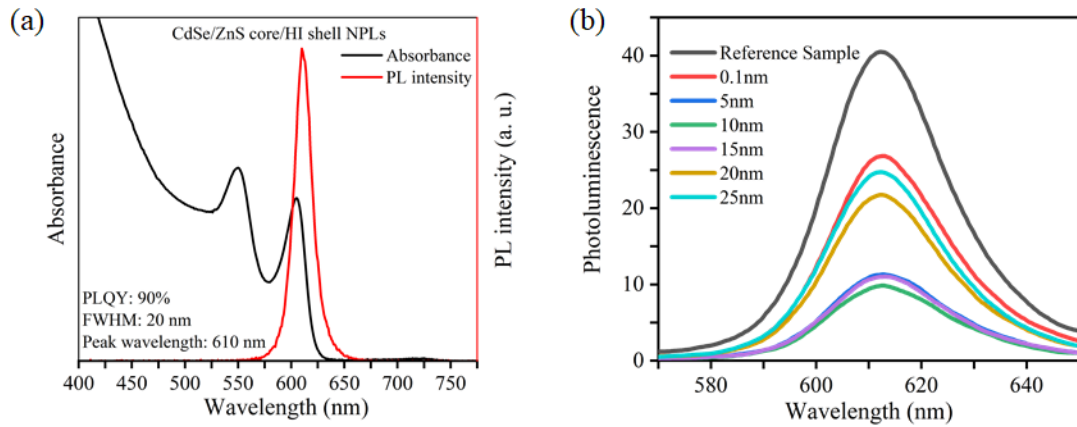
Figure 5.6: (a) Absorption and photoluminescence (PL) spectra of CdSe/ZnS NPLs. (b) PL spectra of solid films of the NPLs-Au assembly with varying thicknesses of the \text{Al}_2\text{O}_3 separation layer.
