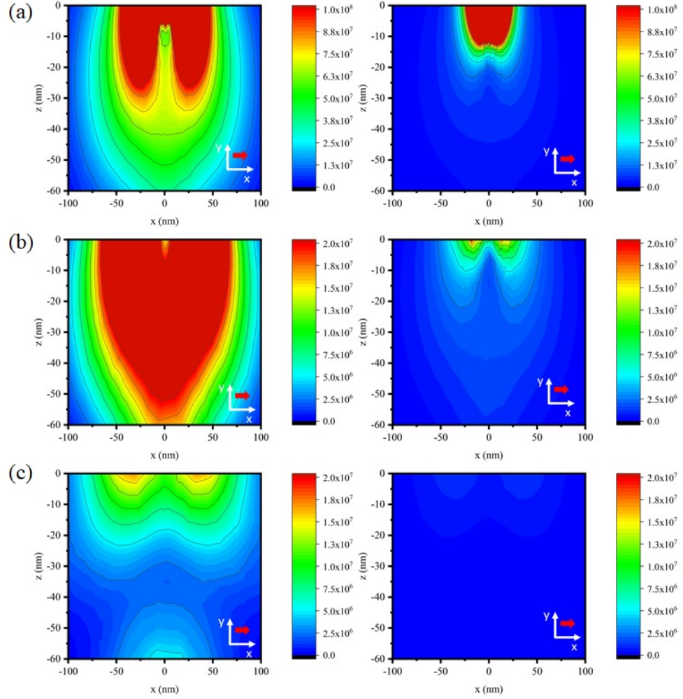
Figure 4.8: Electric field intensity distribution on the xz -plane ( y = 0 ) within silicon region for 4 uniformly distributed dipoles present, when oriented in the plane (left column), with that of single dipole oriented in-plane (right column) with \text{Al}_2\text{O}_3 spacer thickness of (a) 2 nm, (b) 20 nm, and (c) 50 nm. Reproduced with permission from Ref. [83] Copyright 2021, Wiley.
