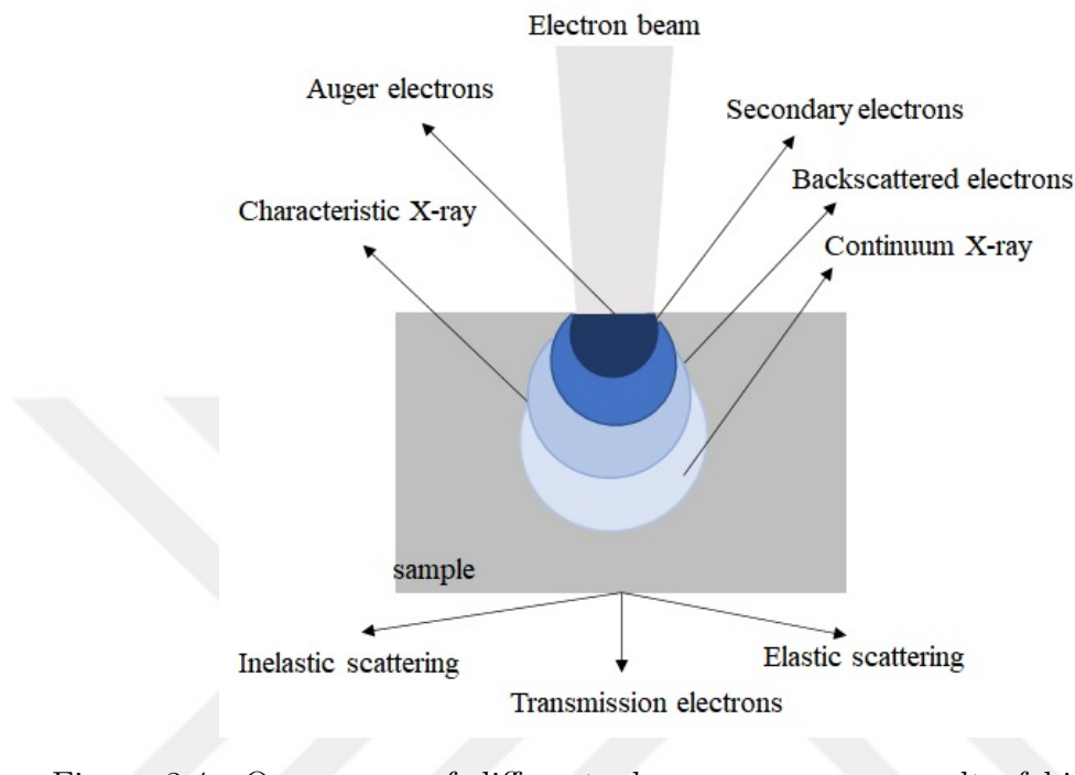
Figure 3.4: Occurrence of different phenomenon as a result of high energetic electron beam interacting with the sample material.
