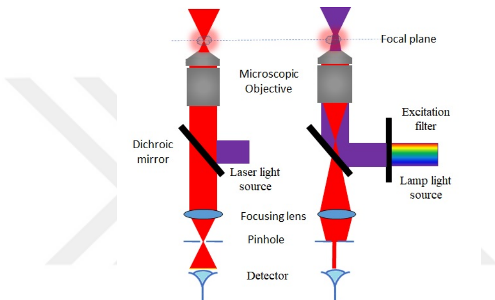
Figure 3.5: Illustration of spot size on the focal plane (a) confocal microscopy and (b) conventional microscopy.
