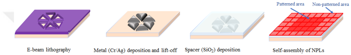
Figure 5.16: Steps involved in forming NPL/Au hybrid structure using EBL technique.
