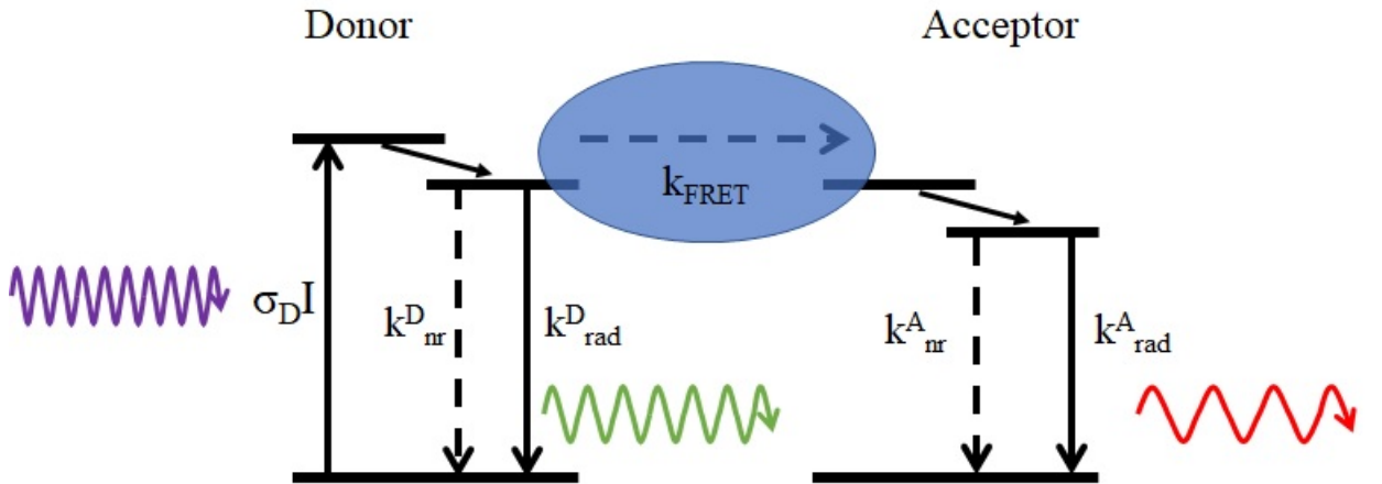
Figure 2.10: FRET: an additional pathway between a donor and an acceptor for energy transfer.
