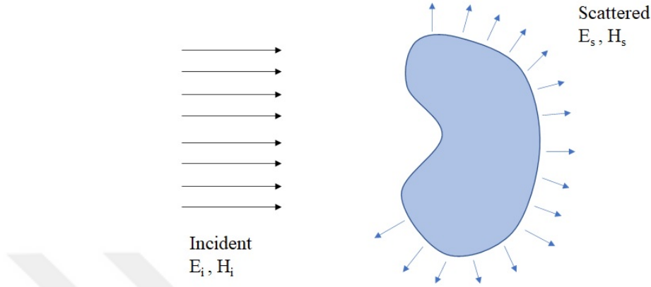
Figure 2.20: Scattering of EM field by an obstacle in response to the incident EM wave.
