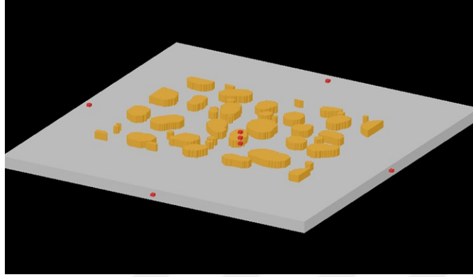
Figure 5.18: Perspective view of the Au nano-island/quartz structure.
