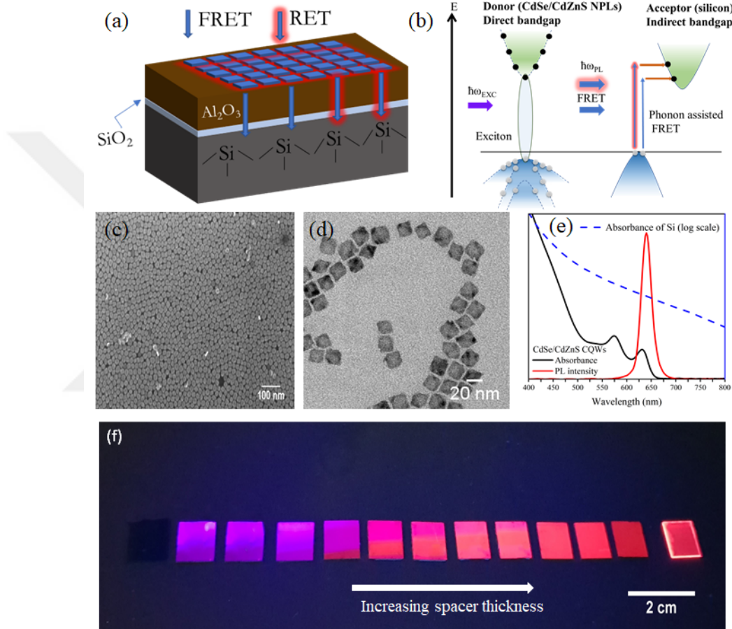
Figure 4.1: (a) Schematic depiction of our hybrid NPL-Al 2 O 3 -Si system. (b) Energy band diagram illustrating the energy transfer from NPLs to crystalline silicon. (c) Scanning electron microscopy image of self-assembled NPLs on the silicon substrate. (d) Transmission electron microscopy image of CdSe/CdZnS core/shell NPLs. (e) Normalized photoluminescence and UV-VIS absorption spectra of CdSe/CdZnS core/hot-injection grown shell NPLs (donor) and absorption spectrum of silicon. (f) Photography of the samples illuminated by a 365 nm UV lamp: Samples are placed from left to right in the order of increasing Al 2 O 3 spacer thicknesses. Reproduced with permission from Ref. [83] Copyright 2021, Wiley.
