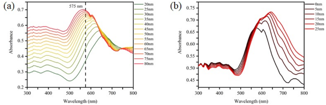
Figure 5.19: (a) Simulated absorption spectra of Au nano-island structure as a function of the height varied from 20 to 80 nm. (b) Simulated absorption spectra of Al 2 O 3 / Au/quartz structure with varying thicknesses of the dielectric spacer.
