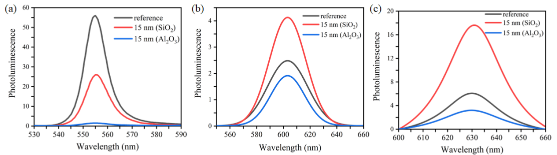
Figure 5.12: PL spectra of solid films of the NPLs-Au assembly with different heterostructures of NPLs (a) 5 ML CdSe core NPLs with an emission peak at 555 nm, (b) CdSe/CdS 4 ML / 1 ML shell NPLs with an emission peak at 602 nm, and (c) CdSe/CdS 4 ML / 2 ML shell NPLs with an emission peak at 628 nm.
