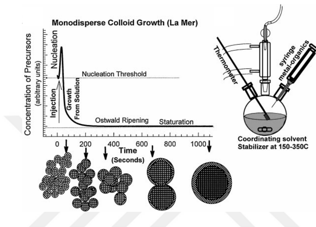
Figure 2.3. The nucleation and growth model describing colloidal synthesis of highly monodisperse NCs proposed by La Mer together with schematic drawing of a typical colloidal synthesis setup. Reprinted with permission from [27].
