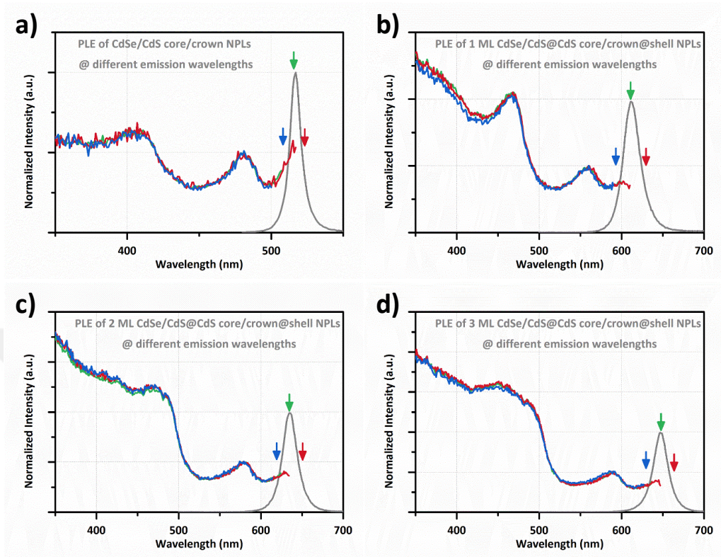
Figure 4.6. Photoluminescence excitation spectra of (a) CdSe/CdS core/crown NPLs having medium crown size and CdSe/CdS@CdS core/crown@shell NPLs having (b) 1 ML CdS shell, (c) 2 ML CdS shell and (d) 3 ML CdS shell taken at different emission wavelengths. Reprinted with permission from [94]. Copyright 2016 WILEY-VCH Verlag GmbH & Co. KGaA, Weinheim.
