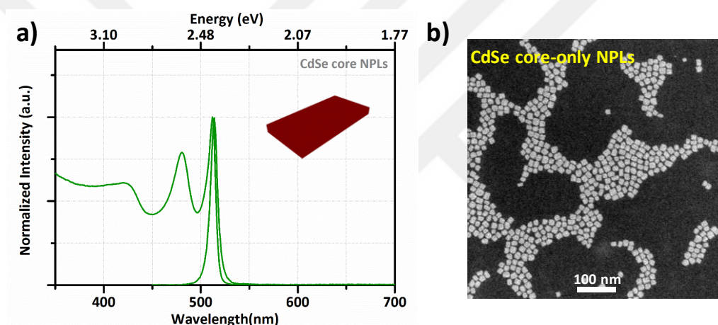
Figure 4.1. (a) Normalized absorption and photoluminescence spectra of CdSe core-only NPLs and (b) HAADF-STEM image of CdSe core-only NPLs. Reprinted with permission from [94]. Copyright 2016 WILEY-VCH Verlag GmbH & Co. KGaA, Weinheim.
