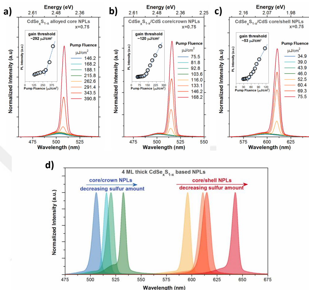
Figure 5.7. Optical gain performances of CdSe x S 1-x /CdS core/crown and core/shell NPLs having different sulfur compositions. As an exemplary case for x = 0.75 amplified spontaneous emission spectra of (a) CdSe x S 1-x core-only NPLs, (b) CdSe x S 1-x /CdS core/crown NPLs, (c) CdSe x S 1-x /CdS core/shell NPLs having 2 ML CdS shell at different excitation fluence. In the insets, the integrated PL intensity are given as a function of the pump fluence. (d) Normalized ASE spectra of CdSe x S 1-x /CdS heterostructures showing highly tunable gain performance varying with the incorporated sulfur amount. Reprinted with permission from [112]. Copyright 2017 American Chemical Society.
