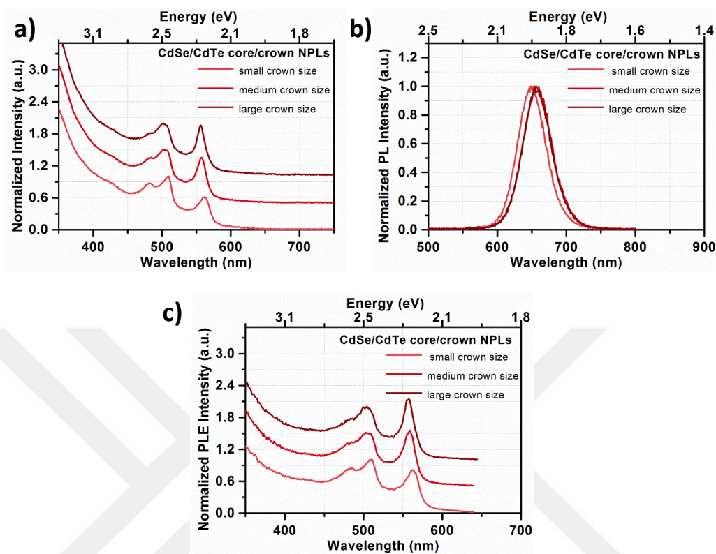
Figure 7.2. (a) Normalized absorption, (b) photoluminescence and (c) photoluminescence excitation spectra of CdSe/CdTe core/crown NPLs having different CdTe crown size. Reprinted with permission from [93]. Copyright 2017 American Chemical Society.
