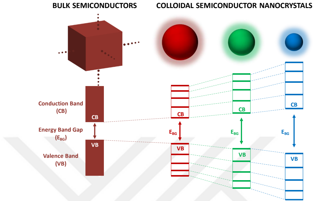
Figure 2.1. Schematic illustration of band diagrams in bulk semiconductors and colloidal semiconductor NCs. While continuous band diagrams are observed in the bulk semiconductors, colloidal semiconductor NCs exhibit quantized energy levels in their band structure. Also, with decreasing the size of the colloidal semiconductor NCs, their effective band gap energy is increased.
