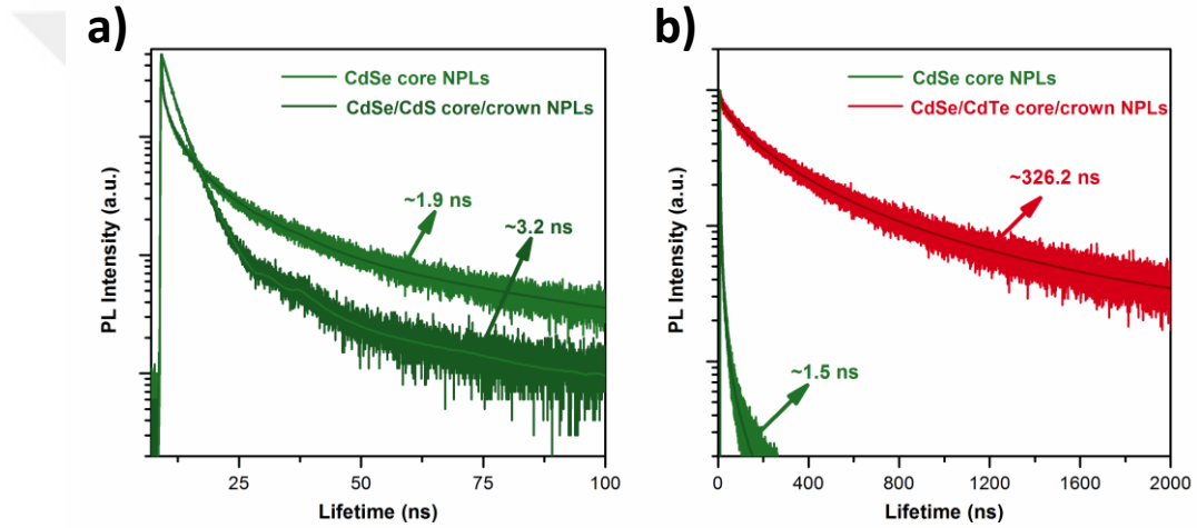
Figure 3.7. Time-resolved fluorescence decays curves of (a) CdSe core and CdSe/CdS core/crown NPLs having Type-I electronic structure and (b) CdSe core and CdSe/CdTe core/crown NPLs having Type-II electronic structure. These core and core/crown heterostructured NPLs were synthesized at our laboratories.
