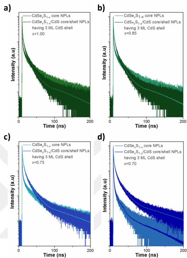
Figure 5.6. Time-resolved fluorescence decay curves of \text{CdSe}_x\text{S}_{1-x}/\text{CdS} core/shell NPLs having 3 ML CdS shell together with their core for the case of (a) x = 1.00 , (b) x = 0.85 , (c) x = 0.75 , and (d) x = 0.70 . Reprinted with permission from [112]. Copyright 2017 American Chemical Society.
