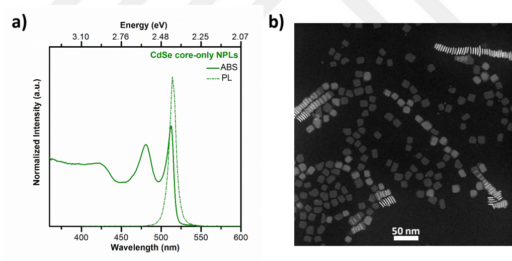
Figure 7.1. (a) Absorption (solid line) and photoluminescence (dotted–dashed line) spectra and (b) HAADF-STEM images of the 4 ML thick CdSe core-only NPLs dissolved in hexane at room temperature, having a lateral size of 16.4 \pm 1.7 nm by 12.6
