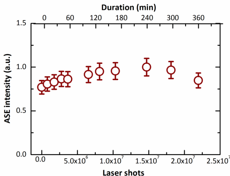
Figure 4.10. Intensity of the amplified spontaneous emission in the core/crown@shell NPLs as a function of pump laser shots (per pulse energy density of 35 \mu\text{J}/\text{cm}^2 ). The optical gain in the core/crown@shell NPLs is highly stable even for 6 h of continuous excitation. Reprinted with permission from [94]. Copyright 2016 WILEY-VCH Verlag GmbH & Co. KGaA, Weinheim.
