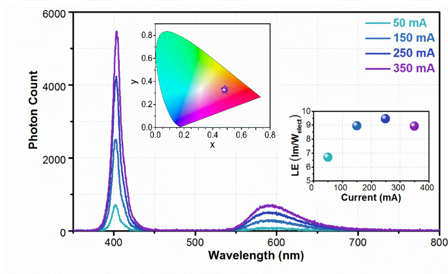
Figure 7.10. Emission spectra of the NPL-integrated LED at varying currents along with luminous efficiency (LE) (inset, right) and CIE 1931 color coordinates (inset, left). Reprinted with permission from [93]. Copyright 2017 American Chemical Society.
