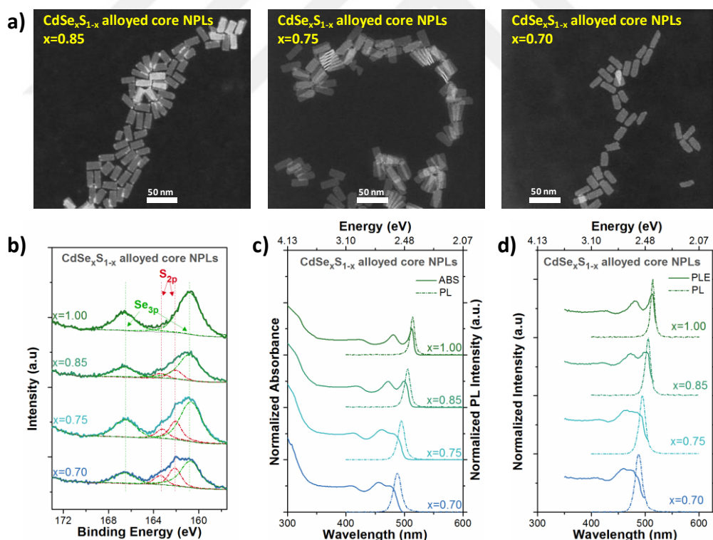
Figure 5.1. (a) HAADF-STEM images of \text{CdSe}_x\text{S}_{1-x} alloyed core NPLs having different sulfur compositions, (b) high-resolution X-ray photoelectron spectra of spin-coated thin
