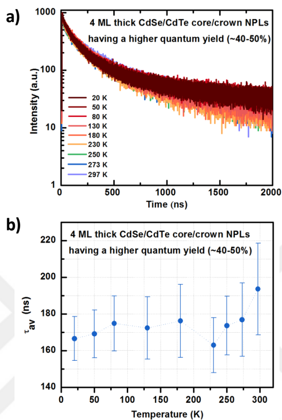
Figure 6.6. (a) Temperature-dependent time-resolved fluorescence decay curves of the CdSe/CdTe core/crown NPLs having a higher PL-QY and (b) their amplitude-averaged fluorescence lifetime. Reprinted with permission from [95]. Copyright 2015 American Chemical Society.
