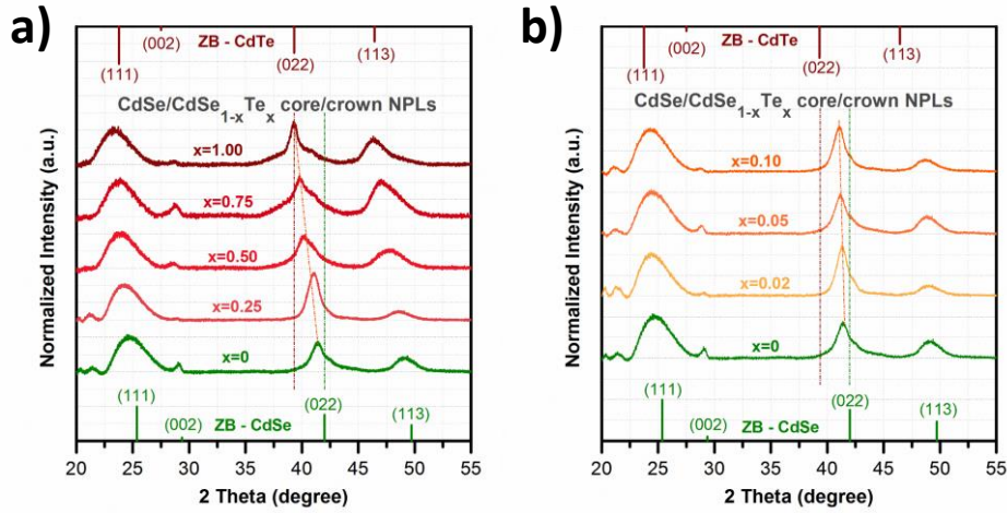
Figure 7.6. X-ray diffraction patterns of the 4 ML thick CdSe core-only NPLs and the CdSe/CdSe 1-x Te x core/crown NPLs having different crown compositions. The green (on the bottom) and the brown bars (on the top) show the diffraction peaks of the bulk CdSe
