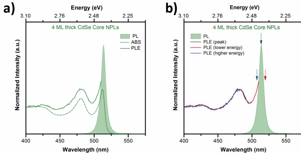
Figure 3.4. (a) Normalized photoluminescence and photoluminescence excitation spectra of our 4 ML thick CdSe core NPLs together with their absorption spectra. (b)
