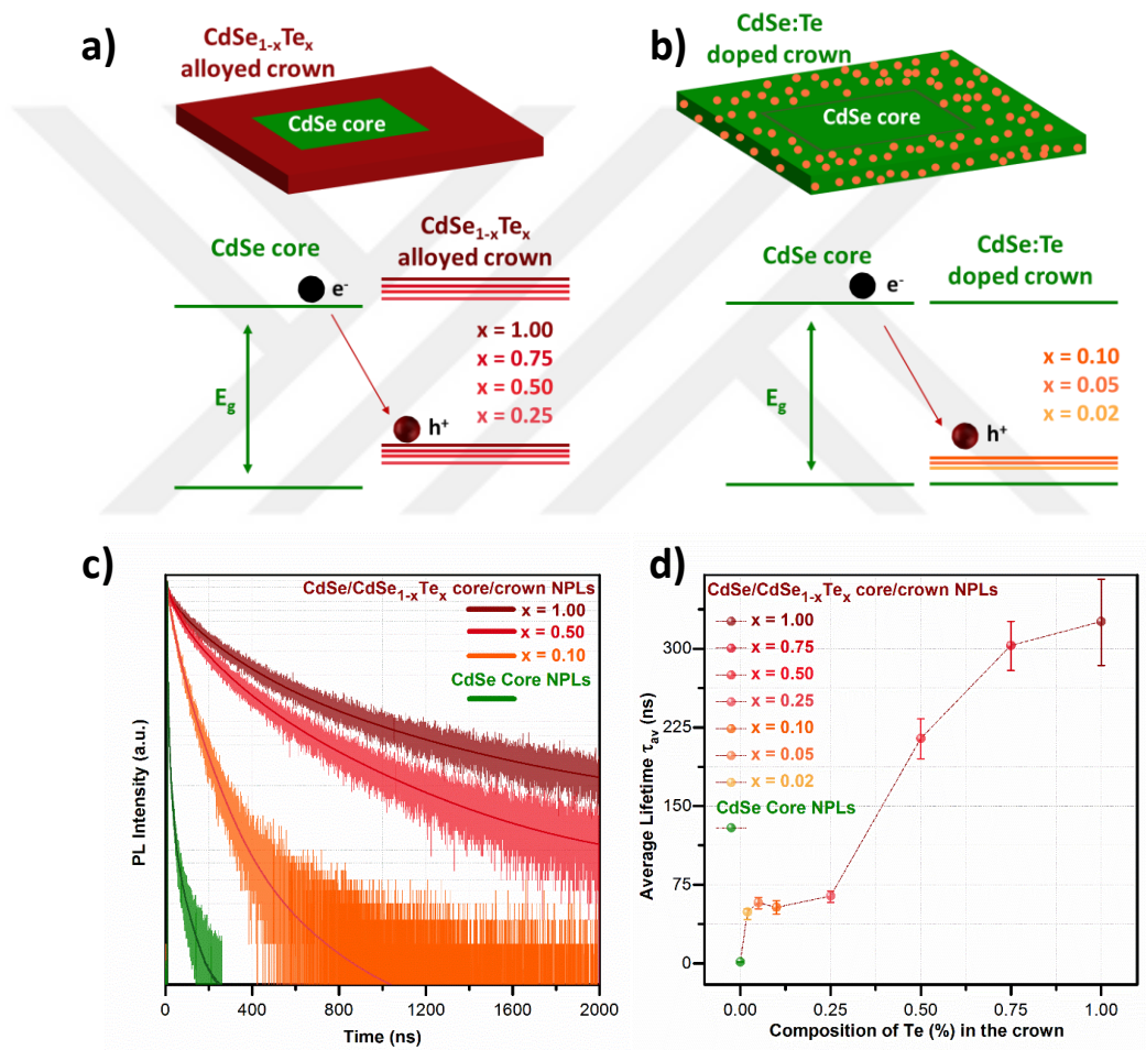
Figure 7.9. Schematic demonstration of band diagrams of the CdSe/CdSe 1-x Te x core/crown NPLs (a) for x \geq 0.25 , and (b) for x \leq 0.10 . (c) Time-resolved fluorescence decay curves of the CdSe core and CdSe/CdSe 1-x Te x core/crown NPLs for different crown region compositions (e.g., x = 1.00 , 0.50 , and 0.10 ). The solid lines on the decay
