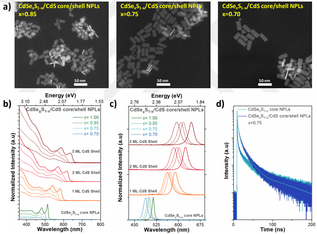
Figure 5.5. (a) HAADF-STEM images of \text{CdSe}_x\text{S}_{1-x}/\text{CdS} core/shell NPLs having 3 ML CdS shell thicknesses, (b) normalized absorbance spectra of \text{CdSe}_x\text{S}_{1-x}/\text{CdS} core/shell NPLs with different sulfur composition and CdS shell thicknesses, (c) PL spectra of \text{CdSe}_x\text{S}_{1-x}/\text{CdS} core/shell NPLs with varying sulfur composition and CdS shell thicknesses, and (d) time-resolved fluorescence decay curves of \text{CdSe}_x\text{S}_{1-x} alloyed core
