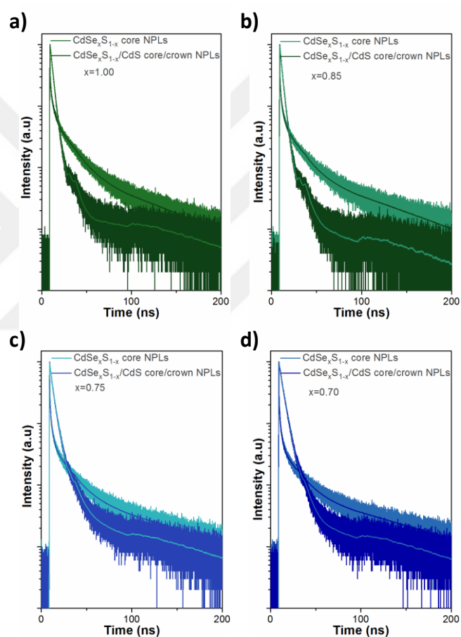
Figure 5.4. Time-resolved fluorescence decay curves of \text{CdSe}_x\text{S}_{1-x}/\text{CdS} core/crown NPLs together with their core for the case of (a) x = 1.00 , (b) x = 0.85 , (c) x = 0.75 and (d) x = 0.70 . Reprinted with permission from [112]. Copyright 2017 American Chemical Society.
