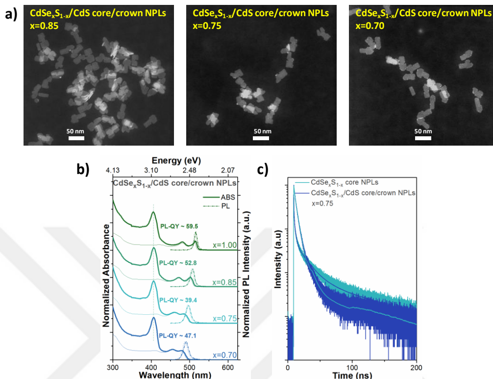
Figure 5.3. (a) HAADF-STEM images of CdSe x S 1-x /CdS alloyed core/crown NPLs having different sulfur compositions, (b) normalized absorbance and photoluminescence spectra of CdSe x S 1-x /CdS core/crown NPLs and (c) time-resolved fluorescence decay curves of CdSe x S 1-x alloyed core and CdSe x S 1-x /CdS core/crown NPLs for the case of x = 0.75 . Reprinted with permission from [112]. Copyright 2017 American Chemical Society.
