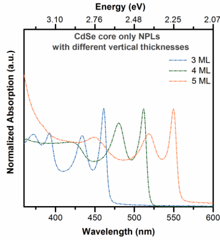
Figure 3.1. Normalized absorption spectra of our CdSe core-only NPLs having different vertical thicknesses, synthesized at our laboratories.
