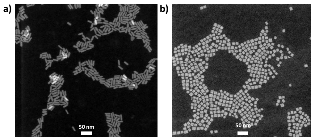
Figure 3.8. HAADF-STEM images of 4 ML thick CdSe core NPLs having (a) rectangular shape and (b) square shape, which were synthesized at our laboratories.
