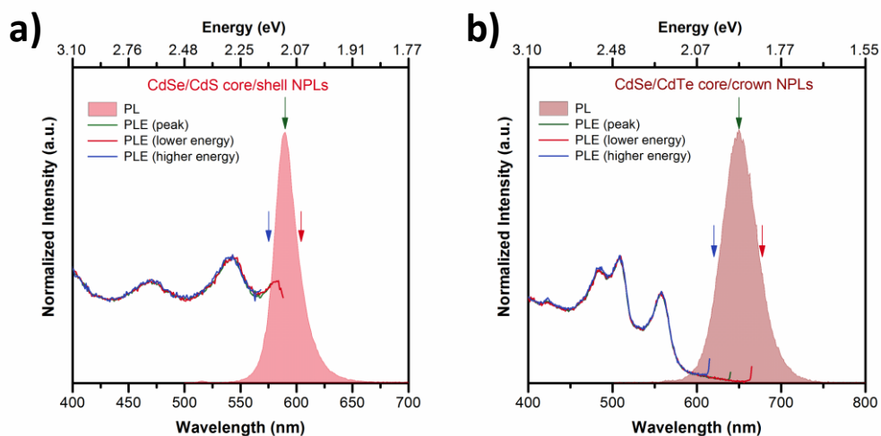
Figure 3.5. Photoluminescence excitation spectra of (a) CdSe/CdS core/shell and (b) CdSe/CdTe core/crown NPLs taken at different emission wavelengths synthesized at our laboratories.
