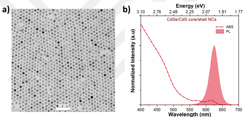
Figure 2.6. (a) High-resolution transmission electron microscopy (TEM) image of our CdSe/CdS core/shell NCs showing highly monodisperse size distribution. (b) Normalized absorption and photoluminescence spectra of our CdSe/CdS core/shell NCs with narrow emission linewidths ( \sim 28 nm).
