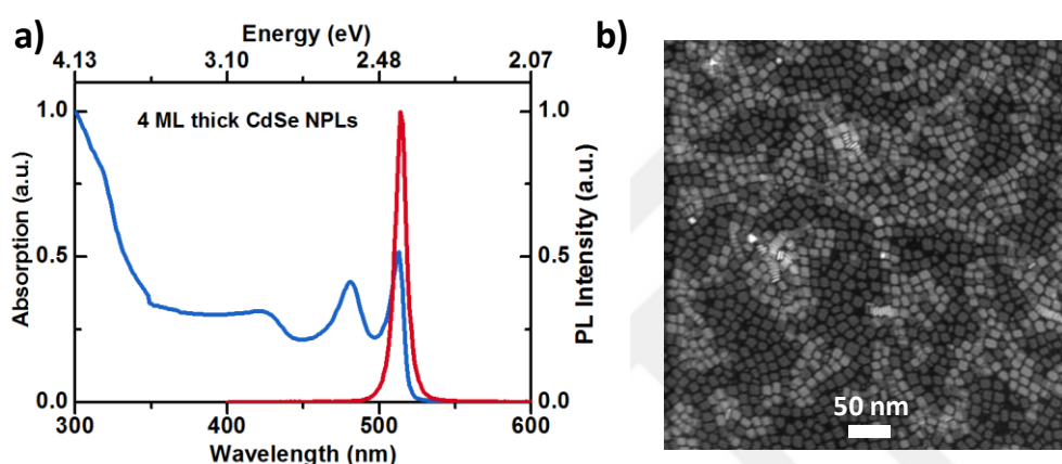
Figure 6.1. (a) Normalized absorption and photoluminescence spectra of 4 ML thick CdSe NPLs dissolved in hexane. (b) HAADF-STEM images of the 4 ML thick CdSe NPLs with a scale bar of 50 nm. Reprinted with permission from [95]. Copyright 2015 American Chemical Society.
