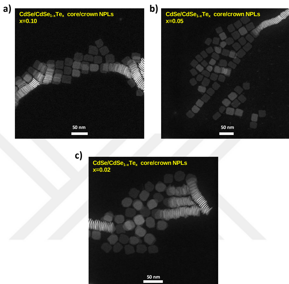
Figure 7.4. HAADF-STEM images of the CdSe/CdSe 1-x Te x core/crown NPLs for different Te compositions (a) x = 0.10 , (b) x = 0.05 , and (c) x = 0.02 in the crown region.
