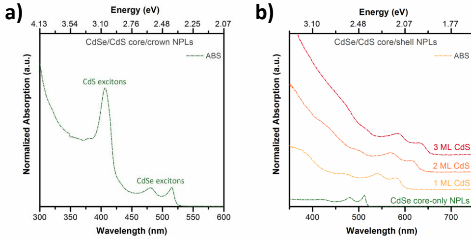
Figure 3.2. Normalized absorption spectra of (a) CdSe/CdS core/crown NPLs and (b) CdSe/CdS core/shell NPLs with different vertical thicknesses synthesized at our laboratories.
