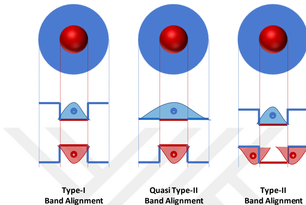
Figure 2.4. Core/shell heterostructures of colloidal semiconductor NCs having different band alignment (Type-I, quasi Type-II and Type-II) along with the localization of electron and hole wavefunctions in these architectures.
