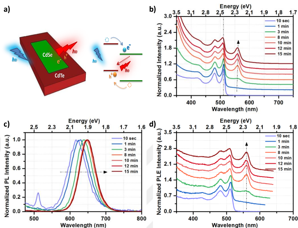
Figure 6.2. Optical characterization of 4 ML thick CdSe/CdTe core/crown NPLs having a higher PL-QY. (a) Schematic representation of carrier photogeneration in both CdSe core and the CdTe crown regions, transfer to core/crown interface, and subsequent radiative recombination resulting in Type-II emission. (b) Normalized absorption, (c) normalized photoluminescence, and (d) normalized photoluminescence excitation spectra of the CdSe/CdTe core/crown NPLs dissolved in hexane with varied crown size. Reprinted with permission from [95]. Copyright 2015 American Chemical Society.
