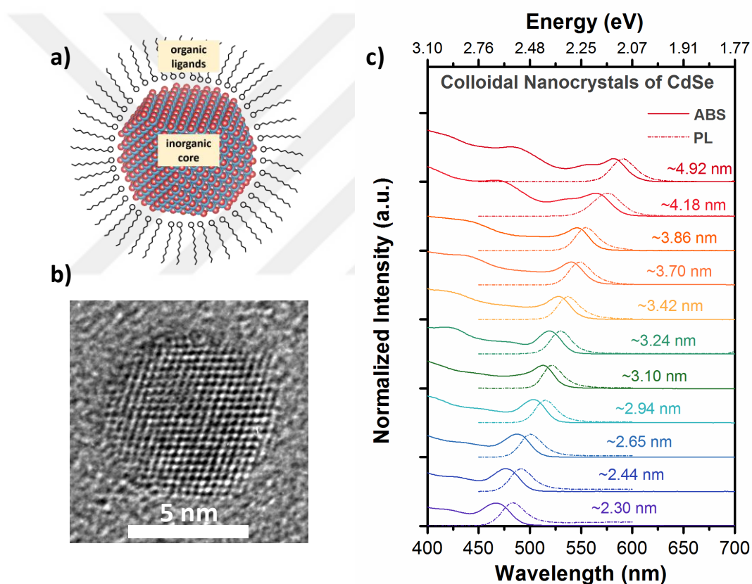
Figure 2.2. (a) Schematic drawing of a colloidal semiconductor NC composed of inorganic core and organic ligands together with (b) a representative high-resolution transmission electron microscopy image of a single colloidal semiconductor NC, synthesized at our laboratories. (c) Normalized absorption and photoluminescence
