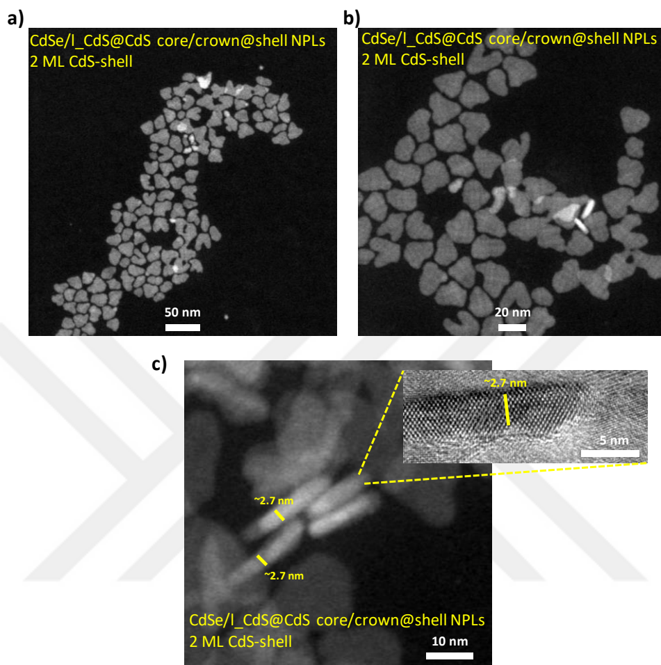
Figure 4.5. HAADF-STEM images of (a), (b) and (c) the CdSe/I_CdS@CdS core/crown@shell NPLs having 2 ML CdS shell thickness at different magnifications. High-resolution TEM image of the CdSe/I_CdS@CdS core/crown@shell NPLs having 2 ML CdS shell is given in the inset. Reprinted with permission from [94]. Copyright 2016 WILEY-VCH Verlag GmbH & Co. KGaA, Weinheim.
