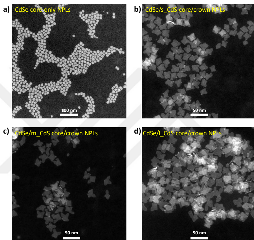
Figure 4.3. HAADF-STEM images of (a) CdSe core-only and CdSe/CdS core/crown NPLs with (b) small, (c) medium, and (d) large CdS crown size. Reprinted with permission from [94]. Copyright 2016 WILEY-VCH Verlag GmbH & Co. KGaA, Weinheim.
