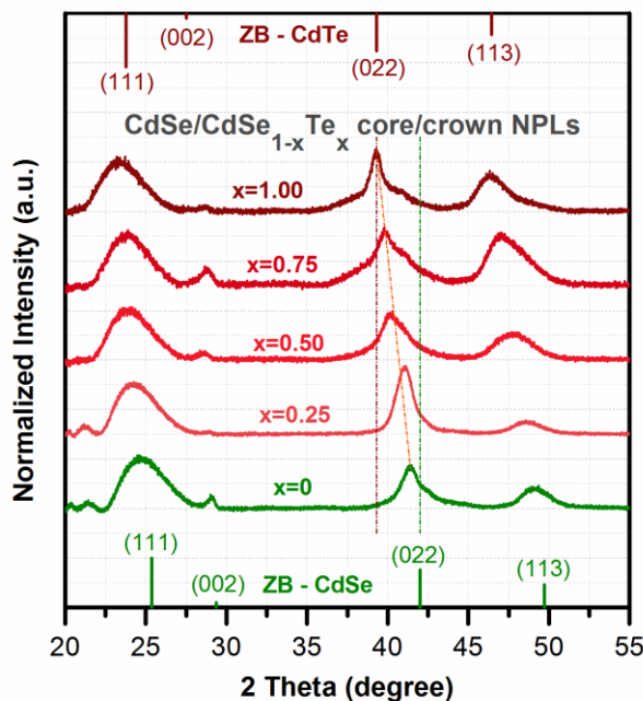
Figure 3.11. Powder XRD patterns of 4 ML thick CdSe core NPLs and CdSe/CdSe 1-x Te x core/crown NPLs having different crown compositions synthesized at our laboratories. Reprinted with permission from [93]. Copyright 2017 American Chemical Society.
