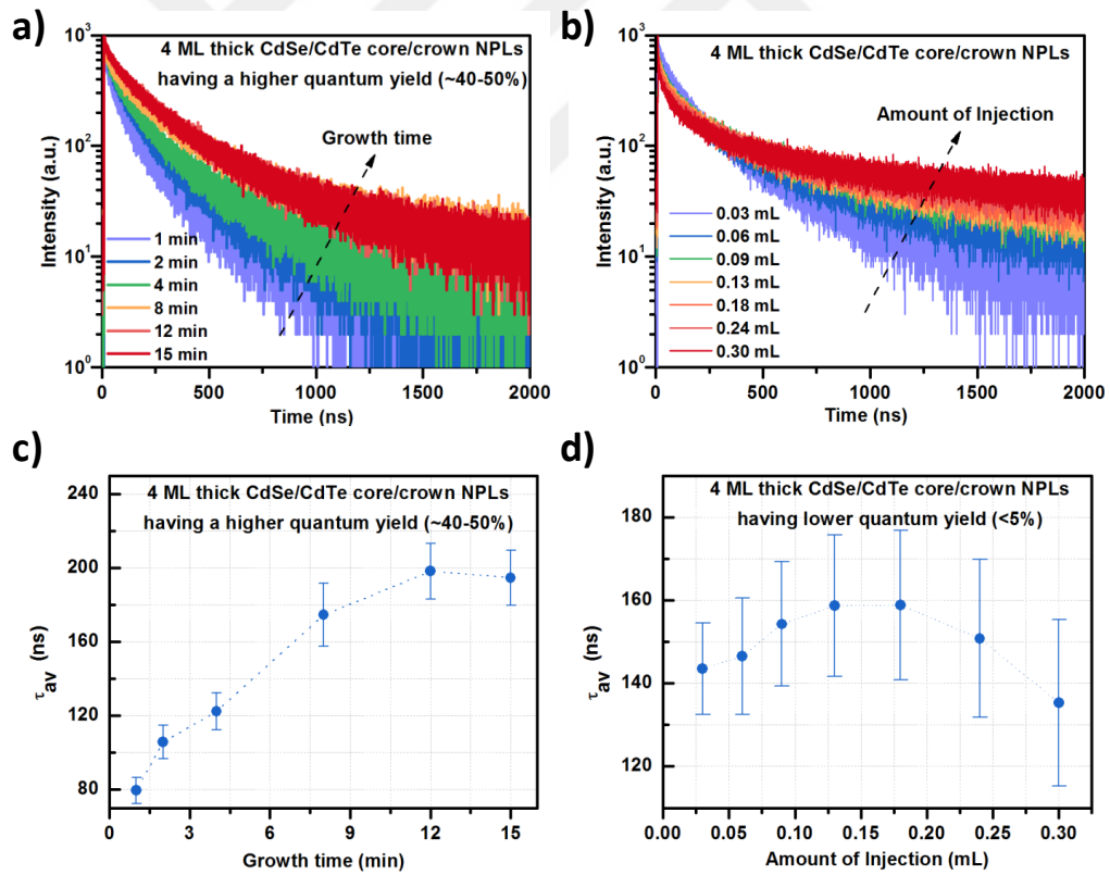
Figure 6.5. Time-resolved fluorescence decay curves of the CdSe/CdTe core/crown NPLs having (a) a higher PL-QY and (b) lower PL-QY with varied crown size. The
