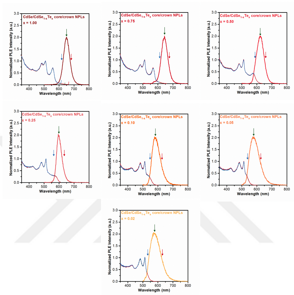
Figure 7.8. Photoluminescence excitation spectra of CdSe/CdSe 1-x Te x core/crown NPLs having different crown composition taken at different emission wavelength. Reprinted with permission from [93]. Copyright 2017 American Chemical Society.
