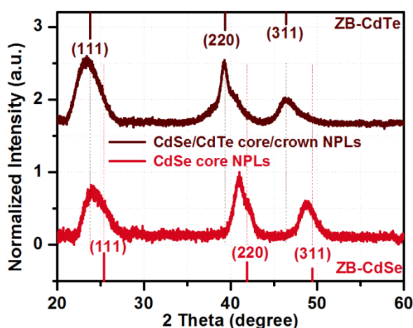
Figure 6.4. X-ray diffraction pattern of 4 ML thick CdSe core NPLs and 4 ML thick CdSe/CdTe core/crown NPLs. Reprinted with permission from [95]. Copyright 2015 American Chemical Society.
