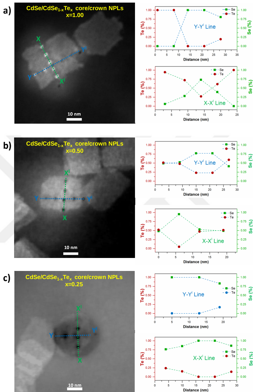
Figure 7.5. HAADF-STEM image of a single CdSe/CdSe 1-x Te x core/crown NPL with blue (Y–Y I ) and green lines (X–X I ) showing the EDX probe position on core/crown NPL together with their line EDX analysis reporting the compositions of selenium and tellurium in the CdSe/CdSe 1-x Te x core/crown NPL, having different crown compositions
