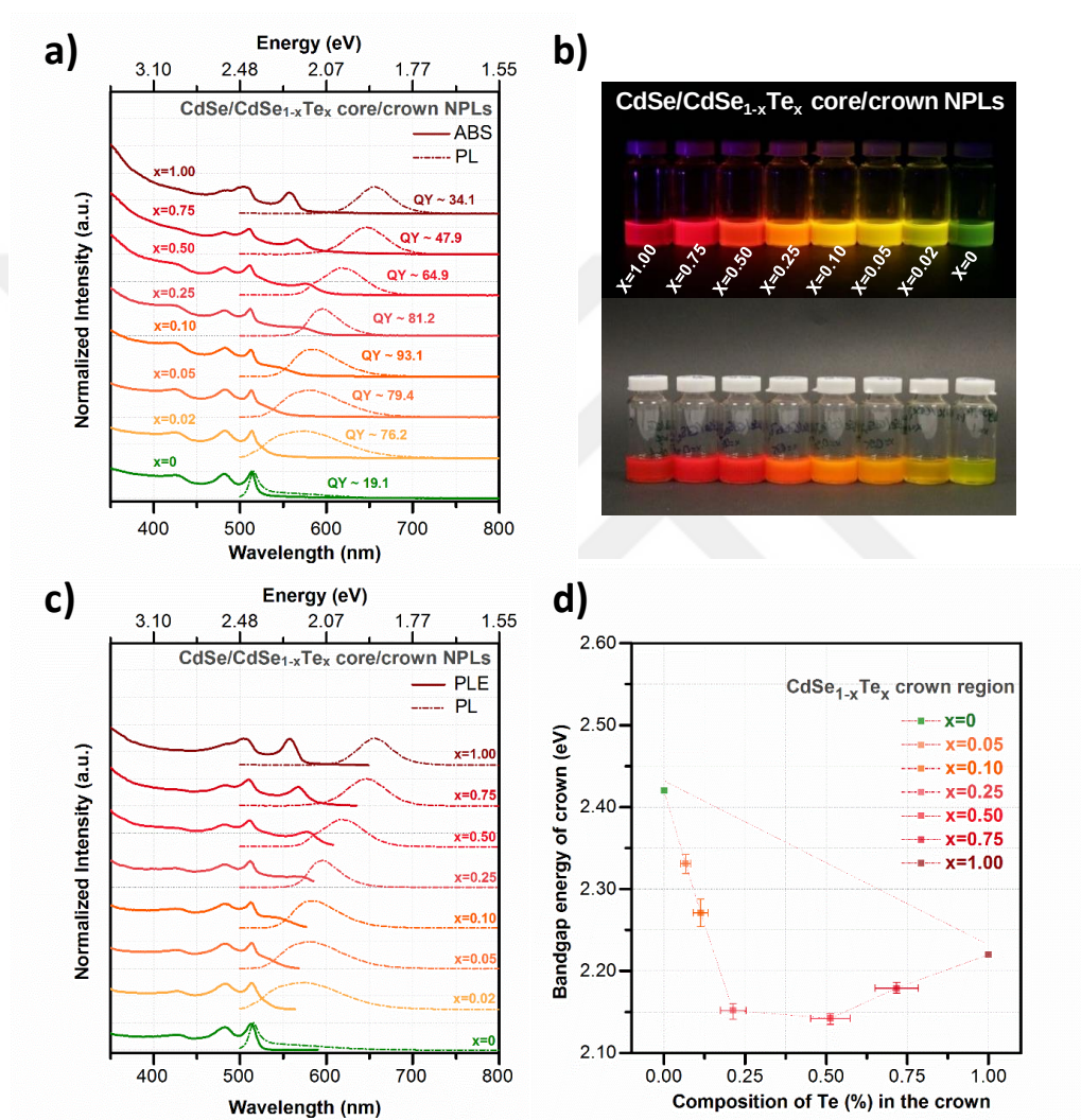
Figure 7.7. (a) Evolution of the absorption and photoluminescence spectra along with PL-QY as a function of the CdSe 1-x Te x crown region composition. (b) The real color images of CdSe/CdSe 1-x Te x core/crown NPLs having different crown compositions dissolved in hexane under UV light (top) and ambient light (bottom). (c) Photoluminescence excitation spectra of the CdSe/CdSe 1-x Te x core/crown NPLs
