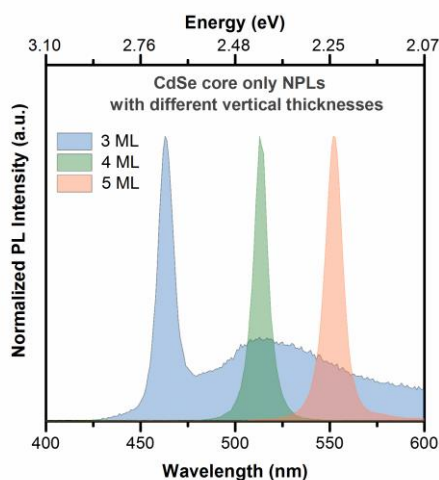
Figure 3.3. Normalized photoluminescence spectra of CdSe core-only NPLs with varying vertical thicknesses synthesized at our laboratories.
