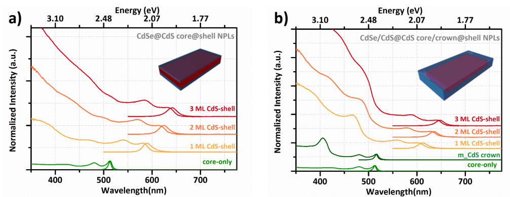
Figure 4.4. Normalized absorption and photoluminescence spectra of (a) CdSe@CdS core@shell, and (b) CdSe/CdS@CdS core/crown@shell NPLs with varying CdS shell
