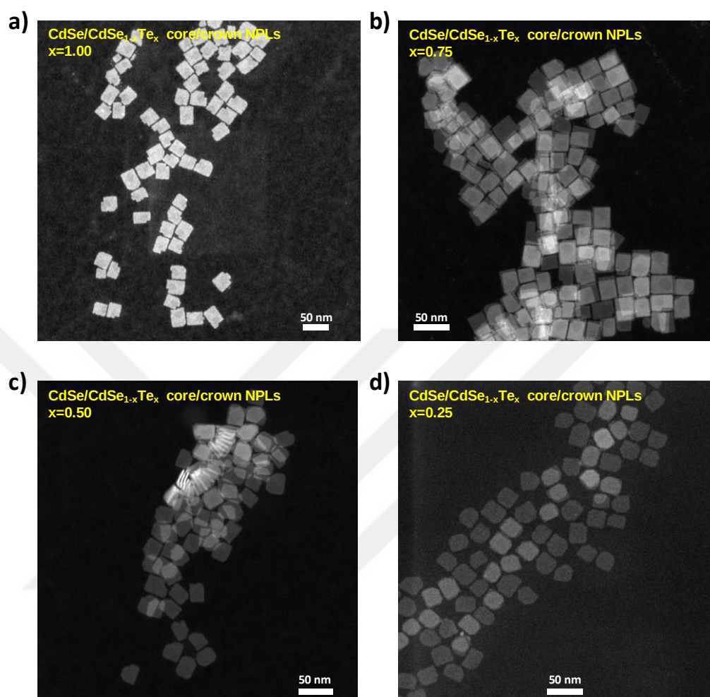
Figure 7.3. HAADF-STEM images of the CdSe/CdSe 1-x Te x core/crown NPLs for different Te compositions (a) x = 1.00 , (b) x = 0.75 , (c) x = 0.50 , and (d) x = 0.25 in the crown region. Reprinted with permission from [93]. Copyright 2017 American Chemical Society.
