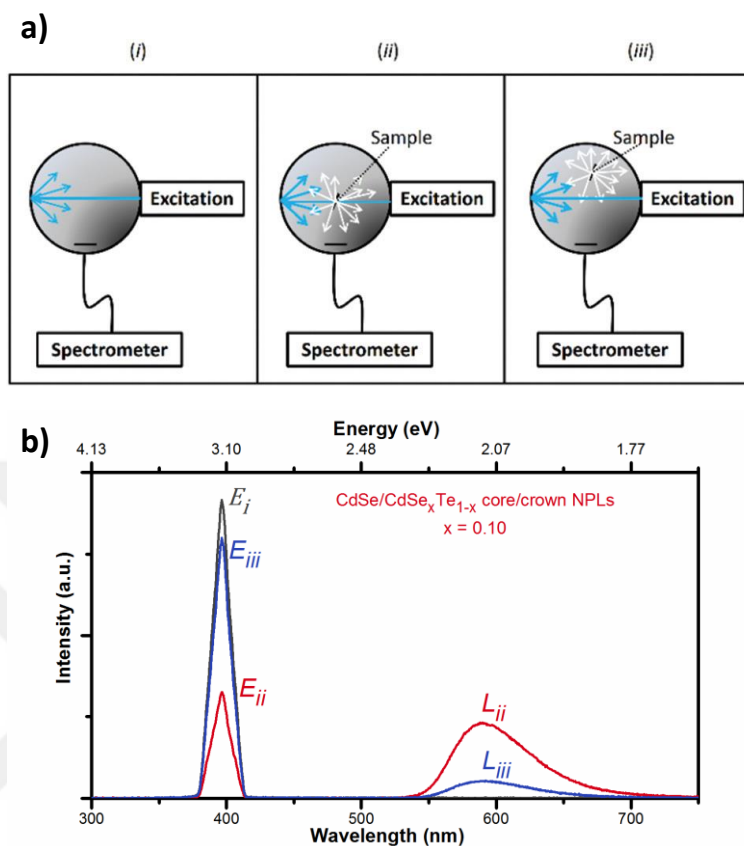
Figure 3.6. (a) Schematic demonstration of different measurement configurations used in the absolute PL-QY measurement method. Reproduced with permission from [92]. Copyright Royal Society of Chemistry 2015. (b) PL-QY measurements of CdSe/CdSe x Te 1-x core/crown NPLs ( x = 0.10 ) performed by following the absolute PL-QY measurements method at our laboratories. While the higher energy sides of the emission spectra show the excitation spectra obtained in different measurement configurations, the lower energy sides of the spectra belong to the emission spectra of the sample obtained in different measurement configurations.
