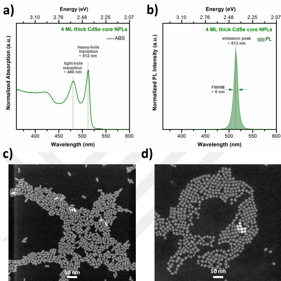
Figure 2.8. Normalized (a) absorption and (b) photoluminescence spectra of our 4 ML thick CdSe core NPLs. HAADF-STEM images of our 4 ML thick CdSe core NPLs with varying lateral dimensions from (c) rectangular-shaped to (d) almost square-shaped.
