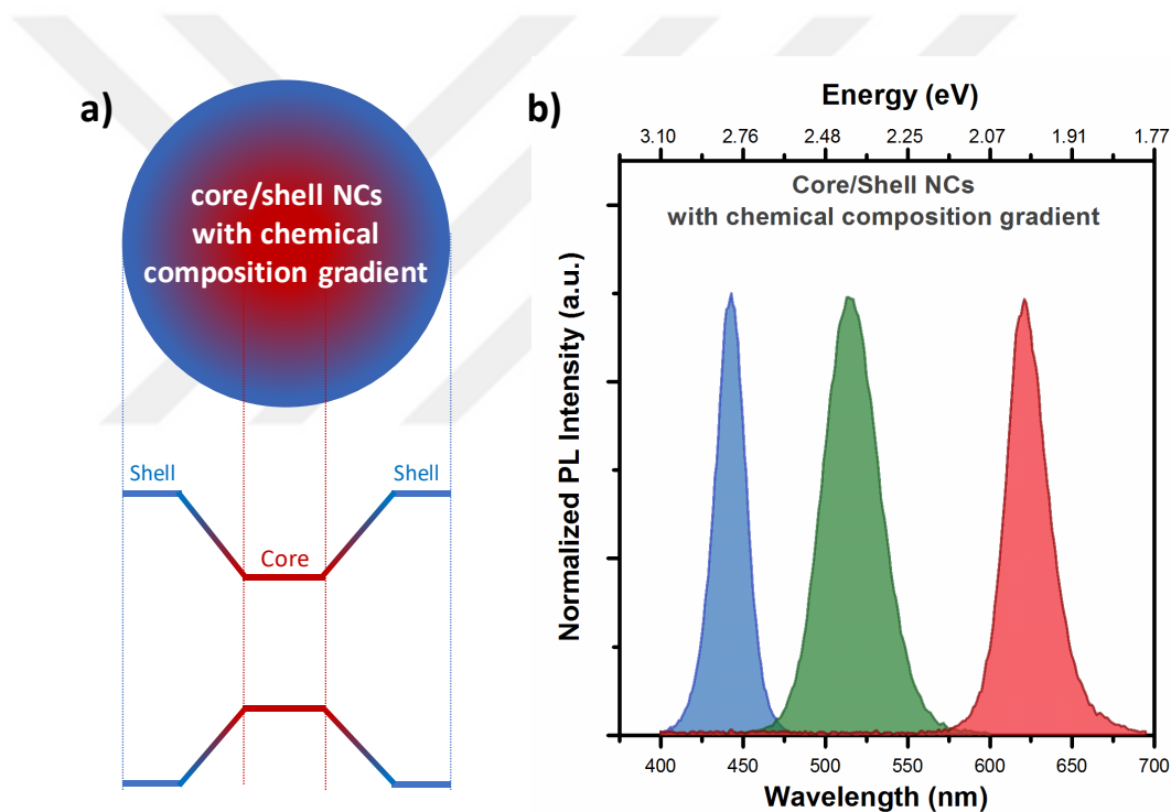
Figure 2.5. (a) Schematic drawing of the core/shell NC having chemical composition gradient structure together with their band alignment. (b) Normalized photoluminescence spectra of blue-, green- and red-emitting colloidal NCs with the chemical composition gradient structure, synthesized at our laboratories.
