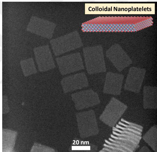
Figure 2.7. High-angle annular dark-field scanning transmission electron microscopy (HAADF-STEM) image of our colloidal NPLs with the inset showing the schematic drawing of atomically-flat colloidal NPLs.
