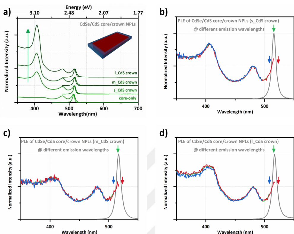
Figure 4.2. (a) Normalized absorption and photoluminescence spectra of CdSe core and CdSe/CdS core/crown NPLs having different crown sizes. Normalized photoluminescence excitation spectra of (b), (c) and (d) CdSe/CdS core/crown NPLs having different crown sizes taken at different emission wavelengths. Reprinted with permission from [94]. Copyright 2016 WILEY-VCH Verlag GmbH & Co. KGaA, Weinheim.
