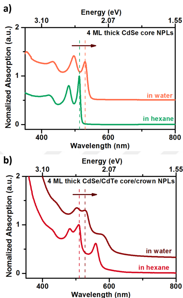
Figure 6.7. Normalized absorption spectra of (a) 4 ML thick CdSe core NPLs and (b) 4 ML thick CdSe/CdTe core/crown NPLs before and after the ligand exchange. Reprinted with permission from [95]. Copyright 2015 American Chemical Society.
