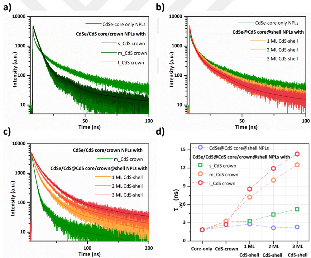
Figure 4.7. Time-resolved fluorescence spectroscopy measurements of (a) CdSe core-only NPLs and CdSe/CdS core/crown NPLs with varying CdS crown size, (b) CdSe@CdS core@shell NPLs, and (c) CdSe/CdS@CdS core/crown@shell NPLs with
