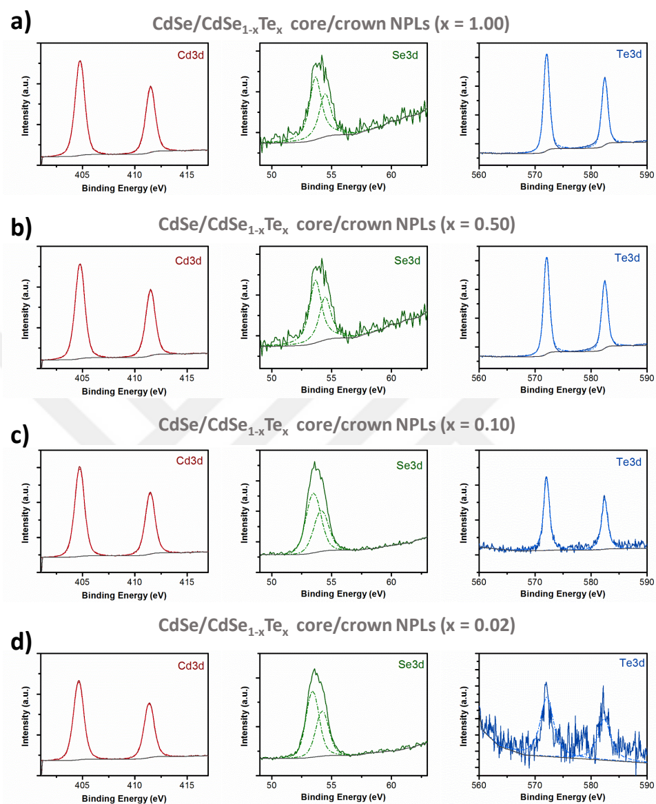
Figure 3.10. The acquired high-resolution XPS spectra of the CdSe/CdSe 1-x Te x core/crown NPLs with varying crown compositions; (a) x = 1.00 , (b) x = 0.50 , (c) x = 0.10 and (d) x = 0.02 , synthesized at our laboratories. Reprinted with permission from [93]. Copyright 2017 American Chemical Society.
