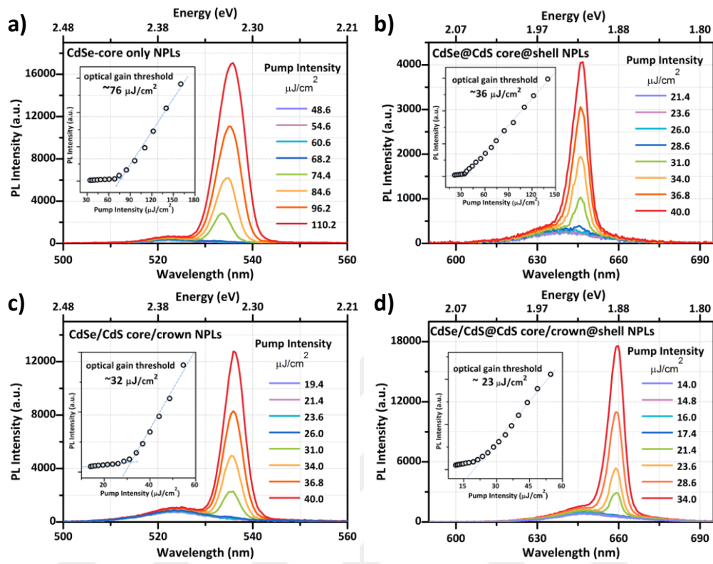
Figure 4.9. Optical gain performances of CdSe-based NPLs having different architectures. Amplified spontaneous emission spectra of (a) CdSe core-only NPLs, (b) CdSe@CdS core@shell NPLs having 2 ML CdS shell thickness, (c) CdSe/CdS core/crown NPLs, and (d) CdSe/CdS@CdS core/crown@shell NPLs having 2 ML CdS shell thickness. The insets show the integrated PL intensity as a function of the excitation intensity. Reprinted with permission from [94]. Copyright 2016 WILEY-VCH Verlag GmbH & Co. KGaA, Weinheim.
