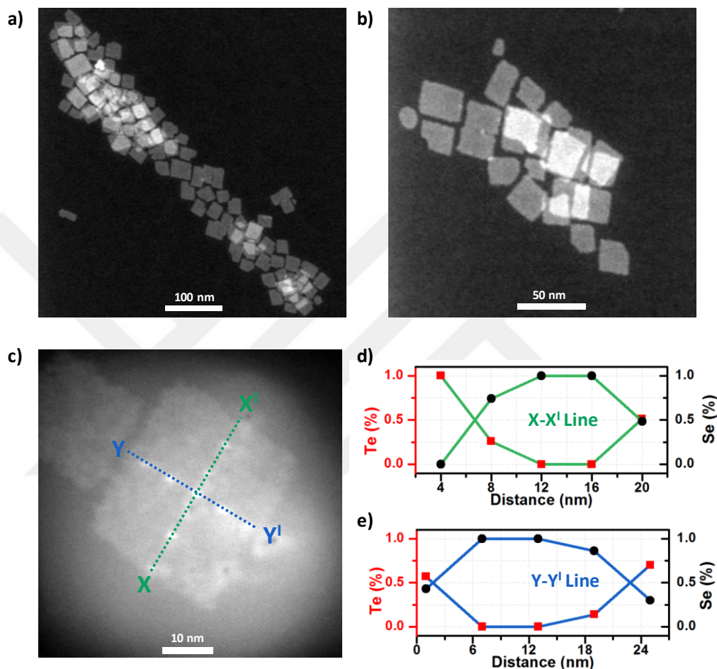
Figure 6.3. Structural characterization of 4 ML thick CdSe/CdTe core/crown NPLs having a higher PL-QY. HAADF-STEM images of CdSe/CdTe core/crown NPLs with a scale bar of (a) 100 and (b) 50 nm. (c) HAADF-STEM image of a single CdSe/CdTe core/crown NPL, with blue (Y–Y') and green lines (X–X') showing the EDX probe position on CdSe/CdTe core/crown NPL and (d, e) the line EDX analysis reporting the compositions of selenium and tellurium in the CdSe/CdTe core/crown NPL, normalized
