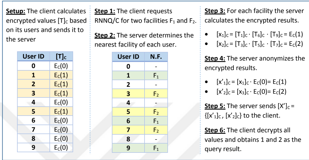
Figure 3.4: An example scenario for RNNQ/C protocol.
