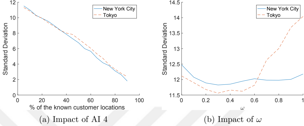
Figure 4.16: Impact of AI 4 and \omega on the standard deviation of rankings in max-inf optimal location query.
