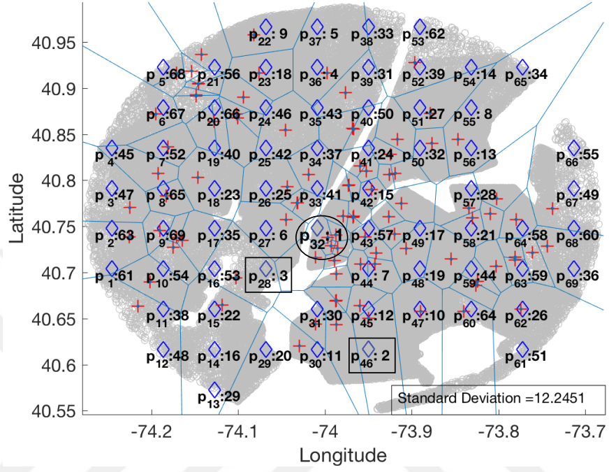
Figure 4.31: Ranking of candidate locations in NYC when k = 100 and synthetic data produced by the clustering-based algorithm is used in min-dist optimal location query.
