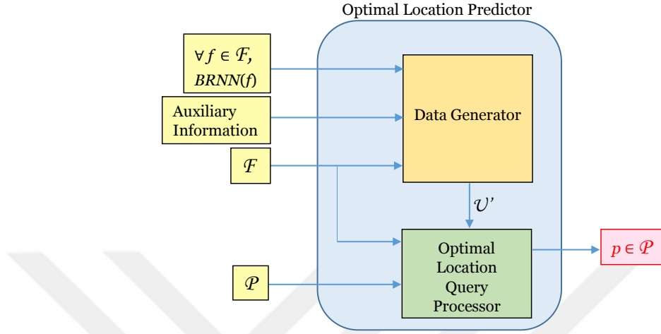
Figure 4.3: Optimal Location Predictor.
