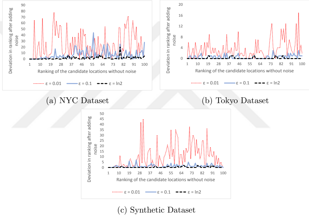
Figure 3.7: Deviation in the rankings of the 100 candidate locations after achieving differential privacy in RNNQ. x axis represents the ranking of the candidate locations when RNNQ is performed with exact query results. y axis represents the change in the ranking of each candidate location when differential privacy is achieved in RNNQ. For instance, in Figure 3.7a the point (5, 65) for \epsilon = 0.01 shows that the 5th best candidate location for the new facility becomes 70th best location after adding noise to the query result. Depending on the maximum change in the ranking, the range of y axis varies for each dataset.
