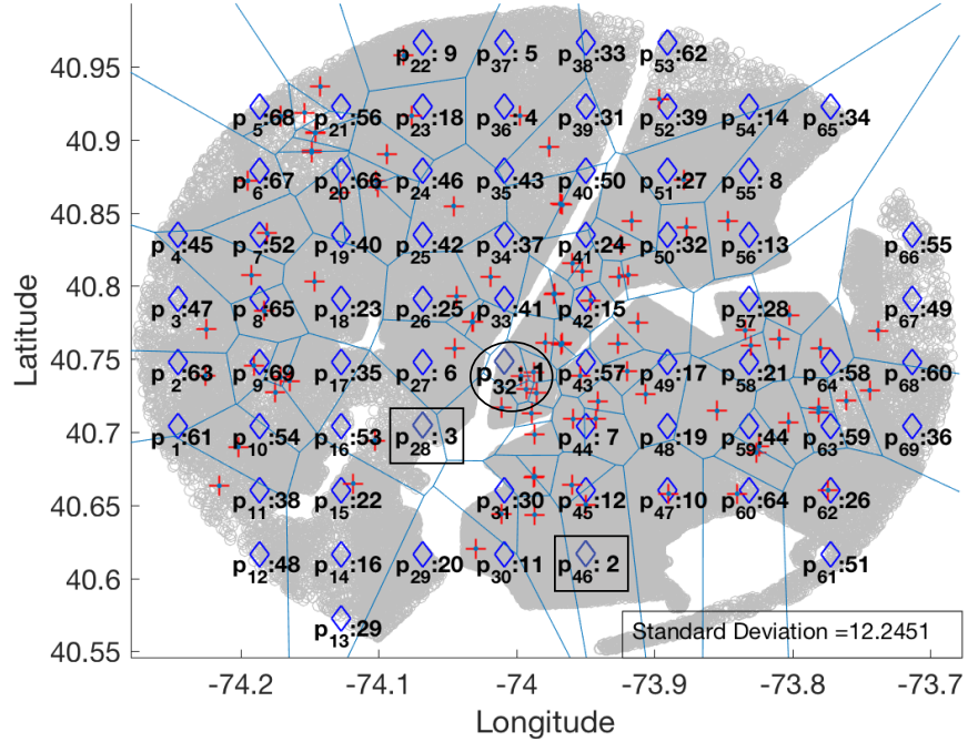
Figure 4.29: Ranking of candidate locations in NYC when k = 1000 and synthetic data produced by the clustering-based algorithm is used in max-inf optimal location query.
