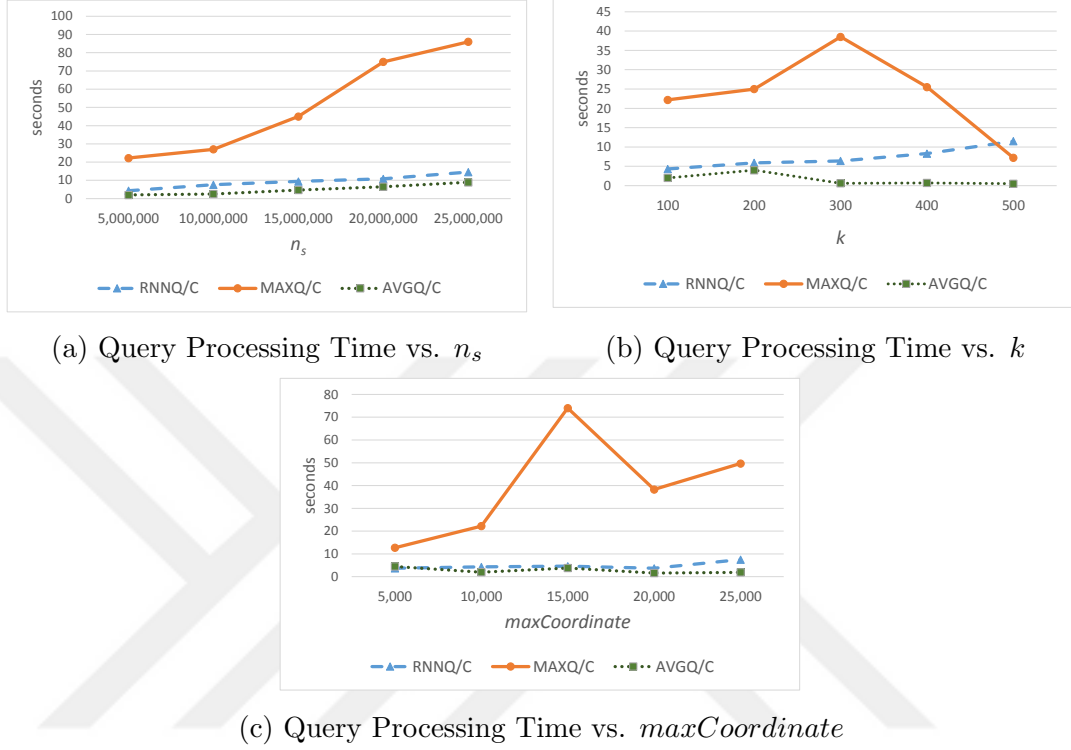
Figure 3.6: Query processing times of the client-based protocols.
