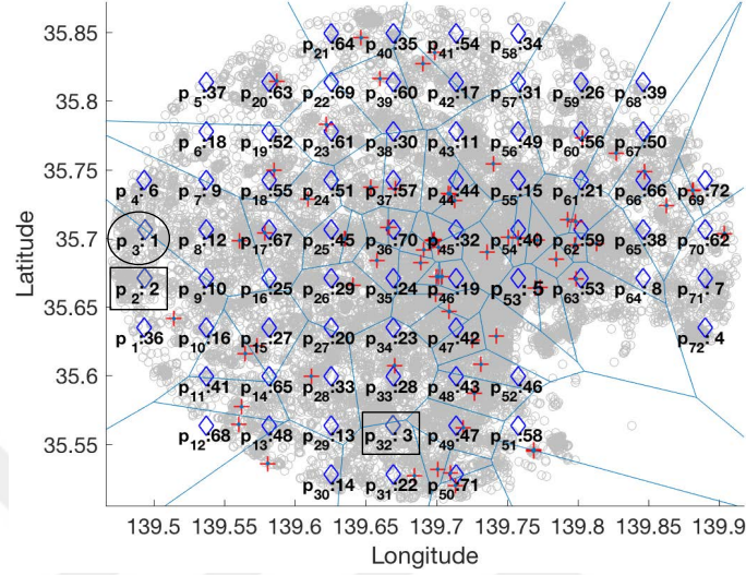
Figure 4.19: Ranking of candidate locations in Tokyo when real data is used in min-dist optimal location query.
