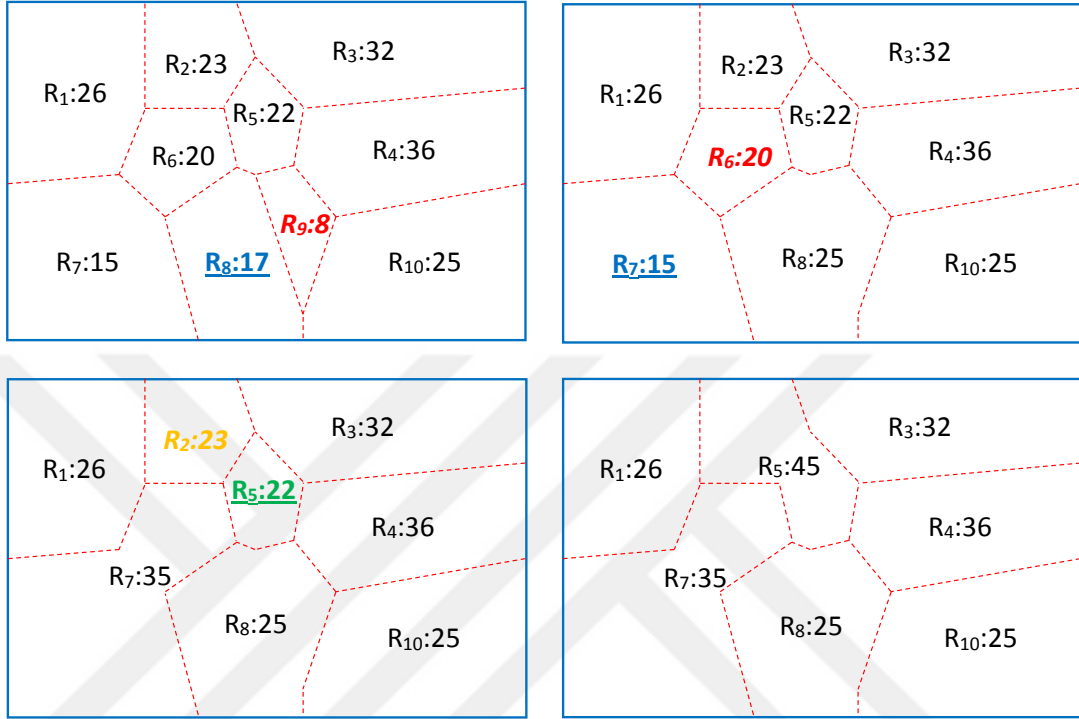
Figure 4.8: An example execution of clustering-based data generation algorithm.
