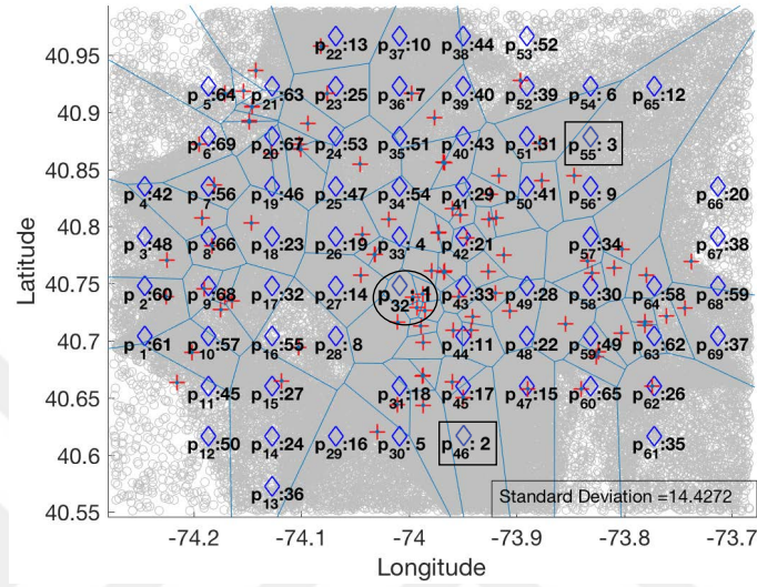
Figure 4.12: Ranking of candidate locations in NYC when the optimal location predictor uses AI 1 in max-inf optimal location query.
