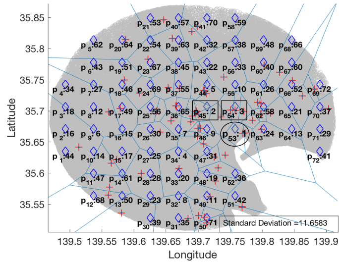
Figure 4.15: Ranking of candidate locations in Tokyo when the optimal location predictor uses AI 2 and AI 3 in max-inf optimal location query.
