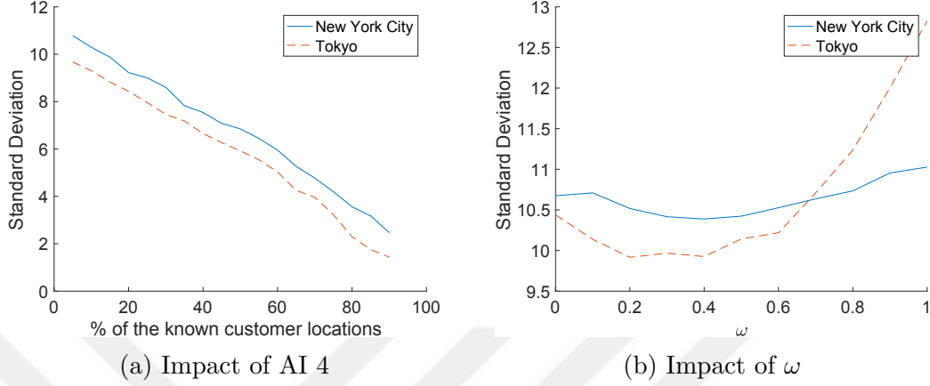
Figure 4.24: Impact of AI 4 and \omega on the standard deviation of rankings in min-dist optimal location query.
