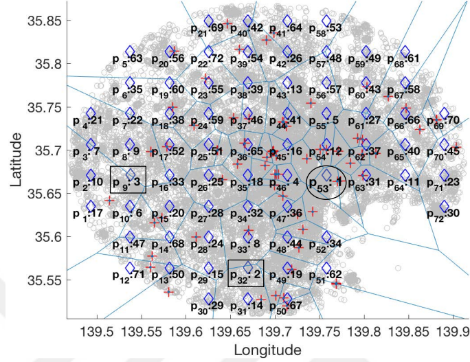
Figure 4.11: Ranking of candidate locations in Tokyo when real data is used in max-inf optimal location query.
