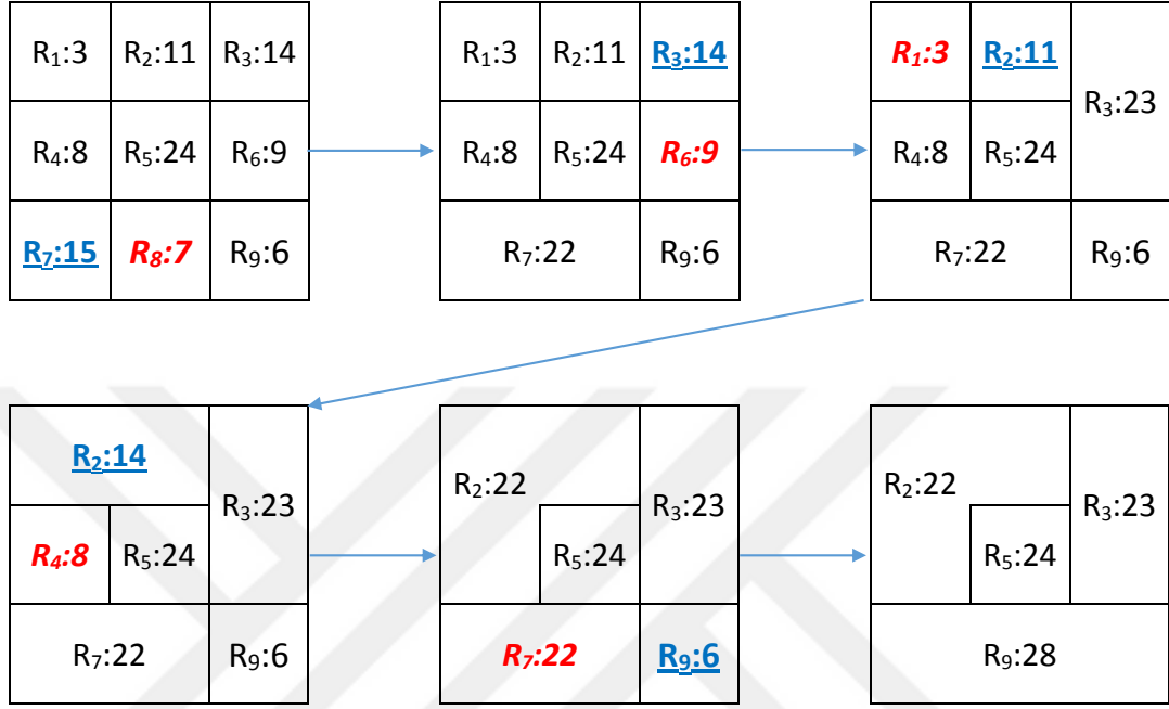
Figure 4.7: An example execution of grid-based data generation algorithm.
