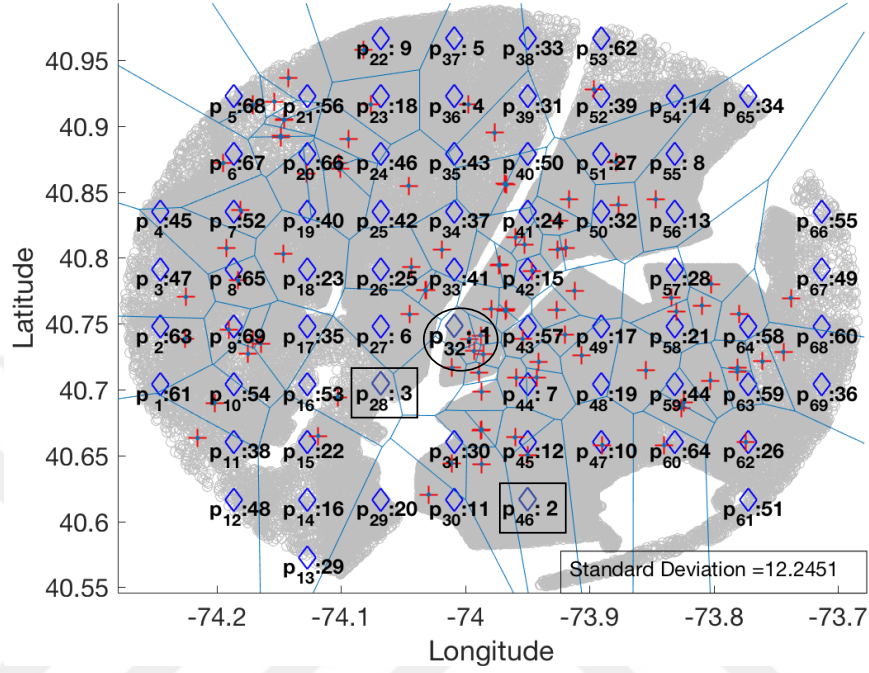
Figure 4.33: Ranking of candidate locations in NYC when k = 1000 and synthetic data produced by the clustering-based algorithm is used in min-dist optimal location query.
