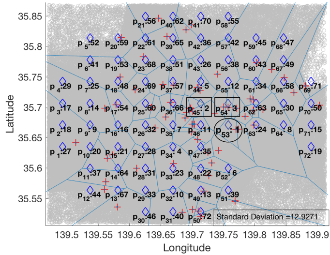
Figure 4.13: Ranking of candidate locations in Tokyo when the optimal location predictor uses AI 1 in max-inf optimal location query.
