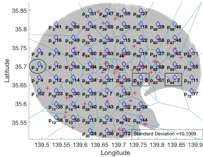
Figure 4.23: Ranking of candidate locations in Tokyo when the optimal location predictor uses AI 2 and AI 3 in min-dist optimal location query.
