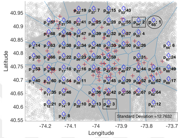
Figure 4.20: Ranking of candidate locations in NYC when the optimal location predictor uses AI 1 in min-dist optimal location query.
