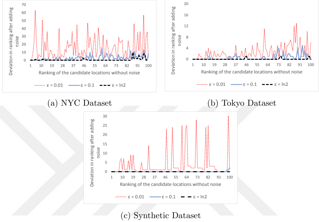
Figure 3.8: Deviation in the rankings of the 100 candidate locations after achieving differential privacy in AVGQ.
