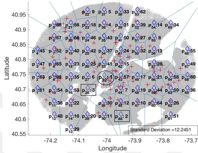
Figure 4.14: Ranking of candidate locations in NYC when the optimal location predictor uses AI 2 and AI 3 in max-inf optimal location query.
