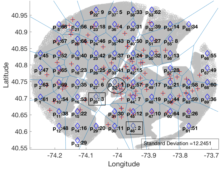
Figure 4.32: Ranking of candidate locations in NYC when k = 1000 and synthetic data produced by the grid-based algorithm is used in min-dist optimal location query.
