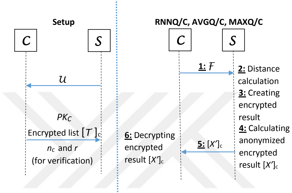
Figure 3.3: Overview of the client-based query processing protocols.
