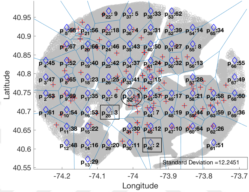
Figure 4.28: Ranking of candidate locations in NYC when k = 1000 and synthetic data produced by the grid-based algorithm is used in max-inf optimal location query.
