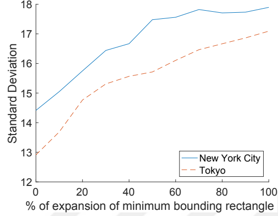
Figure 4.17: Standard deviation of rankings when no AI is provided to the optimal location predictor in max-inf optimal location query.
