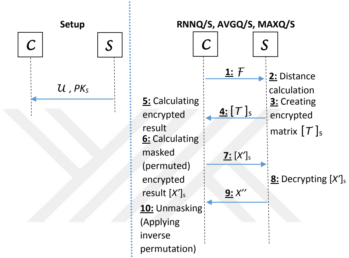
Figure 3.2: Overview of the server-based query processing protocols.
