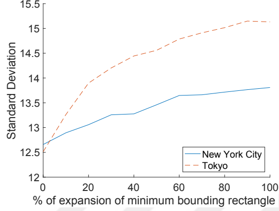
Figure 4.25: Standard deviation of rankings when no AI is provided to the optimal location predictor in min-dist optimal location query.
