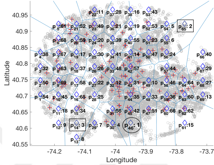
Figure 4.18: Ranking of candidate locations in NYC when real data is used in min-dist optimal location query.
