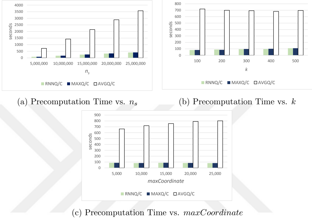
Figure 3.5: Precomputation times of the client-based protocols.
