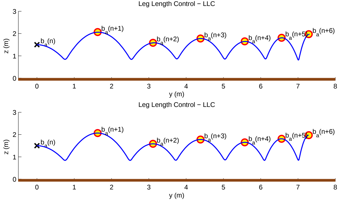
Figure 5.4: Leg Length Control - LLC for Nonsymmetric Steps over a flat surface. Upper : The apex return map used by LLC is based on our approximate stance map. Number of iterations during optimization is around 224 and the computation time is around 0.34 secs for each steps. Lower : “Ground Truth” for LLC. The apex return map used by LLC is based on numeric solution of the SLIP dynamics. Number of iterations during optimization is around 213 and the computation time is around 5.6 secs for each steps. If we also compute the height of the flat ground portion where the SLIP lands for every iteration, the computation time increases to 7.1 secs and 10.8 secs for the upper and lower cases, respectively.
