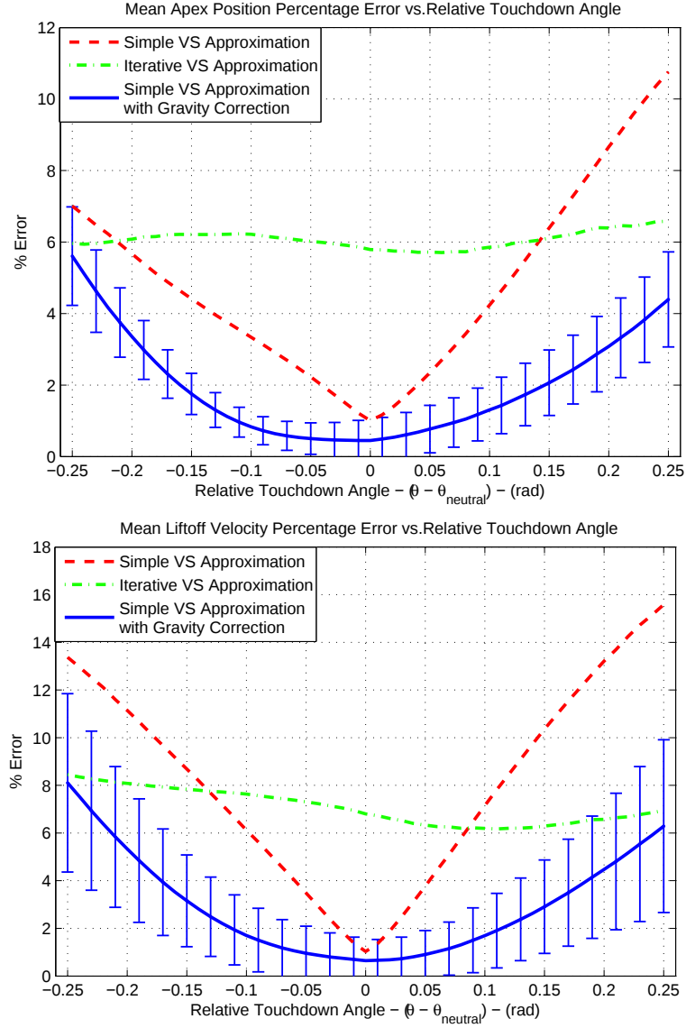
Figure 3.11: Upper: Mean Apex Position Percentage Error ( PE_{ap} ) versus Relative Touchdown Angle ( q_{\theta_{td}} - q_{\theta_{tdn}} ). Lower: Mean Liftoff Velocity Percentage Error ( PE_{lov} ) versus Relative Touchdown Angle ( q_{\theta_{td}} - q_{\theta_{tdn}} ). The vertical bars represent standard deviations for the approximate stance map with gravity correction.
