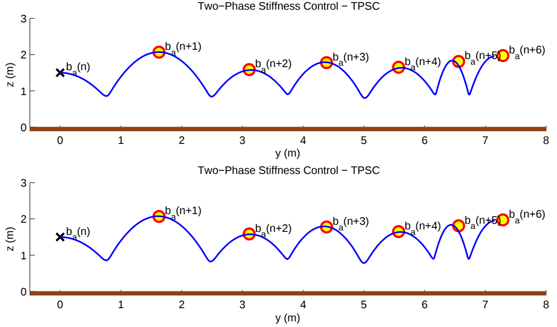
Figure 5.6: Two-Phase Stiffness Control - TPSC for Nonsymmetric Steps over a flat surface. Upper : The apex return map used by TPSC is based on our approximate stance map. Number of iterations during optimization is around 282 and the computation time is approximately 0.56 secs for each steps. Lower : “Ground Truth” for TPSC. The apex return map used by TPSC is based on numeric solution of the SLIP dynamics. Number of iterations during optimization is around 253 and the computation time is around 8.2 secs for each steps. If we also compute the height of the flat ground portion where the SLIP lands for every iteration, the computation time increases to 8.6 secs and 18.4 secs for the upper and lower cases, respectively.
