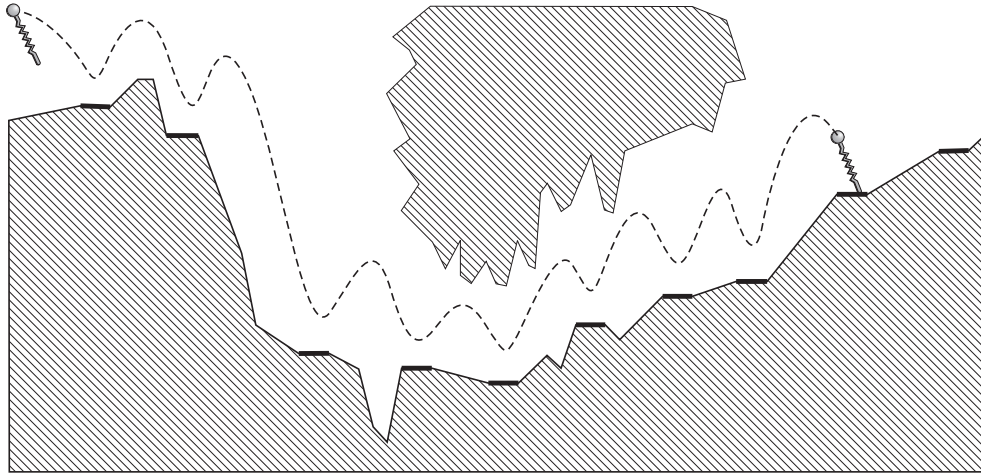
Figure 1.4: An illustrative figure of the spring mass hopper locomotion over an uneven terrain (inspired from [1]).
