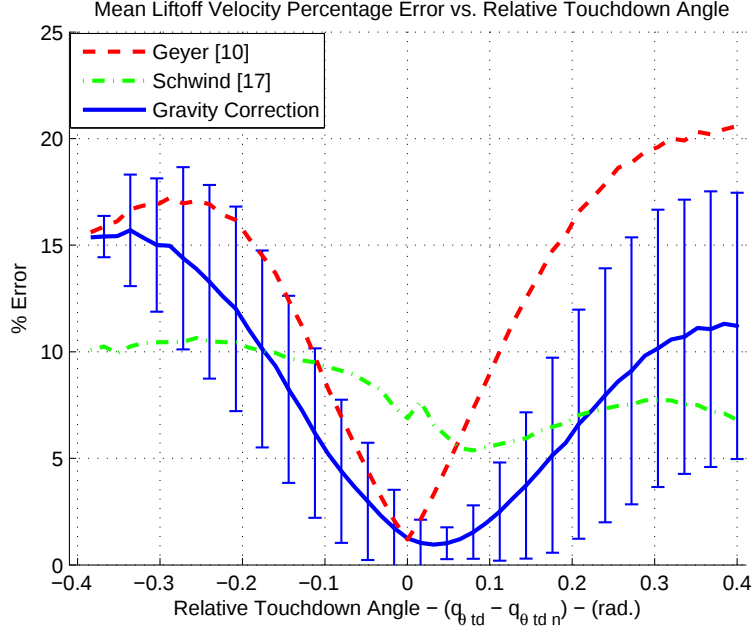
Figure 3.5: Mean Liftoff Velocity Percentage Error ( PE_{lov} ) versus Relative Touchdown Angle ( q_{\theta_{td}} - q_{\theta_{tdn}} ). The vertical bars represent the standard deviations for the approximate stance map with gravity correction.
