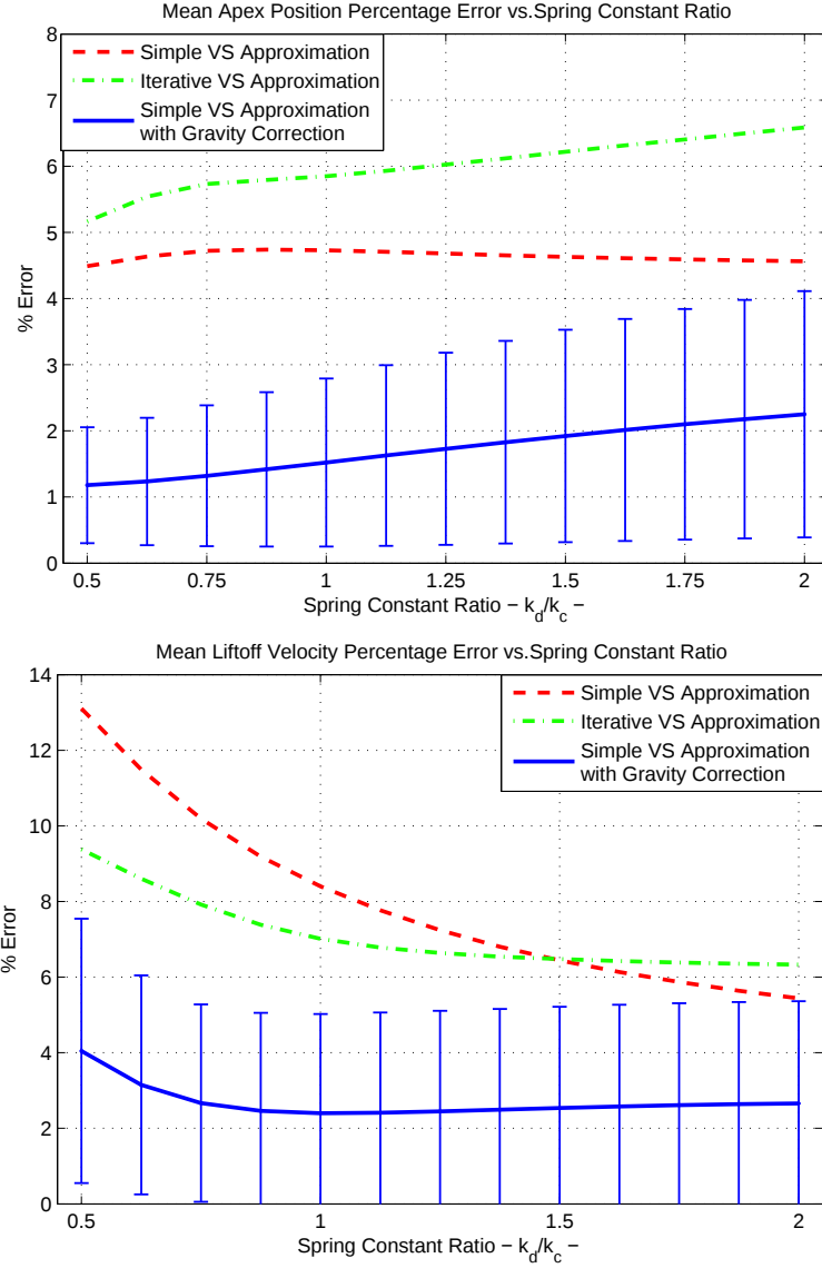
Figure 3.12: Upper: Mean Apex Position Percentage Error ( PE_{ap} ) versus Stiffness Ratio ( k_d/k_c ). Lower: Mean Liftoff Velocity Percentage Error ( PE_{lov} ) versus Stiffness Ratio ( k_d/k_c ). The vertical bars represent standard deviations for the approximate stance map with gravity correction.
