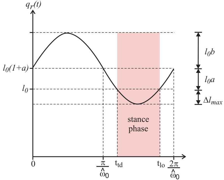
Figure 2.4: General solution for the leg length, q_r(t) , during stance. The sinusoidal solution has amplitude l_0 b and frequency \hat{\omega}_0 with offset l_0(1+a) . Since the solution is only suitable for the stance phase, only the portion where q_r \leq l_0 is significant. The parameter a can also be negative, in which case l_0 will be above l_0(1+a) . \Delta l_{max} represents the maximum leg compression. (reproduced from [2])
