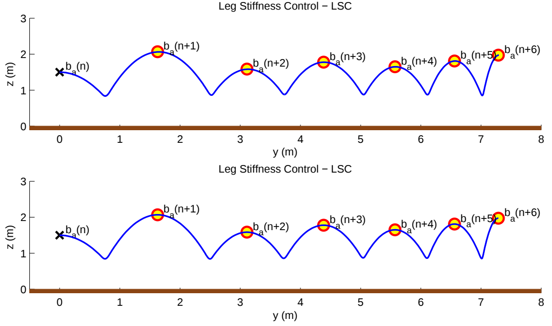
Figure 5.5: Leg Stiffness Control - LSC for Nonymmetric Steps over a flat surface. Upper : The apex return map used by LSC is based on our approximate stance map. Number of iterations during optimization is around 258 and the computation time is approximately 0.35 secs for each steps. Lower : “Ground Truth” for LSC. The apex return map used by LSC is based on numeric solution of the SLIP dynamics. Number of iterations during optimization is around 215 and the computation time is around 5.6 secs for each steps. If we also compute the height of the flat ground portion where the SLIP lands for every iteration, the computation time increases to 8.3 secs and 13.3 secs for the upper and lower cases, respectively.
