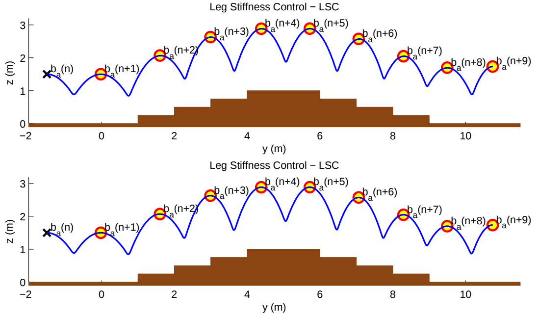
Figure 5.8: Leg Stiffness Control - LSC for Nonymmetric Steps over a flat surface. Upper: The apex return map used by LSC is based on our approximate stance map. Number of iterations during optimization is around 258 and the computation time is approximately 10.6 secs for each steps. Lower: “Ground Truth” for LSC. The apex return map used by LSC is based on numeric solution of the SLIP dynamics. Number of iterations during optimization is around 210 and the computation time is around 13.7 secs for each steps.
