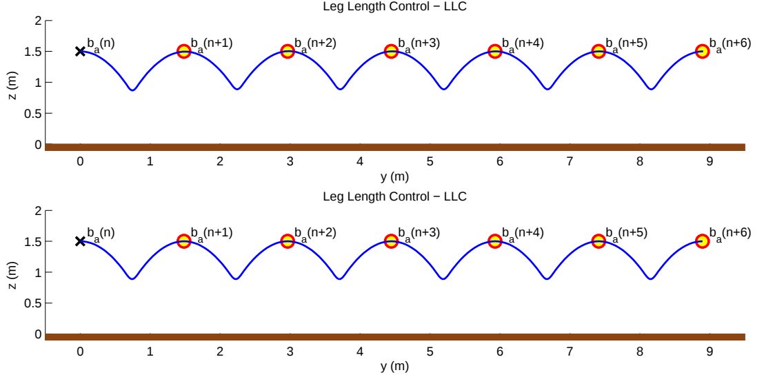
Figure 5.1: Leg Length Control - LLC for Symmetric Steps over a flat surface. Upper: The apex return map used by LLC is based on our approximate stance map. Number of iterations during optimization is around 191 and the computation time is around 0.31 secs for each steps. Lower: “Ground Truth” for LLC. The apex return map used by LLC is based on numeric solution of the SLIP dynamics. Number of iterations during optimization is around 235 and the computation time is around 6.1 secs for each steps. If we also compute the height of the flat ground portion where the SLIP lands for every iteration, the computation time increases to 5.1 secs and 12.4 secs for the upper and lower cases, respectively.
