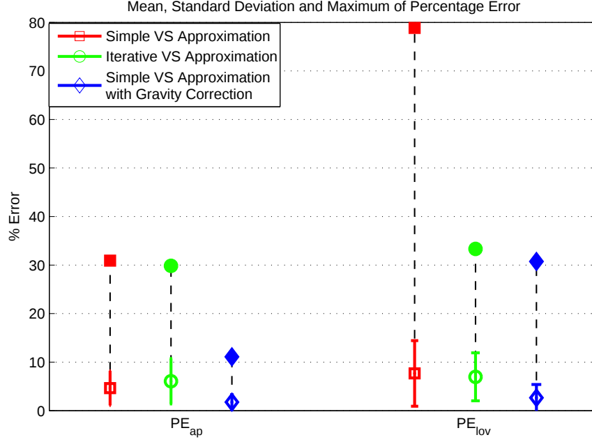
Figure 3.10: Estimation performances for the stance maps of Simple , Iterative and Simple Gravity Corrected Variable Stiffness (VS) Approximations. PE_{ap} (left) and PE_{lo} (right) are apex position and liftoff velocity percentage errors. Empty markers, filled markers and colored vertical bars represent mean, maximum and standard deviations of associated approximations.
