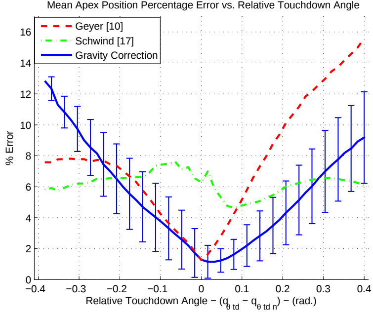
Figure 3.4: Mean Apex Position Percentage Error ( PE_{ap} ) versus Relative Touchdown Angle ( q_{\theta_{td}} - q_{\theta_{tdn}} ). The vertical bars represent standard deviations for the approximate stance map with gravity correction.
