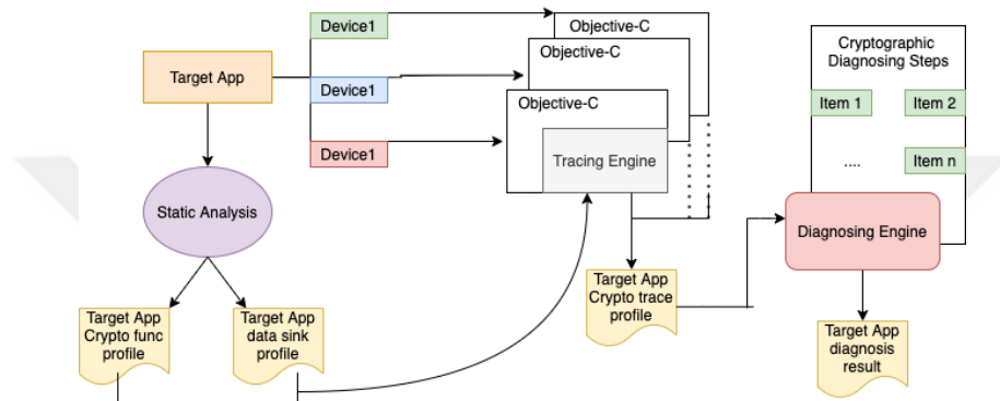
Figure 4.1: Process of iCryptoTracer
