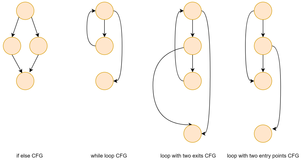
Figure 3.1: CFG examples
