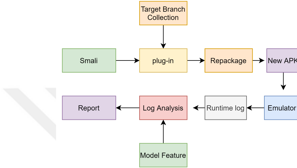
Figure 3.3: Process of CMA
