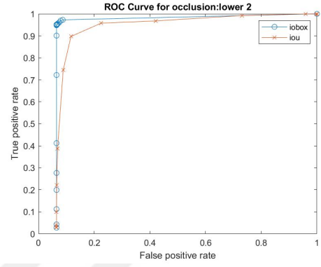
(b) ROC Curve for level 2 lower occlusion
