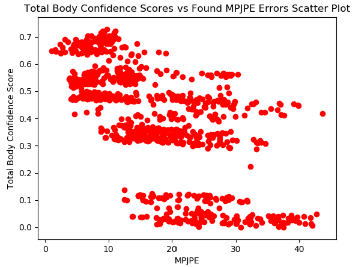
Figure 4.19: Scatter plot of total body predictability scores vs. MPJPE errors of BAKE for sequence 1.
