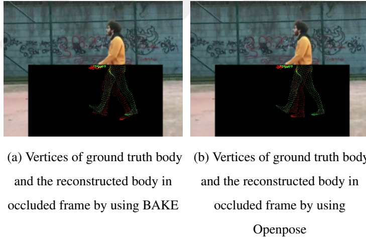
Figure 5.8: Vertices of ground truth and predicted bodies in the occluded region. Red corresponds to the vertices of the predicted body while green corresponds to the vertices of the ground truth body. Since the correspondence of each vertex between two images is known, E_v can be used to measure the similarity of the reconstructed SMPL body in the occluded frame with the ground truth body in the original frame.
