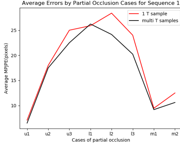
Figure 4.9: Average MPJPE results of BAKE for different strategies to use total body length T . Horizontal axis corresponds to occlusion cases where u is for upper, l is for lower and m is for mid occlusions. Vertical axis is the average MPJPE of test frames for each occlusion case.
