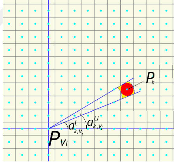
Figure A.1: Illustration of deviation of unit area \|\mathbf{p}_k - \mathbf{p}_k^c\|_2 < \Delta_p for an example point. Red area is the original region. p_{v_i} is the i^{th} visible point and it is set to the center of horizontal and vertical axes for illustration. By defining the angle limits a_{k,v_i}^L and a_{k,v_i}^U , this region expands through the yellow region.
