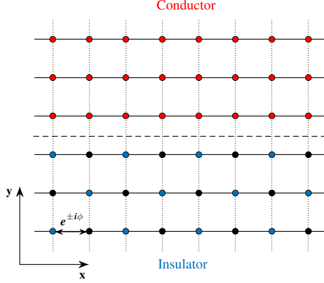
Figure 5.1: Schematic view of the lattice model studied in this thesis. The upper half is a simple tight-binding model (ideal conductor) the lower half is a band-insulator. The dashed line indicates an interface.
