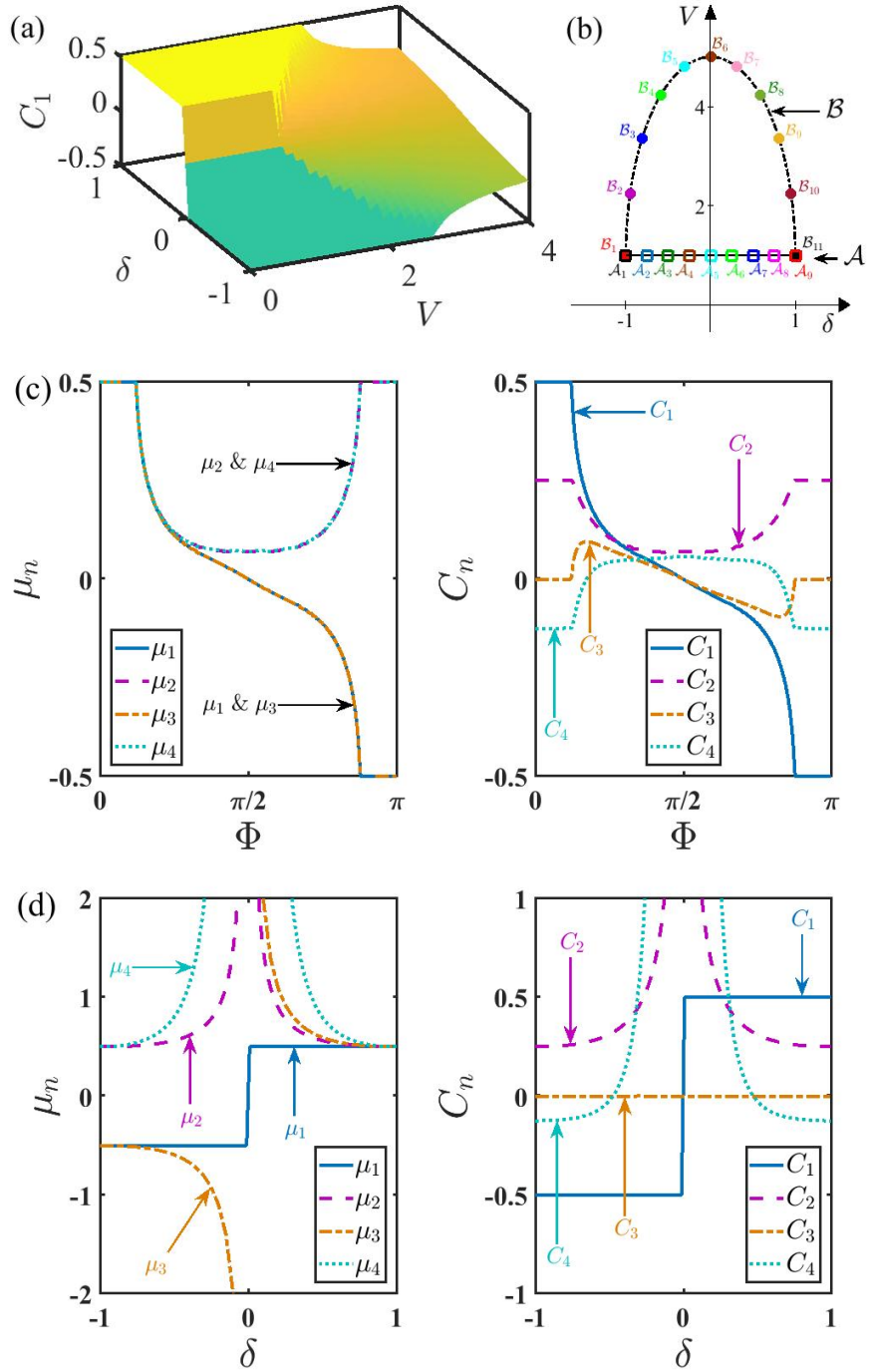
Figure 3.17: (a) First cumulant, ( C_1 ) or polarization, of the interacting Su-Schrieffer-Heeger model as a function of \delta and V . (b) Lines in the \delta - V plane for which we calculate the cumulants and reconstruct the polarization. Two paths are shown between the points -1, 1 and 1, 1 : path \mathcal{A} is a straight line, path \mathcal{B} is a semi-ellipse. (c) Moments and cumulants along the semi-elliptical ( \mathcal{B} ) path. (d) Moments and cumulants along the straight line ( \mathcal{A} ) path.
