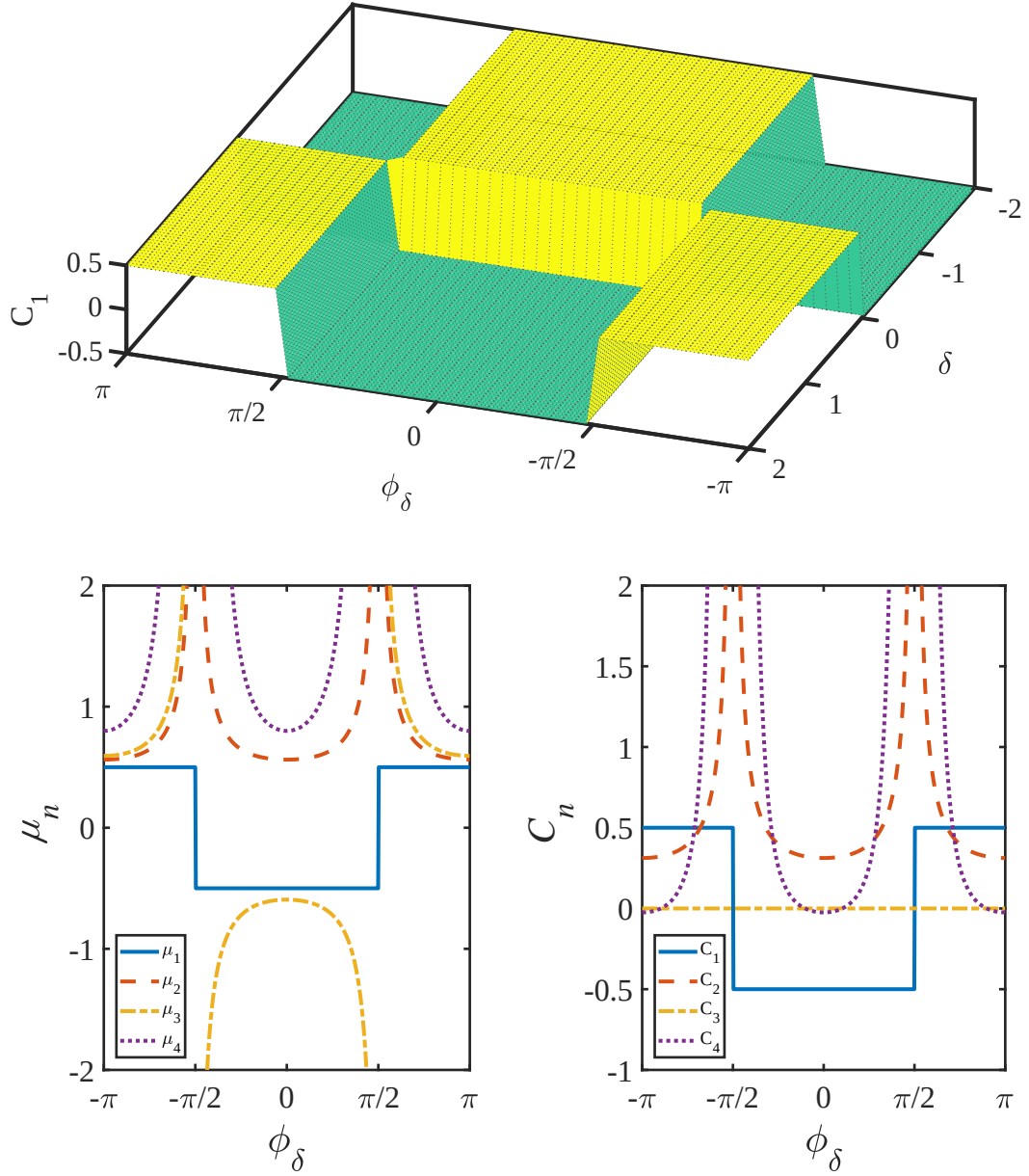
Figure 2.4: Moments and cumulants of GAA model for \delta = 0.5 , \phi_V = 0 , and V = 0 as a function of \phi_\delta .
