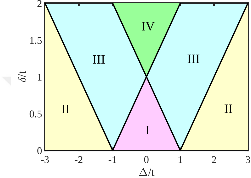
Figure 6.2: Phase diagram of the off-diagonal GAAH model with the p -wave incommensurate modulation amplitude \delta and the p -wave pairing strength \Delta . The hopping incommensurate modulation amplitude is set to \tau = 0 and the phase in the incommensurate modulation is set to k_y = \pi/2 and \varphi = \beta\pi . The phases are (I and II) extended phases, (III) the mobility-edge phase, and (IV) critical phase.
