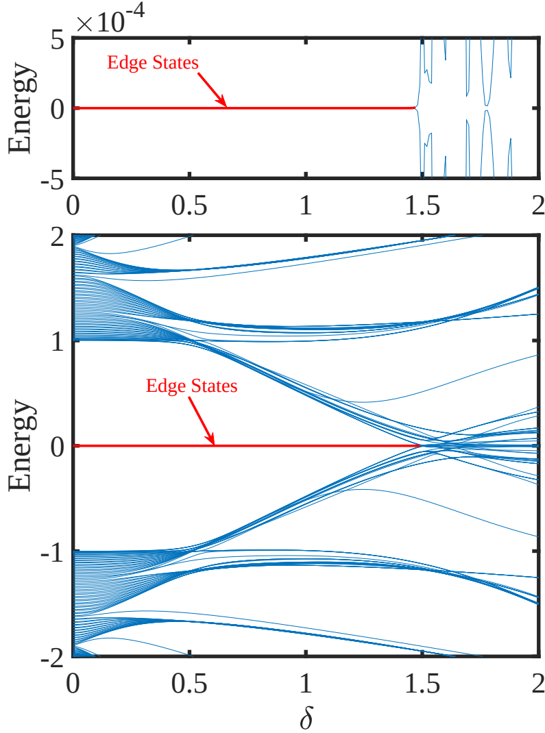
Figure 6.3: The energy spectrum of the off-diagonal GAAH model with p -wave pairing plotted as a function of \delta under OBCs in the lattice dimension with 100 lattice sites. The model parameters are fixed at \tau = 0 , V = 0 , and \Delta = 0.5 . Inside the regions I and II (see figure 6.2) edge states arise.
