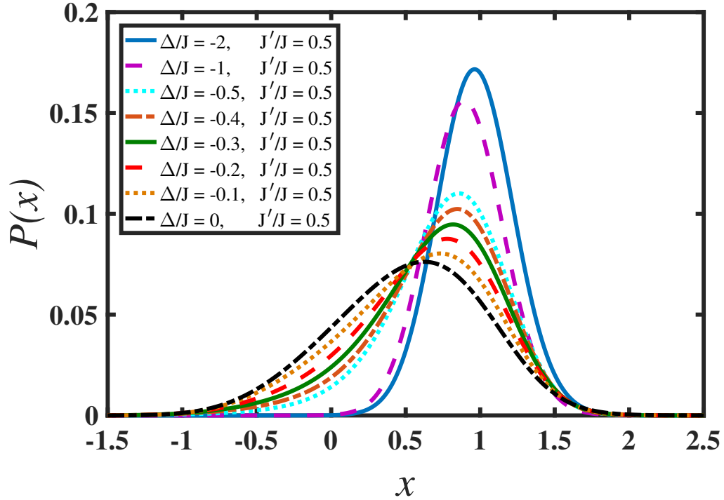
Figure 3.8: Normalized probability distribution of the polarization for different parameters of the Rice-Mele Hamiltonian. In these calculations J = 1 . The unit of length in these figures is the lattice constant. Different values of \Delta/J are shown for J'/J = 0.5 . In the topmost panel ( J'/J = 0 ) the inset shows the distribution for the cases \Delta/J = 0.0, -0.1, -0.2, -0.3, -0.4, -0.5
