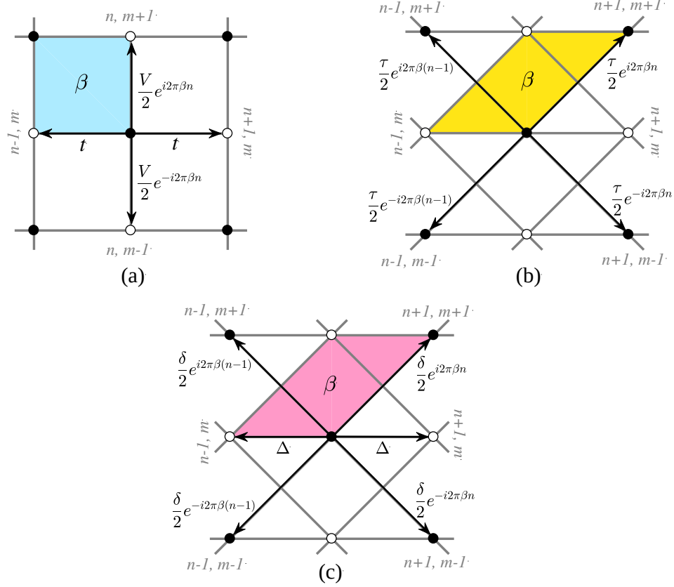
Figure 6.1: Graphical presentations of extended 1d GAAH with nearest and next-nearest hopping (SC pairing) and on-site potential to a 2D Hamiltonian. In the presence of a perpendicular magnetic field with \beta flux quantum per unit cell, the electrons hop on a rectangular lattice. (a) This is the 2D “ancestor” of the diagonal GAAH model which the hopping is to nearest neighbors, (b) This is the 2D “ancestor” of the off-diagonal GAAH model which the hopping is to next-nearest neighbors, and (c) This is the 2D “ancestor” of the SC pairing of GAAH model which the hopping is to nearest and next nearest neighbors. Each rectangular plaquettes which demonstrated by different color are pierced by \beta flux quantum.
