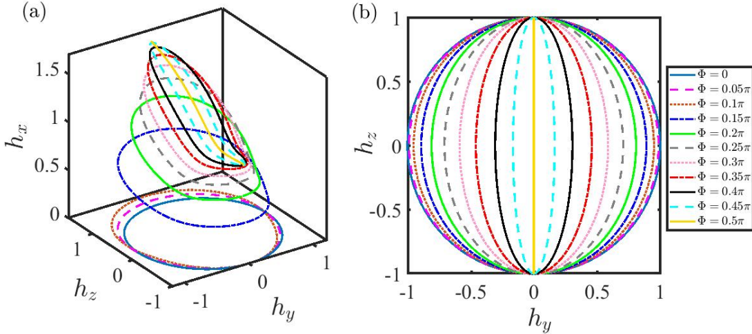
Figure 3.16: Curves traced out by the Hamiltonian in the Brillouin zone. Left panel shows the correlated system, \delta = \cos(\phi) , V = 1 + 4\sin(\phi) . On the right panel \delta = \cos(\phi) , V = 1 . For both panels, the values of the variable \phi are indicated in the legend on the right.
