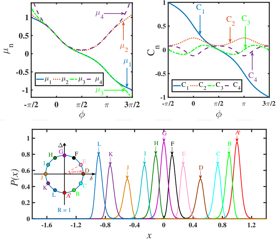
Figure 3.11: Moments, cumulants, and probability distribution along a circle of radius 1 in the \Delta/t vs. \delta/t plane. In these calculations t = 1 . The path encircles the topological point \Delta/t = 0, \delta/t = 0 . The top panels show the gauge invariant moments and cumulants along the circle as a function of angle. The lower panel follows the evolution of the probability distribution. The point A^* is at an angle \phi = -\pi/2 + 2\pi/1000 , not \phi = -\pi/2 . In the lower panel the unit of x is the lattice constant. The points \phi = -\pi/2, 3\pi/2 are excluded from the curves shown in the upper panels.
