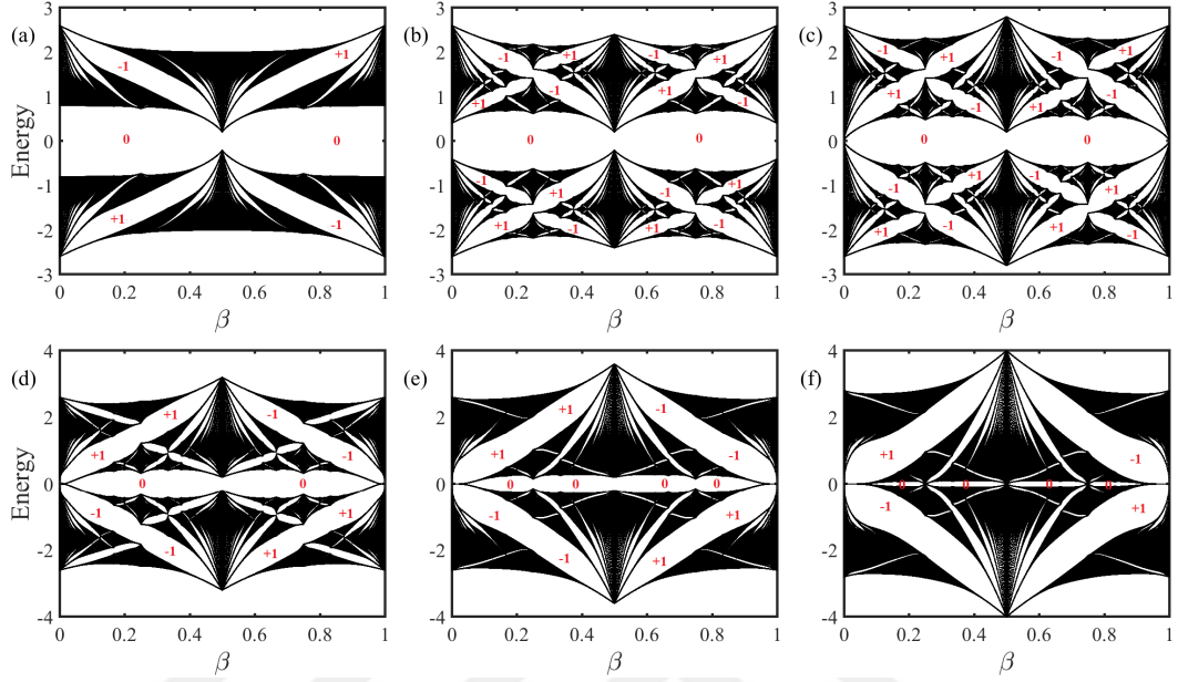
Figure 6.8: Hofstadter butterfly: energy spectrum as a function of magnetic flux per plaquette \beta in Aubry-André lattice with V = 0 , \tau = 0.3 , \Delta = 0.4 , and (a) \delta = 1 , (b) \delta = 0.2 , (c) \delta = 0.4 , (d) \delta = 0.6 , (e) \delta = 0.8 , (f) \delta = 1 .
