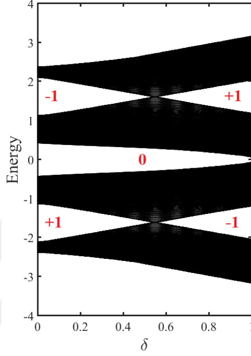
Figure 6.11: The evolution of the energy bands for \beta = 0.25 , V = 1 , \tau = 0.3 , and \Delta = 0.4 as function of \delta shown in Fig. (6.10). Gaps are labeled with their Chern numbers.
