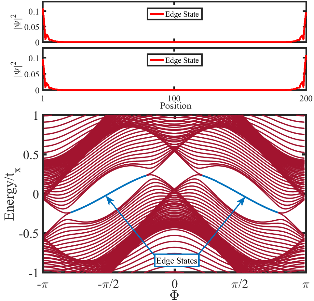
Figure 4.3: Lower panel: band structure of a system of size 100 sites with open boundary conditions. In this calculation t_x = 1 , t_y = 1 , and t_{xy} = 0.3 . Inside the lobes (see inset of Fig. 4.2) edge states arise. Upper two panel: squared modulus of the wavefunction for the two edge states averaged over the two legs of the ladder, for \Phi = \pi/2 for a system of 200 sites.
