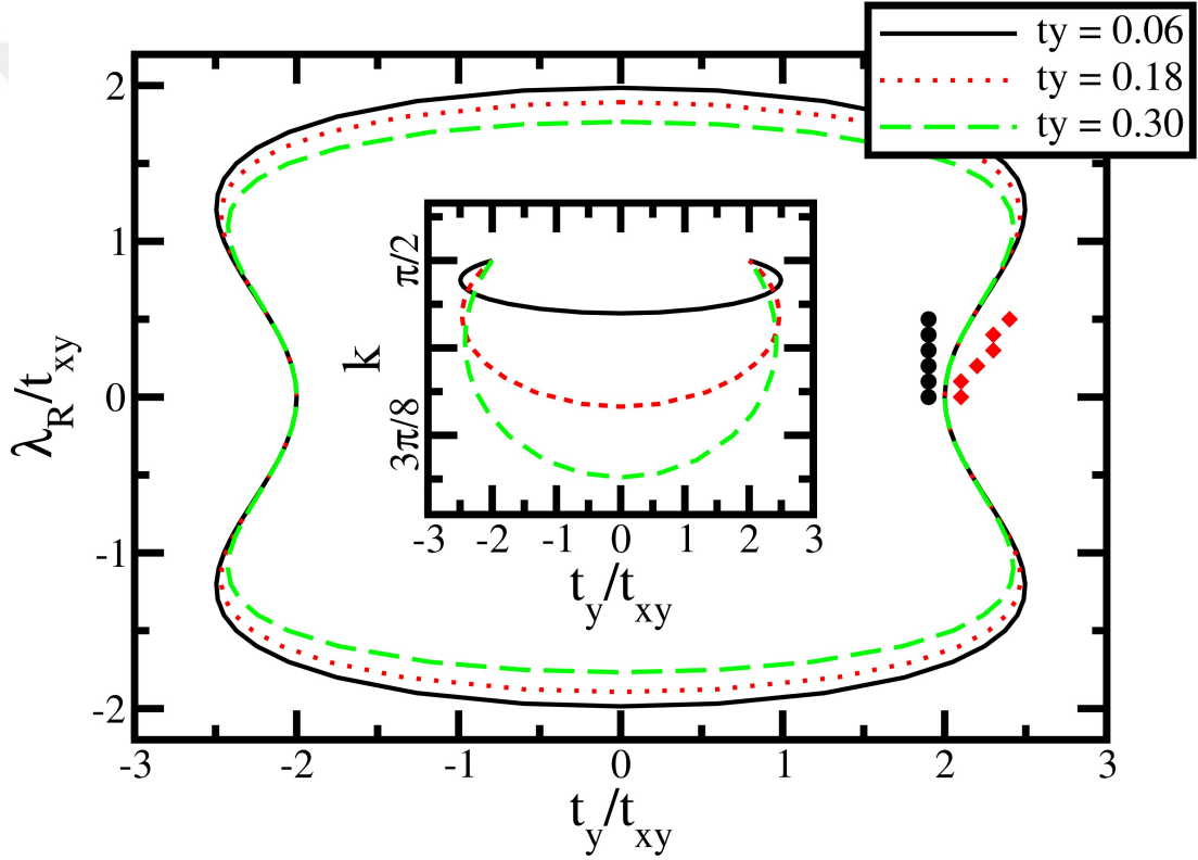
Figure 4.9: Main figure: phase diagram for systems with t_x = 1, t_{xy} = 0.06, 0.12, 0.18 in the t_y vs. \lambda_R plane. The inset indicates the k vector at which gap closure occurs as a function of t_y/t_{xy} . The black filled circles and red filled diamonds on the left side of the phase diagram indicate systems for which we have tested our Středa-Widom formula. For the black filled circles we found a quantized quantum spin Hall response, while we found no response for the red diamonds.
