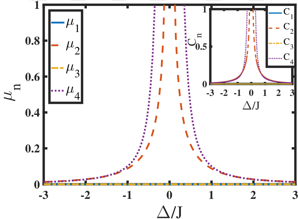
Figure 3.4: Moments for J'/J = 1 as a function of \Delta/J . In these calculations J = 1 . The inset shows the corresponding cumulants. In the limit \Delta/J \rightarrow 0 (the topological point of the model) the even cumulants diverge, while the odd cumulants are always zero for this case.
