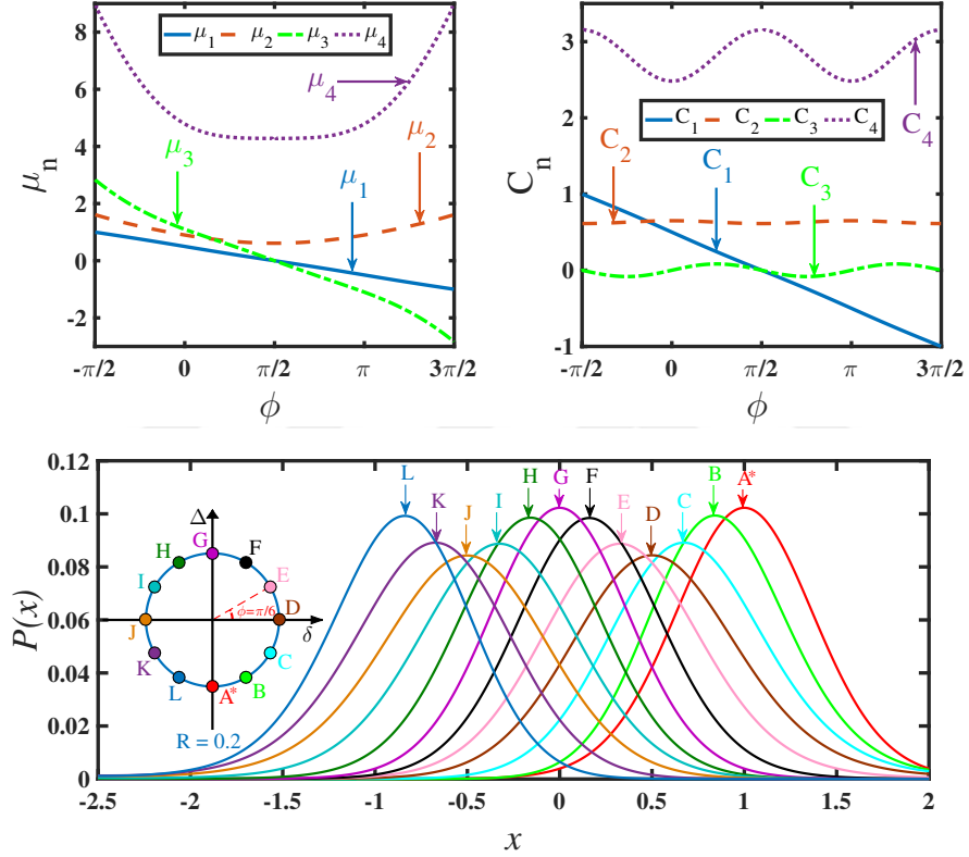
Figure 3.12: Moments, cumulants, and probability distribution along a circle of radius 0.2 in the \Delta/t vs. \delta/t plane. In these calculations t = 1 . The path encircles the topological point \Delta/t = 0, \delta/t = 0 . The upper panel shows the gauge invariant moments and cumulants along the circle as a function of angle. The top panels shows the gauge invariant moments and cumulants along the circle as a function of angle. The lower panel follows the evolution of the probability distribution. The point A^* is at an angle \phi = -\pi/2 + 2\pi/1000 , not \phi = -\pi/2 . In the lower panel the unit of x is the lattice constant. The points \phi = -\pi/2, 3\pi/2 are excluded from the curves shown in the upper panels.
