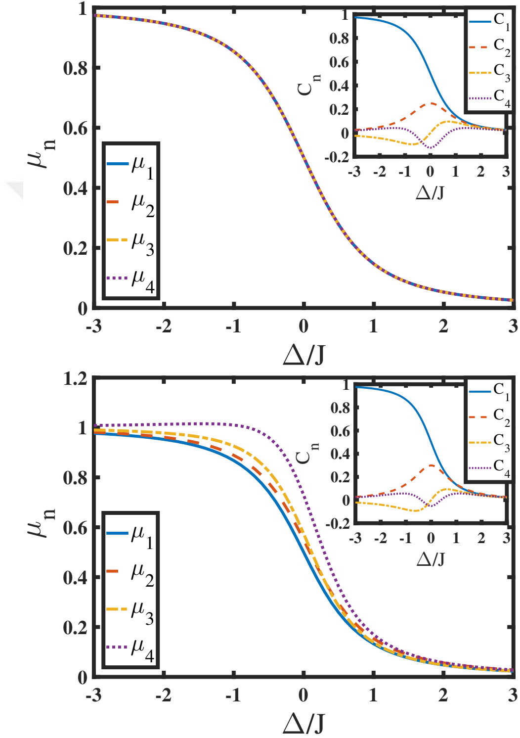
Figure 3.2: Moments for J'/J = 0 (upper panel) and 0.3 (lower panel) as a function of \Delta/J . In these calculations J = 1 . For J'/J = 0 the curves are identical. The insets show the corresponding cumulants.
