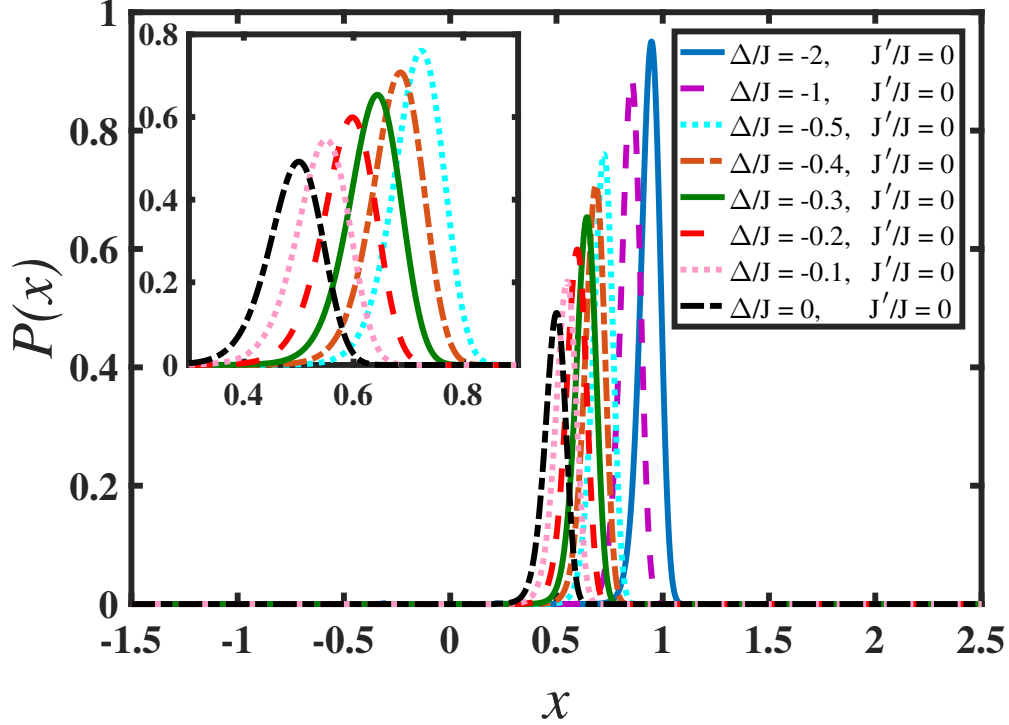
Figure 3.6: Normalized probability distribution of the polarization for different parameters of the Rice-Mele Hamiltonian. In these calculations J = 1 . The unit of length in these figures is the lattice constant. Different values of \Delta/J are shown for J'/J = 0.0 . In the topmost panel ( J'/J = 0 ) the inset shows the distribution for the cases \Delta/J = 0.0, -0.1, -0.2, -0.3, -0.4, -0.5
