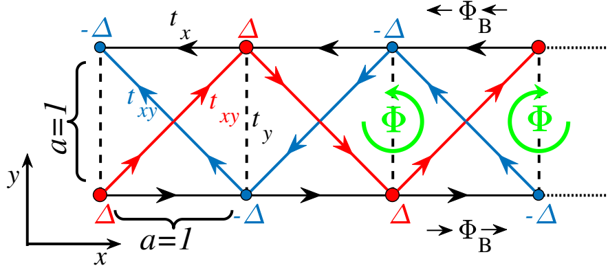
Figure 4.1: Ladder model. The hopping parameters are defined as follows: t_x denotes hopping along the legs of the ladder, t_y denote the hoppings perpendicular to legs, t_{xy} denotes hoppings occurring diagonally between legs, connecting second nearest neighbors. The sites in red(blue) indicate where the site dependent potential is positive(negative). A Peierls phase of \Phi is introduced along the diagonal hoppings. These can be thought of as arising from magnetic impurities residing halfway through the perpendicular ( t_y ) hoppings and arranged antiferromagnetically.
