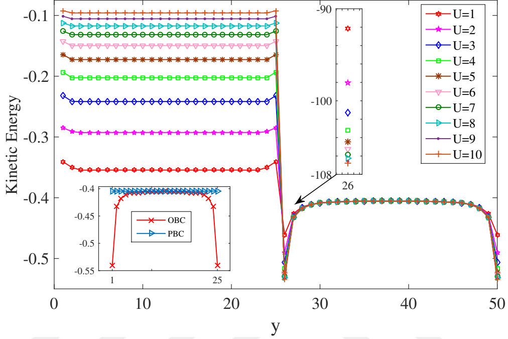
Figure 5.4: Kinetic energy resolved to bonds parallel to the interface for different values of U . The variable y indicates the y -coordinate of the bonds according to Figure 5.1. Clearly, the kinetic energy is peaked (in the negative direction) at the interface. The inset shows the value of the kinetic energy for bonds running along the interface for different values of U . The size of the systems studies is 50 \times 200 .
