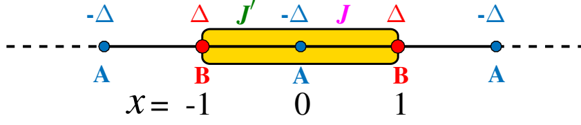
Figure 3.1: Schematic representation of the Rice-Mele model. \Delta represents the on-site potential, A and B refer to the different sublattices. J and J' are the alternating hoppings. The unit cell is indicated in yellow. The x label corresponds to localization within the unit cell ( -1 < x < 1 ). The variable x is continuous, below, in our subsequent calculations, the probability distribution will be shown as a function of x . The unit of x is the lattice constant.
