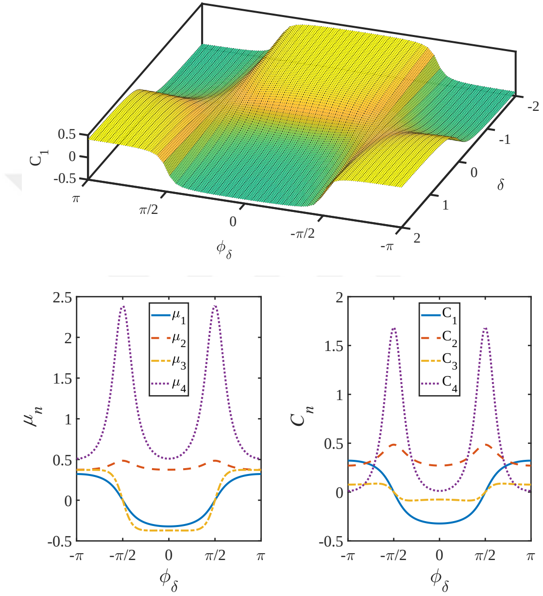
Figure 2.5: Moments and cumulants of GAA model for \delta = 0.5 , \phi_V = 0 , and V = 0.5 as a function of \phi_\delta .
