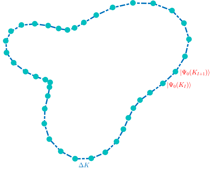
Figure 2.1: Discrete representation of a closed curve in parameter space.
