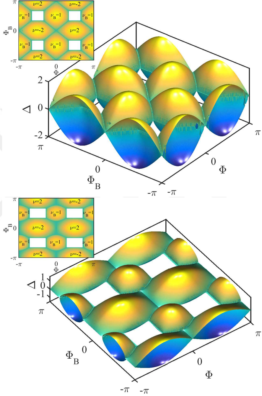
Figure 4.4: Examples of phase diagrams in three dimensions. The upper(lower) panel shows the phase diagram \Delta , \Phi , \Phi_B for t_x = t_y = t_{xy} = 1 ( t_x = t_y = 1, t_{xy} = 0.75 ). The phase diagram was determined by searching for the gap closure.
