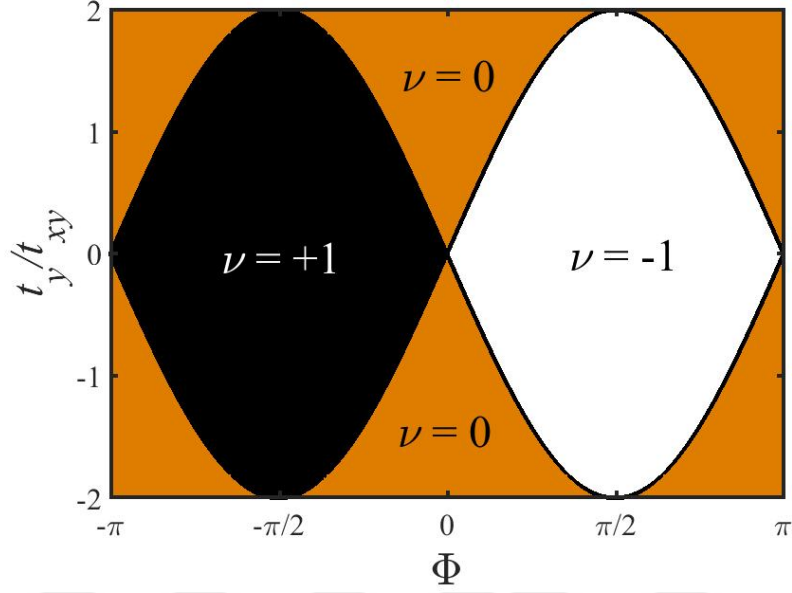
Figure 4.7: Phase diagram of the system where gap closure occurs. The numbers in the figures denote the topological winding number.
