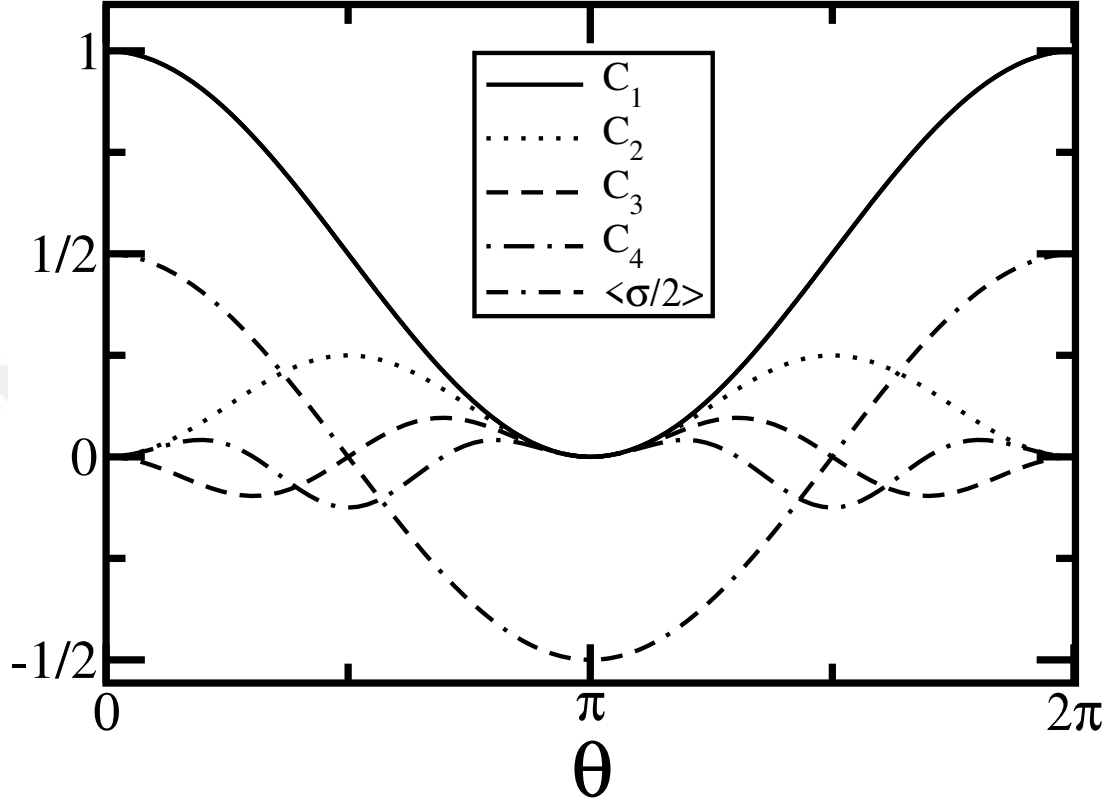
Figure 2.2: Cumulants of a spin- \frac{1}{2} particle in a precessing field.
