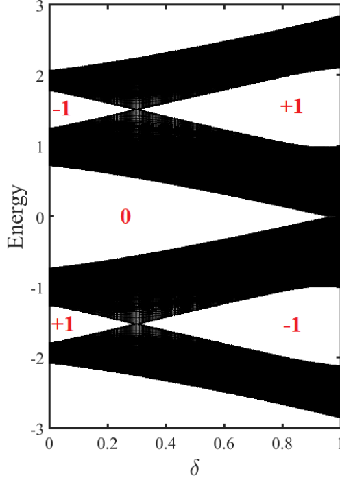
Figure 6.9: The evolution of the energy bands for \beta = 0.25 , V = 0 , \tau = 0.3 , and \Delta = 0.4 as function of \delta shown in Fig. (6.8). Gaps are labeled with their Chern numbers.
