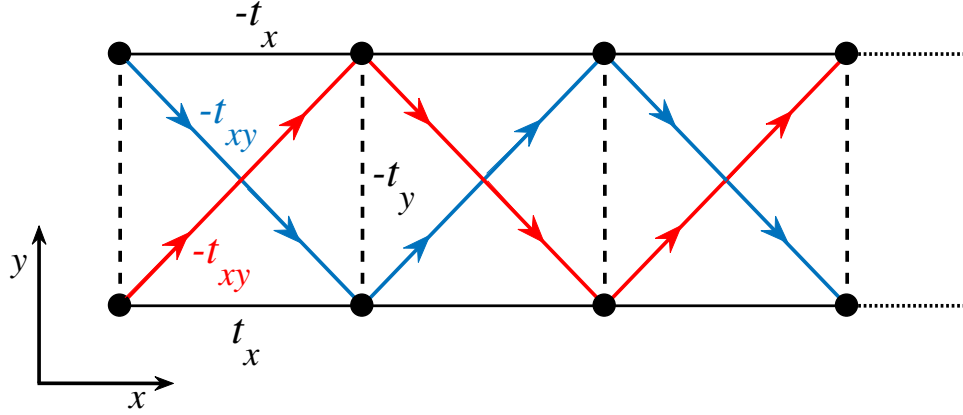
Figure 4.6: Graphic representation of our model. t_x(t_y) denotes hoppings along horizontal(vertical) bonds. t_{xy} denotes diagonal bonds. We apply Peierls phases along the diagonal bonds along the directions indicated.
