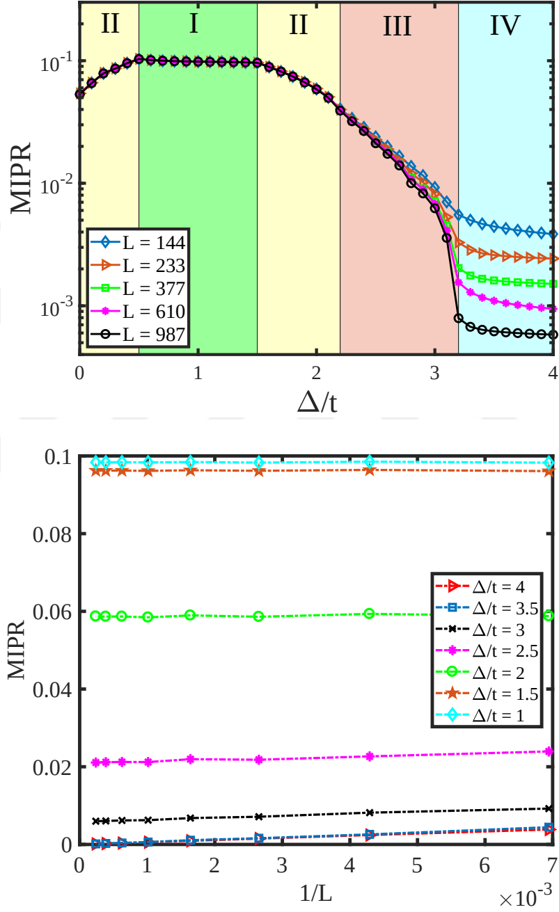
Figure 6.6: Upper panel: MIPR (log-scale) as a function of p -wave superfluid pairing \Delta/t for different chain lengths L for \tau = 1 and \delta/t = 0.5 . Bottom panel: MIPR with the inverse system size 1/L . For the extended phase, MIPR tends to zero as L increases.
