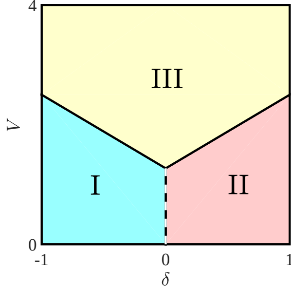
Figure 3.15: Phase diagram. I and II are SSH states (Hartree-Fock approximation). III is a CDW type phase, with finite skew when \delta differs from zero. The dashed line indicates a Fermi sea (ideal conductor).
