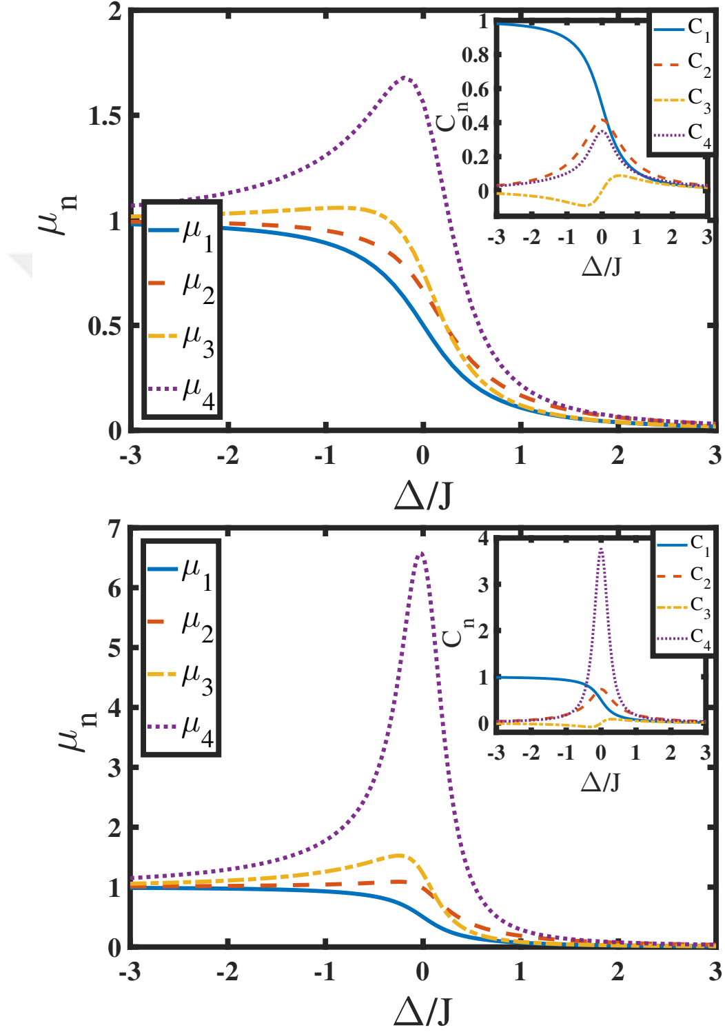
Figure 3.3: Moments for J'/J = 0.5 (upper panel) and 0.7 (lower panel) as a function of \Delta/J . In these calculations J = 1 . The insets show the corresponding cumulants.
