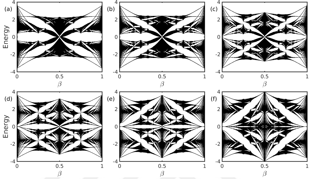
Figure 6.10: Hofstadter butterfly: energy spectrum as a function of magnetic flux per plaquette \beta in Aubry-André lattice with V = 1 , \tau = 0.3 , \Delta = 0.4 , and (a) \delta = 1 , (b) \delta = 0.2 , (c) \delta = 0.4 , (d) \delta = 0.6 , (e) \delta = 0.8 , (f) \delta = 1 .
