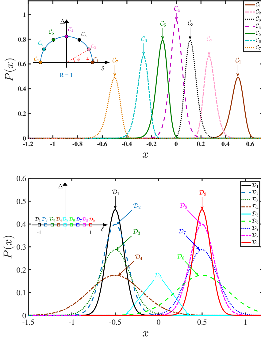
Figure 3.19: Reconstructed polarization for the Rice-Mele model along the paths indicated in the inset of each plot. The paths are represented on the \delta - \Delta plane.
