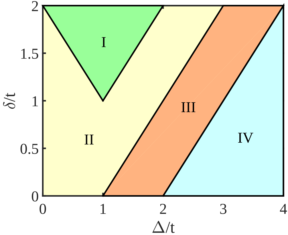
Figure 6.7: Phase diagram of the generic GAAH model with the p -wave incommensurate modulation amplitude 0 < \delta \leq 2 and the p -wave pairing strength 0 \leq \Delta \leq 4 . The hopping incommensurate modulation amplitude is set to \tau = 1 , the on-site potential incommensurate modulation amplitude is set to V/t = 1 , and the phase in the incommensurate modulation is set to k_y = \pi/2 and \varphi = \beta\pi . The phases are (I) localized phase, (II) critical localized phase, (III) critical extended phases, (IV) extended phases.
