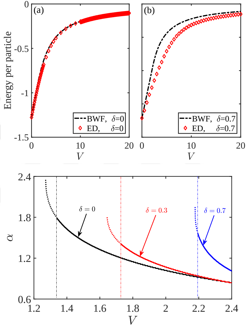
Figure 3.14: Upper panel: The variational ground state energy per particle for (a) \delta = 0 , and (b) \delta = 0.7 based on the Baeriswyl wave function compared to exact diagonalization for 12 lattice sites. Lower panel: the variational parameter as a function of interaction strength for \delta = 0, \pm 0.3 and \pm 0.7 . Solid lines indicate the global minimum in the CDW type insulating phase. Dashed lines indicate metastable insulating phases on the metallic side of the phase diagram.
