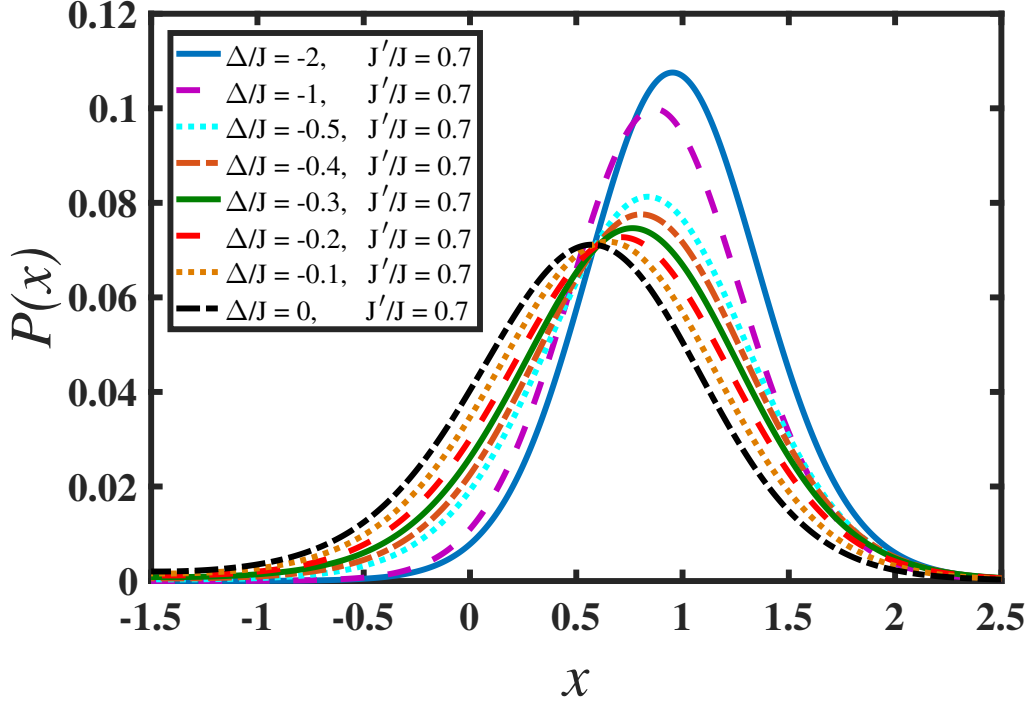
Figure 3.9: Normalized probability distribution of the polarization for different parameters of the Rice-Mele Hamiltonian. In these calculations J = 1 . The unit of length in these figures is the lattice constant. Different values of \Delta/J are shown for J'/J = 0.7 . In the topmost panel ( J'/J = 0 ) the inset shows the distribution for the cases \Delta/J = 0.0, -0.1, -0.2, -0.3, -0.4, -0.5
