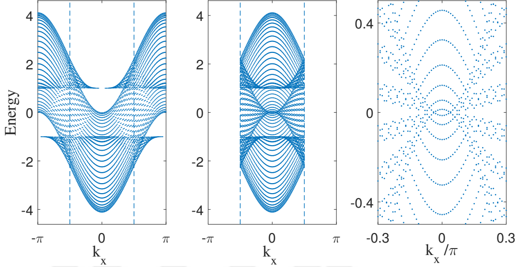
Figure 5.2: Band structure of the model with U = 1 as a function of k_x . The lattice is bipartite in the x -direction, the Brillouin zone in this direction is halved (restricted Brillouin zone). The left side is the raw data, the center plot is the data in the restricted Brillouin zone, the right shows the band structure zoomed to near the Fermi level at half-filling.
