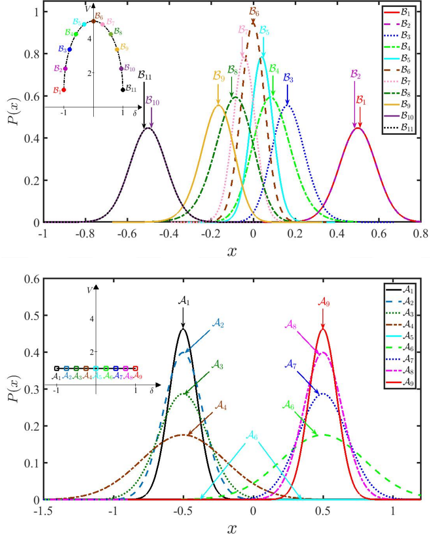
Figure 3.18: Reconstructed polarization distributions along the two paths shown indicated in Fig. 3.17. The upper panel(lower panel) shows reconstructed polarizations along the ellipse(straight line) between the points -1, 1 to 1, 1 on the \delta - V plane.
