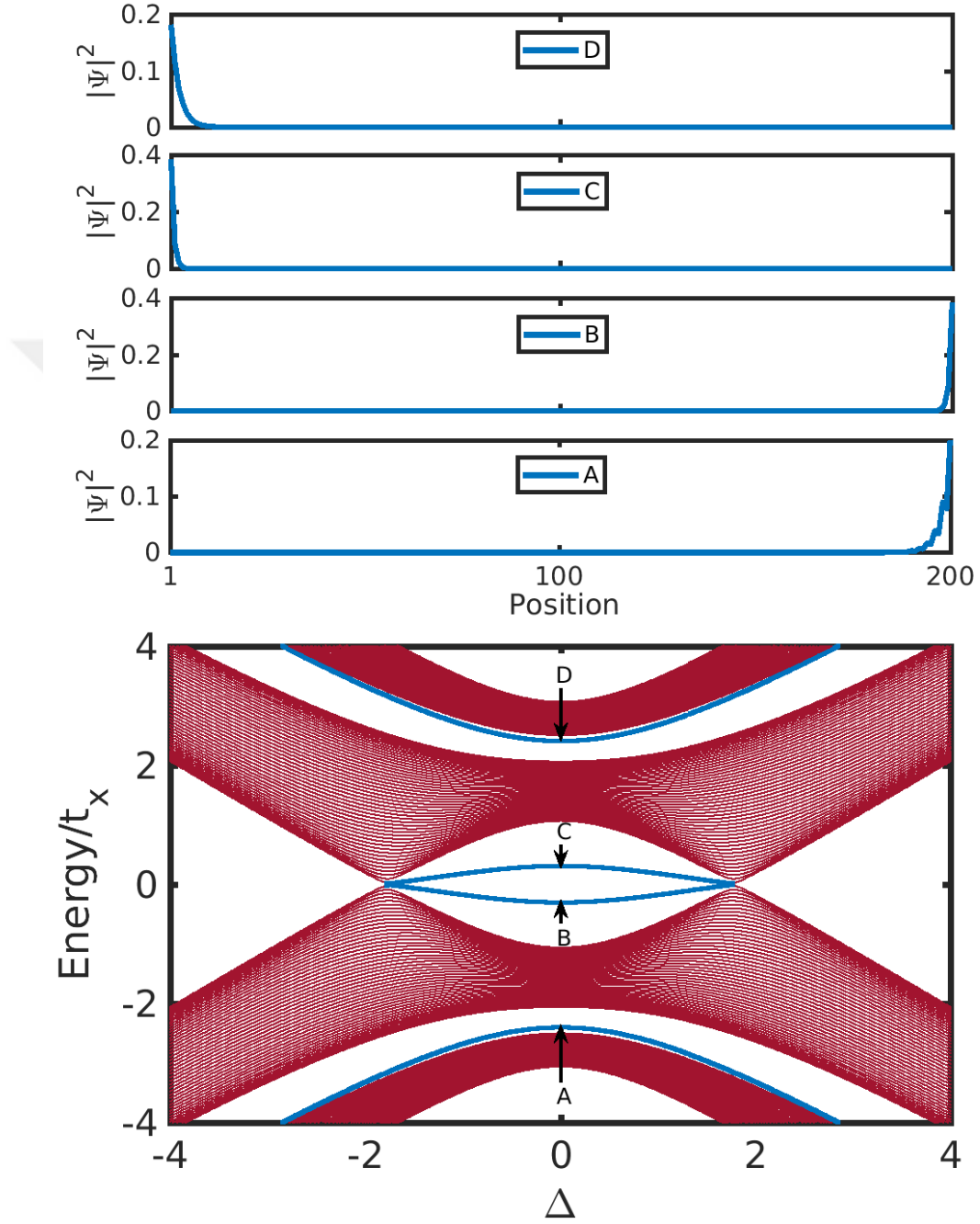
Figure 4.5: Band structure of system with finite \Gamma = 0.5 and edge states (upper four panels). The other parameters are t_x = t_y = t_{xy} = 1 , \Phi = \pi/2 , and \Phi_B = 0 . The variable \Delta is scanned. Localized edge states are found at quarter, half, and three-quarter fillings.
