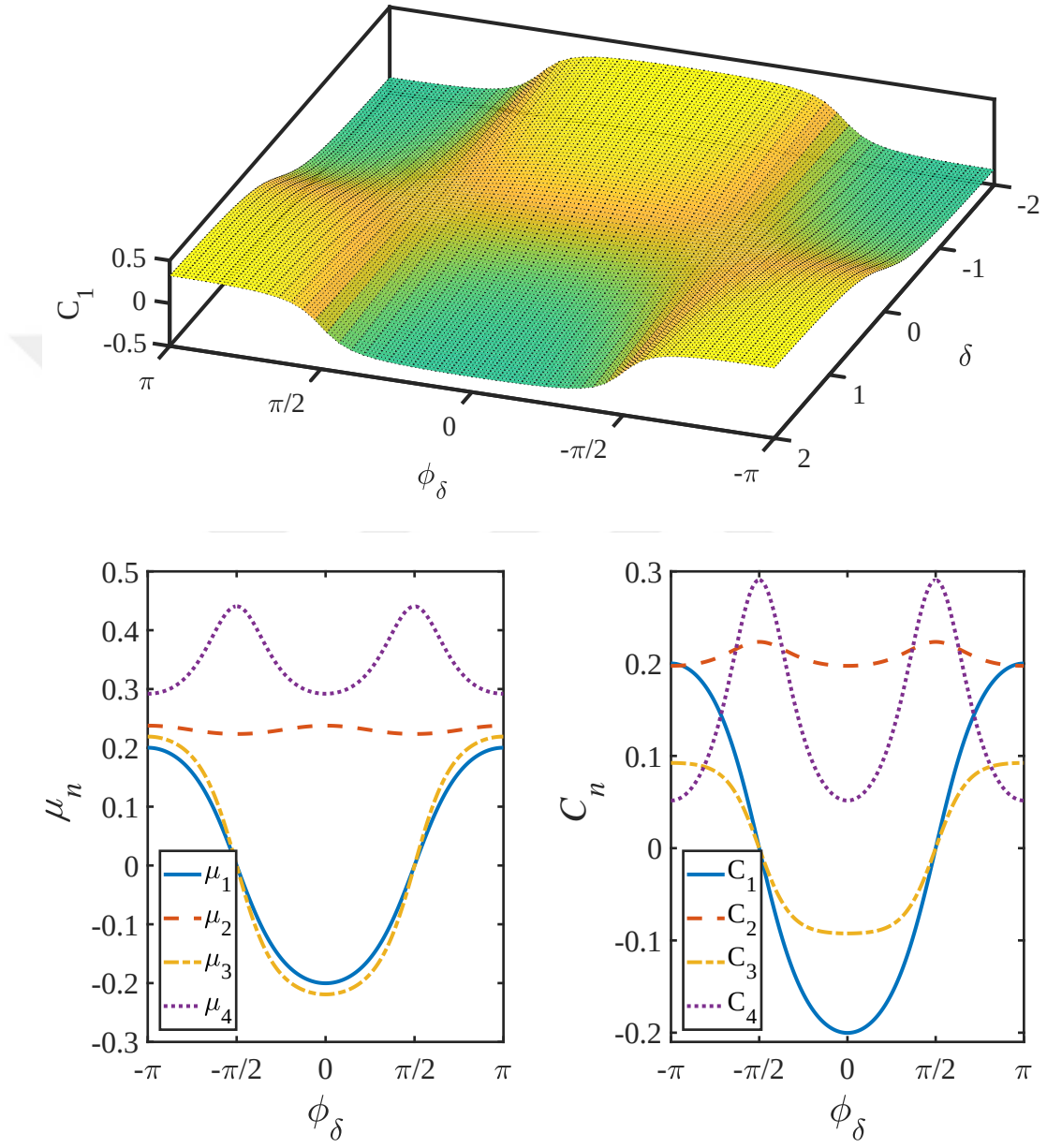
Figure 2.6: Moments and cumulants of GAA model for \delta = 0.5 , \phi_V = 0 , and V = 1 as a function of \phi_\delta .
