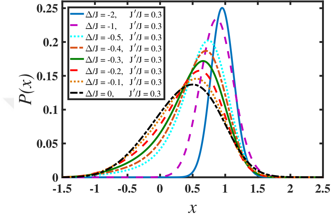
Figure 3.7: Normalized probability distribution of the polarization for different parameters of the Rice-Mele Hamiltonian. In these calculations J = 1 . The unit of length in these figures is the lattice constant. Different values of \Delta/J are shown for J'/J = 0.3 . In the topmost panel ( J'/J = 0 ) the inset shows the distribution for the cases \Delta/J = 0.0, -0.1, -0.2, -0.3, -0.4, -0.5
