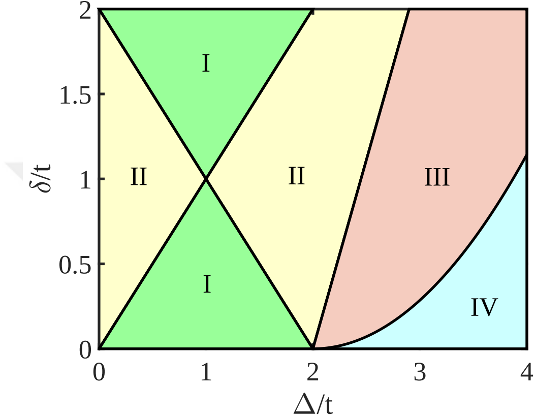
Figure 6.5: Phase diagram of the off-diagonal GAAH model with the p -wave incommensurate modulation amplitude 0 < \delta \leq 2 and the p -wave pairing strength 0 \leq \Delta \leq 4 . The hopping incommensurate modulation amplitude is set to \tau = 1 and the phase in the incommensurate modulation is set to k_y = \pi/2 and \varphi = \beta\pi . The phases are (I) localized phase ( |\delta - \tau| ), (II) critical localized phase, and (III) extended phases.
