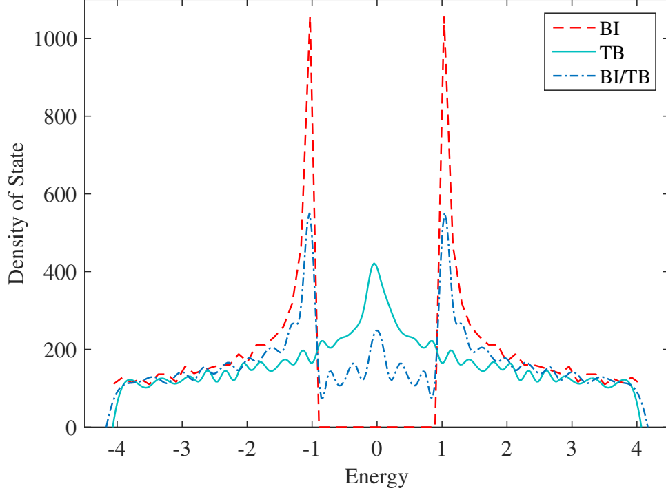
Figure 5.3: Density of states for crystalline insulator, tight-binding, and model with an interface between the two ( U = 1 ). The crystalline insulator is gapped, the system with interface is not gapped, but the density is smaller near E = 0 than in the tight-binding system.
