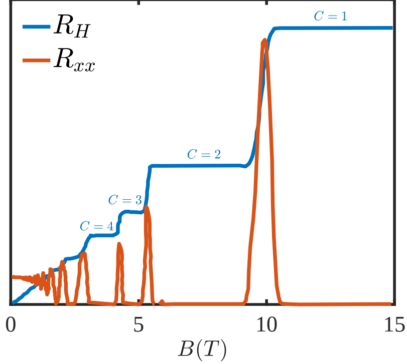
Figure 1.1: This is the integer quantum Hall effect. R_H is the Hall resistance and R_{xx} is the longitudinal resistance.
