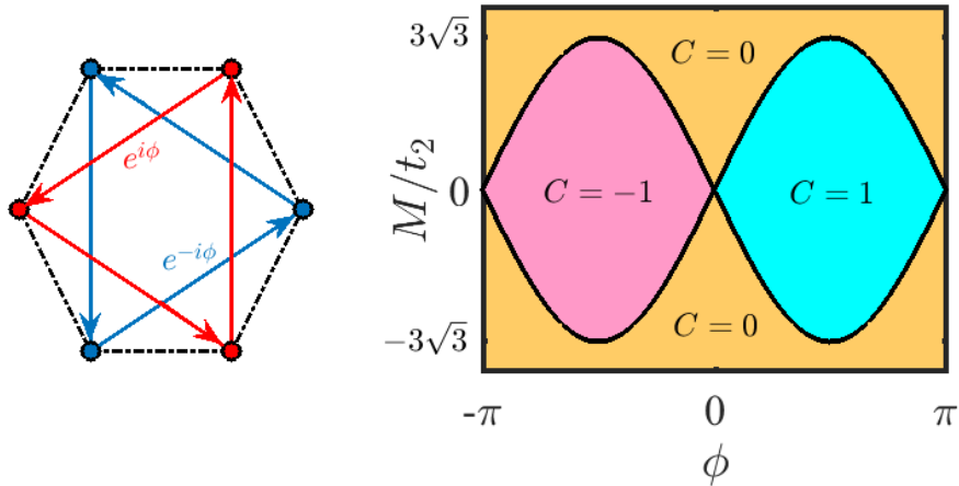
Figure 1.3: Phase diagram of the Haldane model as a function of \phi and M/t_2 .
