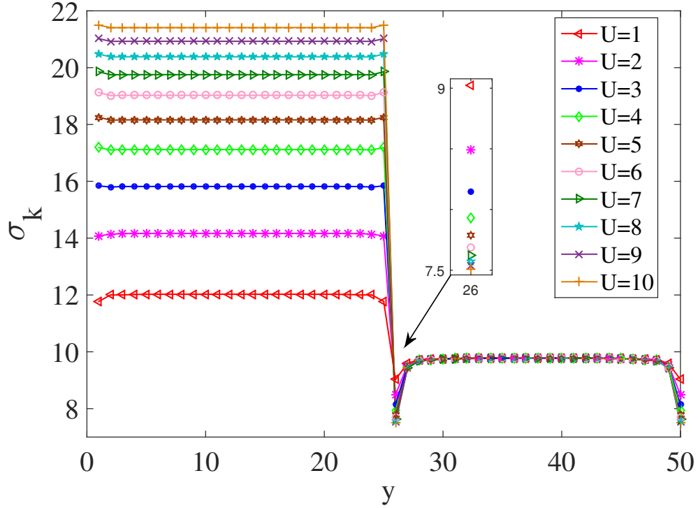
Figure 5.6: Spread in the total momentum resolved as a function of y coordinate for different values of the strength of the external potential. The spread in the total momentum is minimized at the interface. The size of the systems studied was 50 \times 200 .
