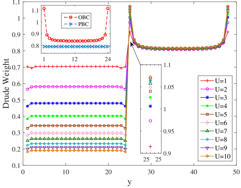
Figure 5.5: The Drude weight (resolved to bonds along the y direction) as a function of y coordinate for different values of the strength of the external potential U . The Drude weight is peaked at the interface. The left inset shows the resolved Drude weight for a tight-binding model with periodic and open boundary conditions. The right inset shows the value of the Drude weight for the interface. The Drude weight is peaked at the interface. The value at the peak increases as a function of U . The size of the systems is 48 \times 200 .
