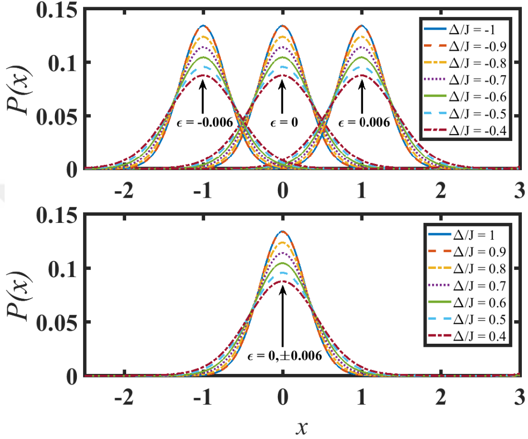
Figure 3.10: Normalized probability distribution of the polarization for cases J' = J and J' = J \pm \epsilon ( \epsilon = 0.006 ). In these calculations J = 1 . The unit of length is the lattice constant. Different values of \Delta/J are shown. Upper panel(lower panel): \Delta/J < 0 ( \Delta/J > 0 ).
