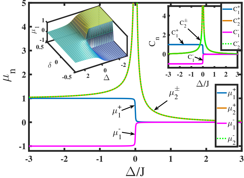
Figure 3.5: First two moments and cumulants (right inset) for J = 1 , J' = J \pm 0.006 . Left inset shows the first moment on the \Delta - \delta plane, indicating the singular behavior along the line \Delta < 0, \delta = 0 .
