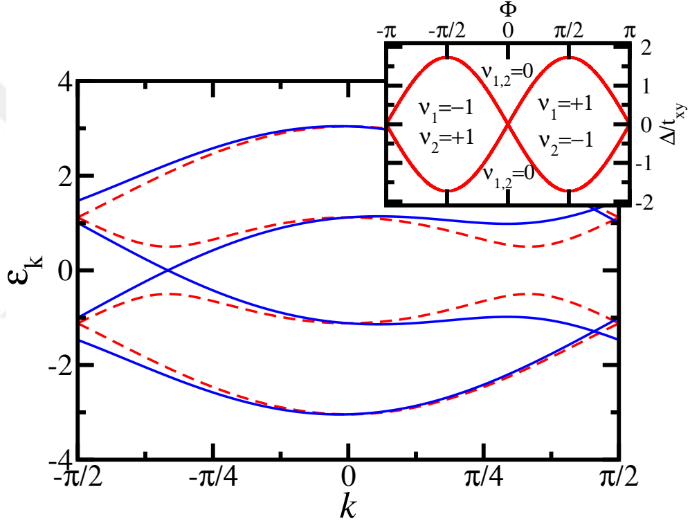
Figure 4.2: Band structure within the reduced Brillouin zone (RBZ). The red dashed lines indicate the band structure for a system with t_x = 1, t_y = 1, t_{xy} = 0, \Delta = 0.5 . At half-filling this system is gapped. For t_y = 0 the gaps would be at the edge of the RBZ ( k = \pm \frac{\pi}{2} ). Finite t_y causes the gaps to move towards the origin (the gap is at k^\pm = \pm \arccos(\frac{t_y}{2t_x}) ). The blue solid lines indicate gap closure when t_{xy} is made finite ( t_{xy} \sin(k^\pm) \sin(\Phi) = \Delta, (\Phi = \frac{\pi}{2}) ). The inset shows the phase diagram (where gap closure occurs) for t_x = 1, t_y = 1 . The lines separate two insulating phases. The red(black) lines indicates gap closure occurring at k^+(k^-) .
