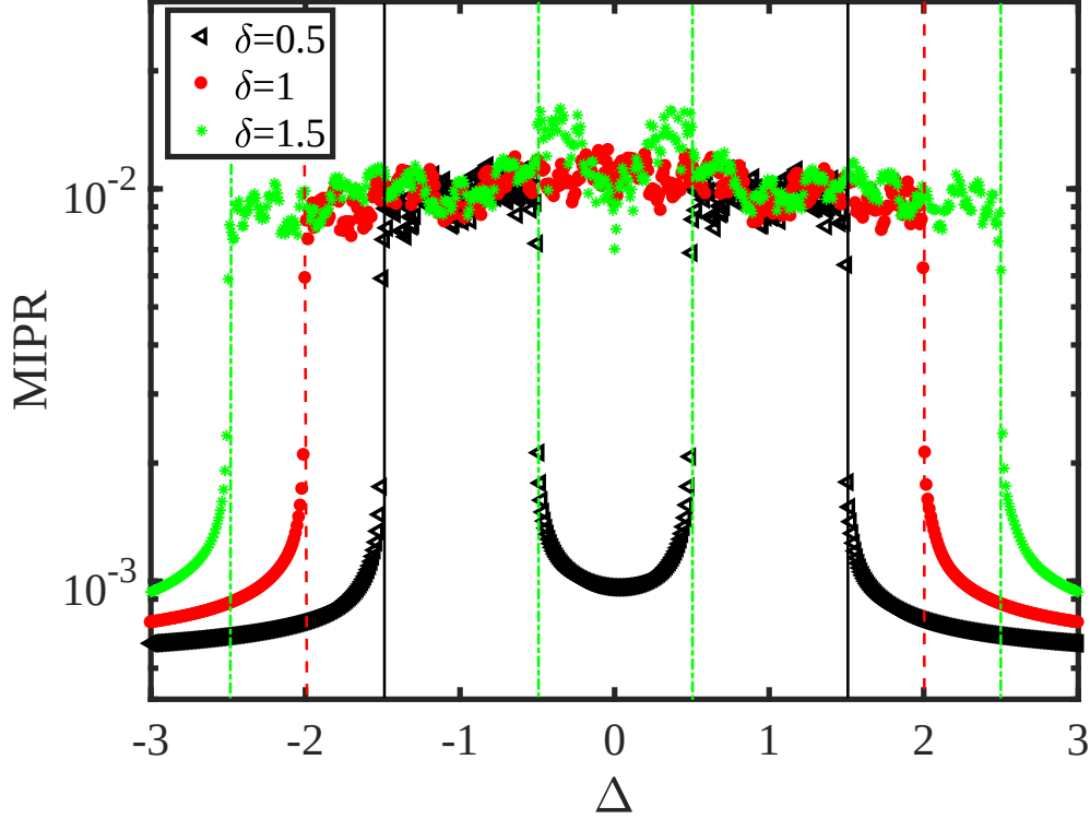
Figure 6.4: MIPR as a function of p -wave superfluid pairing \Delta for the indicated values of modulation amplitude \delta . The dashed lines, dot-dashed lines, and solid lines demonstrate the abrupt changes of the MIPR at phase boundaries.
