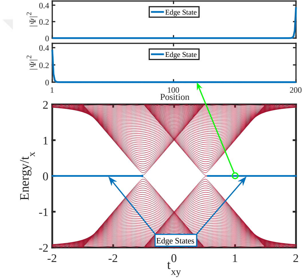
Figure 4.8: Energy spectrum of the shifted Creutz model with 200 sites, open boundary conditions as a function of t_{xy} . The parameters are t_x = 1 and t_y = 1 . The blue lines indicate states which are not present when periodic boundary conditions are applied. The square magnitude of these states are shown in the upper panels. They are localized near the edges of the chain.
