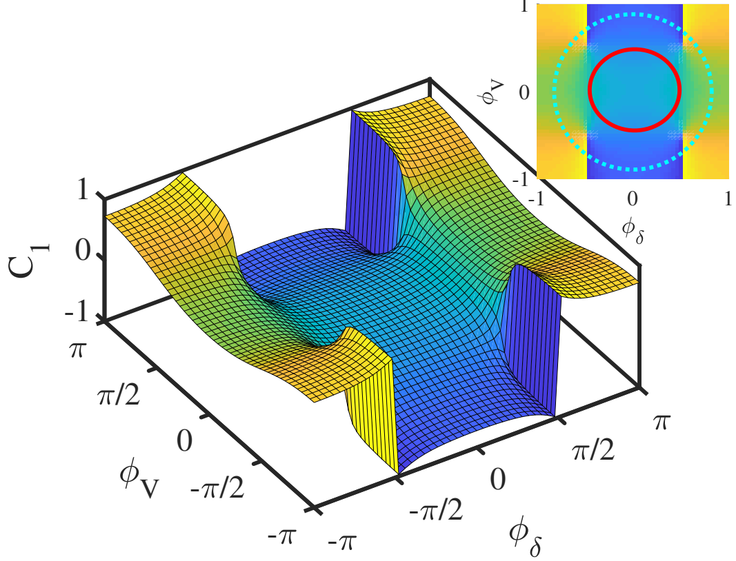
Figure 2.7: Polarization as a function of \phi_\delta and \phi_V in the pure commensurate modulations of GAA Hamiltonian. At \phi_\delta = 0 and \phi_V = 0 , if the radius of closed path encloses it is larger than \pi/2 , there are four singularities (from the first cumulant in a 3D plot we can appreciate the singularities) and the change in polarization is equal to e/2 (dash line circle of right inset). Also, if the radius of close path is smaller than \pi/2 , the change in polarization is equal to zero (solid line circle of right inset).
