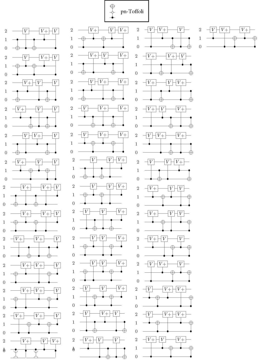
Figure A.2 : Subgates of Toffoli with positive and negative control lines.
