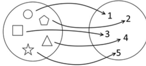
Figure 3.1 : Bijection Function.
