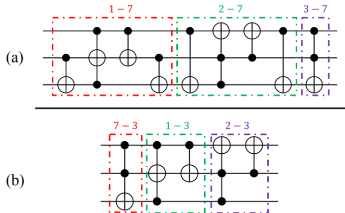
Figure 4.7 : Representations of the functions in Table 4.4. (a) TD approach, (b) OPT approach.
