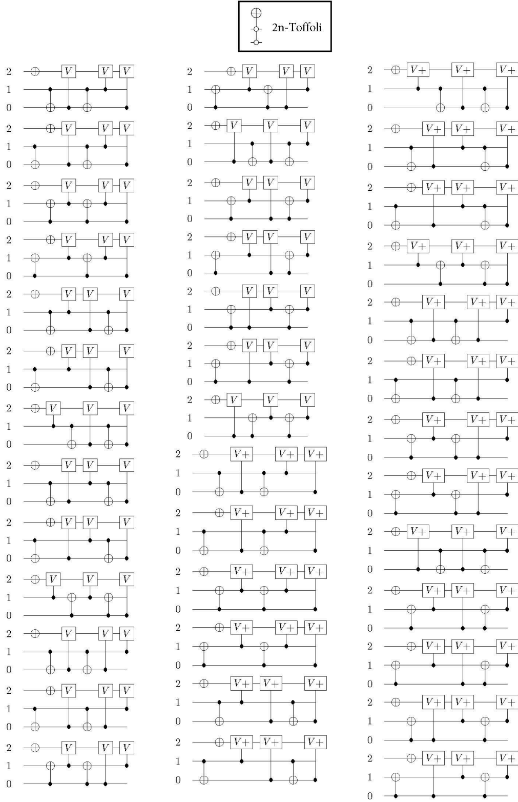
Figure A.3 : Subgates of Toffoli with negative control lines.
