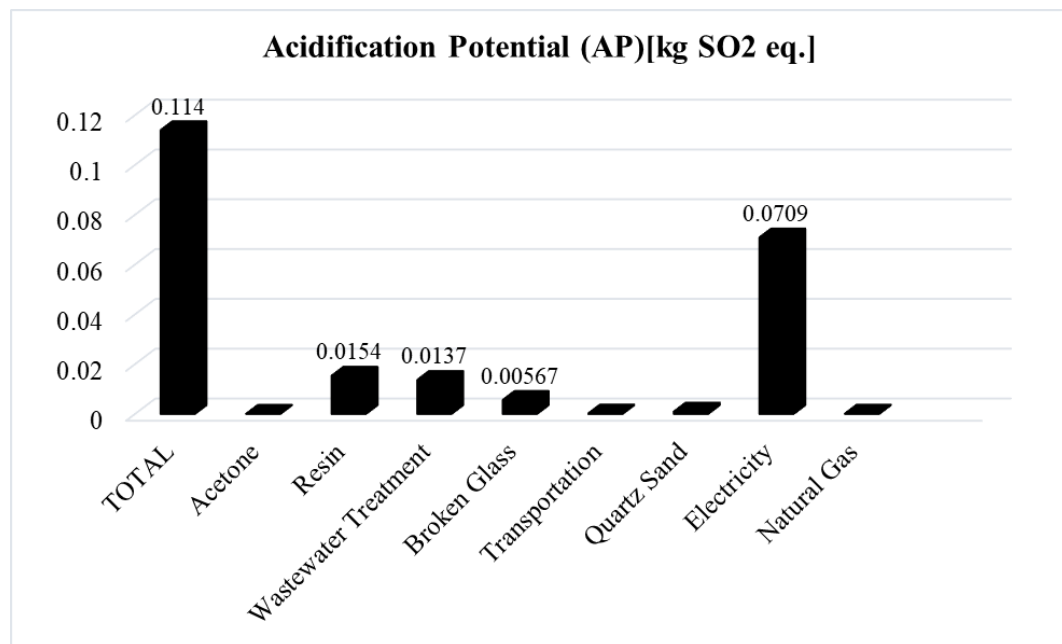
Figure 5.2 Acidification potential
